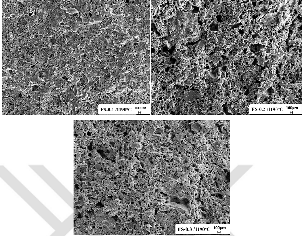
Görsel 7.7. FS-0.1 ( 2,0\text{gr/cm}^3 ); FS-0.2 ( 1,61\text{gr/cm}^3 ), FS-0.3 ( 1,67\text{gr/cm}^3 ) bünyeleri
