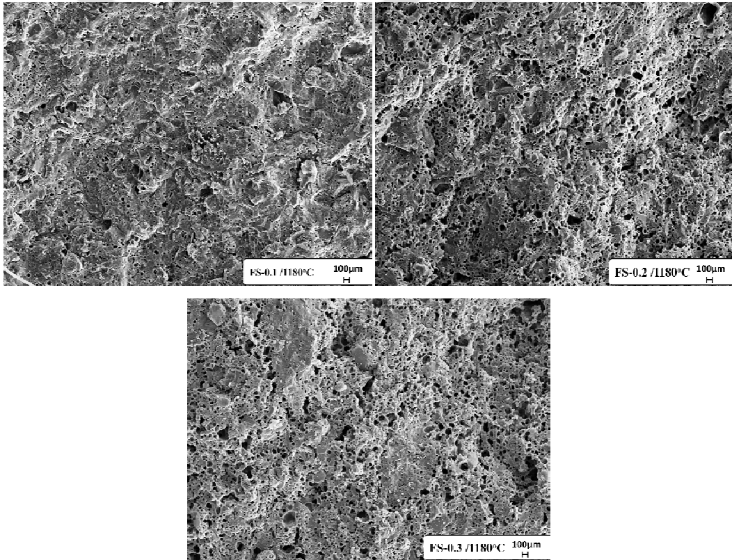
Görsel 7.6. FS-0.1 ( 2,24\text{gr}/\text{cm}^3 ); FS-0.2 ( 1,84\text{gr}/\text{cm}^3 ), FS-0.3 ( 1,77\text{gr}/\text{cm}^3 ) bünyeleri
