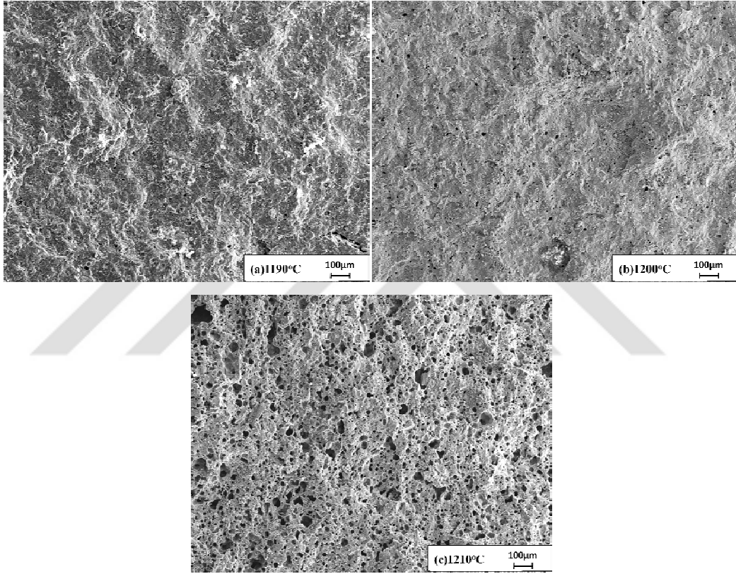
Şekil 7.9. FCe bünyeler ( \rho_{1190} : 2,45\text{gr}/\text{cm}^3 , \rho_{1200} : 2,42\text{gr}/\text{cm}^3 , \rho_{1210} : 1,81\text{gr}/\text{cm}^3 )
