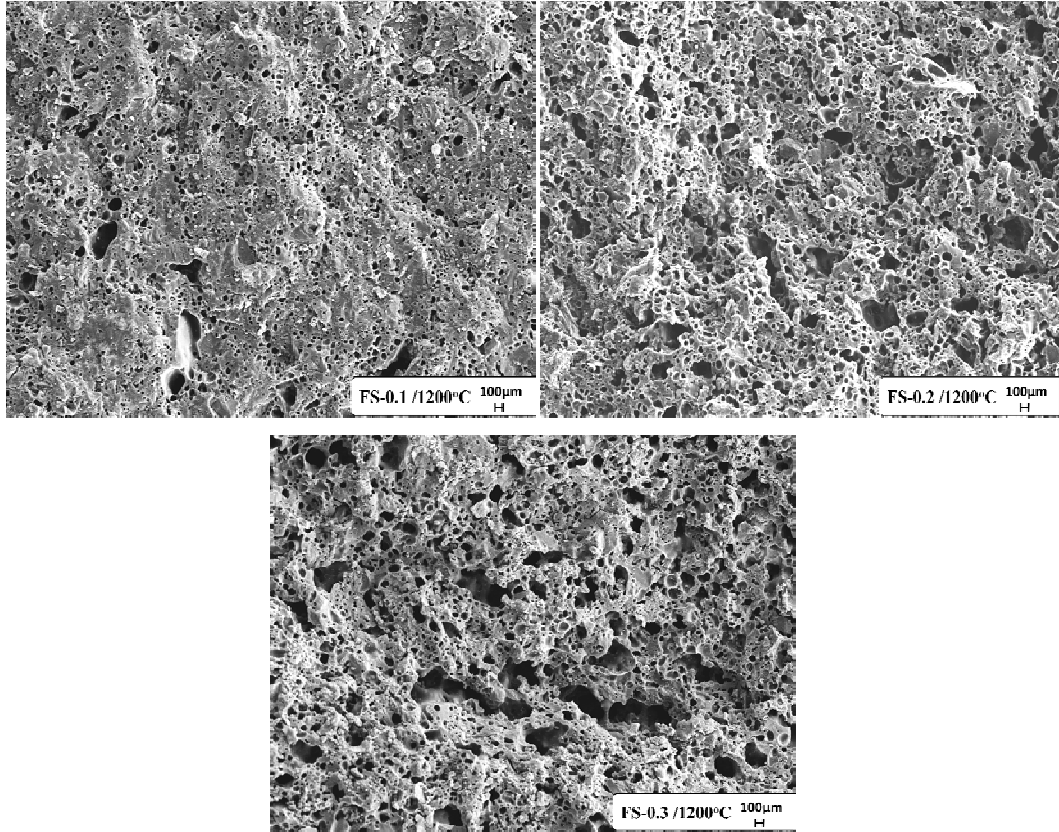
Görsel 7.8. FS-0.1 ( 1,82\text{gr/cm}^3 ); FS-0.2 ( 1,54\text{gr/cm}^3 ), FS-0.3 ( 1,57\text{gr/cm}^3 ) bünyeleri
