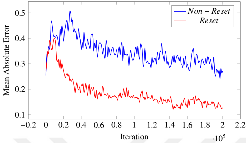
(a) Reset mechanism impact on MAE.
