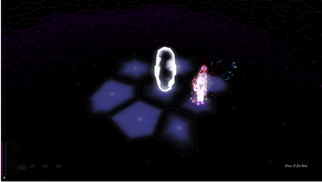
Figure 6.1: This figure shows the learning scenario. The agent is stimulated by positive reward when it navigates to the portal. Negative reward is given if it traverses out of bounds. After each trial, the agent respawns at a random Voronoi cell. The agent starts with random movement and learns better behaviors in terms of reward during the scenario.
