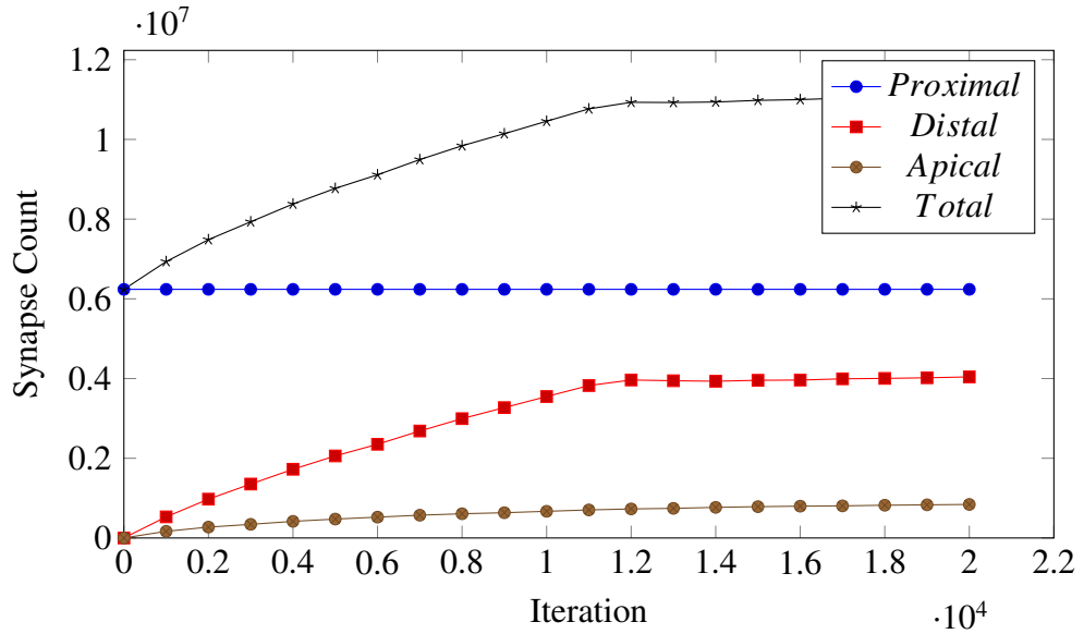
Figure 6.2: Synapse count increase with respect to iterations.
