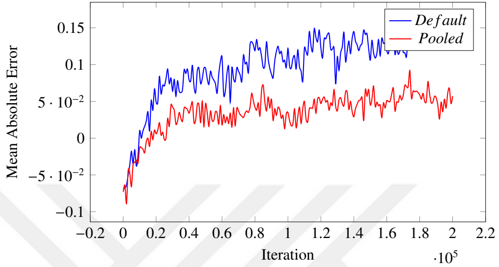
(a) The impact of segment eligibility traces feature on MAE.
