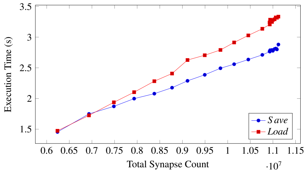
Figure 6.4: Serialization timings due to synapse count.
