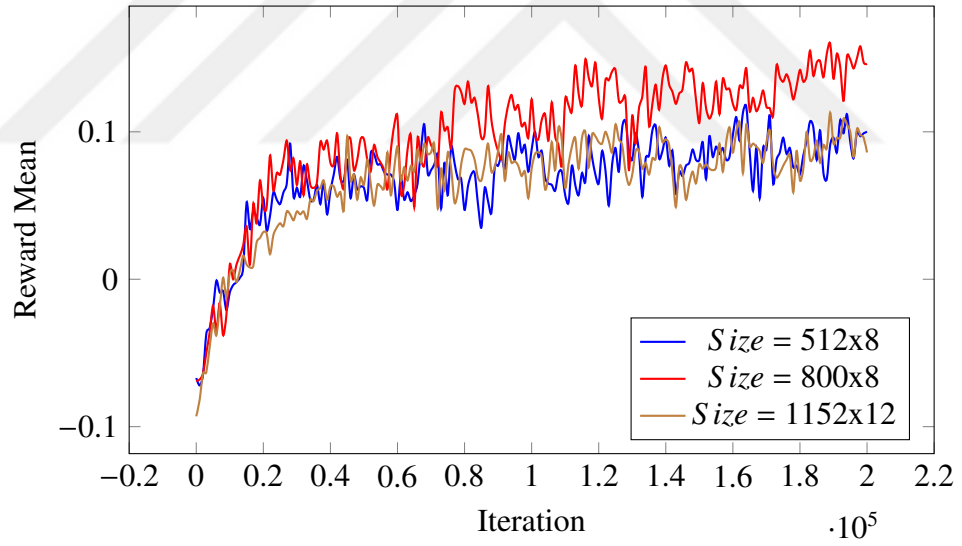
(b) The impact of layer size on reward measurements.
