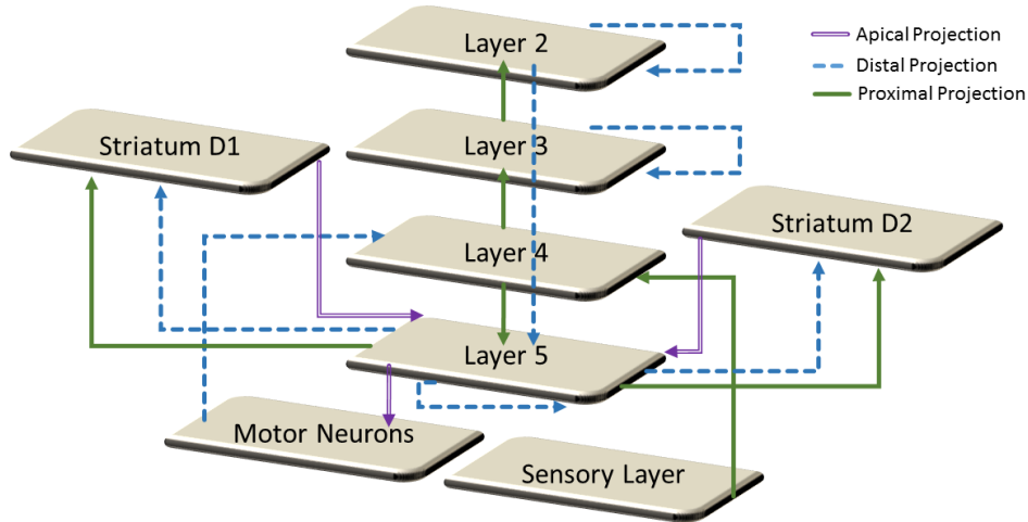
Figure 4.4: Information flow of our agent architecture. Layer 5 integrates information from most of the cortical layers.
