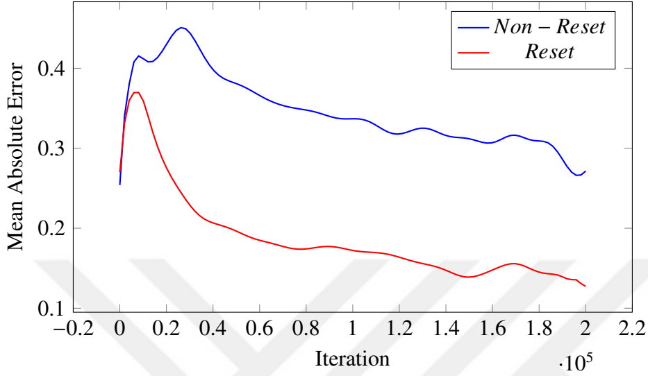
(a) Reset mechanism impact on MAE.
