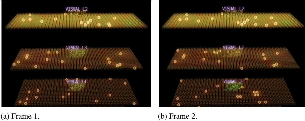
Figure 5.8: Layer 2 and 3 representations that are more stable and with smoother transitions compared to layer 4 on sequential frames.
