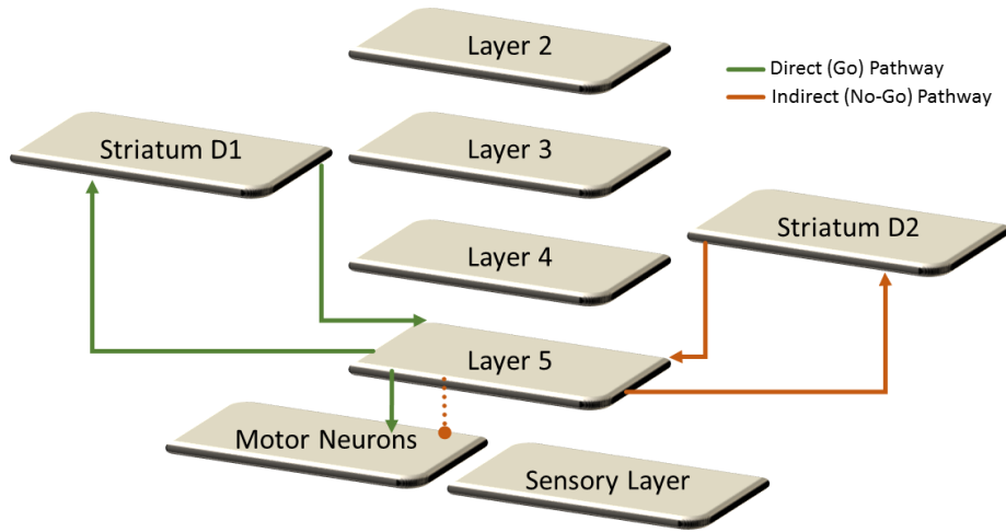
Figure 4.8: Abstract reward circuitry pathways in our framework. Note that all the connections between layer 5 and striatum layers are excitatory. Layer 5 inhibits and excites motor neurons depending on those excitations.
