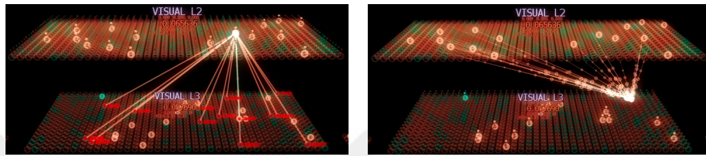
(a) Default proximal dendrite visualization of an L2 column sampling from L3 columns. (b) Mirror dendrite showing proximal propagation of an L3 column to L2 columns.
