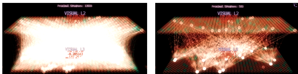
(a) 13933 synapses iterated on vanilla Spatial Pooler. (b) 582 synapses iterated on mirror synapses optimization.
