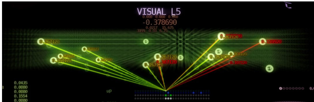
Figure 4.6: Through its apical denrites, the motor neuron at the 13th index of the row associates its activation with the current layer 5 activation above.
