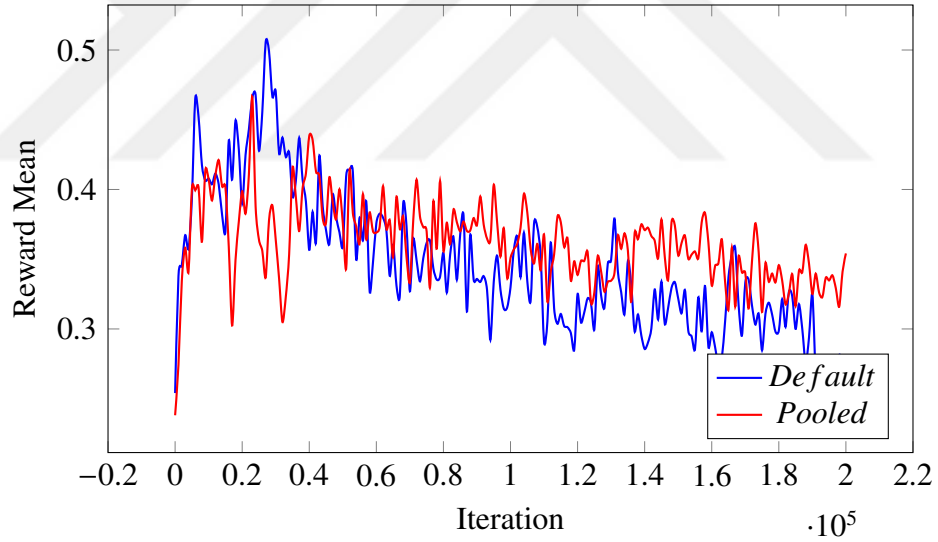
(b) The impact of segment eligibility traces feature on reward average.
