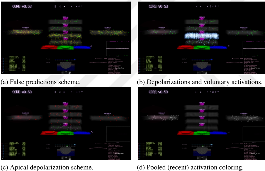
Figure 3.18: Core information colorizations. Green = successful prediction, yellow = false prediction, red = unpredicted activation, blue = predictive, purple = apically predictive, cyan = go voluntary active, orange = nogo voluntary active, white = neurons with nonzero eligibility traces.
