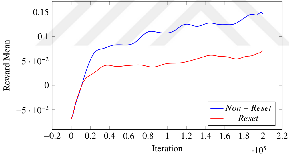
(b) Reset mechanism impact on reward averages.
