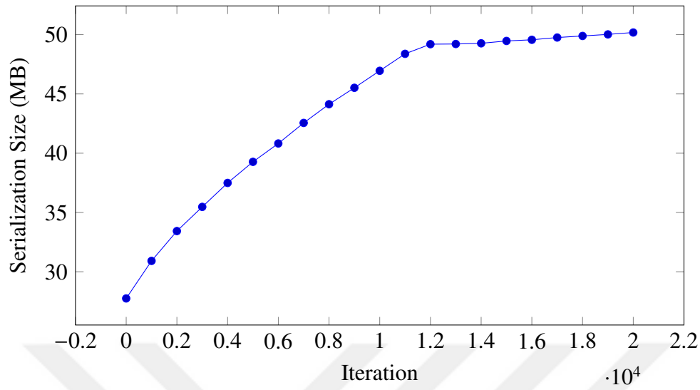
Figure 6.3: Serialization size growth with respect to iterations.
