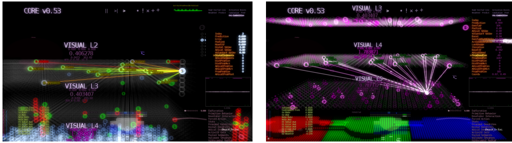
(a) An active distal segment of a layer 2 neuron sampling from nearby neurons. (b) The proximal dendrite of a layer 5 column sampling from layer 4.
