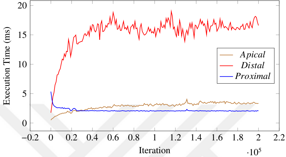
Figure 6.5: Execution timings of the modifications to proximal synapses (Spatial Pooler), distal synapses (Temporal Memory) and apical synapses (Apical Temporal Memory). The timings show the total cost for all HTM layers of the architecture. Non-reset, non-pooled segments configuration with parameters \lambda = 0.6 , \text{learningrate} = 0.5 , \text{discountrate} = 0.95 and 800 \times 8 layersizes.
