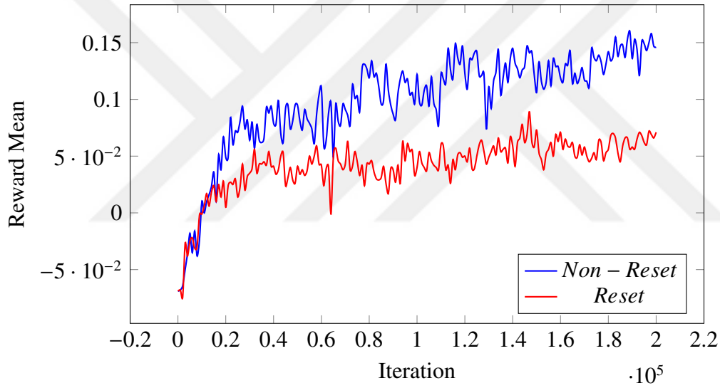
(b) Reset mechanism impact on reward averages.
