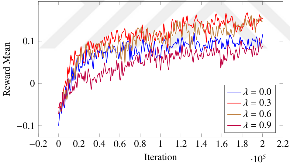
(b) The impact of lambda on reward mean.
