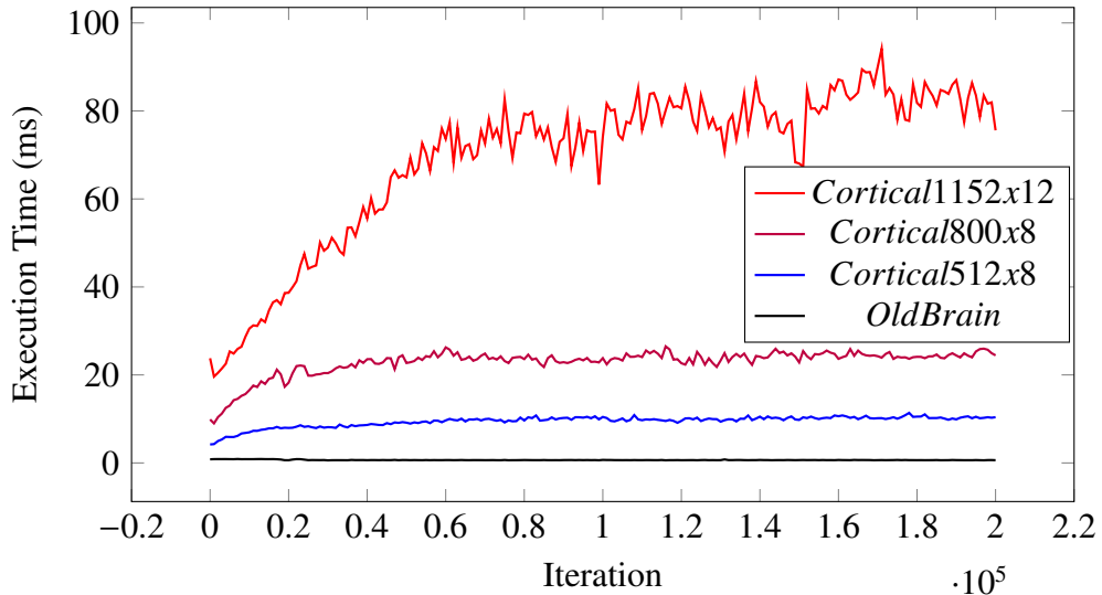
Figure 6.6: Total Cortical System measurements due to layer sizes of the architecture. Non-reset, non-pooled segments configuration with parameters \lambda = 0.6 , \text{learningrate} = 0.5 and \text{discountrate} = 0.95 .
