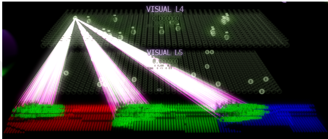
Figure 3.12: The topology between layer 4 and color channels. The layer 4 mini-columns sample the visual data according to their position among the layer.
