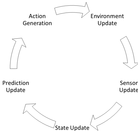
Figure 4.1: Computational cycle of the agent.
