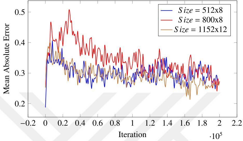
(a) The impact of layer size on MAE measurements.
