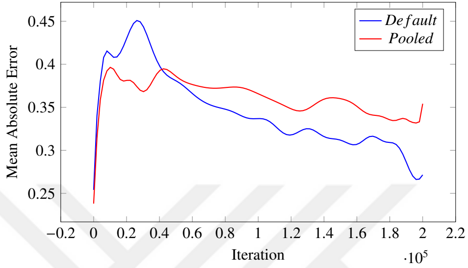
(a) The impact of segment eligibility traces feature on MAE.
