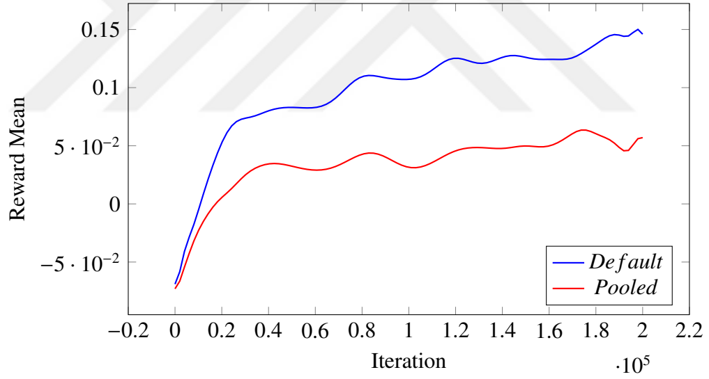
(b) The impact of segment eligibility traces feature on reward average.
