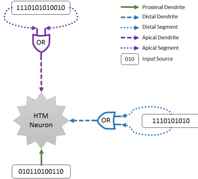
Figure 2.5: HTM neuron model. Proximal synapses are shared among all the neurons of a minicolumn and these synapses activate minicolumns. Distal and apical synapses carry contextual information and determine which neurons to fire among an activated minicolumn.
