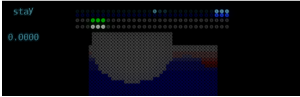
Figure 3.7: Motor neuron array on top and visual sensor image below. The top 4 rows of circles above the visual image represent the states of motor neurons via coloring. Circles on the same column (neurons on the same index of their row) are different colorings of the same neuron.
