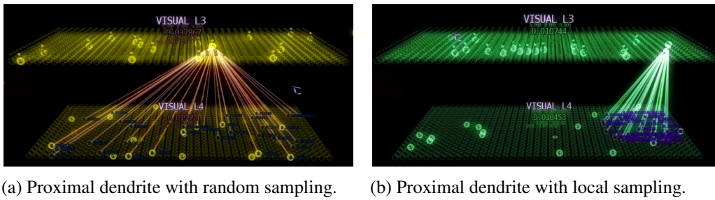
Figure 2.6: A proximal dendrite with no topology is on the left while another with a positional topology is on the right.
