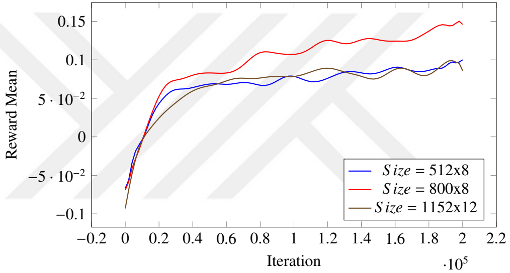
(b) The impact of layer size on reward measurements.
