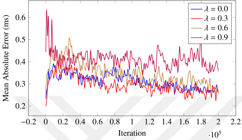
(a) The impact of lambda on MAE.
