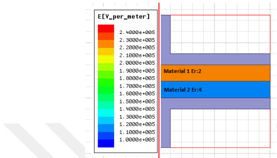
Figure 2-12 Electric field distribution in a medium with two different dielectric
