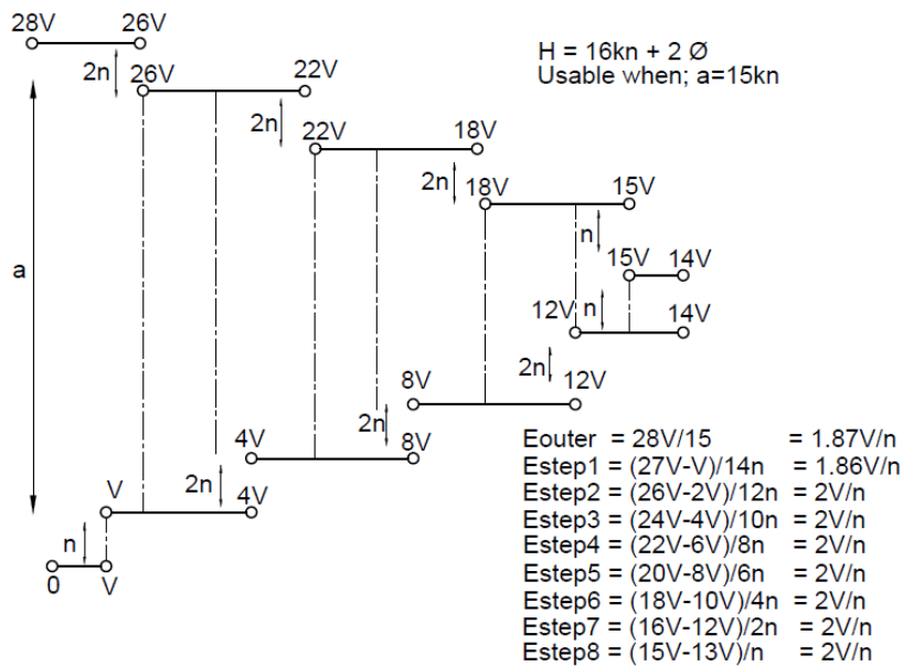
Figure 3-17 1-3-4-4-2 layer template
