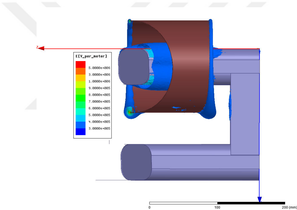
Figure 4-2 3D analysis of a single copper foil with automatic meshing
