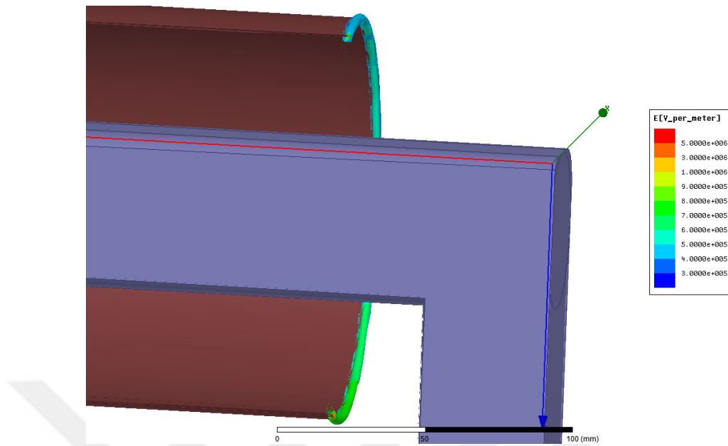
Figure 4-4 Electrical field gradient of the area with focused mesh
