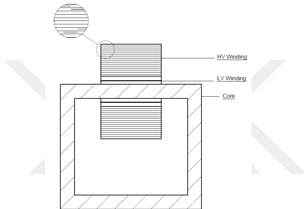
Figure 3-1 Winding section of a voltage transformer
