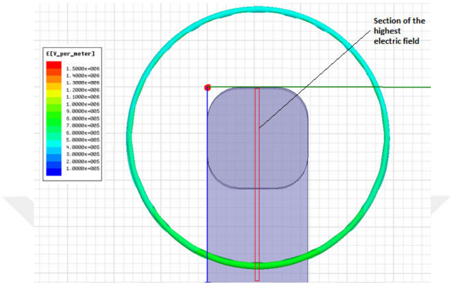
Figure 4-5 Side view of the 3D analysis of the copper foil
