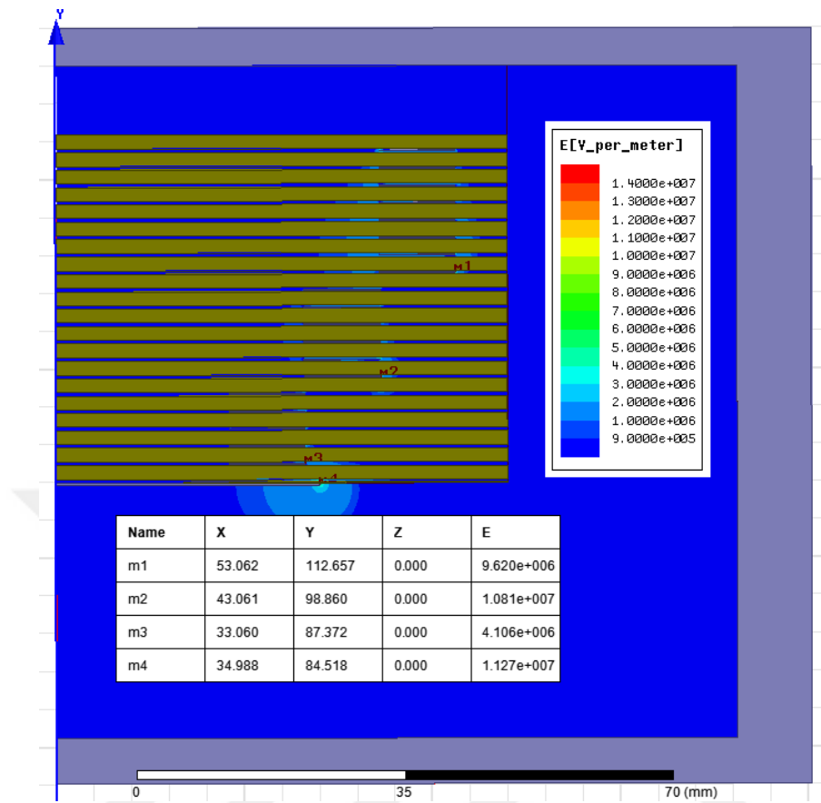
Figure 4-11 Electrical field distribution of the modified design
