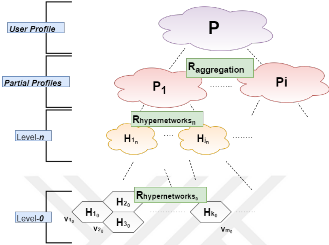
Figure 7.1: User Hypernetwork Multi-Level Design
