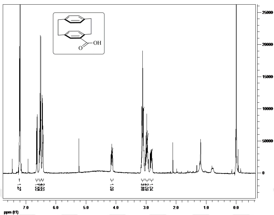
Figure A 6. ^1\text{H} NMR spectrum of [2.2] paracyclophane-2-carboxylic acid (8).
