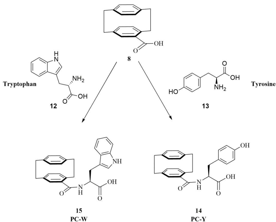
Scheme 8. Synthesis of PC-W and PC-Y .
