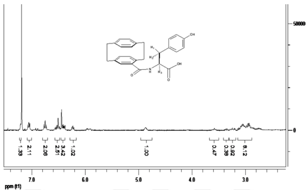
Figure A 8. ^1\text{H} NMR spectrum of [2.2] paracyclophanoyl tyrosine (14).
