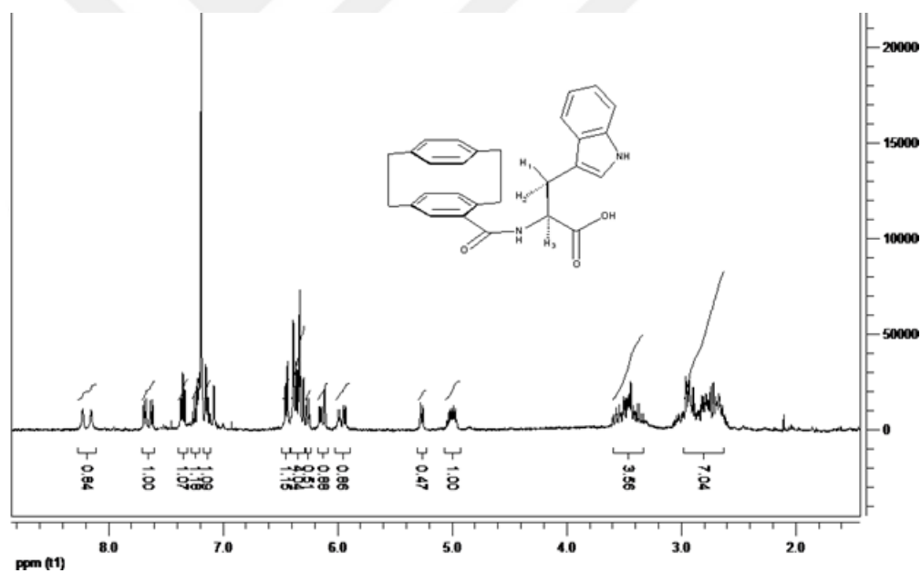
Figure A 9. ^1\text{H} NMR spectrum of [2.2] paracyclophanoyl tryptophan (15).
