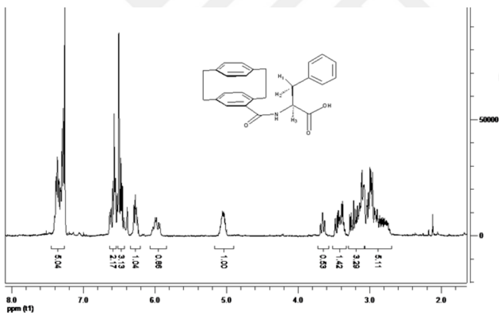
Figure A 7. ^1\text{H} NMR spectrum of [2.2] paracyclophanoyl phenylalanine (11).
