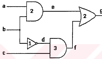
Figure A.1. An example circuit
