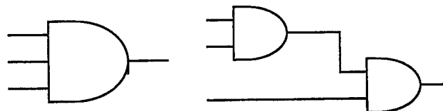
Figure 4.2. Gate decomposition
