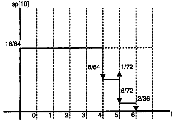
Figure A.4. Tag w_g^{10} of node g
