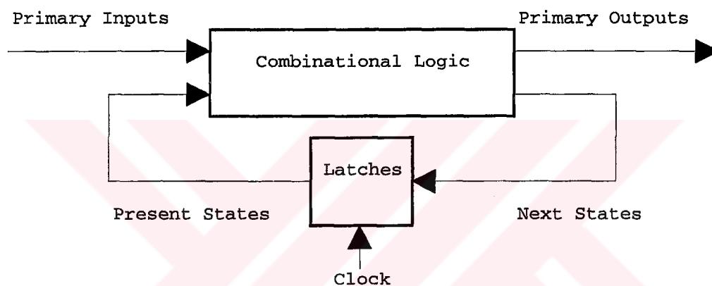
Figure 5.1. A synchronous sequential circuit
