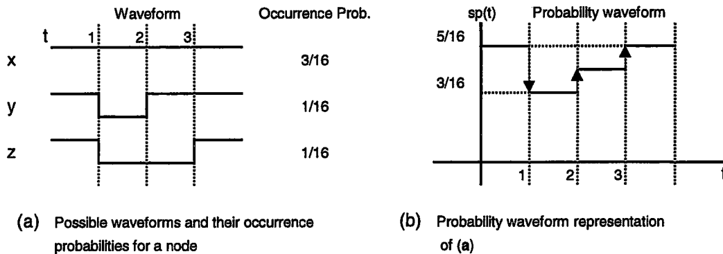
Figure 4.1. Probability Waveforms
