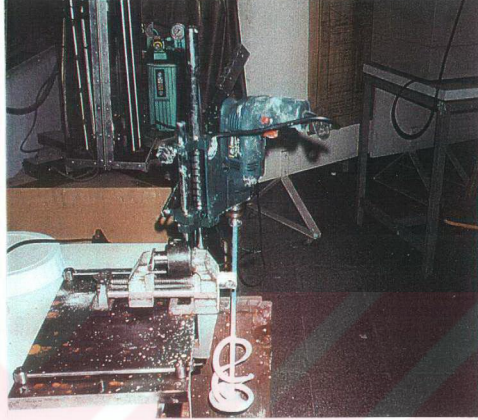
Figure 4.3. Mixer with the fixing apparatus
