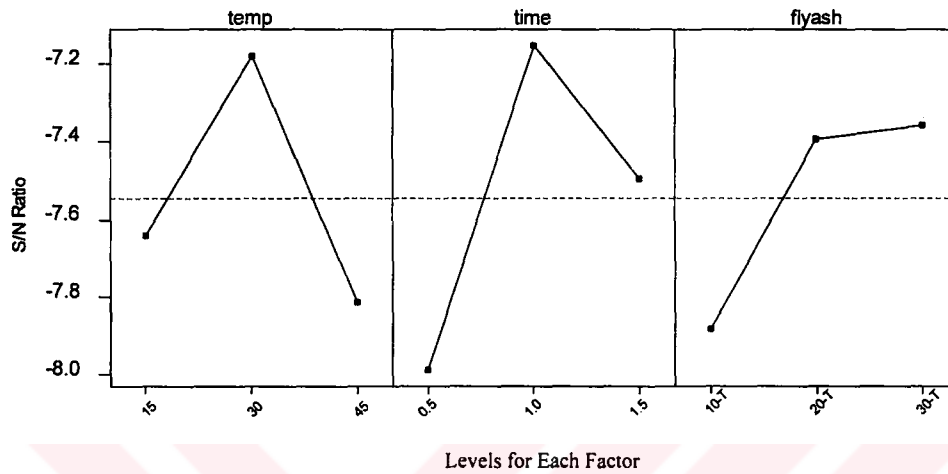
Figure 5.6. Main effect plot for (S/N) ratios (Output: Surface roughness)
