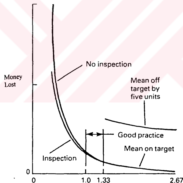
Figure 3.3. Effect of standard deviation on quality loss [23]
