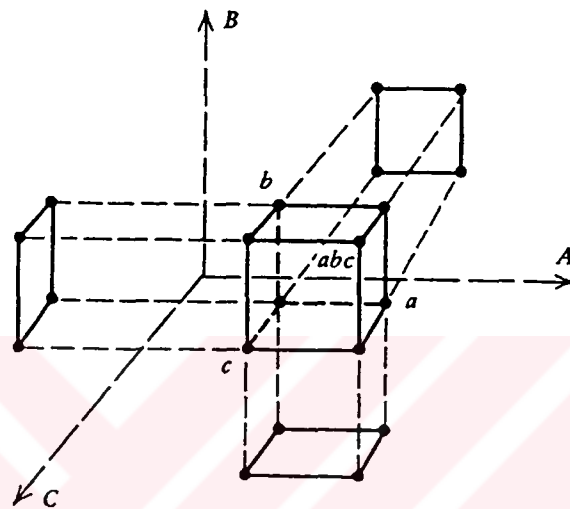
Figure 3.1. Projection of a 2^{3-1} design into three 2^2 designs [20]
