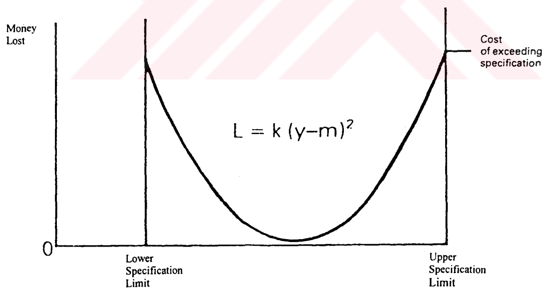
Figure 3.2. Loss function [22]
