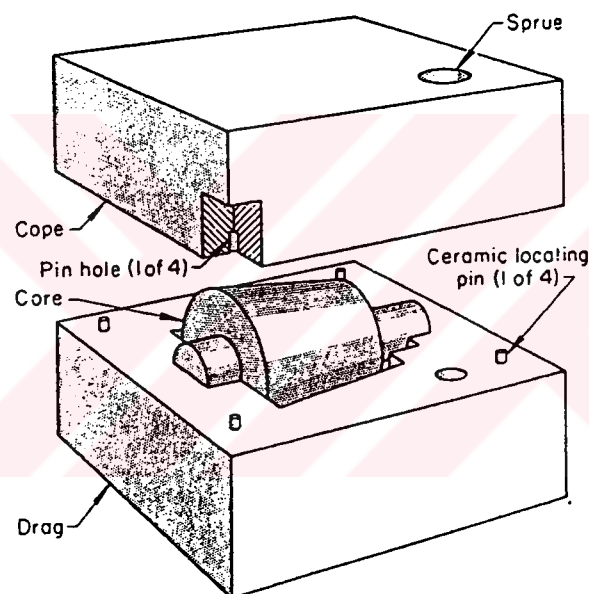
Figure 2.2. Plaster mold and core [4]
