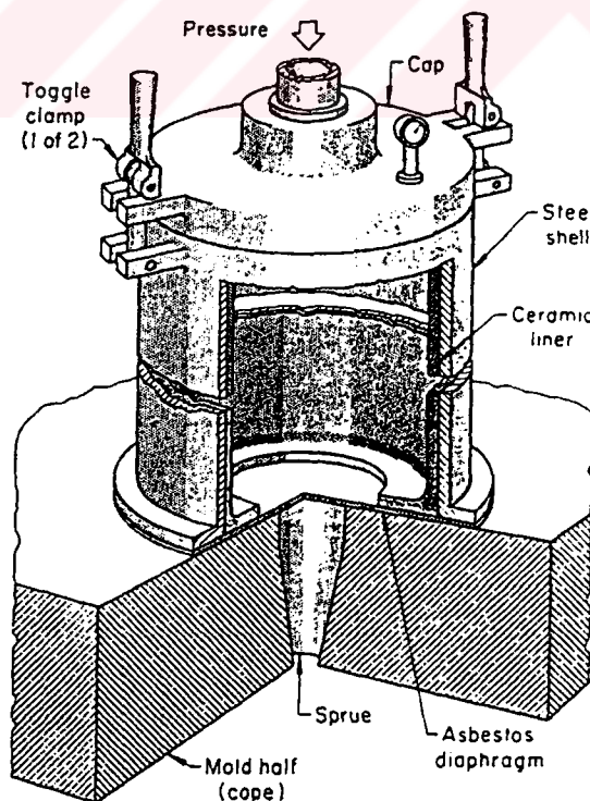
Figure 2.6. Cylinder for pouring a casting with pressure assist [4]
