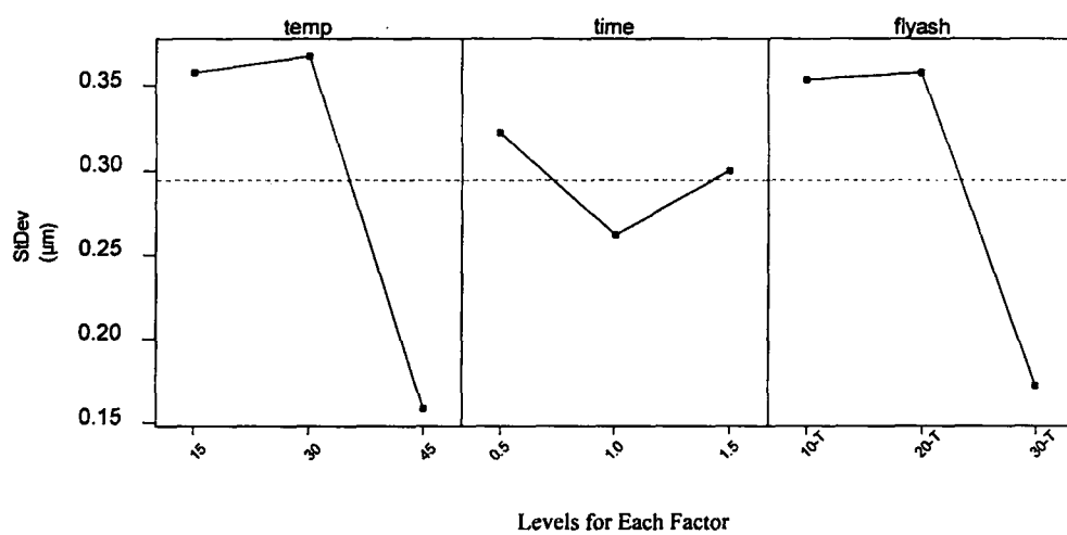
Figure 5.5. Main effect plot for standard deviations (Output: Surface roughness)
