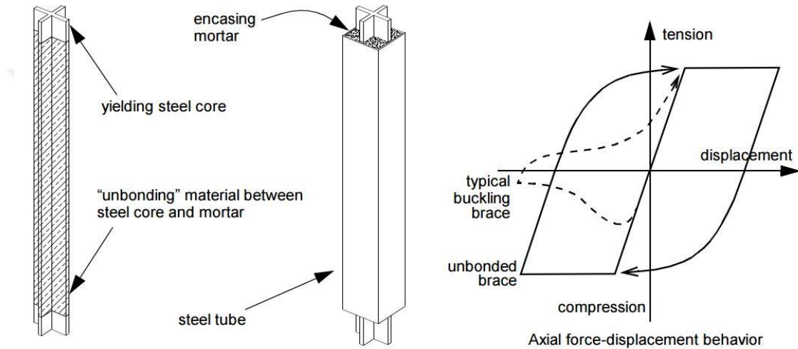
Figure 1.5. Scheme and hysteretic behavior of a typical concrete-encased BRB (Clark et al. 1999).
