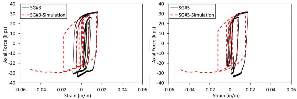
(a) SG Group I (SG#3 and SG#5)
