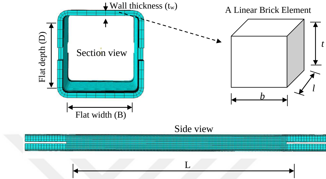
Figure 3.15. Meshing of the square hollow bracing in the simulated SCBF
