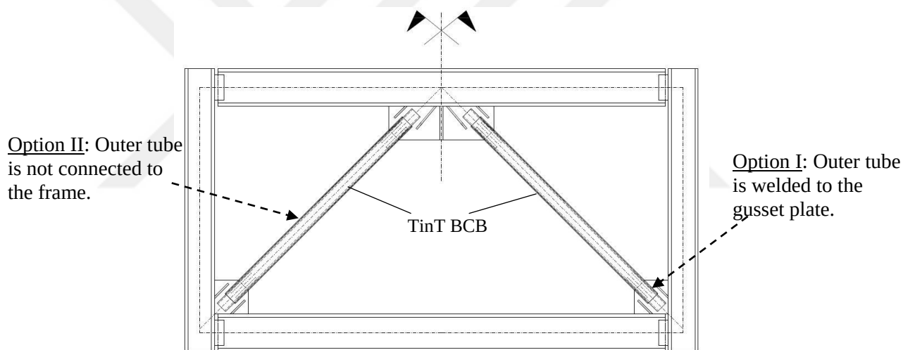
Figure 2.31. TinT-BCB frame with possible applications of buckling-controllers
