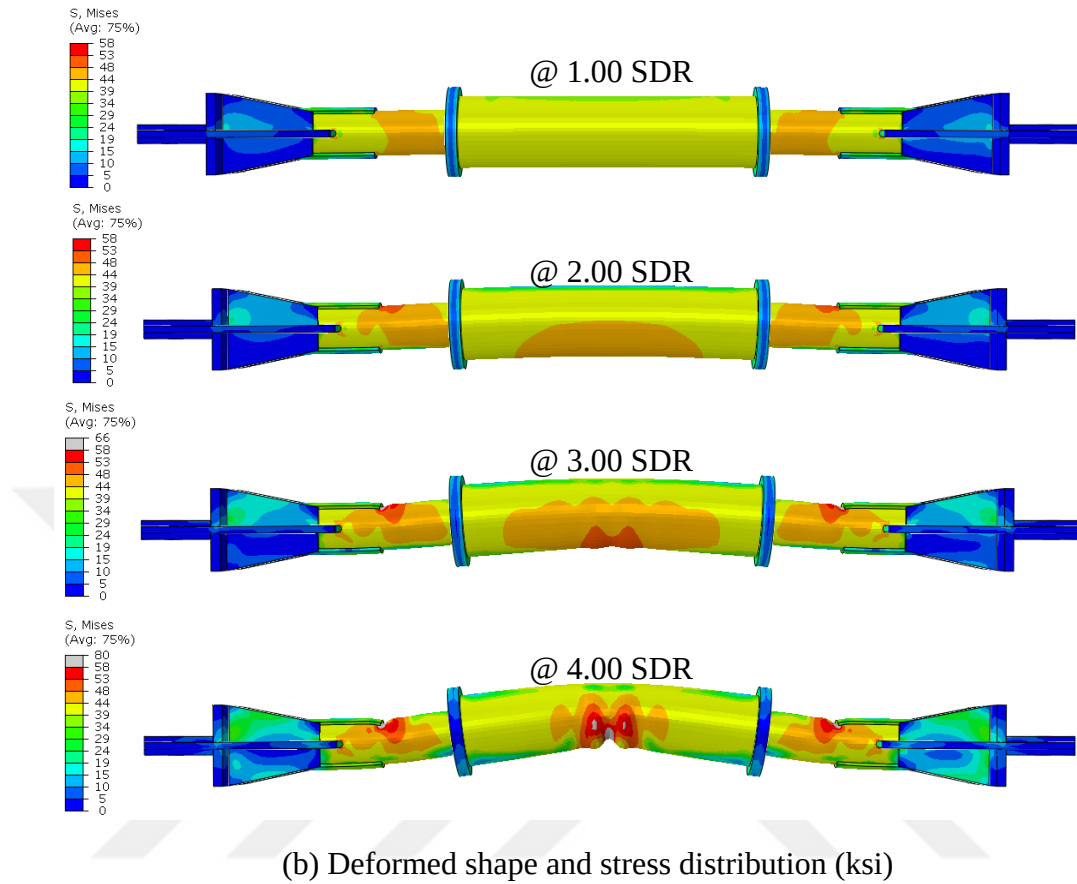
Figure 4.12. Hysteretic response, deformed shape and stress distribution (ksi) of Specimen#3
