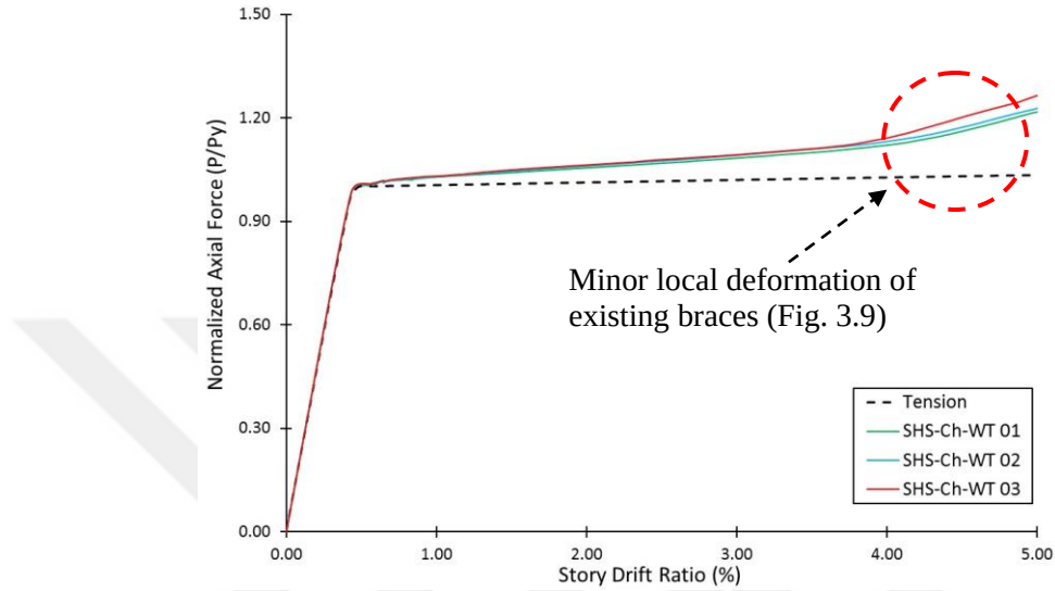
Figure 3.8. Pushover results of SHS-Ch-WT group
