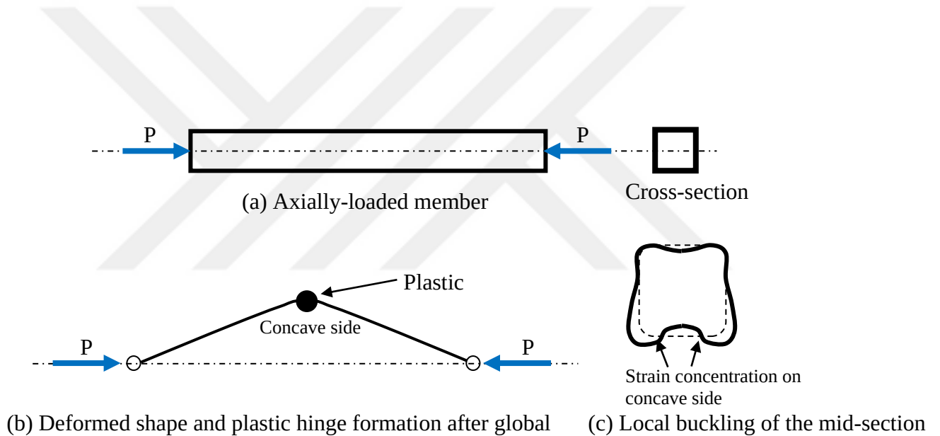
Figure 3.19. Illustration of global and local buckling of an axially-loaded member
