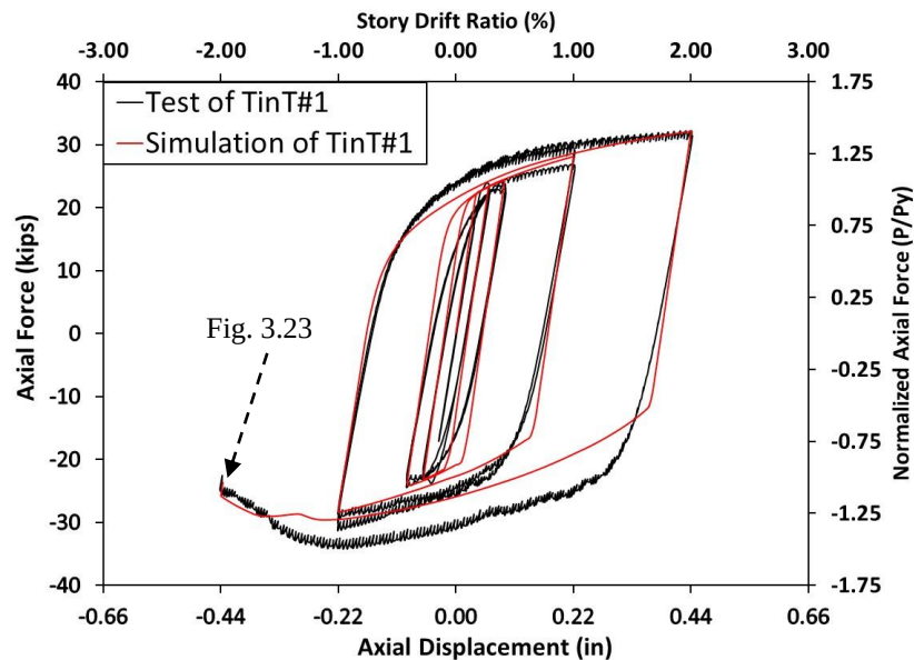
Figure 3.20. Cyclic behavior of TinT-BCB from the experiment and numerical simulation
