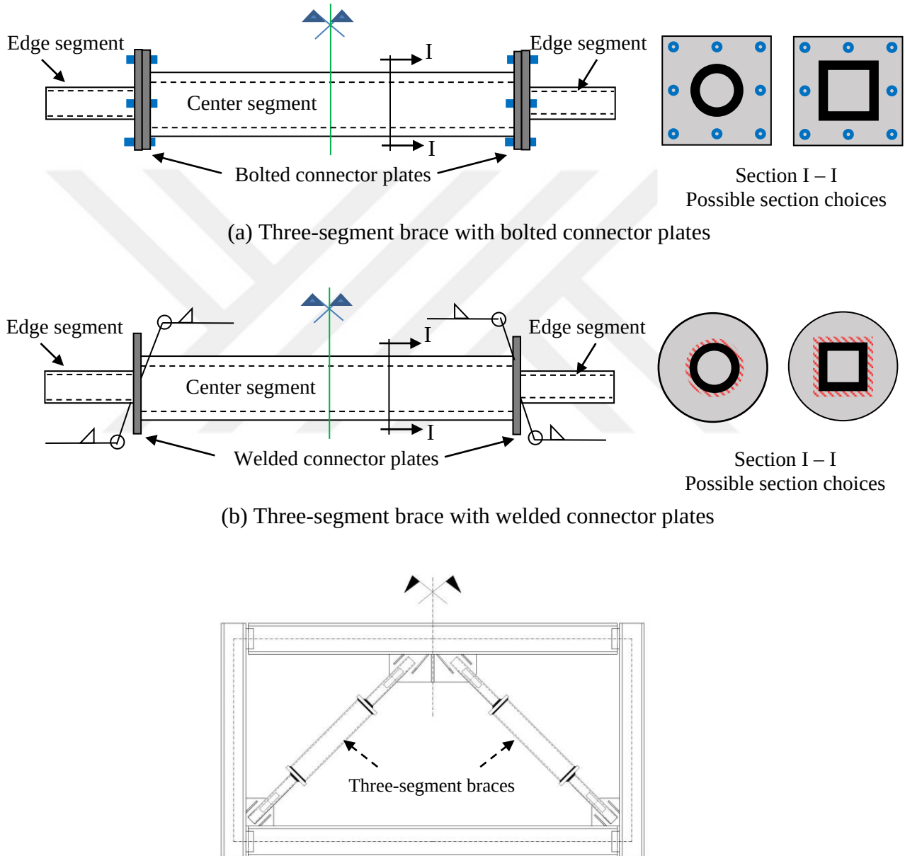
(c) Configuration of a CBF with three-segment braces
