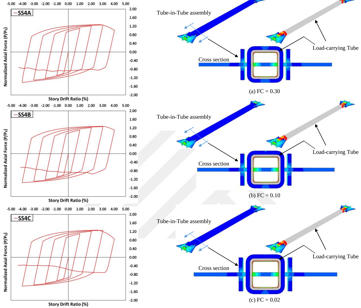
Figure 2.26. Response of SS4 group with gap = 1/32'' and t_{BC} = 0.50'' . Left column: hysteresis; Right column: deformation and relative stress distribution at 2% SDR in compression
