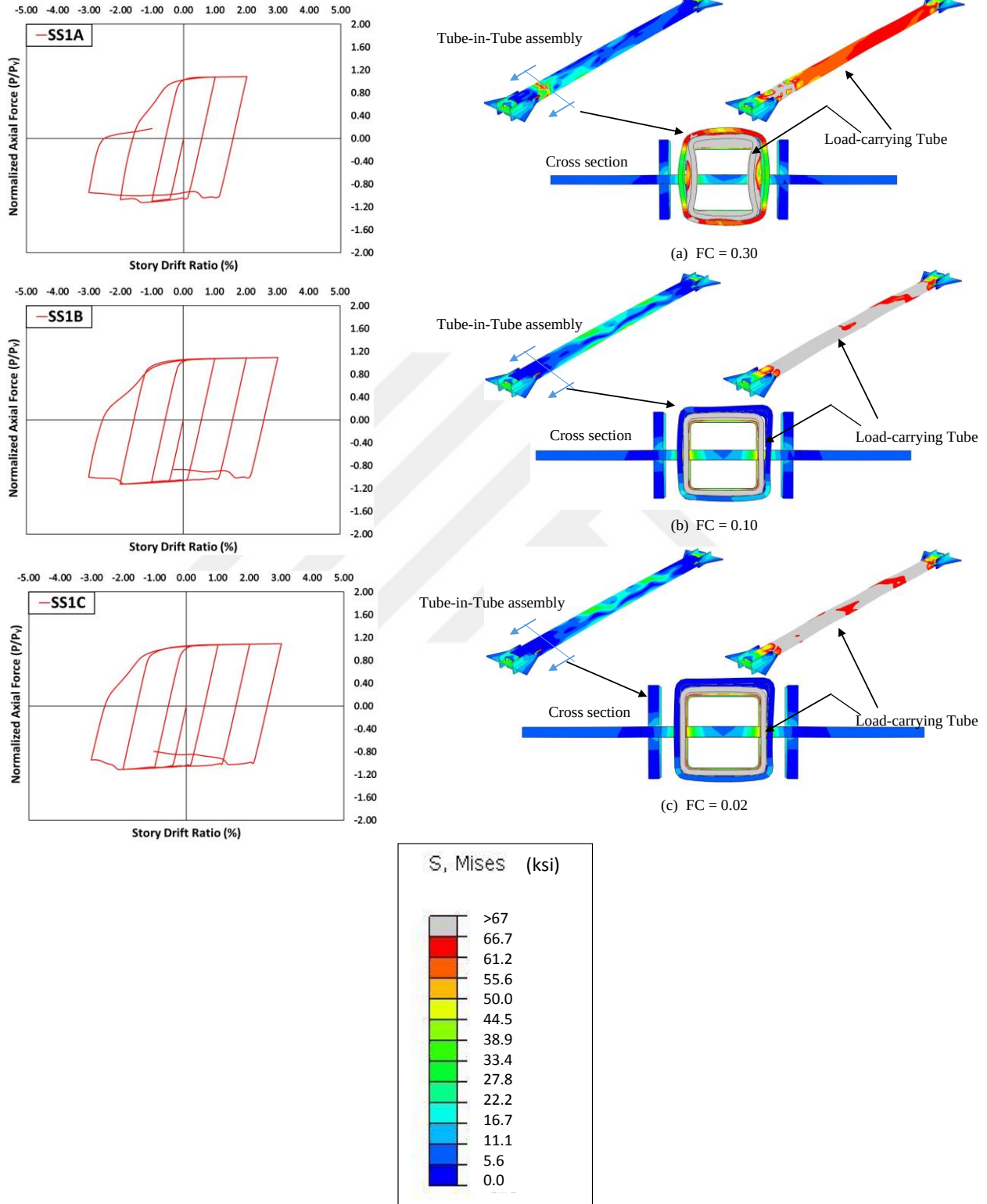
Figure 2.23. Response of SS1 group with gap = 1/16'' and t_{BC} = 0.25'' . Left column: hysteresis; Right column: deformation and relative stress distribution at 2% SDR in compression
