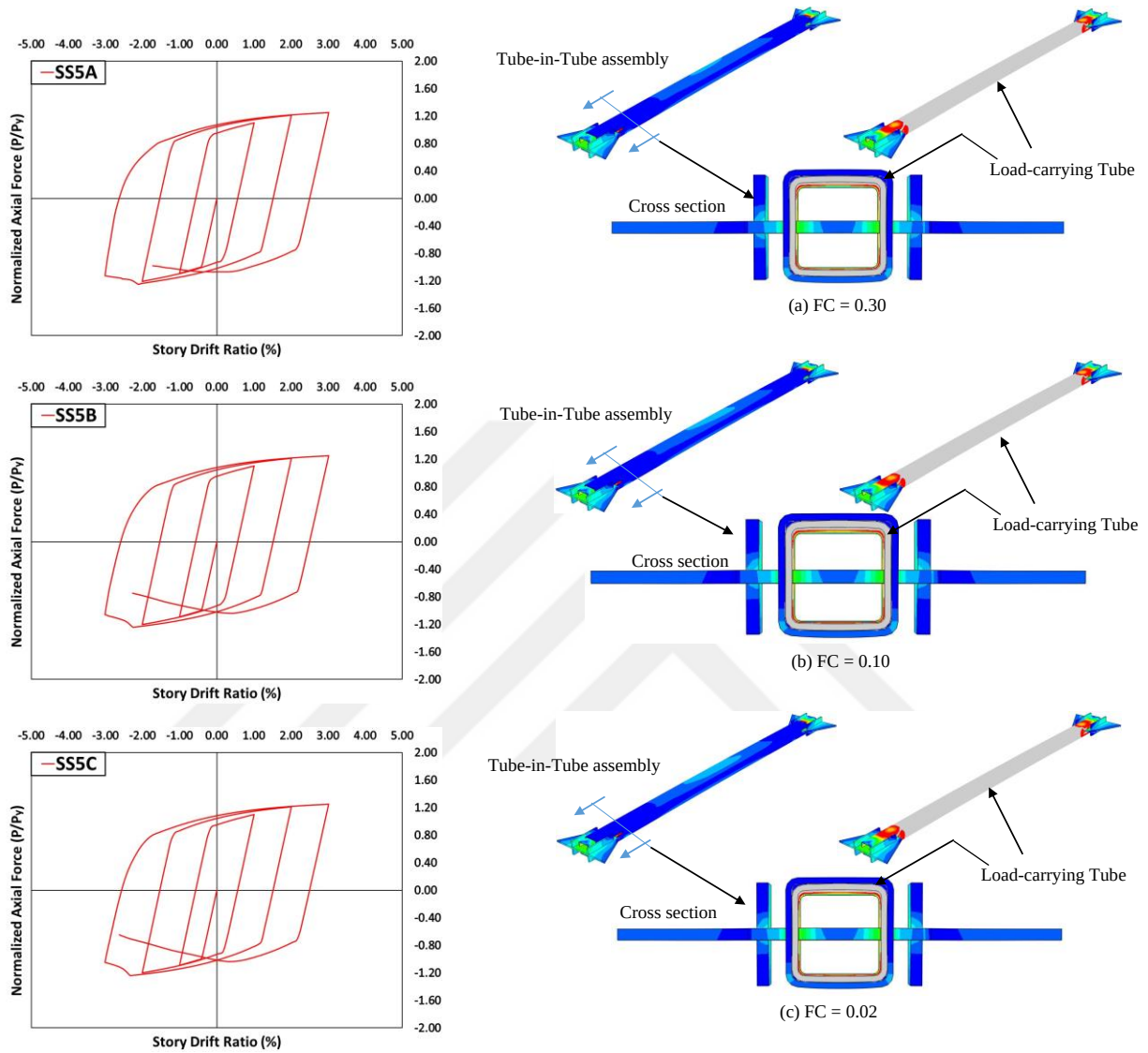
Figure 2.27. Response of SS5 group with gap = 0.02'' and t_{BC} = 0.25'' . Left column: hysteresis; Right column: deformation and relative stress distribution at 2% SDR in compression
