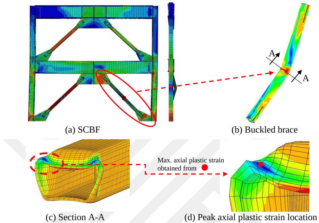
Figure 3.16. Illustration of plastic strain data processing
