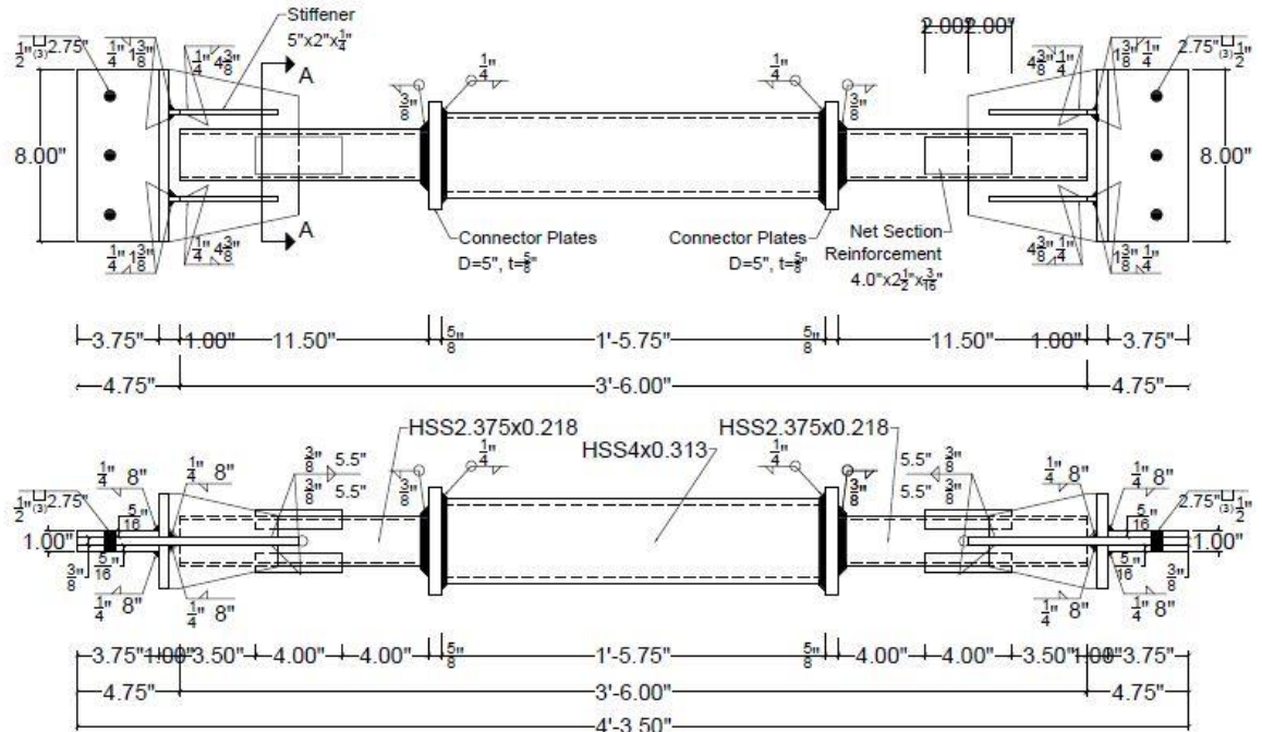
Figure 4.16. Drawings of Specimen 2
