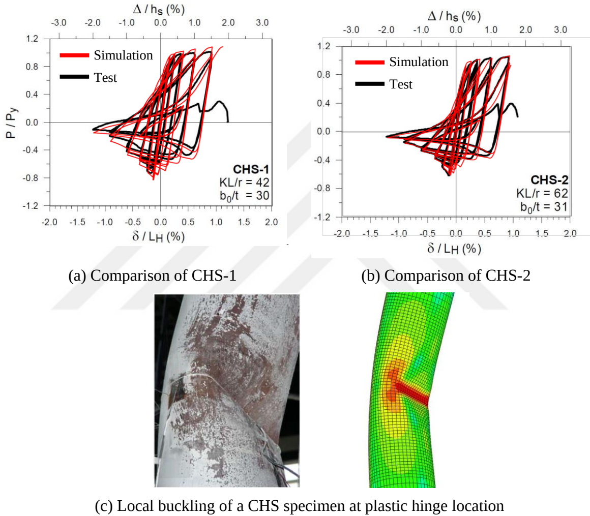
Figure 3.26. Simulation of circular hollow sections tested by Tremblay et al. (2008)
