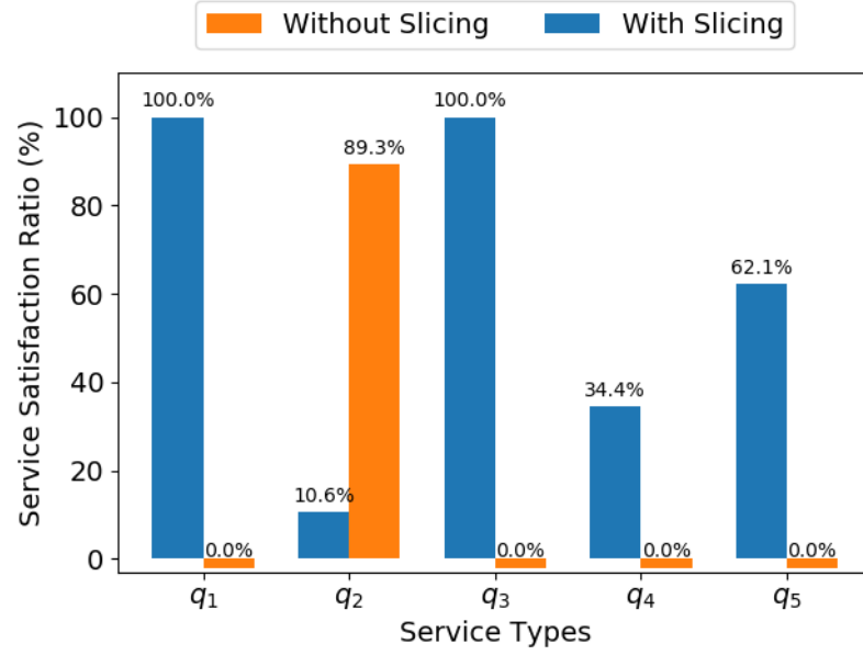
Figure 5.3. Service satisfaction ratios in case of an emergency.
