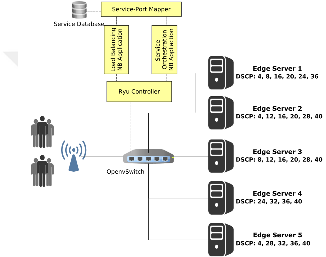
Figure 6.4. Experiment setup for the performance evaluation of the framework.
