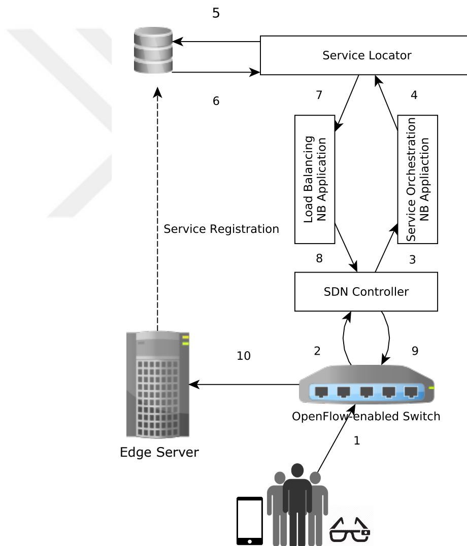
Figure 6.2. Processes for forwarding the service request to the edge server.
