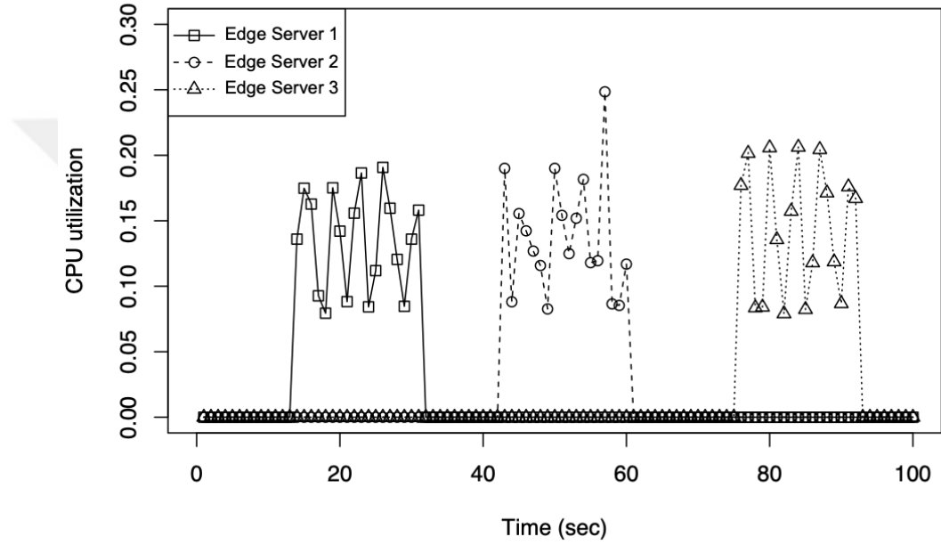
Figure 6.3. Demonstration of the service-centric behavior at the corresponding edge servers.
