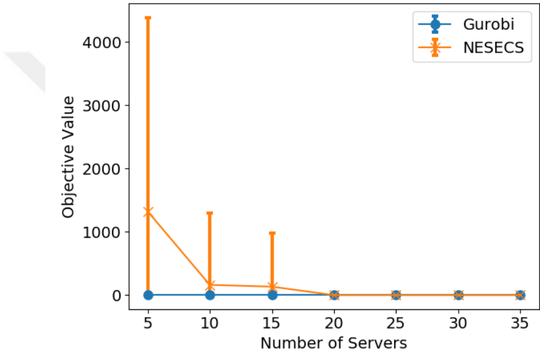
Figure 5.5. Effect of the number of servers on the objective value for 50 nodes and 50 users case.
