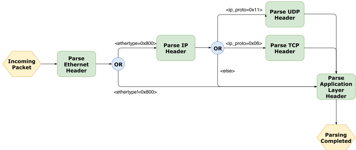
Figure 6.18. Stages of the parser implementation.
