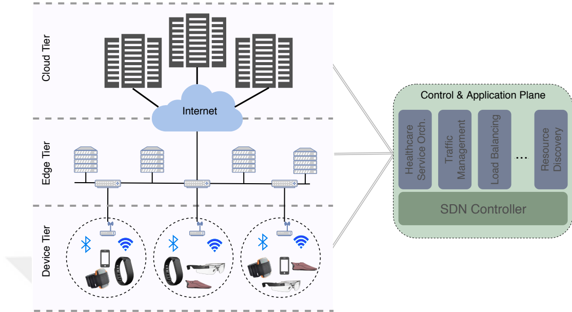
Figure 6.10. SDN-based multi-tier computing and communication architecture.
