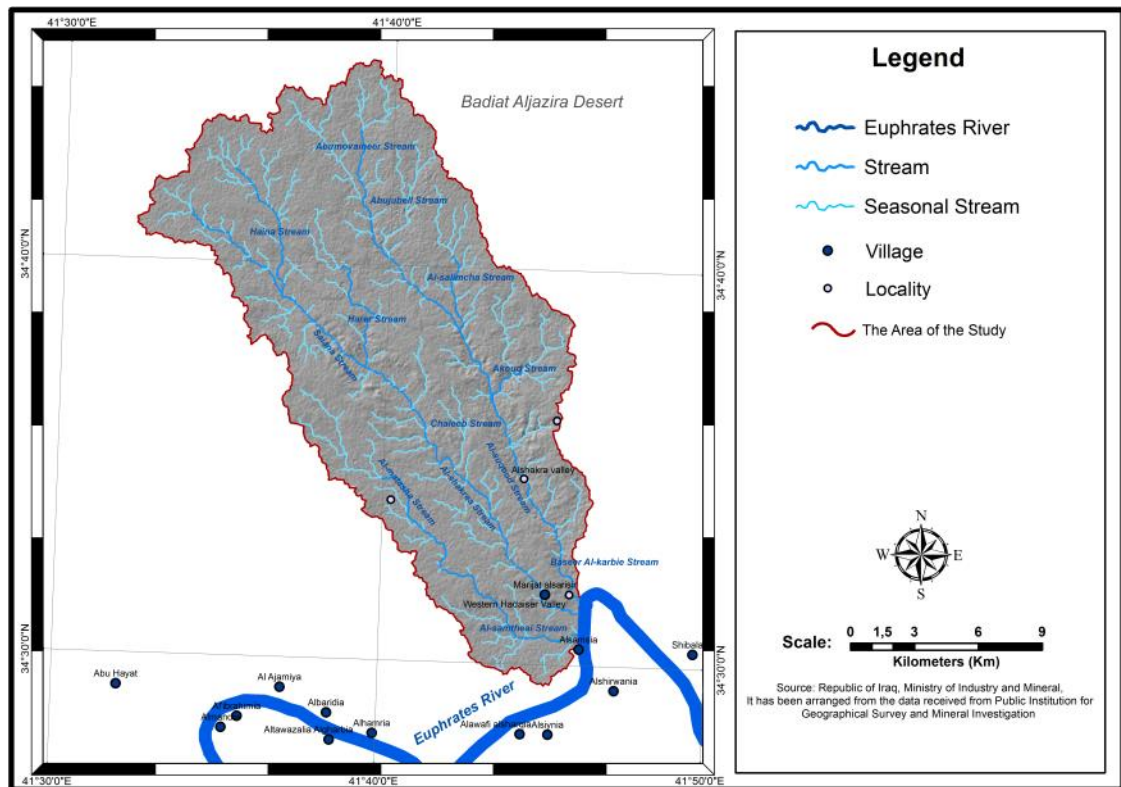
Map 8. Hydrography Map of the Study Area
