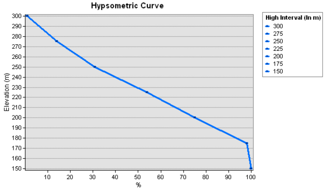
Figure 20. Hypsometric Curve of the Al-Samtheai Stream Basin
