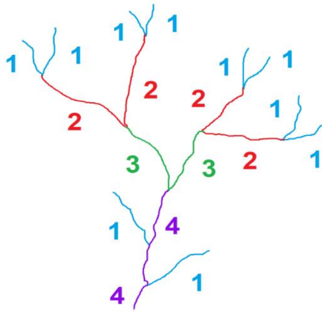
Figure 4. Stream Order Numbers According to Strahler (1952)
