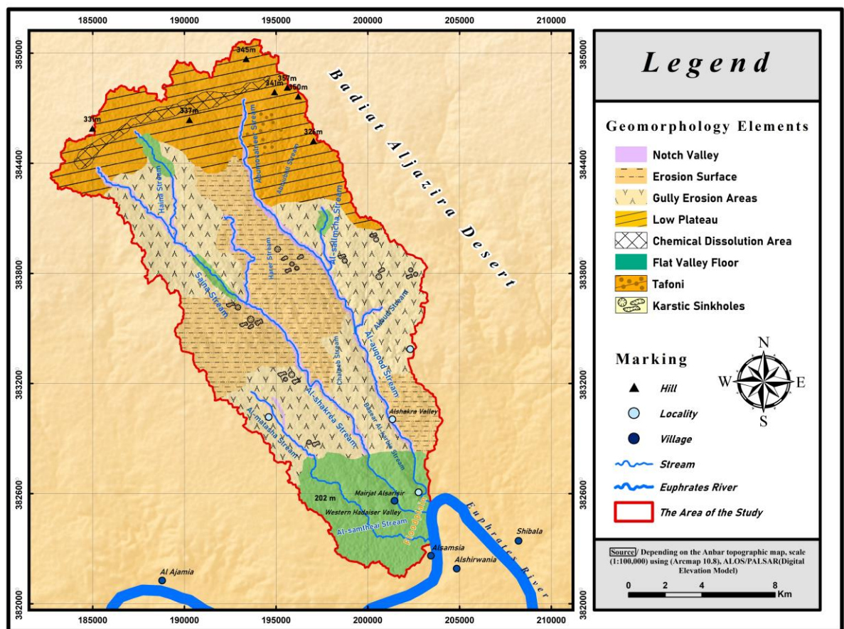
Map 9. Geomorphology Map of the Study Area
