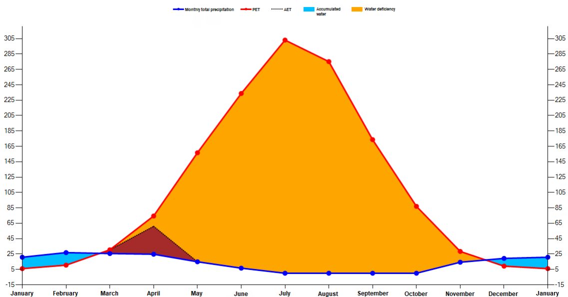
Thornthwaite Water Balance Chart of Anah Station
