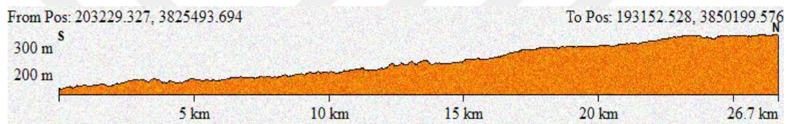
Figure 7. North-South Direction Profile of the Al-Auqood Stream Basin
