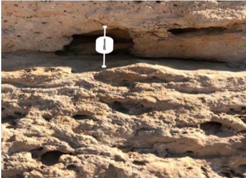
Photograph 23. Dissolved karstic sinkhole at a depth of 20 cm between tafoni in the Al-Shakrea Stream basin
