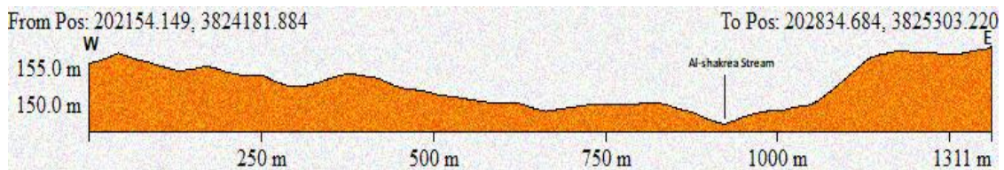
Figure 11. West-East Direction Profile of the Al-Shakrea Stream Basin in the Estuary Region
