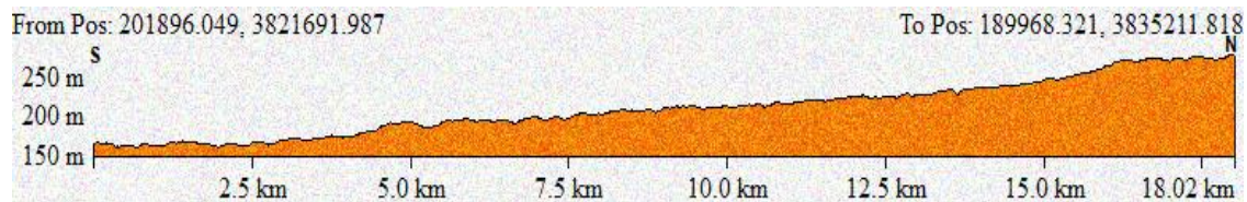
Figure 8. North-South Direction Profile of Al-Samtheai Stream Basin
