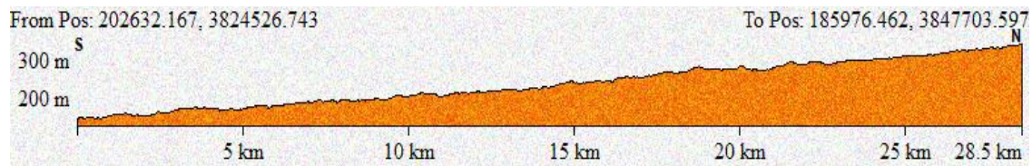
Figure 6. North-South Direction Profile of the Al-Shakrea Stream Basin
