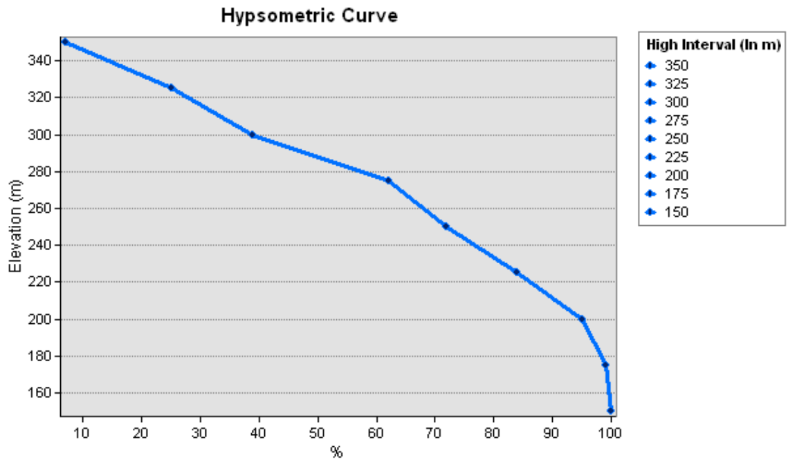
Figure 18. Hypsometric Curve of the Al-Shakrea Stream Basin
