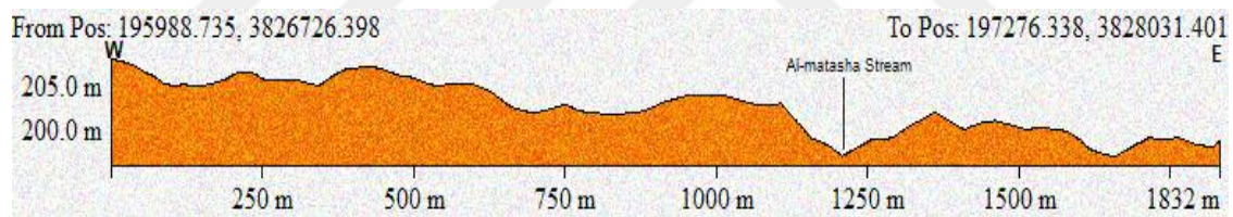
Figure 16. West-East Direction Profile of the Al-Samtheai Stream Basin in the Middle Region
