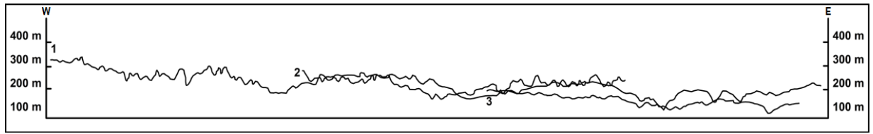
Figure 3. Profiles Showing Level Differences in the Study Area
