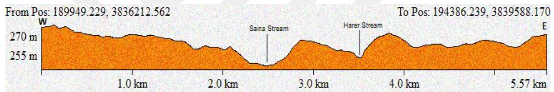
Figure 10. West-East Direction Profile of the Al-Shakrea Stream Basin in the Middle Region
