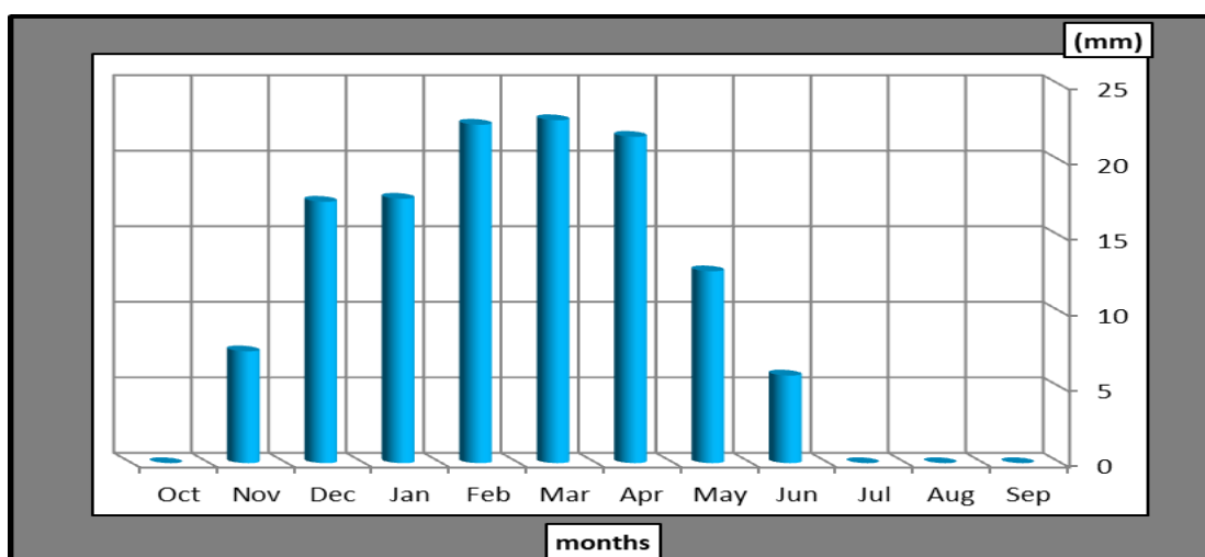
Figure 4. Amount of Rains of the Al-Qaim Station (1980-2019)
