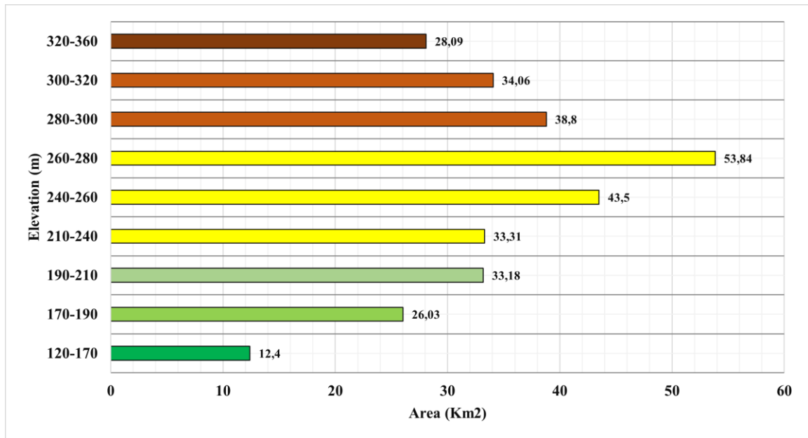
Figure 5. Altitude Categories in the Study Area
