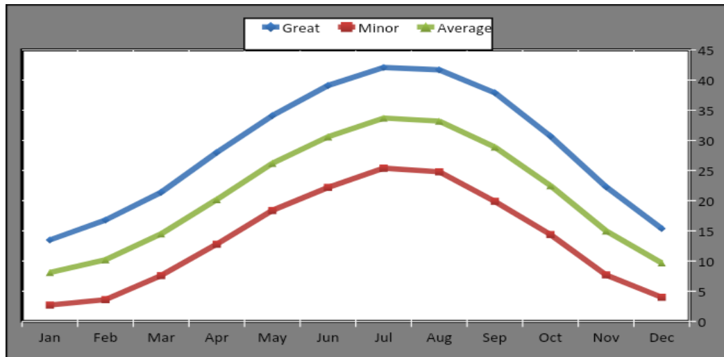
Figure 2. Graph of Monthly Maximum, Minimum, and Average Temperatures of the Anah Station (1980-2019)
