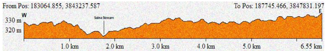
Figure 9. West-East Direction Profile of the Al-Shakrea Stream Basin in the Source Region
