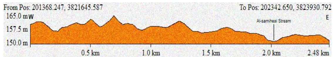
Figure 17. West-East Direction Profile of the Al-Samtheai Stream Basin in the Estuary Region
