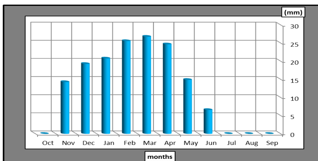
Figure 5. Amount of Rains of the Anah Station (1980-2019)
