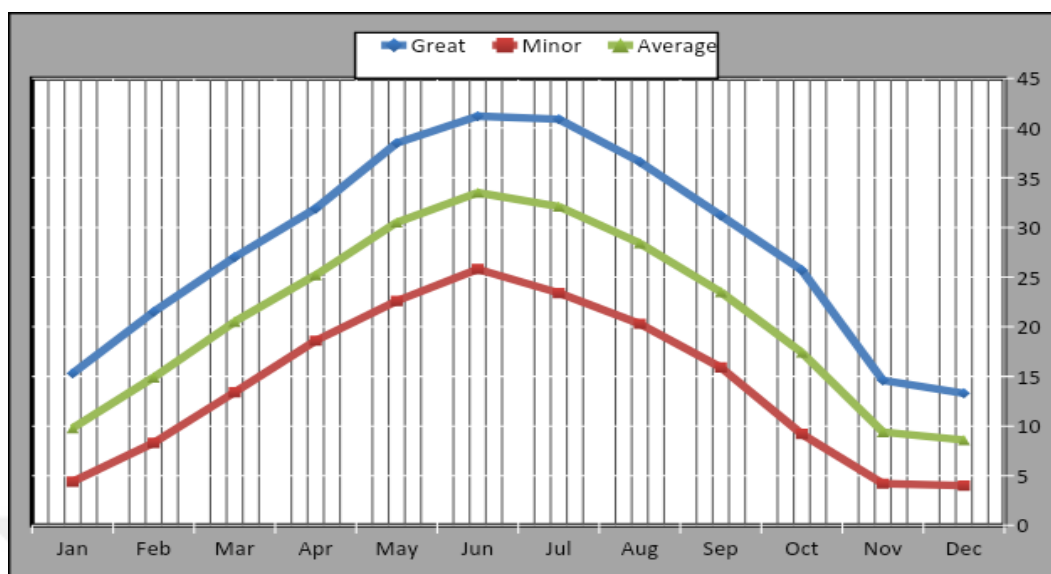
Figure 1. Seasonal and Average Monthly Temperatures of the Al-Qaim Station (1980-2019)
