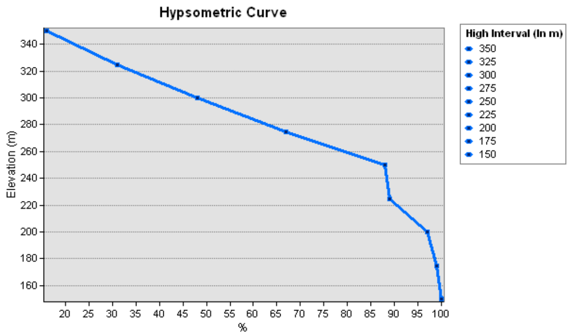
Figure 19. Hypsometric Curve of the Al-Auqood Stream Basin
