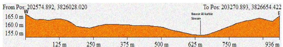
Figure 14. West-East Direction Profile of the Al-Auqood Stream Basin in the Estuary Region
