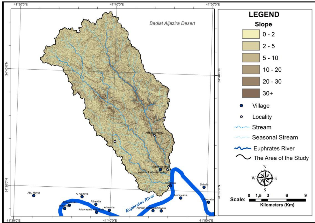
Map 12. Slope Map of the Study Area
