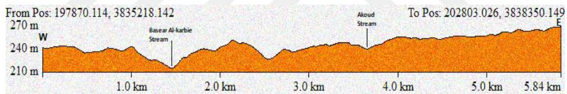
Figure 13. West-East Direction Profile of the Al-Auqood Stream Basin in the Middle Region
