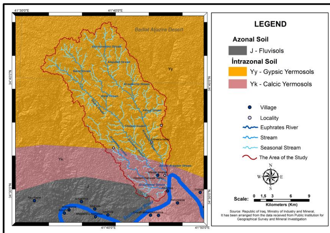
Map 7. Soil Map of the Study Area
