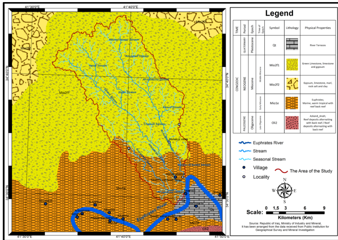
Map 2. Geology Map of the Study Area
