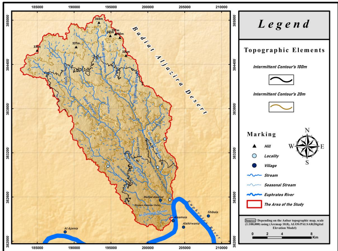
Map 13. Topographical Characteristics of the Study Area
