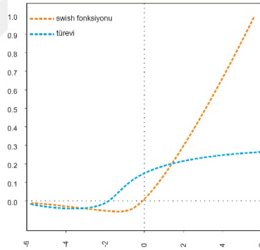
Swish
