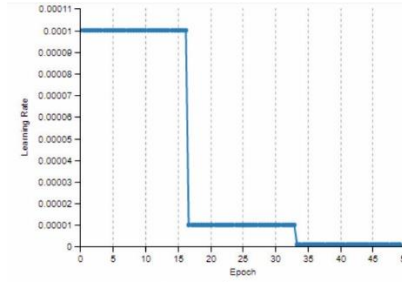
step down
