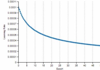
inverse
