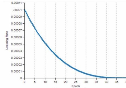
polynomial
