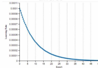
exponential
