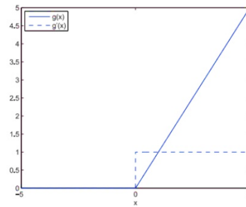
ReLu
