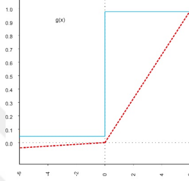
Leaky ReLu
