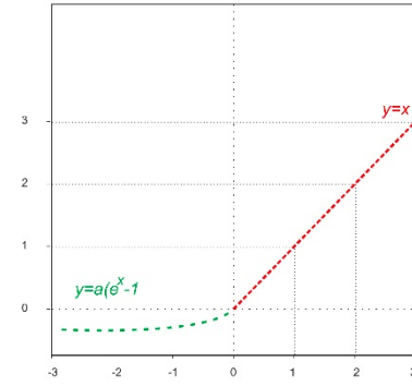
E-ReLu
