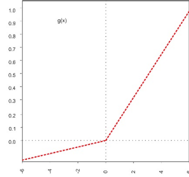
Parameterized ReLu
