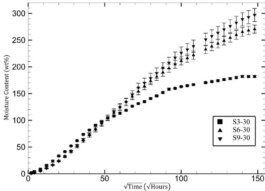
Figure 66. Mass gain data of Rohacell foam core sandwich composite manufactured under 30 psi pressure
