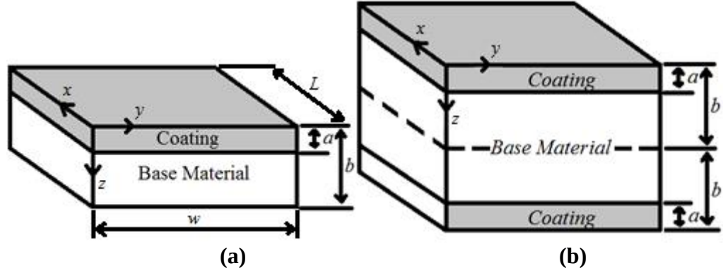
Figure 16. The representation of the model geometry (a) for a single coating layer of thickness a . The total sample thickness is b . (b) for a symmetric coating layer of thickness a . The total sample thickness is 2b .
