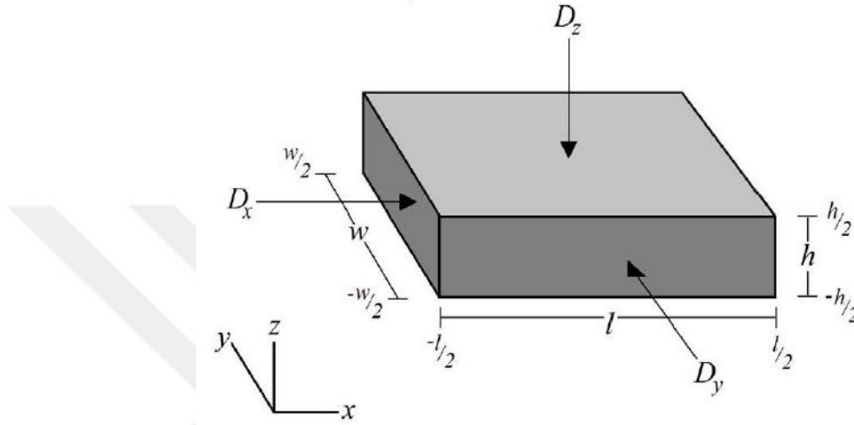
Figure 11. The representative figure for finite slab and the three-dimensional Fickian model geometry.
