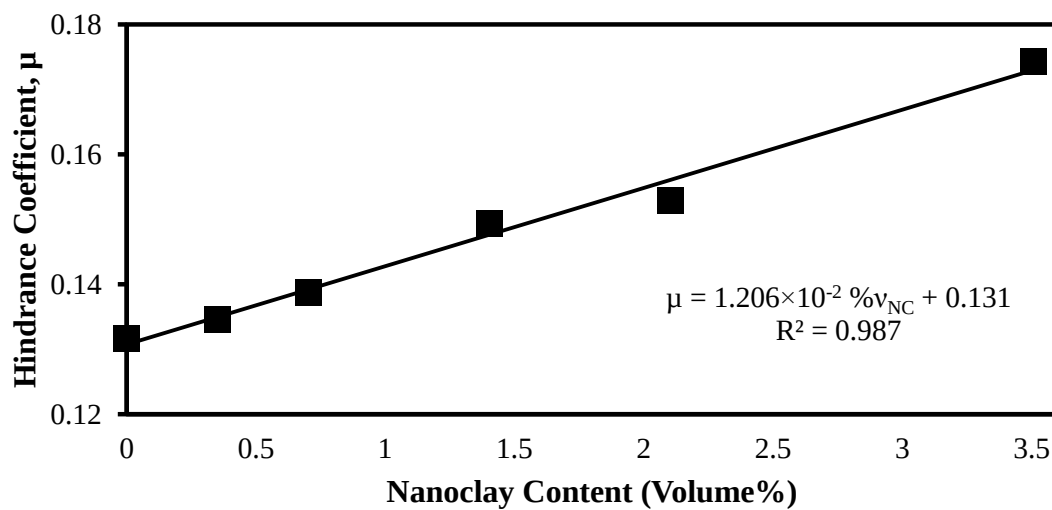
Figure 27. Effect of nanoclay loading in EPON 862 epoxy on hindrance coefficient.
