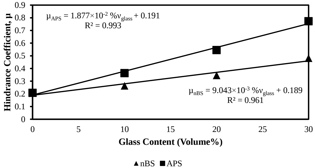
Figure 35. Effect of APS and nBS glass sphere loading in DGEBA epoxy on hindrance coefficient.
