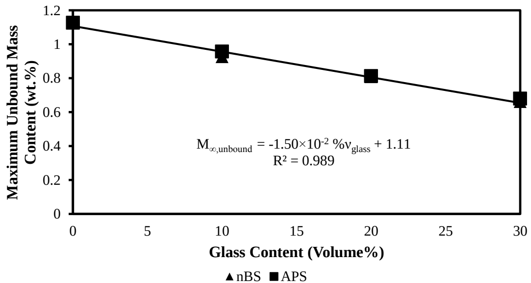
Figure 37. Effect of APS and nBS glass sphere loading in DGEBA epoxy on maximum unbound moisture content.
