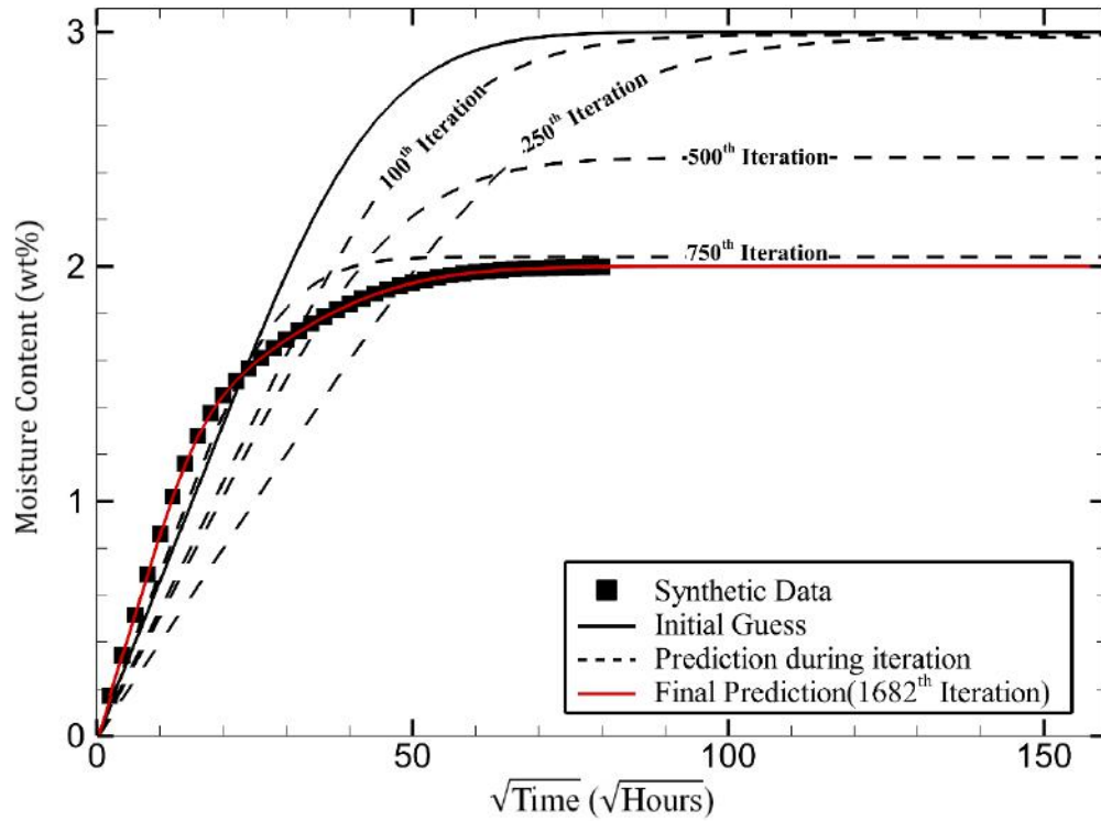
Figure 14. Absorption parameter recovery from thermo-gravimetric synthetic data.
