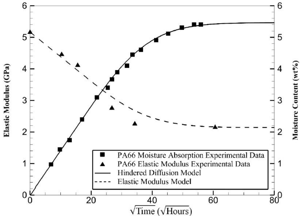
Figure 78. Variation in elastic modulus and mass gain due to moisture absorption into polyamide-6.6
