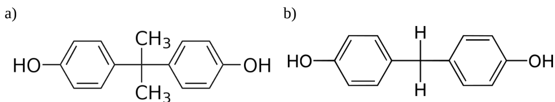
Figure 31. Schematics of a) Bisphenol-A and b) Bisphenol-F
