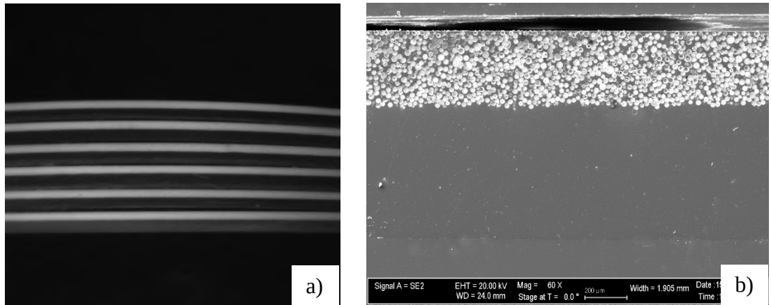
Figure 42. a) Optical microscopy image of 6 immersion samples showing multilayer of 31% thick glass sphere/epoxy, and 69% thick epoxy b) a representative SEM image of a sample.
