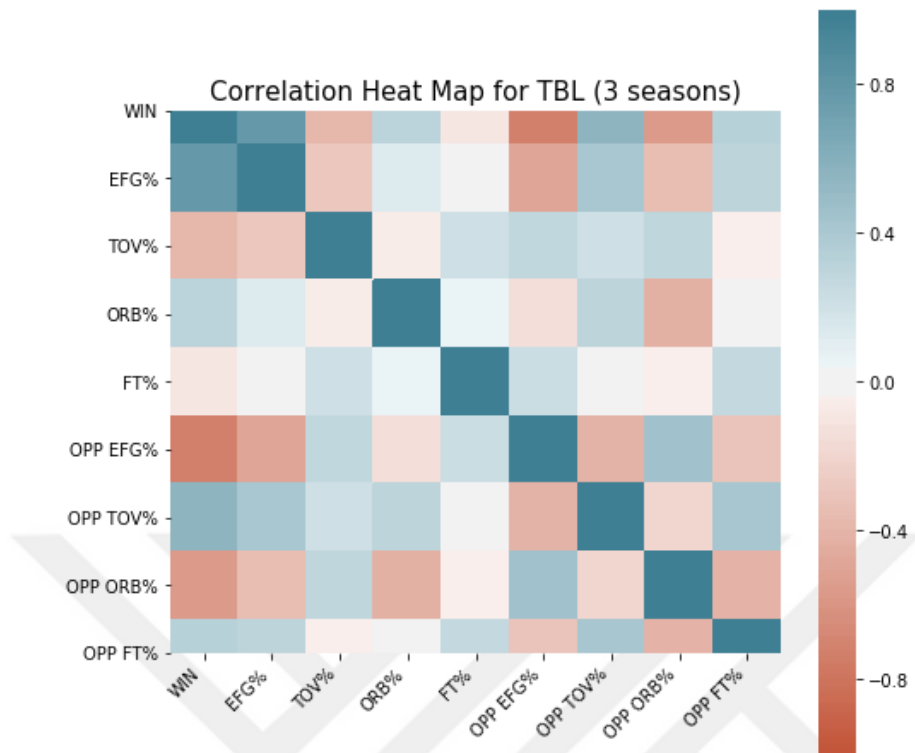
Figure 5: Correlation table for Four Factor metrics (for the team and opposite team) in TBL between 2016-2017 and 2018-2019 seasons
