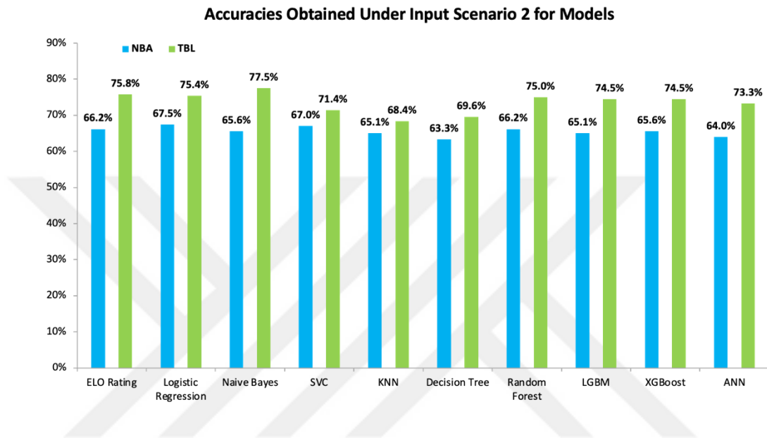
Figure 23: Comparison of models for NBA and TBL under input scenario 2
