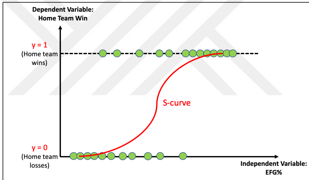
Figure 19: Mathematical Logic Behind Logistic Regression with Example
