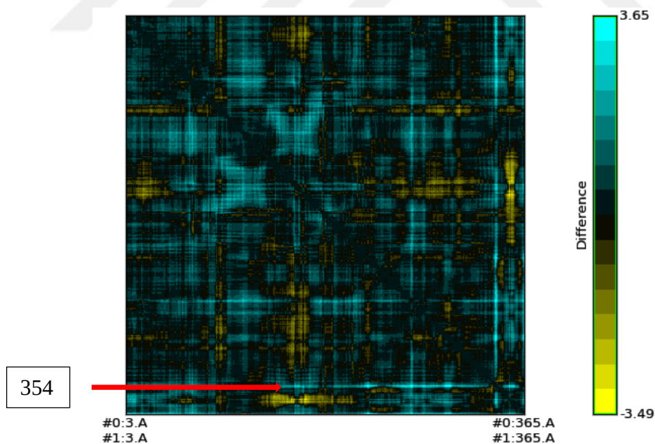
Figure 3.25 R-R distance map of V254E vs. wild type CYP119. Numbers of most flexible residues indicated in boxes.
