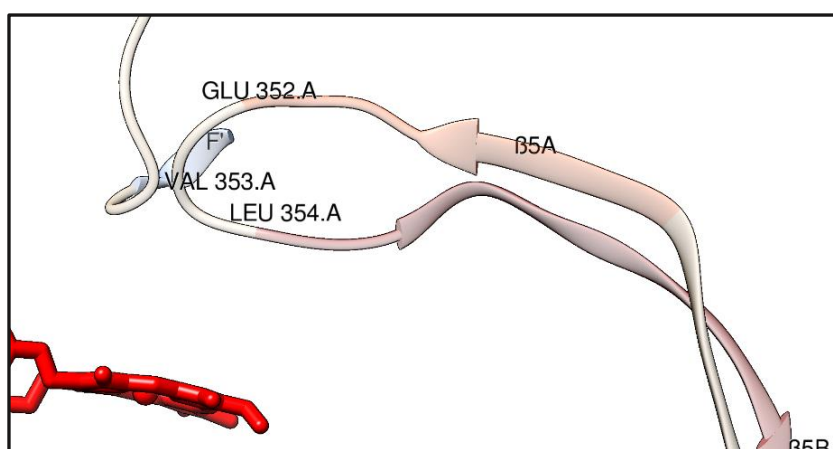
Figure 1.16 EVL region of CYP119 with heme group.
