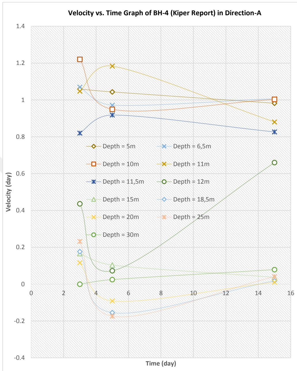
Figure A.5- Velocity vs. Time Graph of BH-4 (Kiper Co.) in Direction-A.
