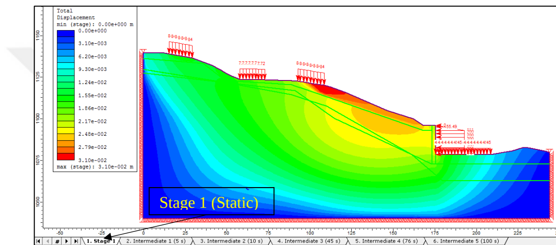
Figure 6.22. Static displacements for the undrained model.
