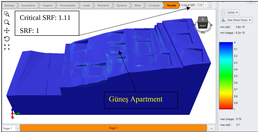
Figure 5.24. Distribution of shear strains following three-dimensional analyses at SRF of 1.
