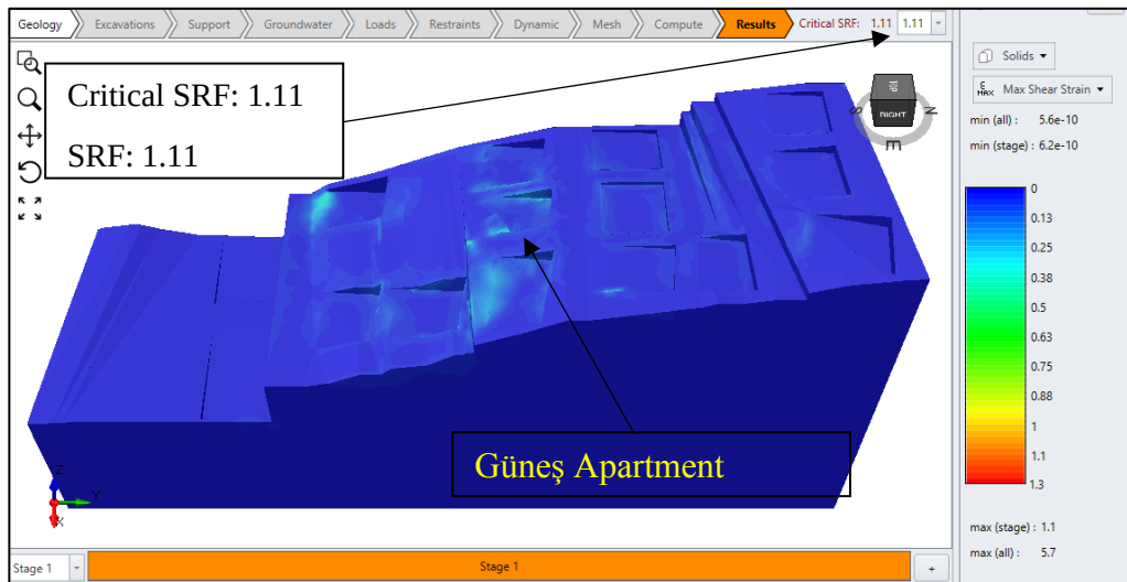
Figure 5.25. Strain accumulation zones at the critical SRF.
