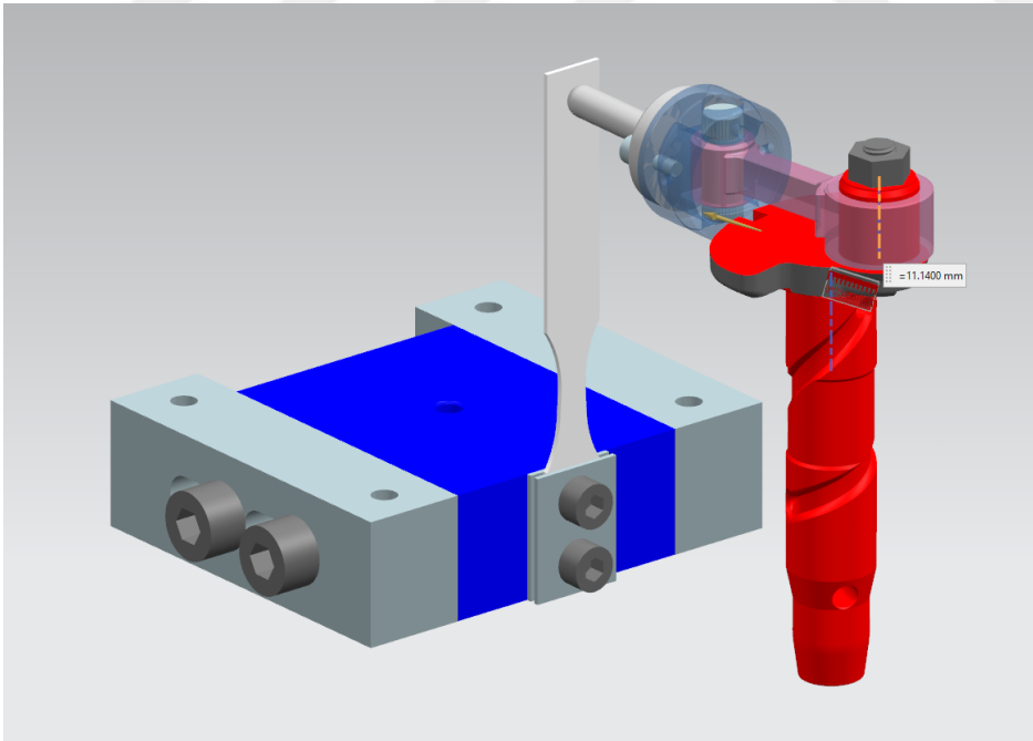
Figure 3.45. Maximum Displacement Orientation of Fatigue Test Machine, which corresponds to a distance of 11 mm on crank shaft & 22 mm Displacement on Fatigue Specimen
