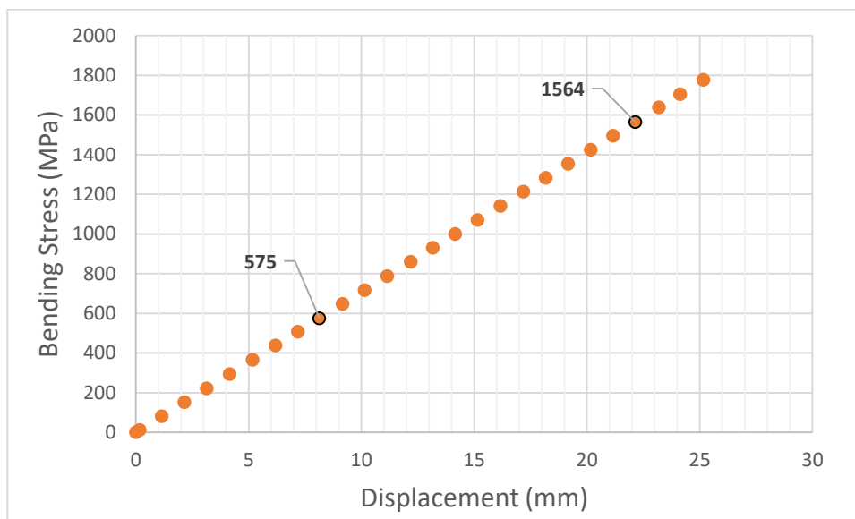
Figure 4.25. Analytical Maximum Bending Stresses
