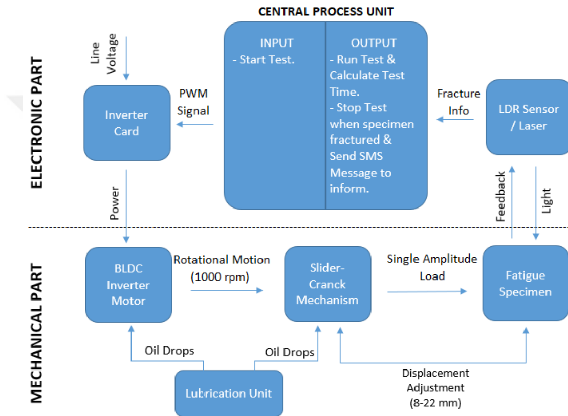
Figure 3.10. Flowchart of Fatigue Test Machine & Set-up
