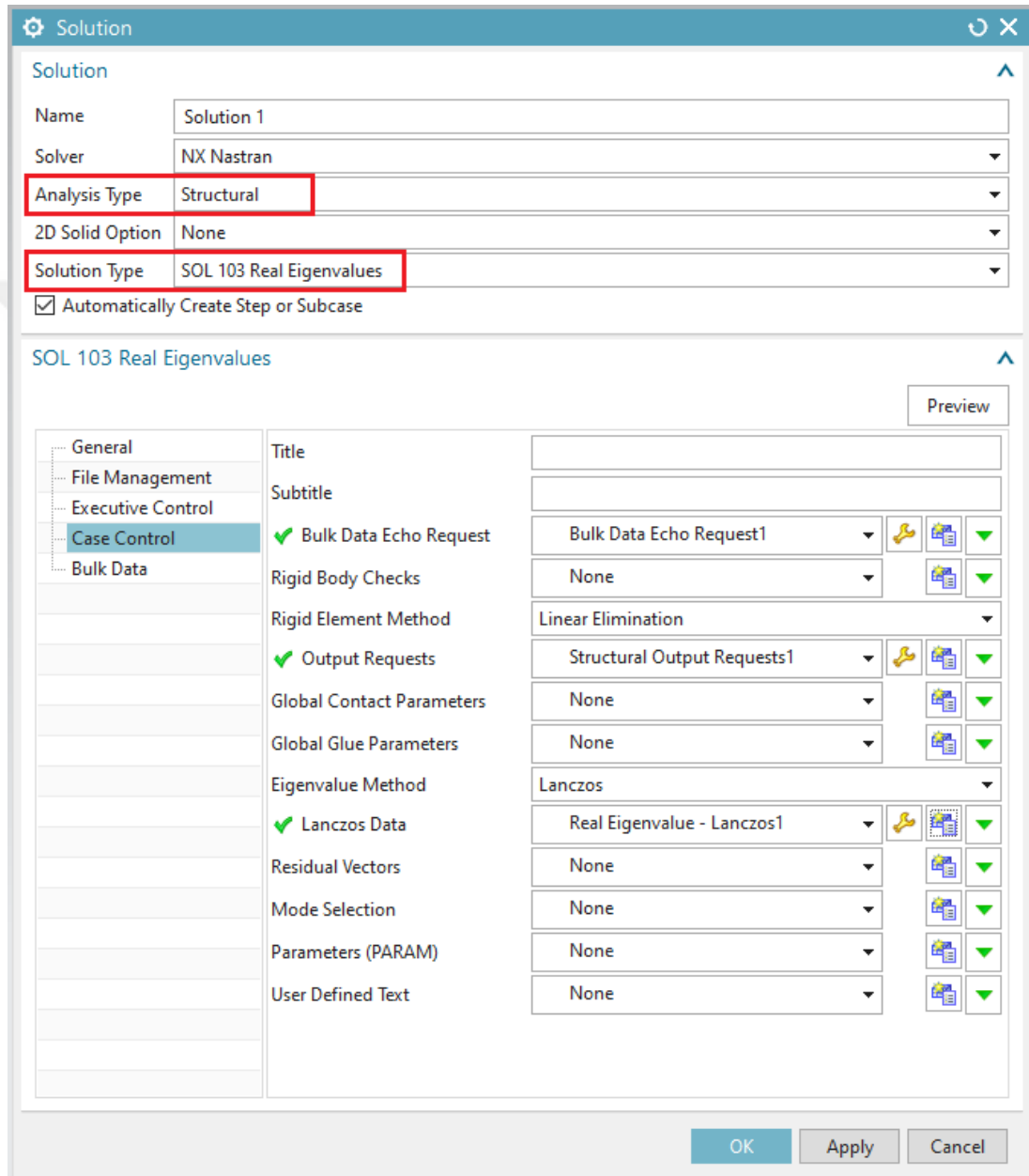
Figure 3.21. Solution Type of Numerical Modal Analysis on Fatigue Specimen Model
