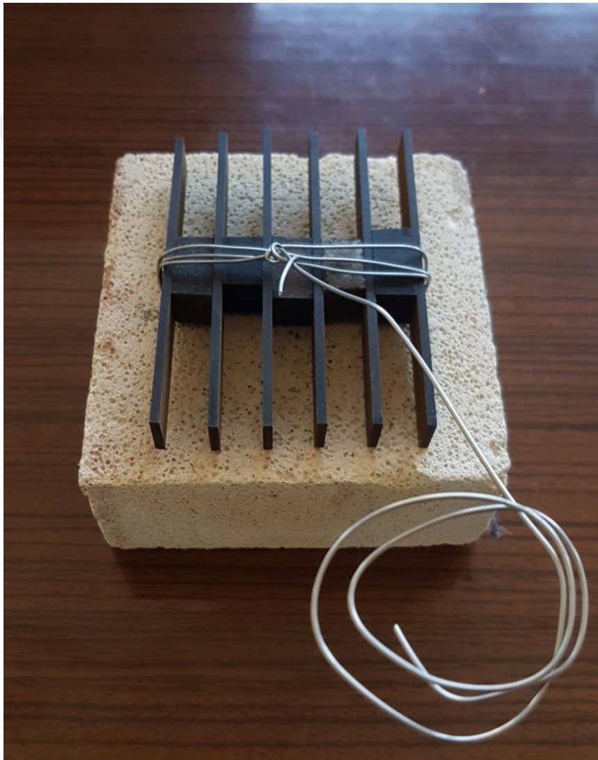
Figure 3.25. Fatigue Specimens before Heat Treatment Process
