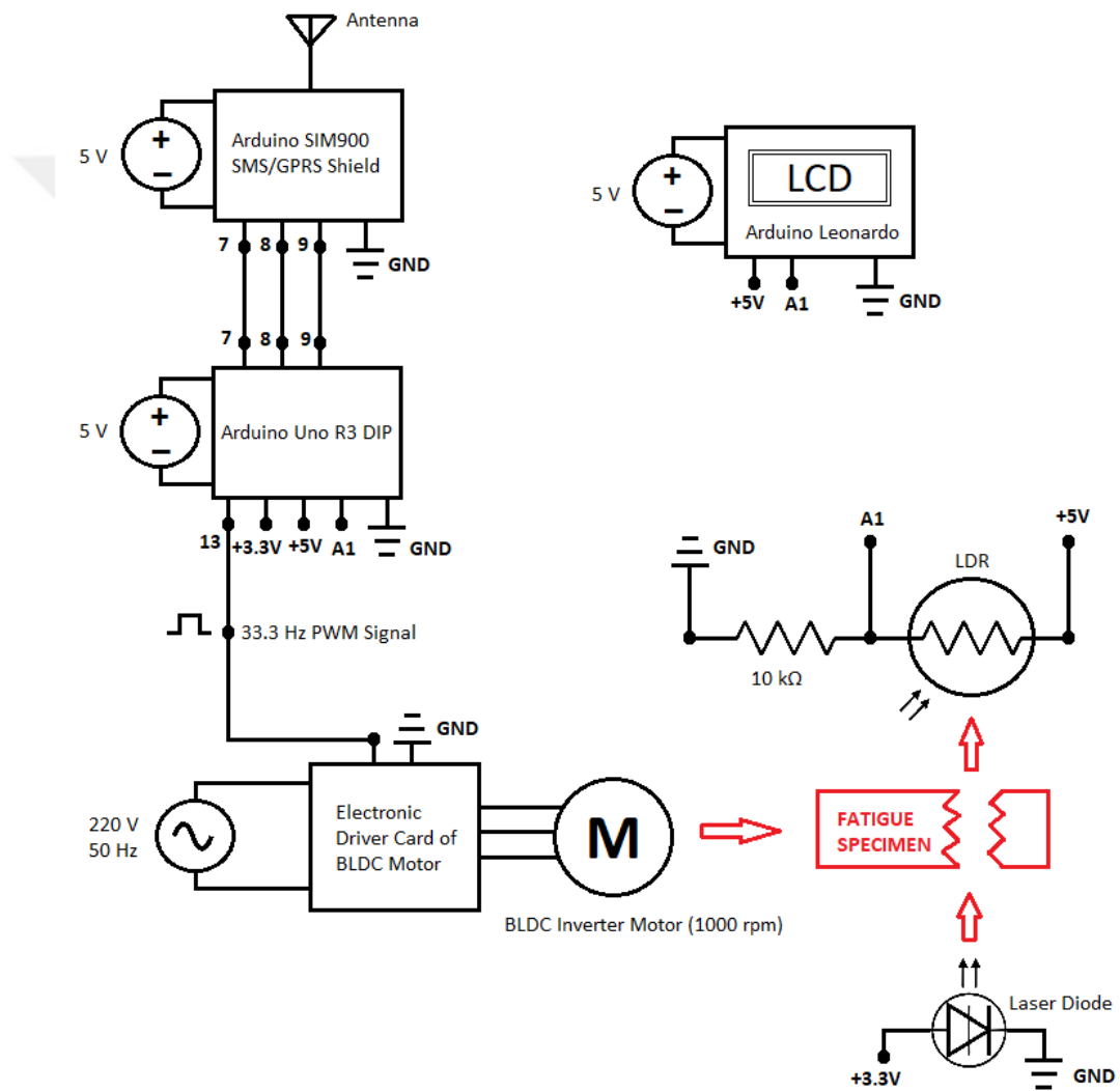
Figure A.1. Circuit Diagram of Central Process Unit
