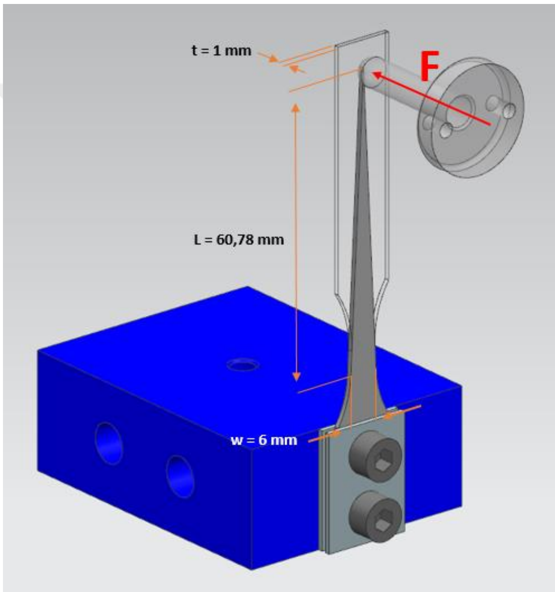
Figure 4.24. Dimensions needed for Simple Beam Equation
