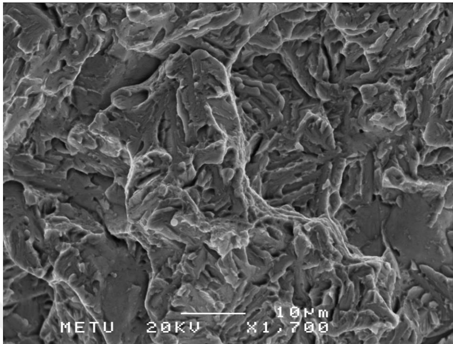
Figure 4.39. Fast Fracture Zone of a LB-250 Fatigue Specimen, which shows cleavages
