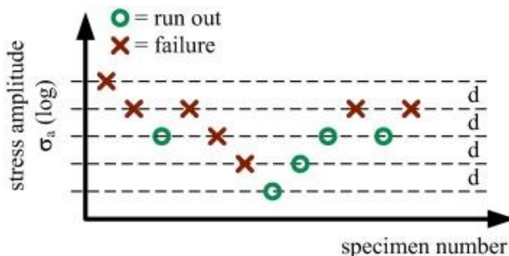
Figure 2.6. Staircase Method [15]
