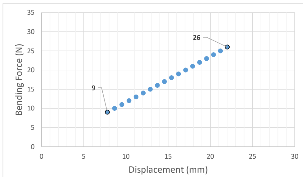
Figure 4.14. Numerical Bending Forces
