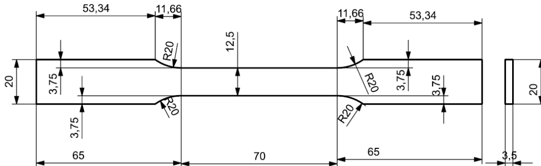
Figure 3.4. Technical Drawing of Tensile Test Specimen [37]
