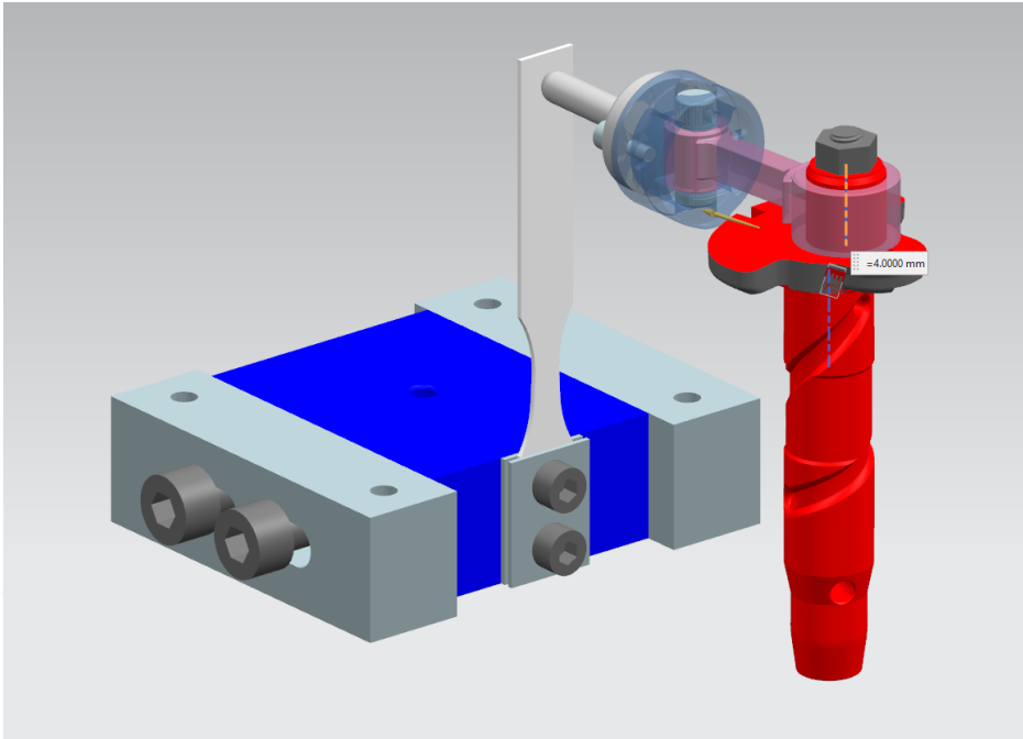
Figure 3.44. Minimum Displacement Orientation of Fatigue Test Machine, which corresponds to a distance of 4 mm on crank shaft & 8 mm Displacement on Fatigue Specimen
