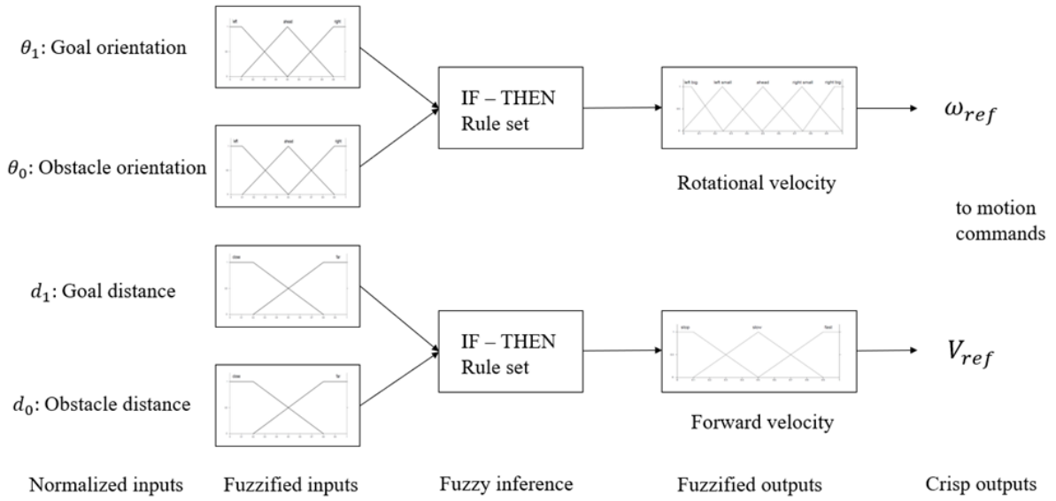
Figure 3.8. Fuzzy Reactive Control Interface
