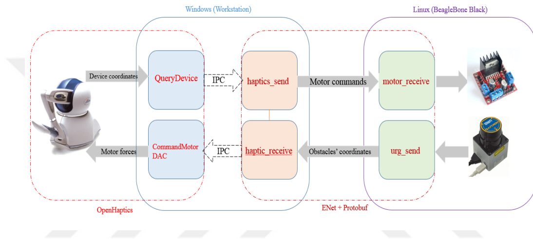
Figure 4.15. General overview of the communication platform
