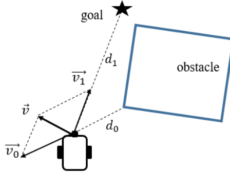
Figure 3.7. Superposition of the effects of the goal and an obstacle
