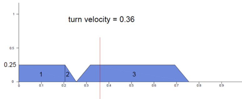
Figure 3.15. Center of area defuzzification method
