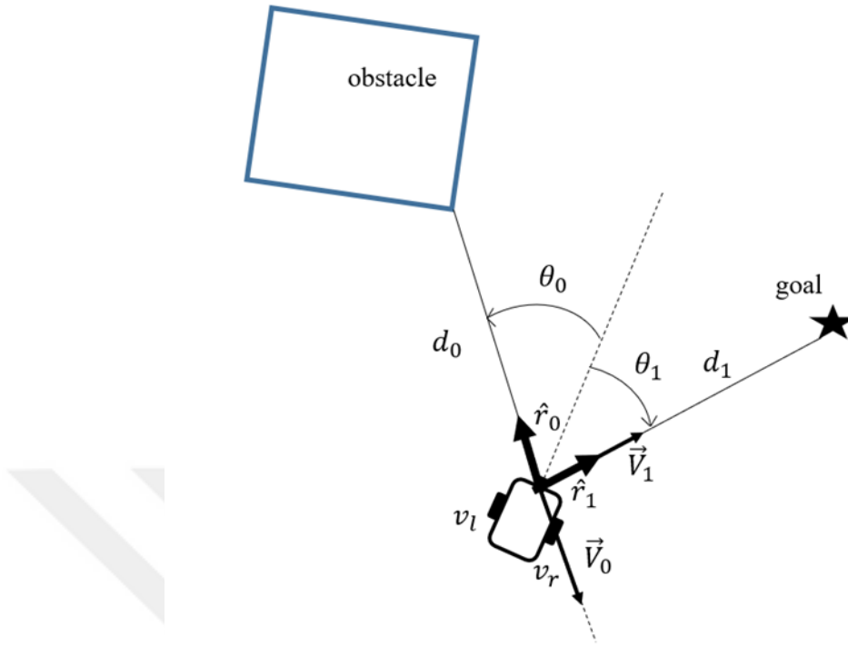
Figure 3.20. force vector affecting the robot
