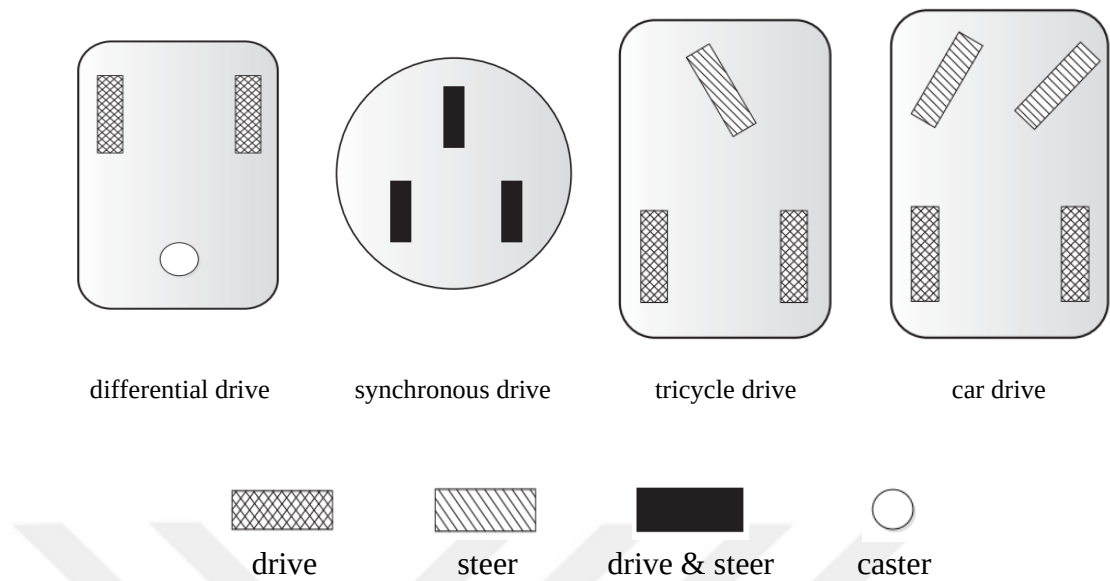
Figure 2.2. Wheeled mobile robot classification
