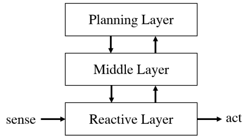
Figure 2.3. Three-layer hybrid Control Architecture
