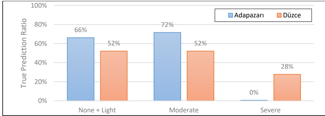
Figure 3.1. True prediction ratios of linear discriminant and tripartite category model (Equation 3.1)
