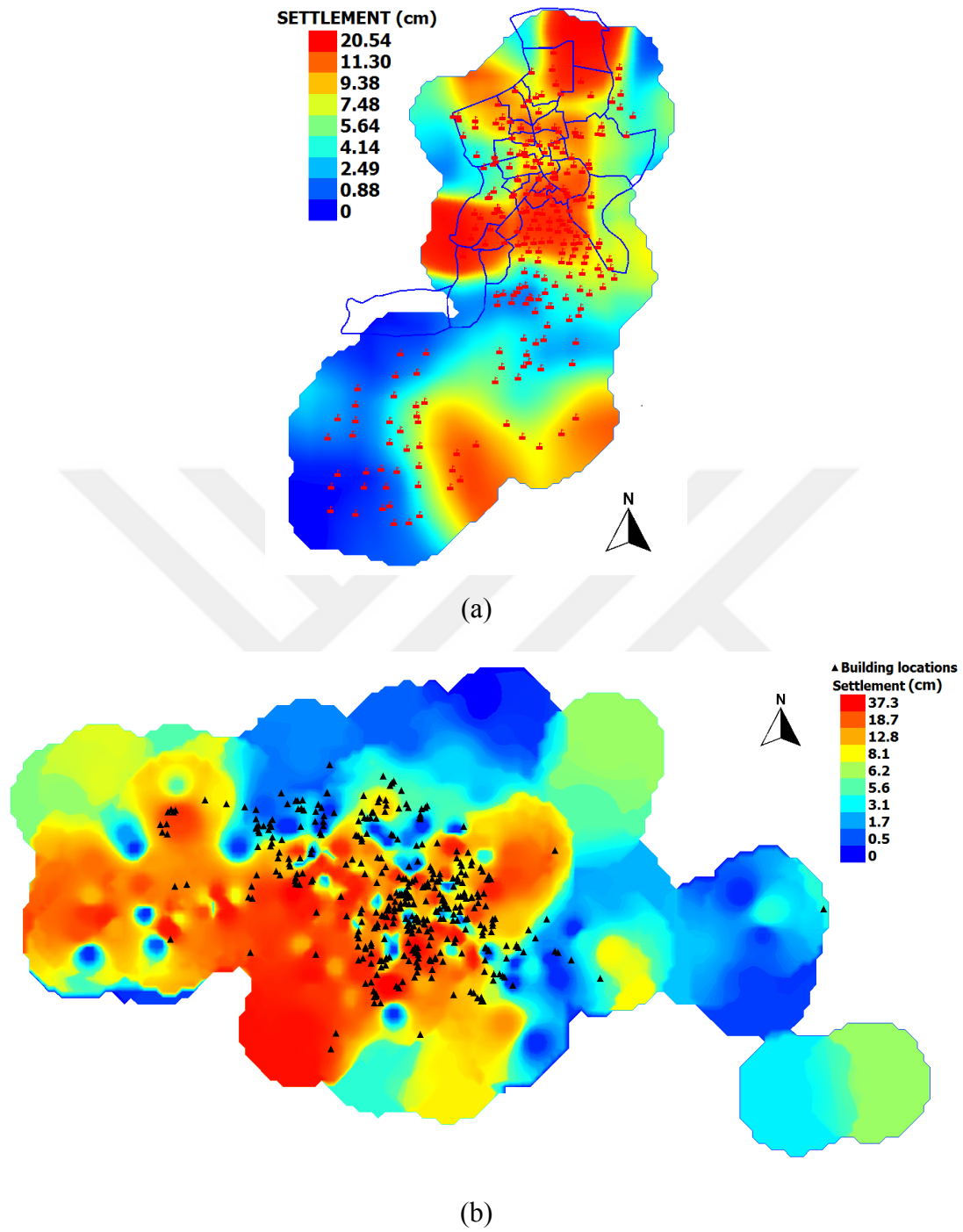
Figure 2.12. Liquefaction Induced Settlement Contours in Adapazarı (a) and in Düzce (b)
