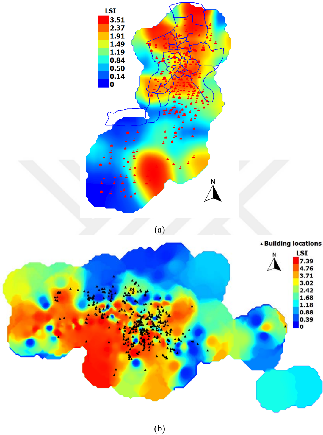
Figure 2.9. Liquefaction Severity Index contours in Adapazarı (a) and in Düzce (b).
