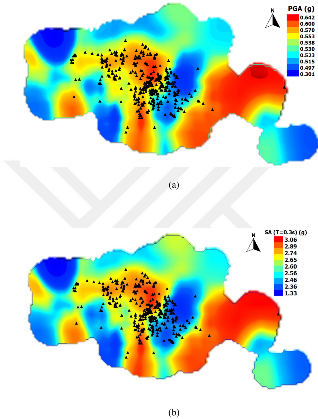
Figure 2.7. Contours for (a) PGA (g) and (b) Spectral Acceleration (g) for T=0.3s in Düzce
