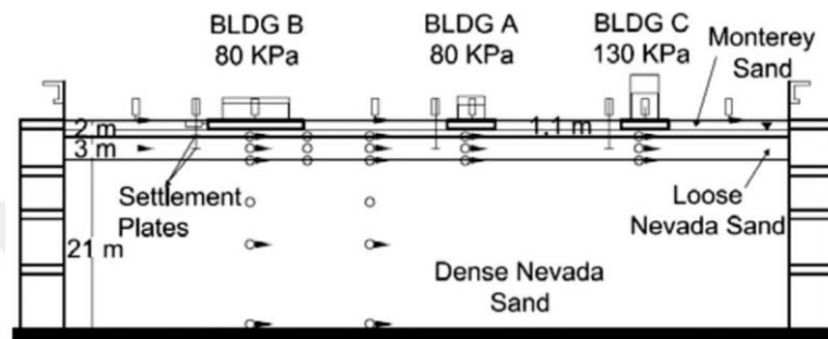
Figure 1.11. Centrifuge testing model by Dashti et al (2009)
