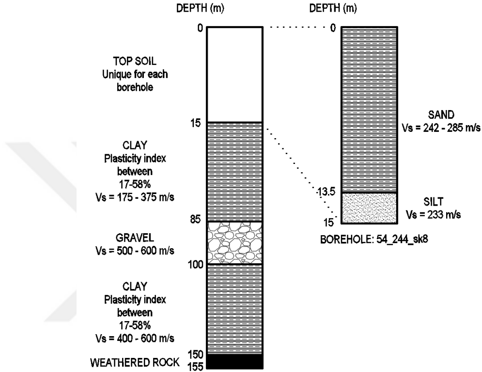
Figure 2.3. 1-D soil column used in site response analysis by Yilmaz (2004) with a sample borehole used to define the top soil layers in Adapazari
