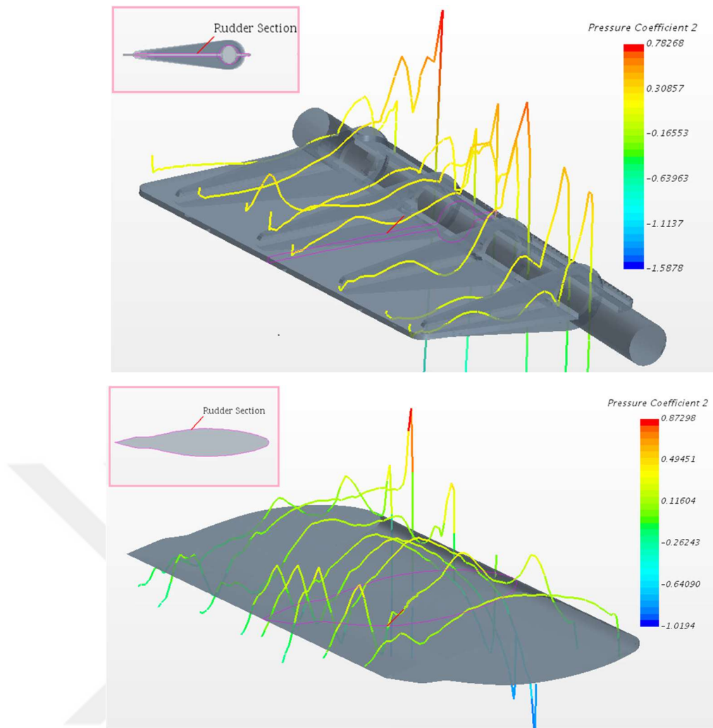
Figure 6-31 2D Pressure Distribution Plots over 3D rudder surfaces (Top; The Princess Royal Rudder, Right; Conventional Rudder)
