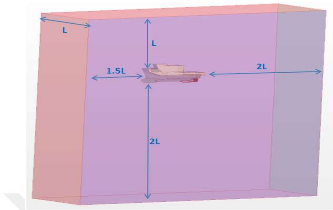
Figure 7-12 Computational Flow Domain (Full Scale)
