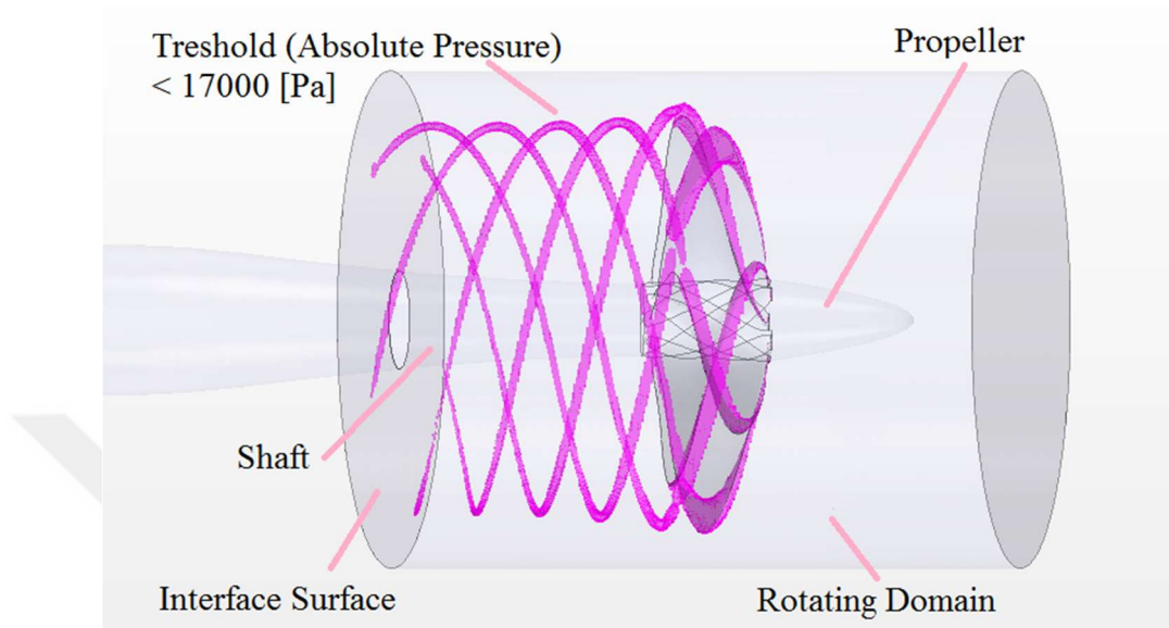
Figure 5-7 Absolute pressure threshold below 17000 [Pa]
