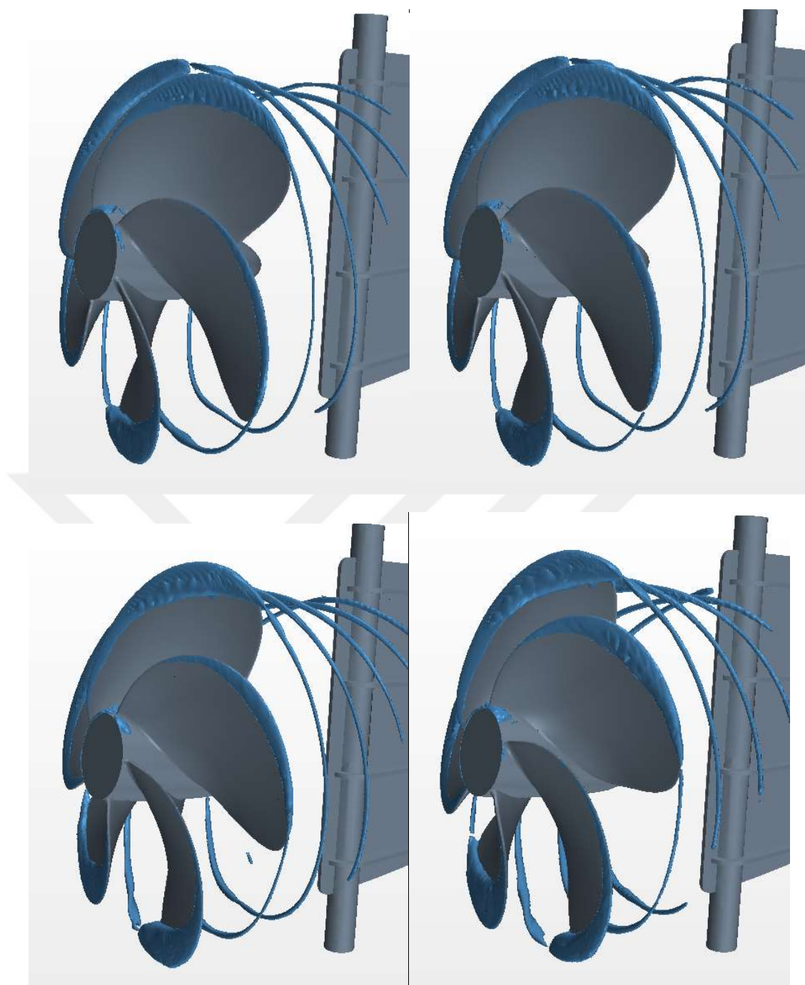
Figure 6-25 The Princess Royal Propeller – Rudder Arrangement: Condition 4 – CFD Results; Cavitation Pattern including extended TVC
