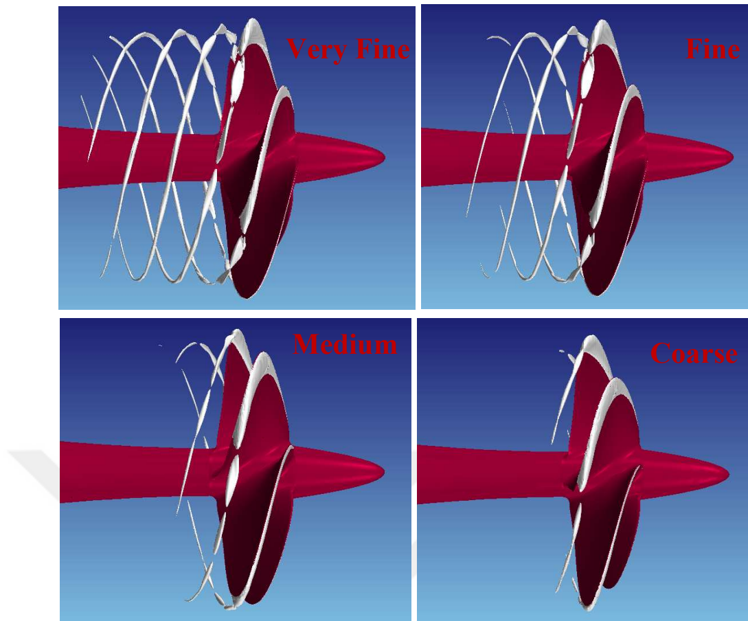
Figure 3-16 Tip Vortex Cavitation Extension for V&V Studies
