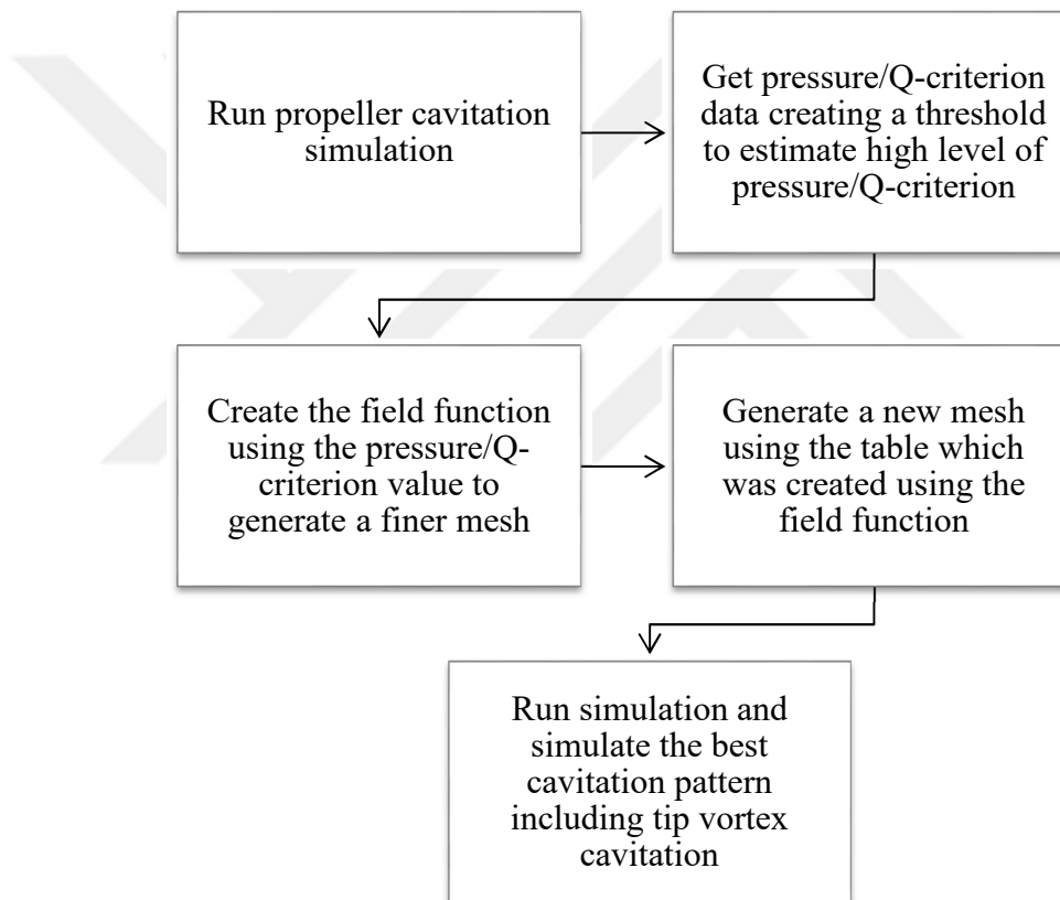
Figure 5-9 Modified Flow chart summarising MARCS in order to reduce total number of cells
