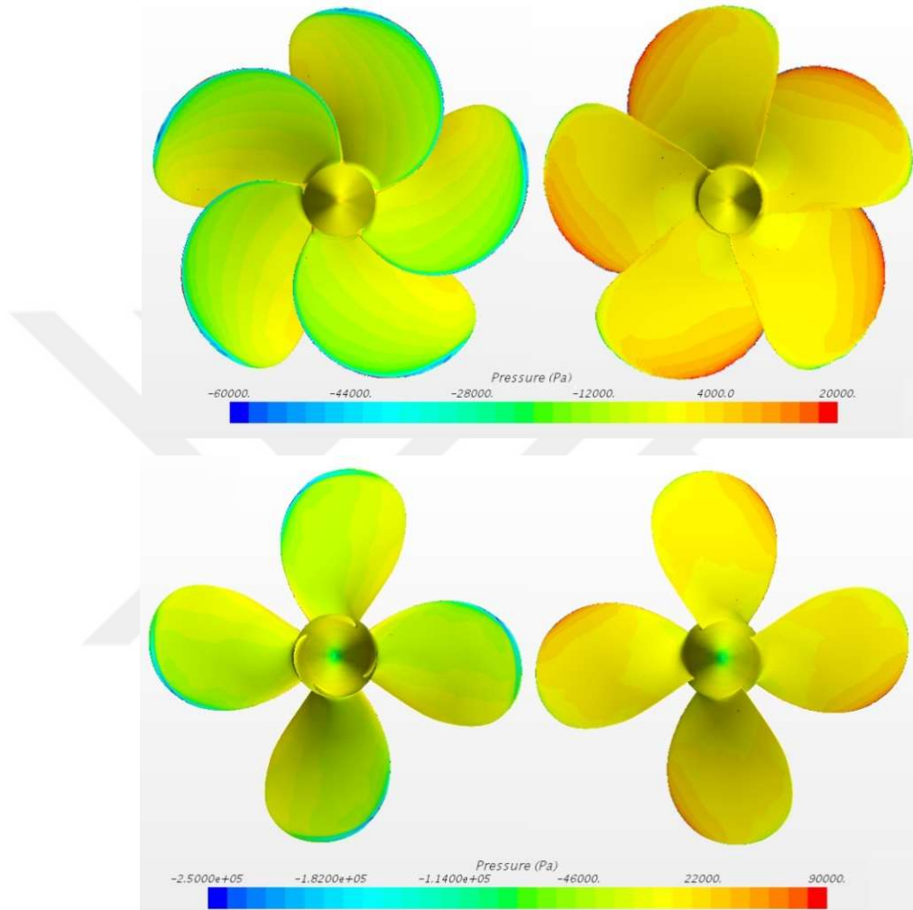
Figure 4-10 Pressure distribution on propeller surfaces (Left; Suction Side, Right; Pressure Side) (Top; The Princess Royal , Bottom; INSEAN E779A )
