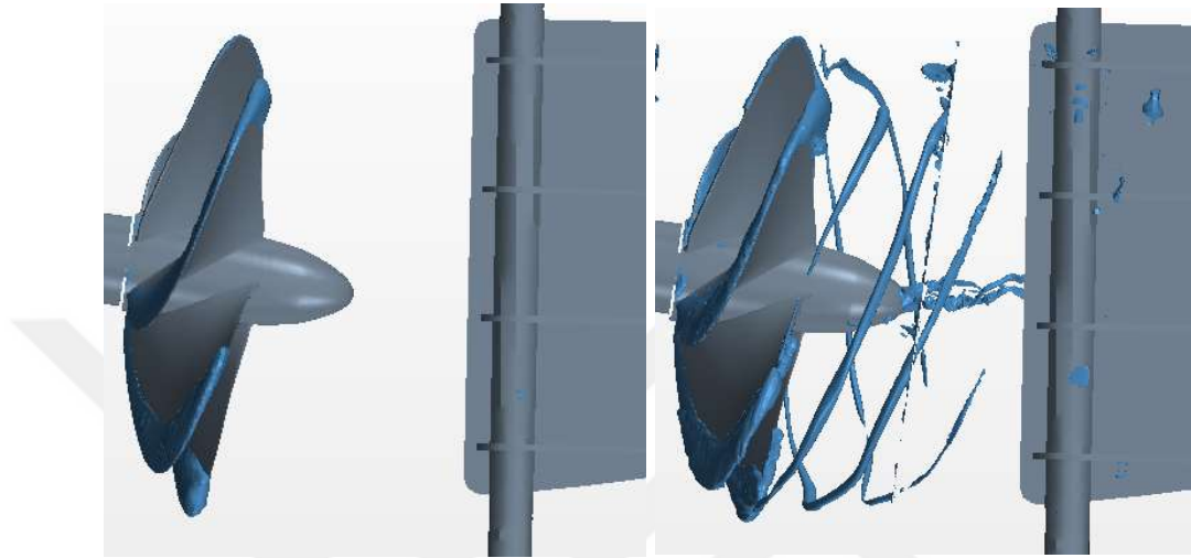
Figure 7-21 CFD Results- Cavitation pattern (Left; Sheet Cavitation, Right; tip vortex cavitation (MARCS) (Model Scale)
