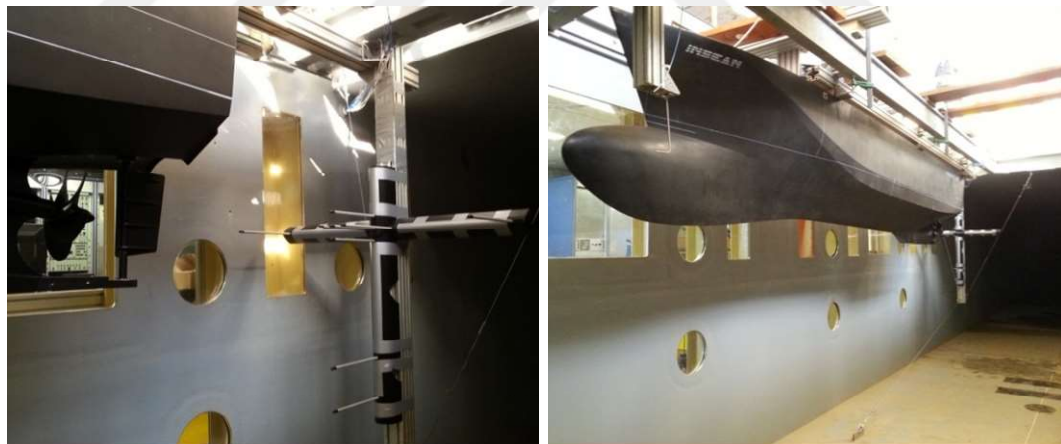
Figure 7-4 Cavitation observations: set up arrangement
