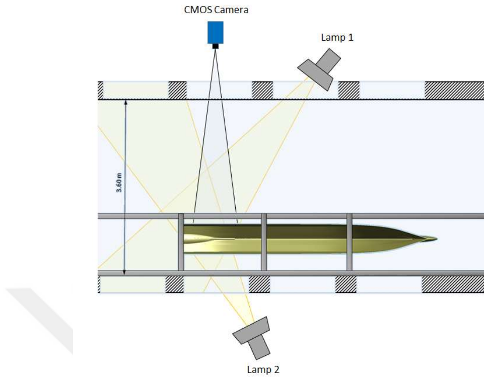
Figure 7-3 Stroscopic lights and camera arrangement
