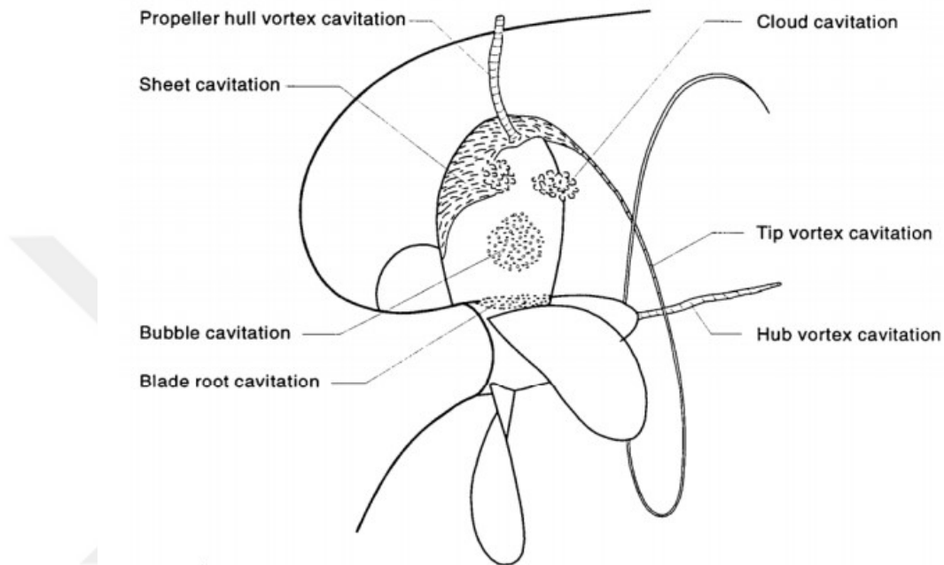
Figure 2-6 Cavitation Types (ITTC, 2002)
