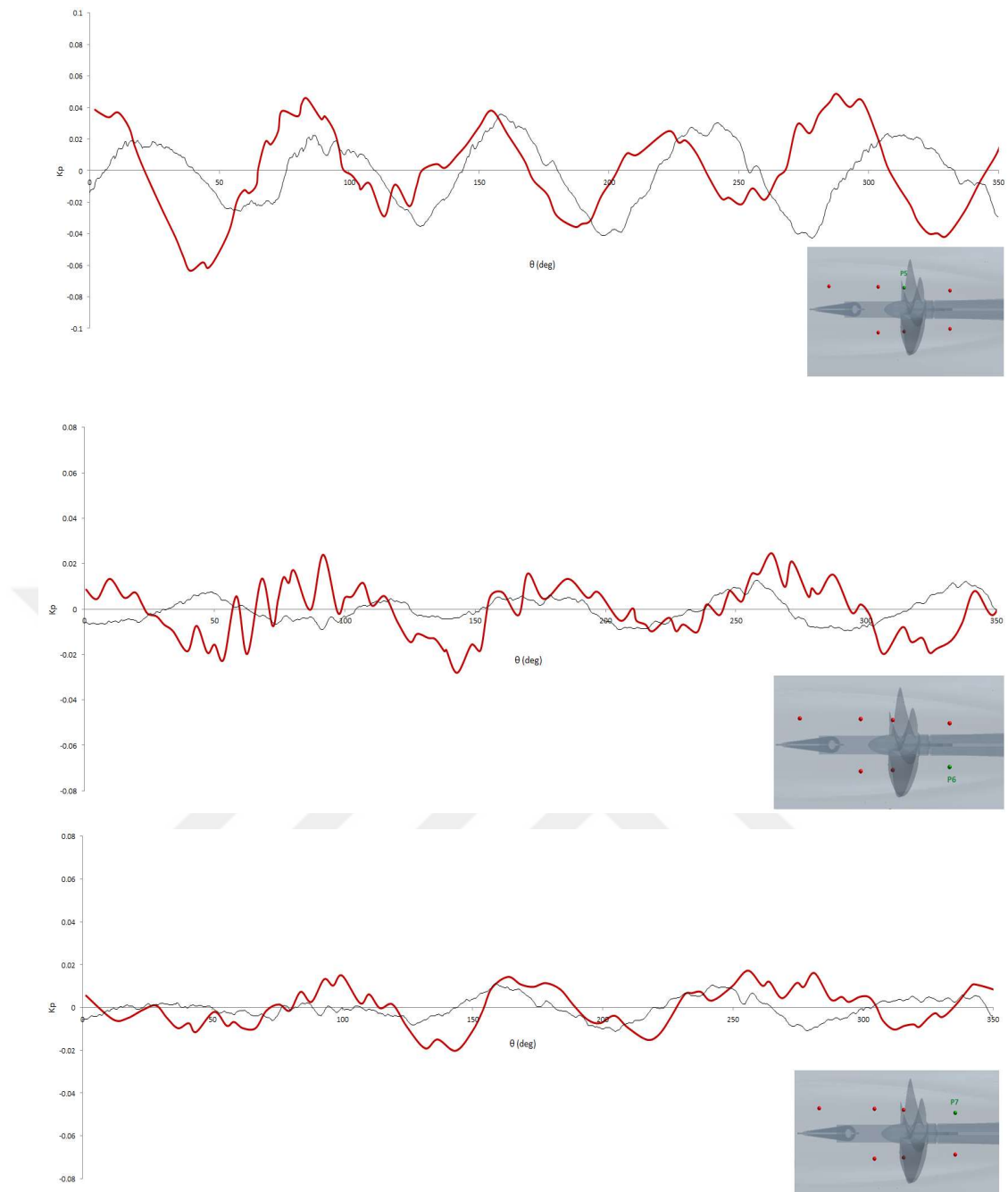
Figure 7-24 Hull Pressure Fluctuations Comparisons between EFD (Red) and CFD (Black) Results (Sheet Cavitation, From Top to Bottom; P5, P6 and P7)
