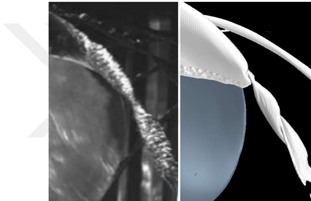
Figure 5-13 The INSEAN E779A : Comparison of Results Tip Vortex Cavitation Roll-up (Left; EFD, Right; CFD, MARCS)
