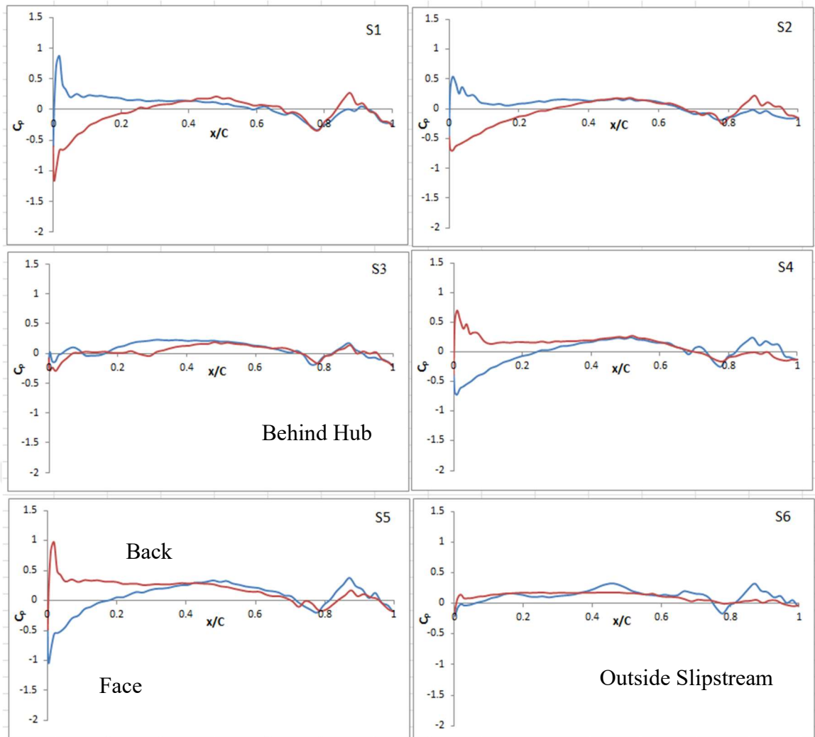
Figure 6-17 The Propeller-Convectional Rudder Arrangement : Chordwise pressure distribution at 6 spanwise positions for rudder (MARCS) (From top to bottom; S1-S6) (Red: Back, Blue: Face)
