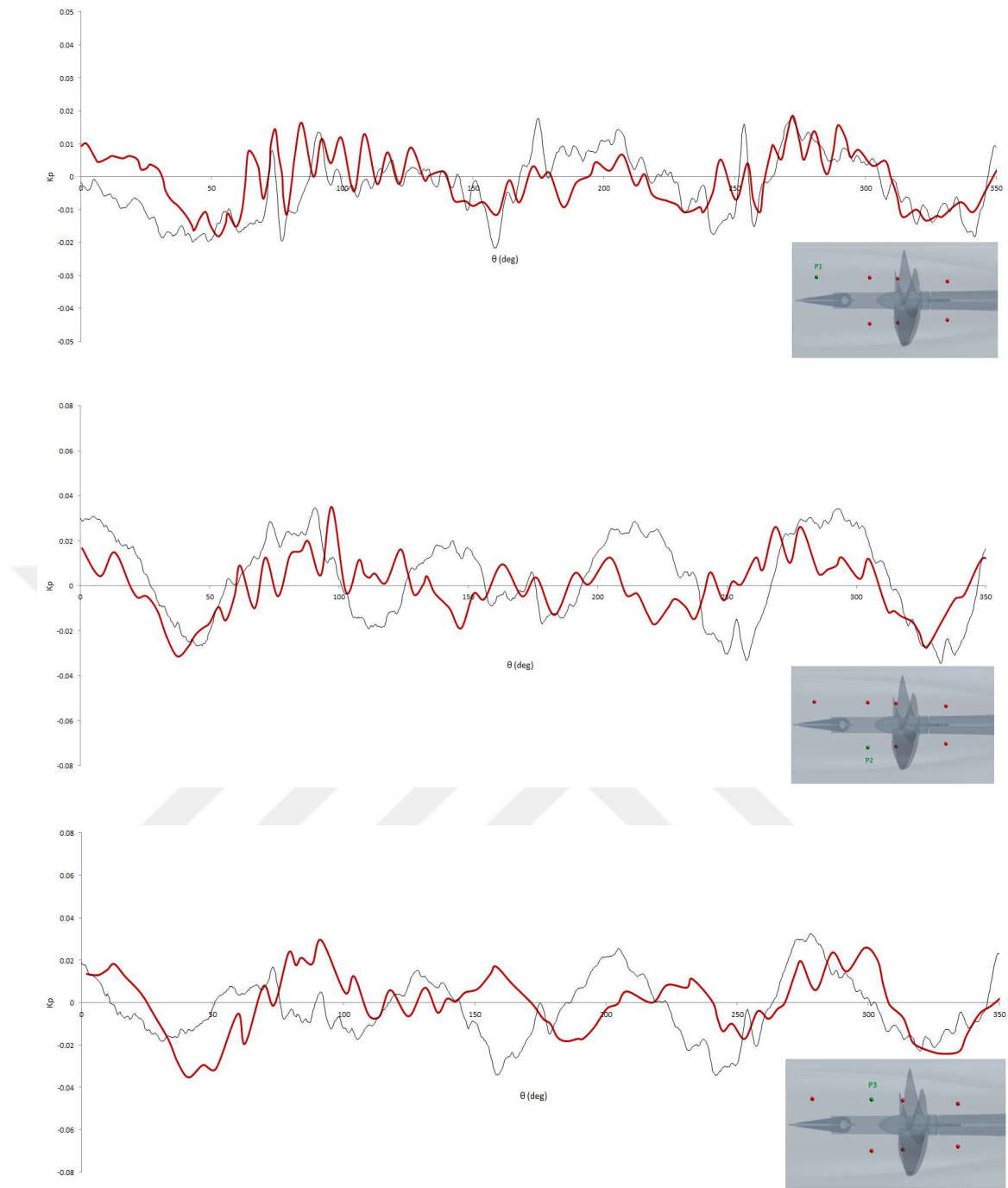
Figure 7-23 Hull Pressure Fluctuations Comparisons between EFD (Red) and CFD (Black) Results (Sheet Cavitation, From Top to Bottom; P1, P2 and P3)
