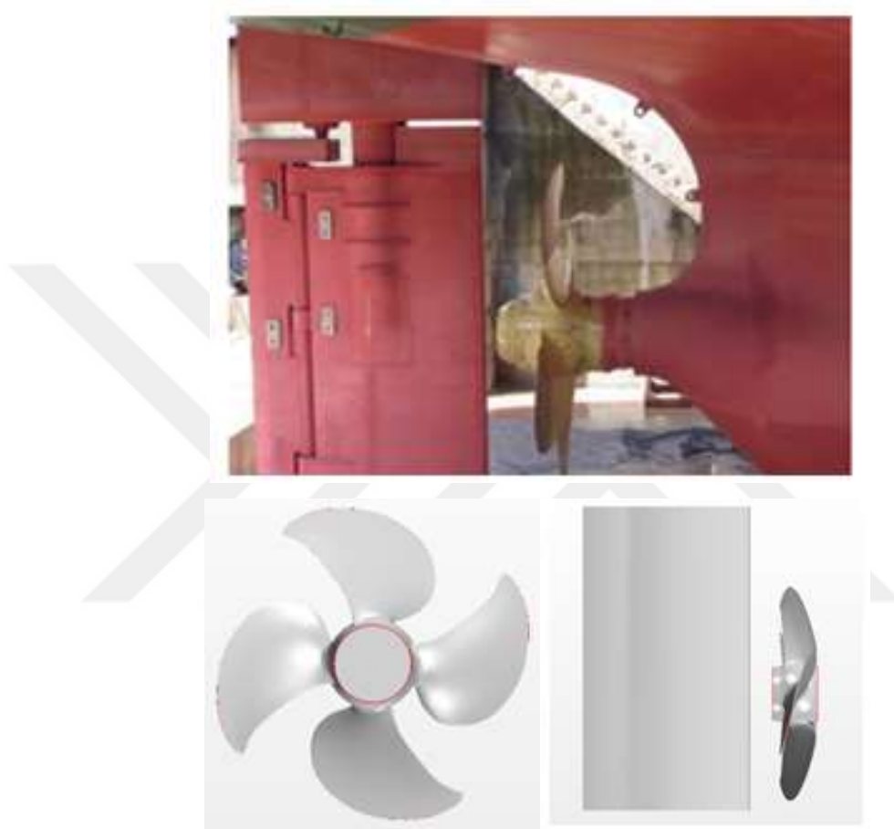
Figure 6-3 Propeller-Conventional Rudder Arrangement
