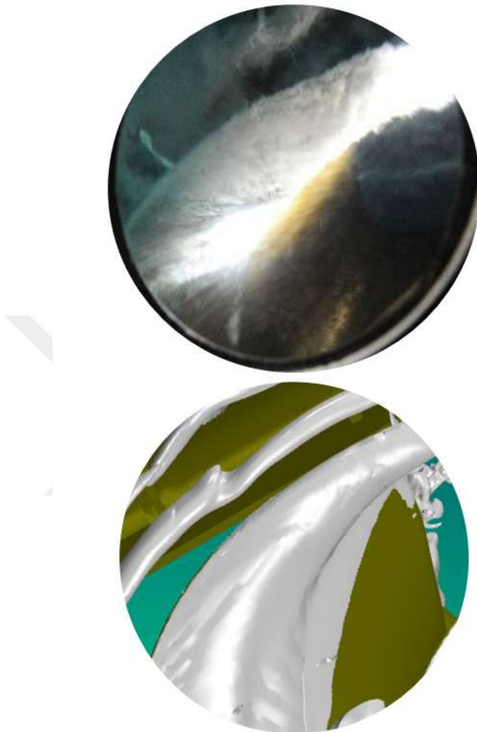
Figure 7-27 Cavitation pattern Comparisons between Sea Trials and CFD (Full Scale) (Top; Sea Trials, Bottom; CFD) (MARCS - tip vortex cavitation)
