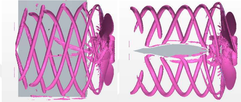
Figure 6-6 Isosurface of Q\text{-Criterion} = 20000 \text{ s}^{-2}
