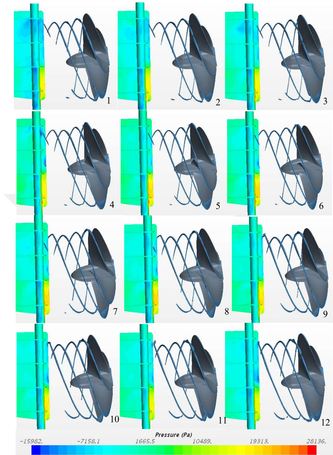
Figure 6-34 The Princess Royal Propeller – Rudder Arrangement: The deformation of the TVC in the presence of the rudder and pressure distribution on the rudder (Starboard side view)
