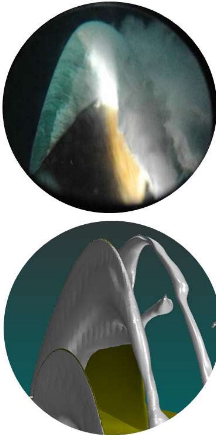
Figure 7-28 Cavitation pattern Comparisons between Sea Trials and CFD (Full Scale) (Top; Sea Trials, Bottom; CFD) (MARCS - tip vortex cavitation)
