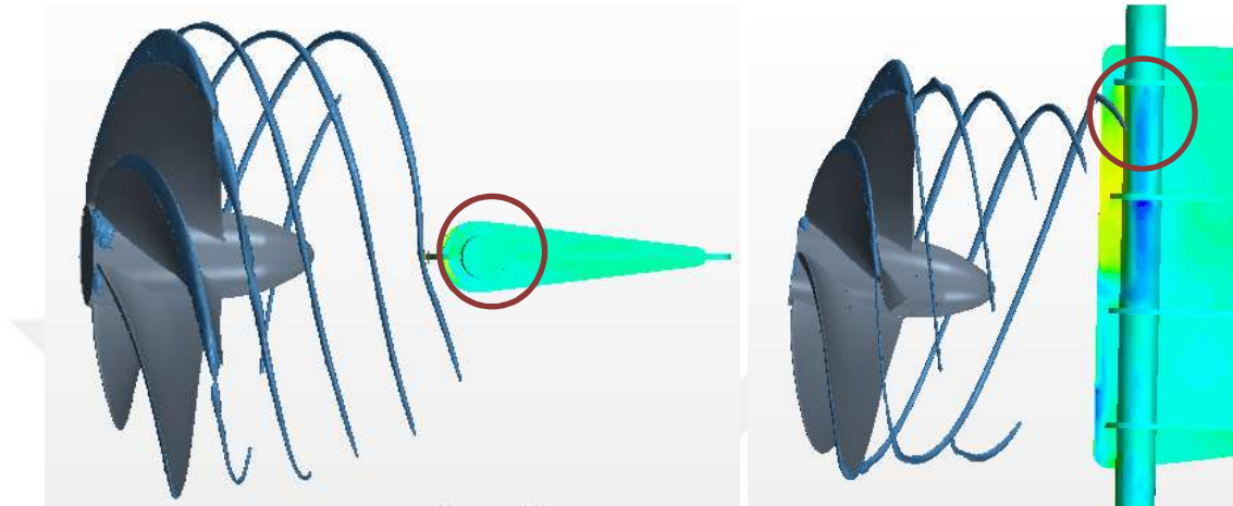
Figure 6-28 The Princess Royal Propeller – Rudder Arrangement: Vortex Interaction with Leading Edge
