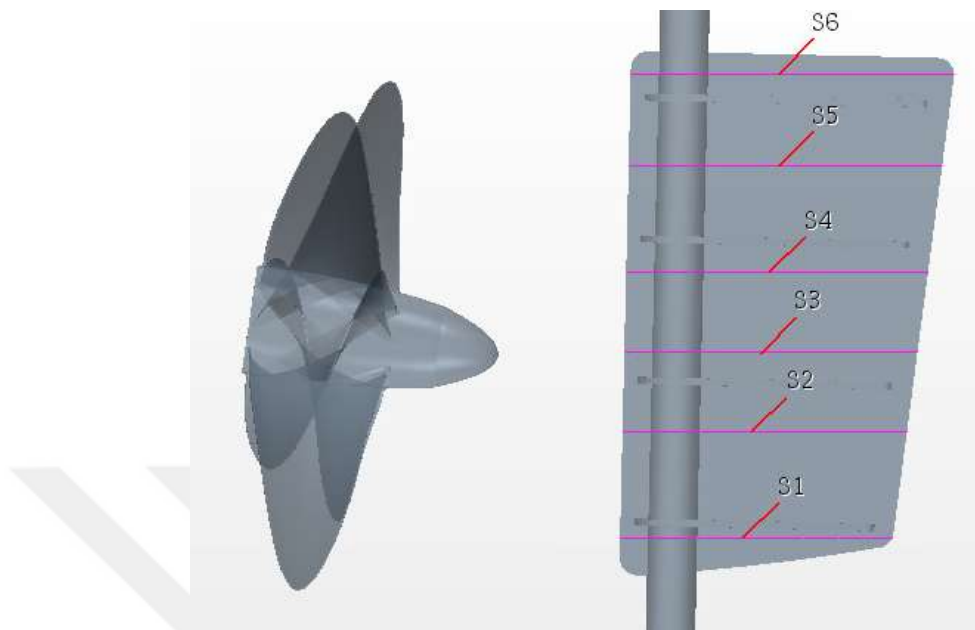
Figure 6-29 The Princess Royal Propeller – Rudder Arrangement : Section Planes (z direction) for pressure distribution calculations
