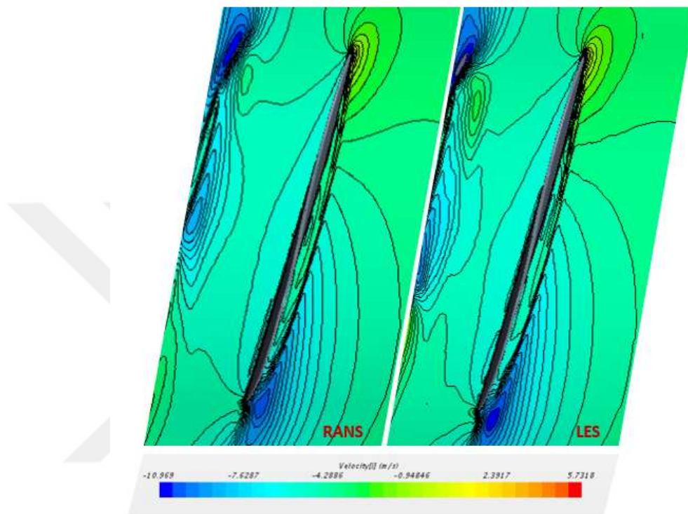
Figure 5-32 Axial Velocity Comparisons between RANS and LES (0.9R Cylindrical Section)
