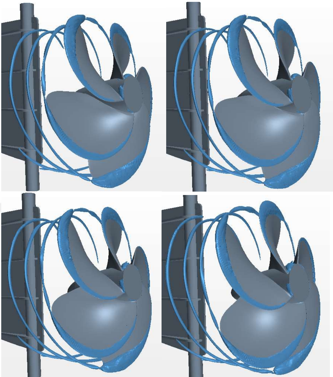
Figure 6-27 The Princess Royal Propeller – Rudder Arrangement : Condition 4 – CFD Results; Cavitation Pattern including extended TVC
