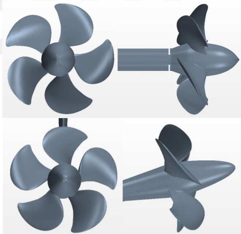
Figure 3-6 CAD geometry of the PPTC VP 1304 Propeller (Top; PPTC with axial shaft, Bottom; PTTC with inclined shaft)
