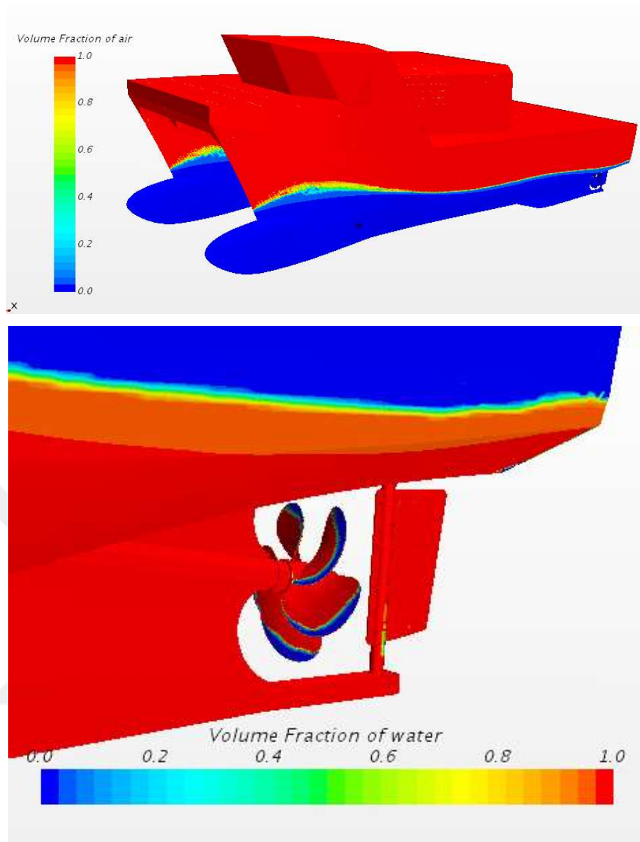
Figure 7-25 Free surface representation (Full Scale) (Top; Volume Fraction of Air, Bottom; Volume Fraction of Water including sheet cavitation on propeller blades)
