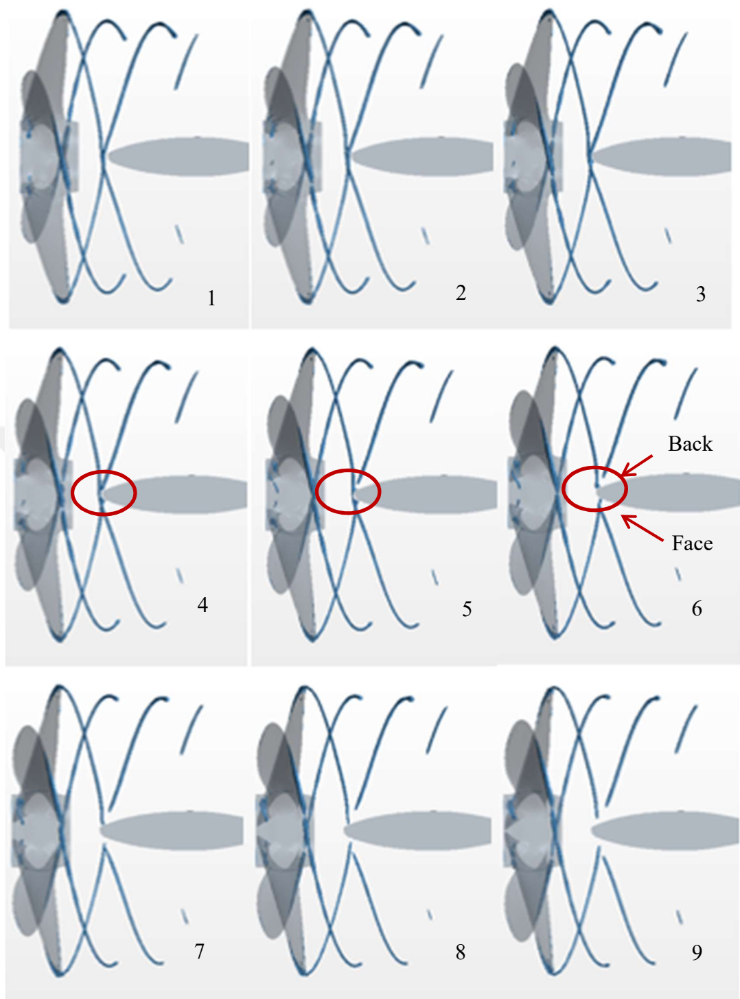
Figure 6-19 The Propeller-Convectional Rudder Arrangement : Vortex Interaction with Rudder Leading Edge (From Top View)
