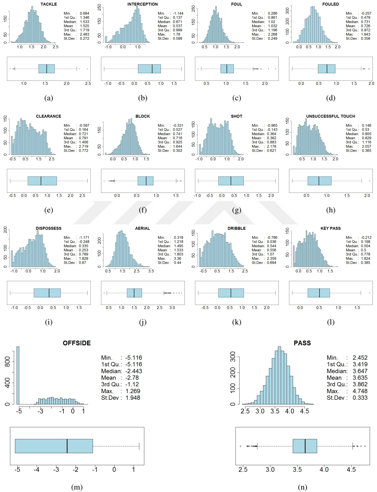
Figure 4.9: Summary of upper level count variables after \log(x + c) is applied
