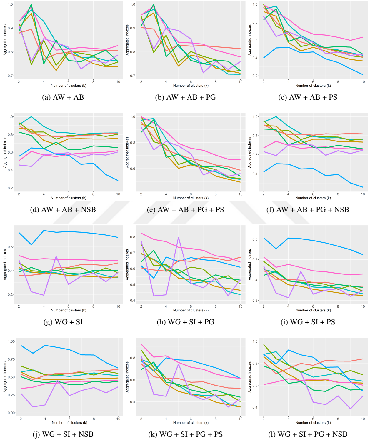
Figure 7.21: Different aggregated index considerations with Z-score standardisation for SEED data set.
