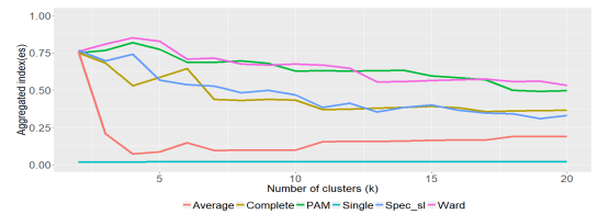
(j) CVNN ( \kappa = 10 ) Index K \sim [2 : 20]
