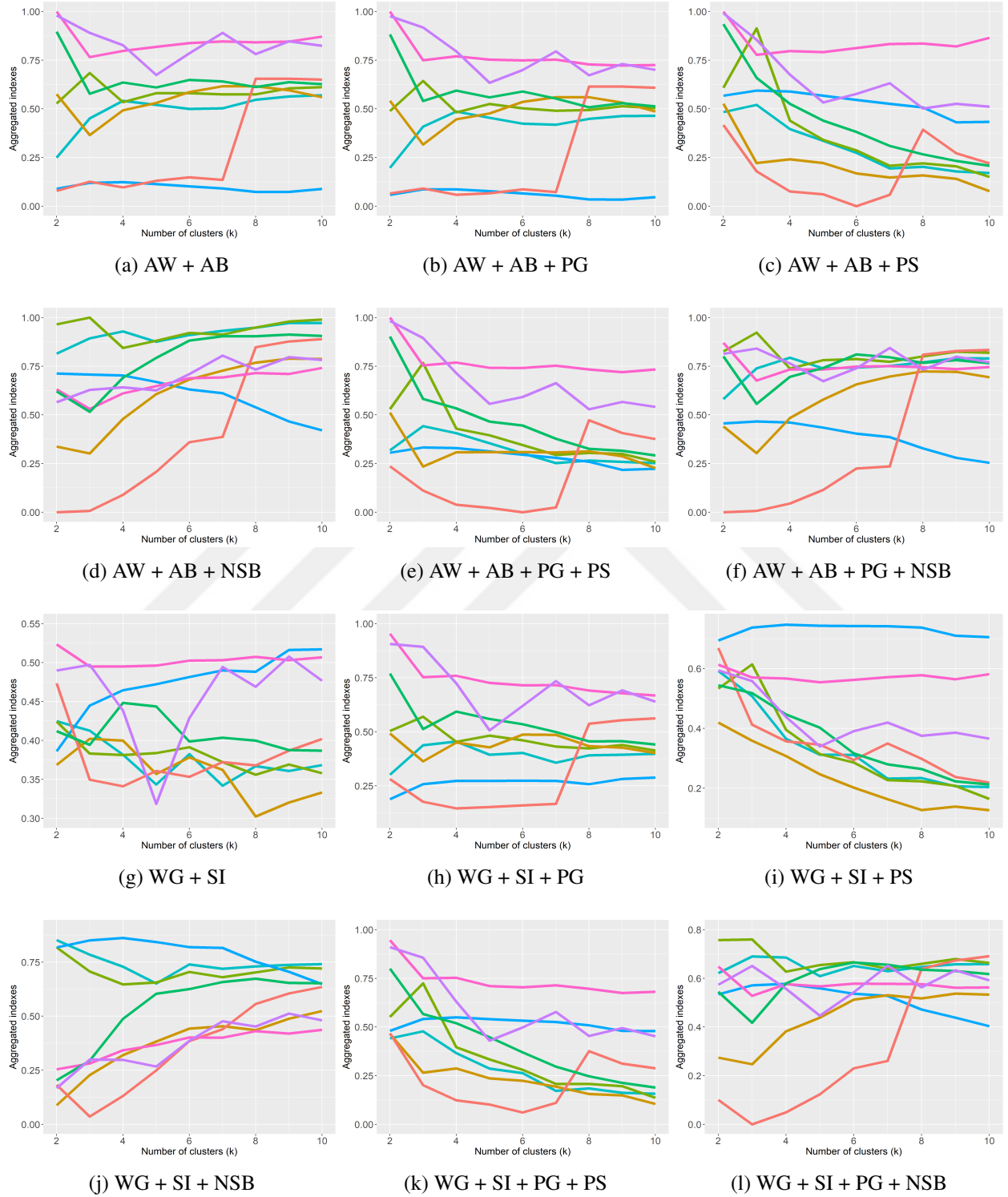
Figure 7.19: Different aggregated index considerations with Range standardisation for WINE data set.
