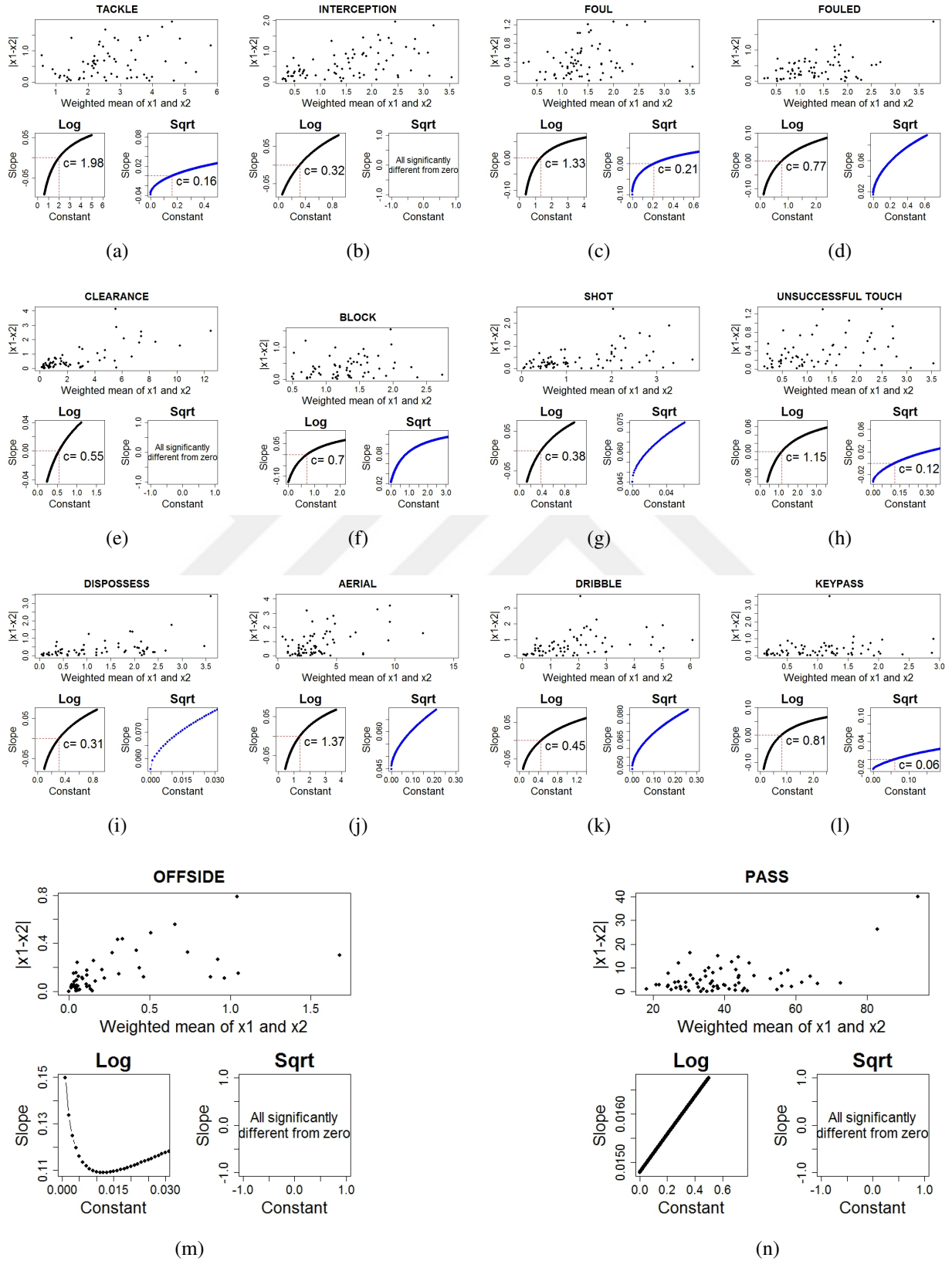
Figure 4.8: Analysis for optimal constant values on log and square root transformations
