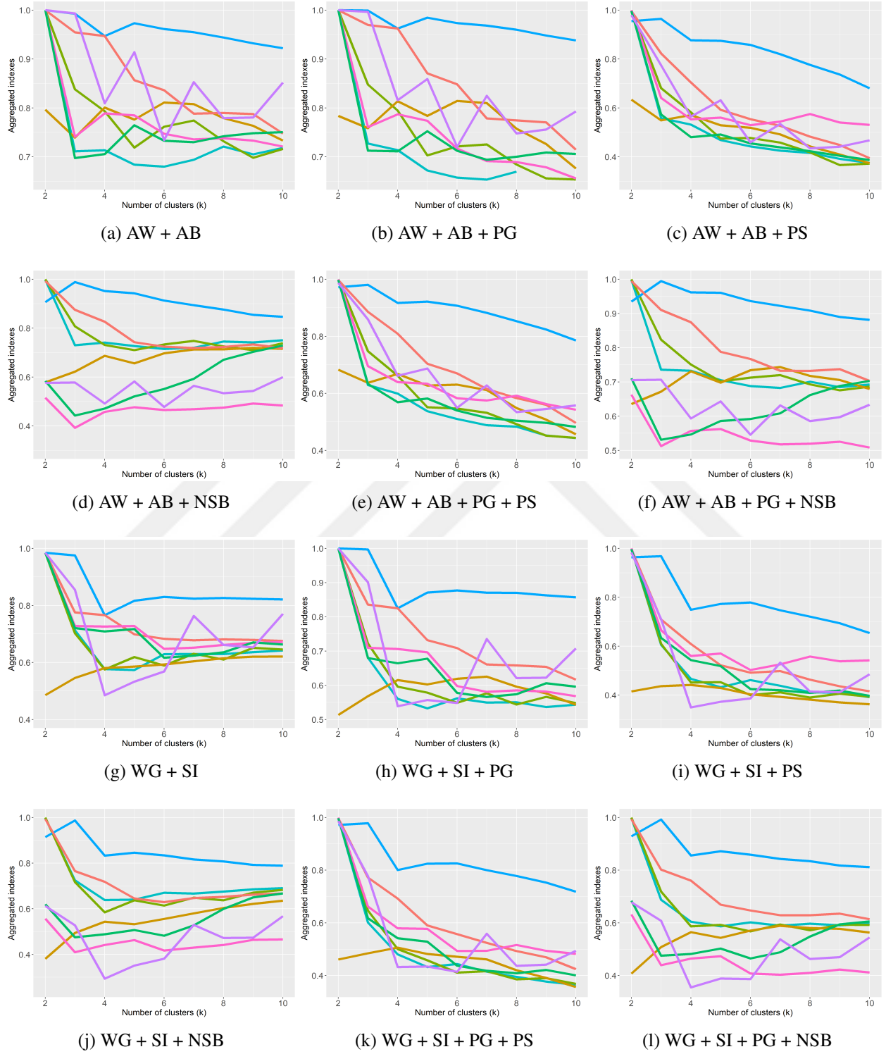
Figure 7.15: Different aggregated index considerations with Z-score standardisation for IRIS data set.
