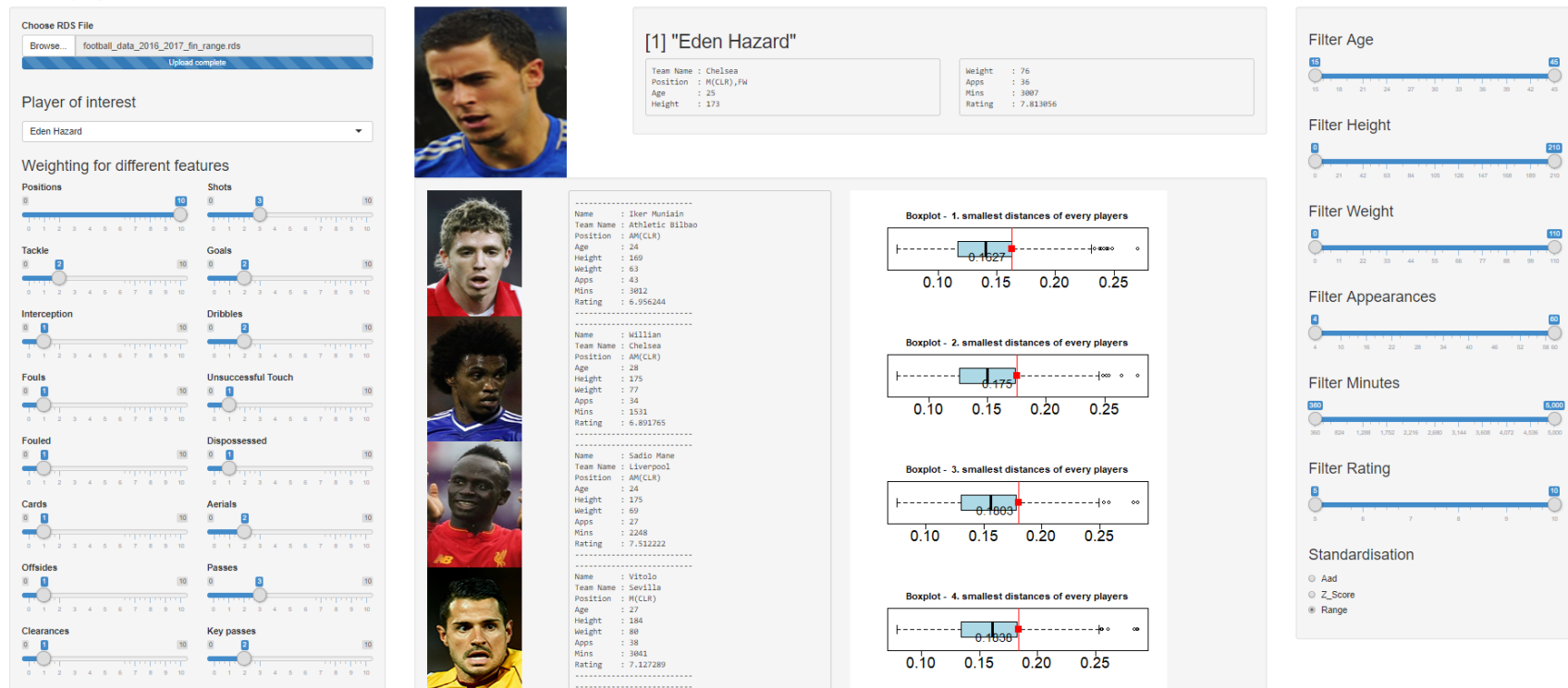
Figure B.4: R Shiny implementation for distance queries of football players
