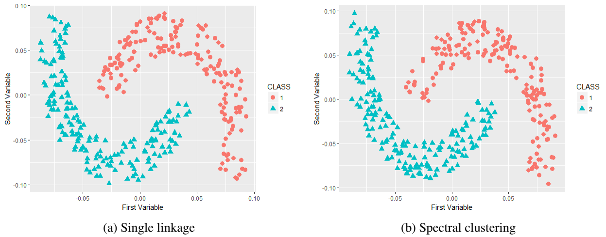
Figure 7.6: Two clusters in two dimensions with two moon shapes - Two dimensional representation of a randomly selected simulated data set out of 50 replications
