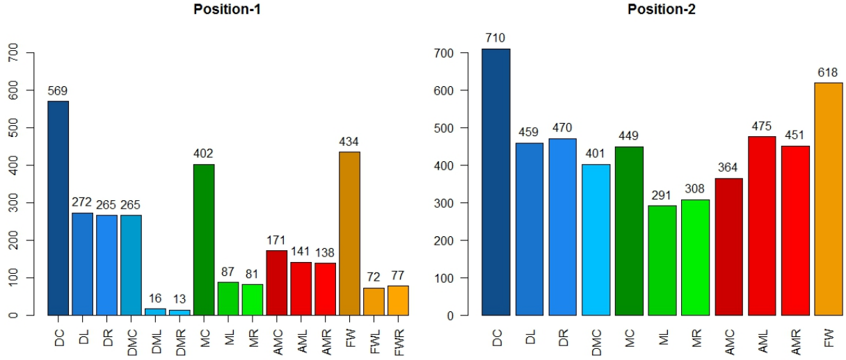
Figure 4.2: Frequencies of position variables, Y_{(15)} and Y_{(11)} , respectively.
