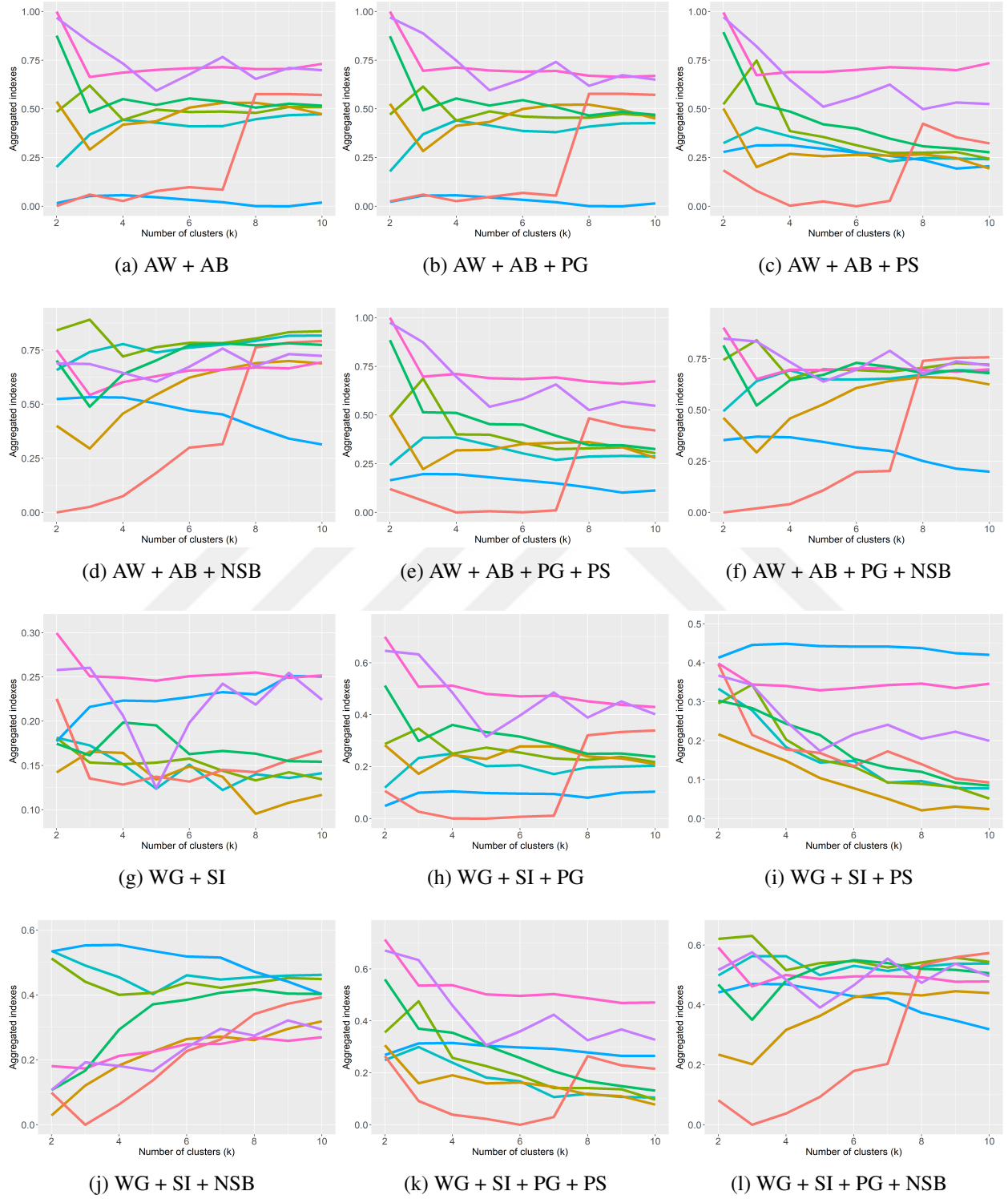
Figure 7.18: Different aggregated index considerations with Z-score standardisation for WINE data set.
