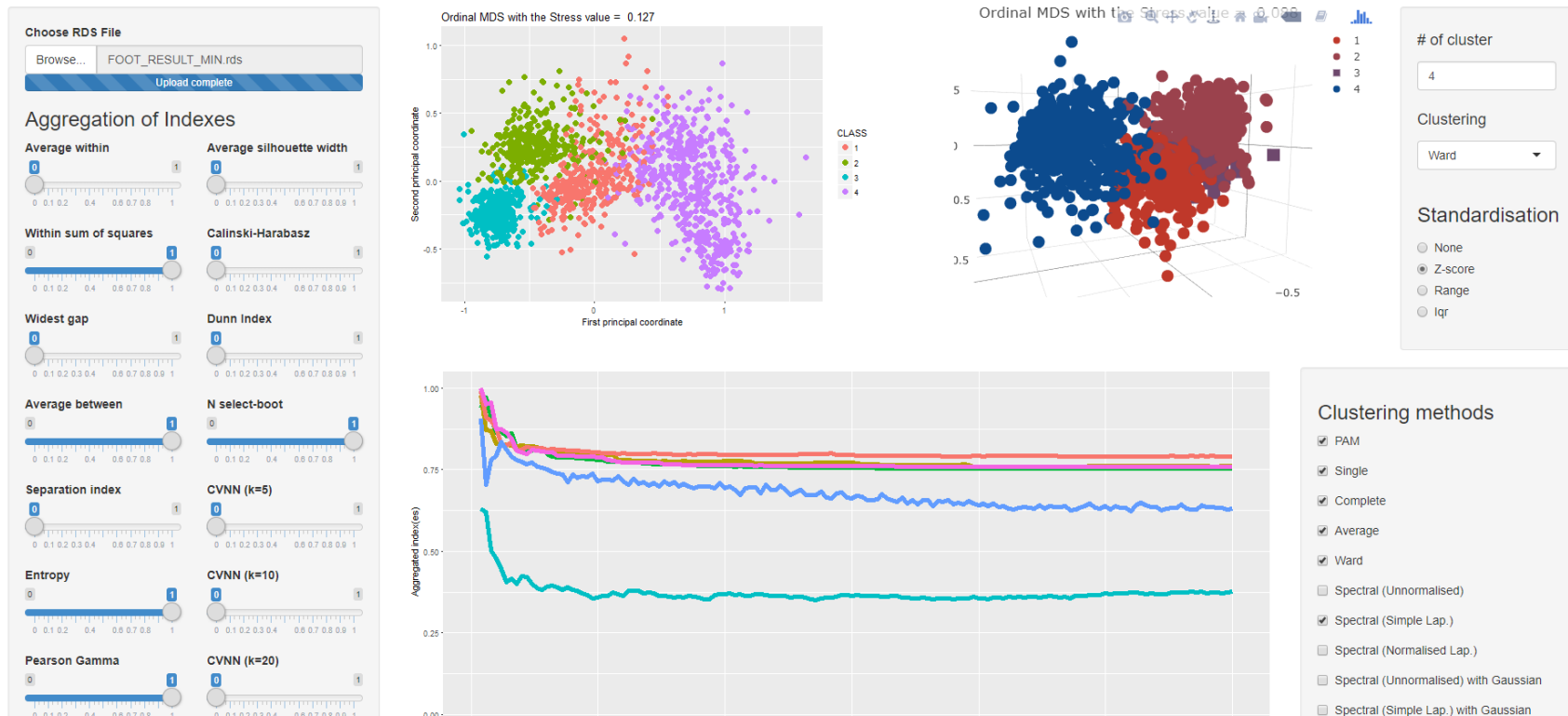
Figure B.3: R Shiny implementation for aggregation of clustering quality indexes on the football data sets
