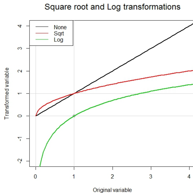
Figure 4.6: Comparison between non-linear concave transformations and no transformation
