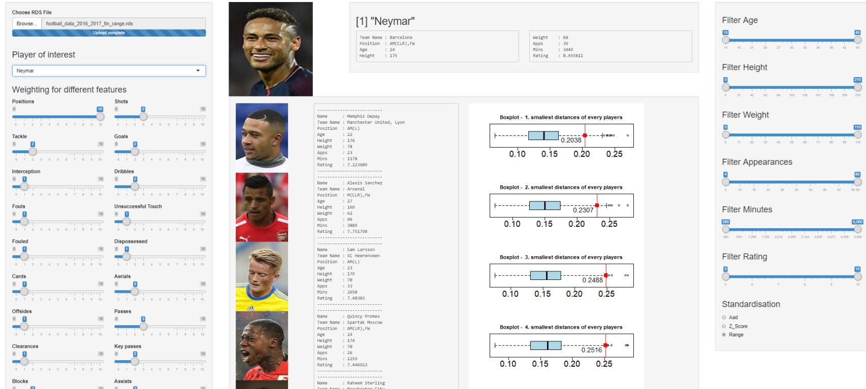
Figure 4.16: Distance query examples with the application of R Shiny - Neymar
