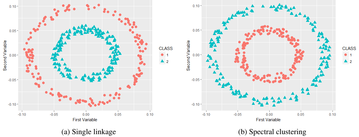
Figure 7.5: Two clusters in two dimensions with ring shapes - Two dimensional representation of a randomly selected simulated data set out of 50 replications
