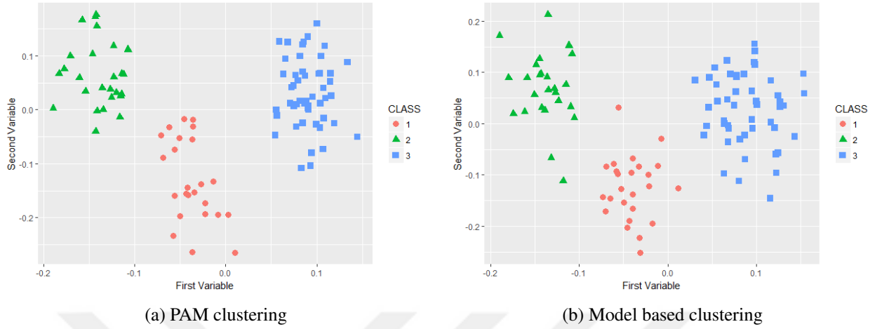
Figure 7.1: Three clusters in two dimensions - Two dimensional representation of a randomly selected simulated data set out of 50 replications
