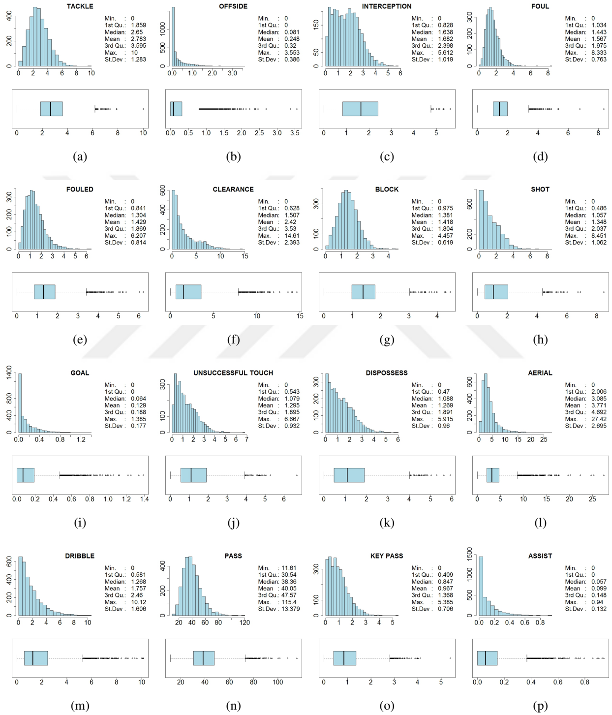
Figure 4.4: Summary of upper level count variables represented as per 90 minutes
