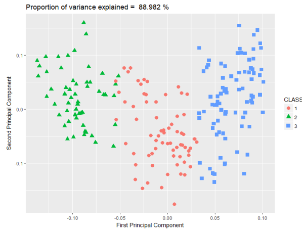
(a) Model based clustering ( K = 3 )
