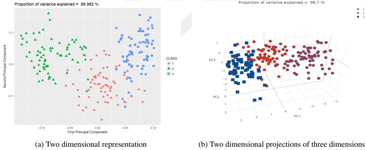
Figure 7.12: Two dimensional representation and two dimensional projections of three dimensions (PCA) of SEED data set with true class labels
