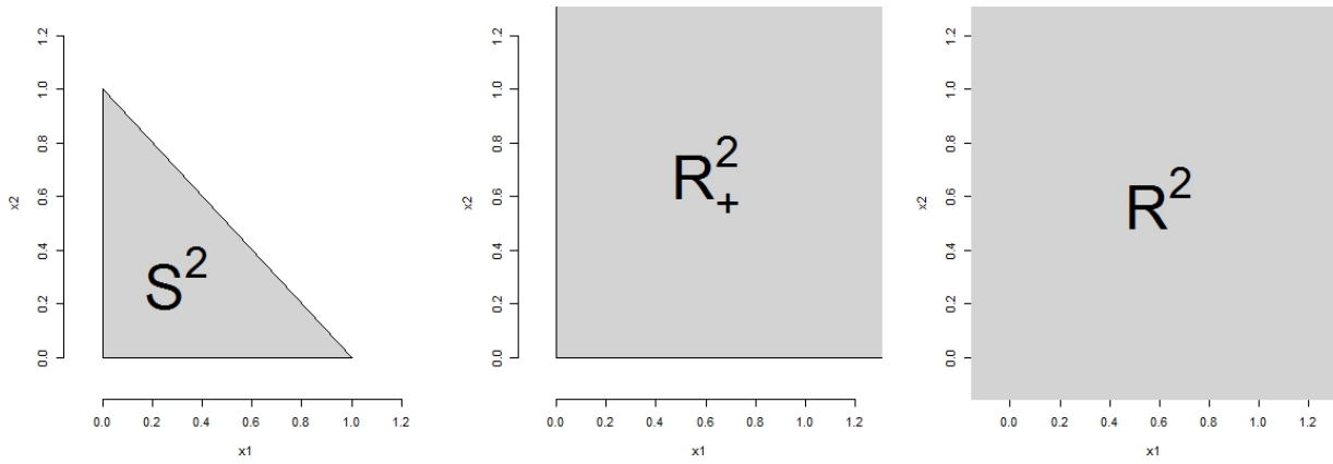
Figure 3.2: The relationship of S^2 , \mathbb{R}_+^2 and \mathbb{R}^2
