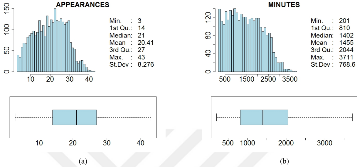
Figure 4.3: Summary of time variables
