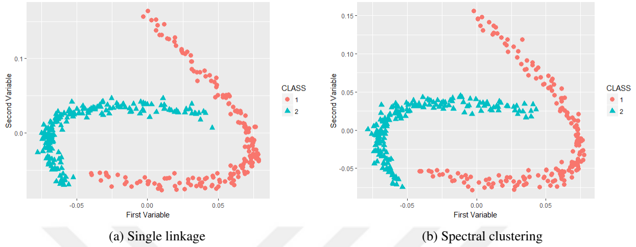
Figure 7.7: Two clusters in two dimensions with parabolic shapes - Two dimensional representation of a randomly selected simulated data set out of 50 replications
