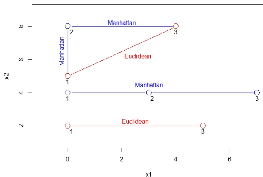
Figure 3.1: Euclidean (red) and Manhattan/city block distances (blue).
