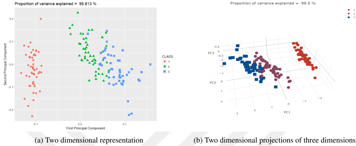
Figure 7.8: Two dimensional representation and two dimensional projections of three dimensions (PCA) of IRIS data set with true class labels
