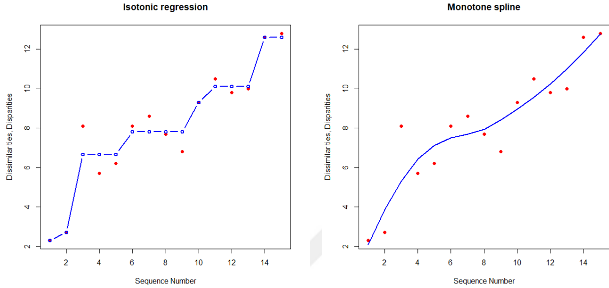
Figure A.1: Diagrams for the artificial example
