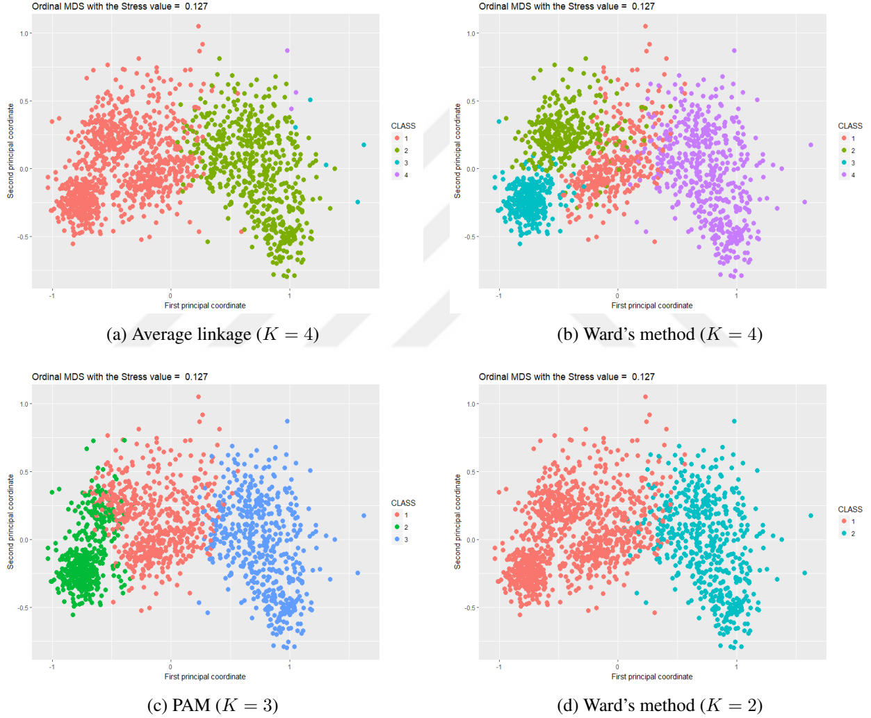
Figure 8.3: Two dimensional representation (MDS) of FOOTBALL data set for different clusterings
