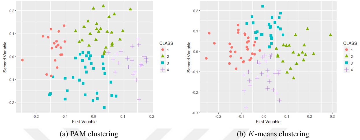
Figure 7.3: Four clusters in two dimensions that are not well separated - Two dimensional representation of a randomly selected simulated data set out of 50 replications
