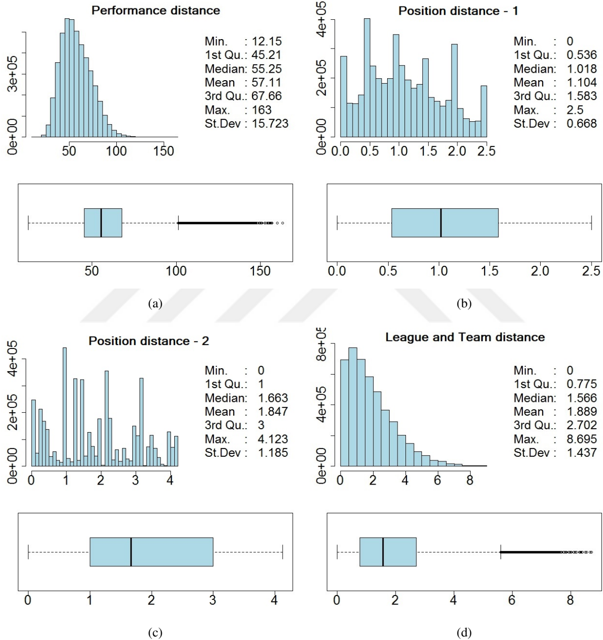
Figure 4.13: Summary of the distances
