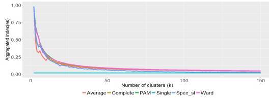
(a) CH Index K \sim [2 : 150]
