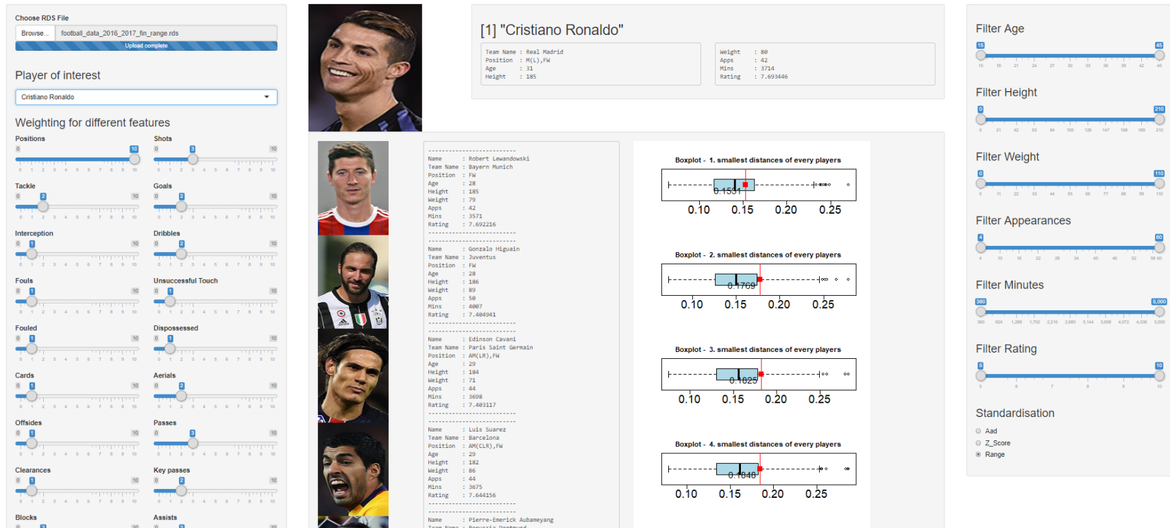
Figure 4.15: Distance query examples with the application of R Shiny - Cristiano Ronaldo
