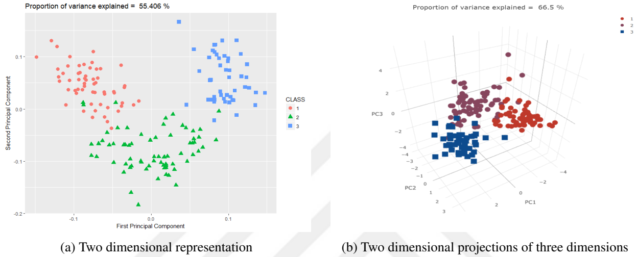
Figure 7.10: Two dimensional representation and two dimensional projections of three dimensions (PCA) of WINE data set with true class labels
