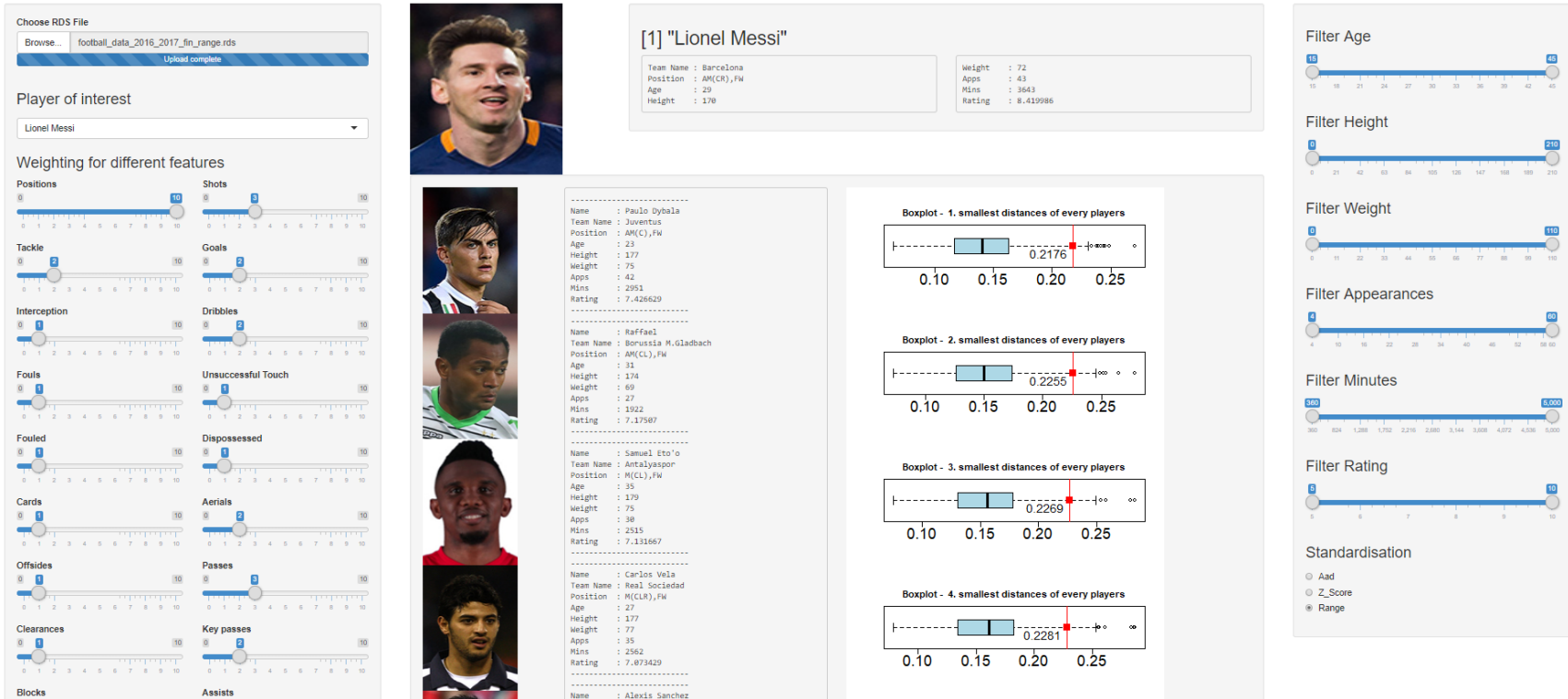
Figure 4.14: Distance query examples with the application of R Shiny - Lionel Messi
