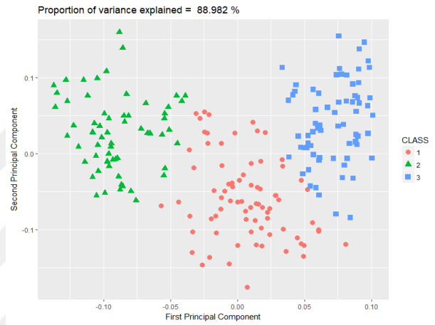
(b) PAM ( K = 3 )
