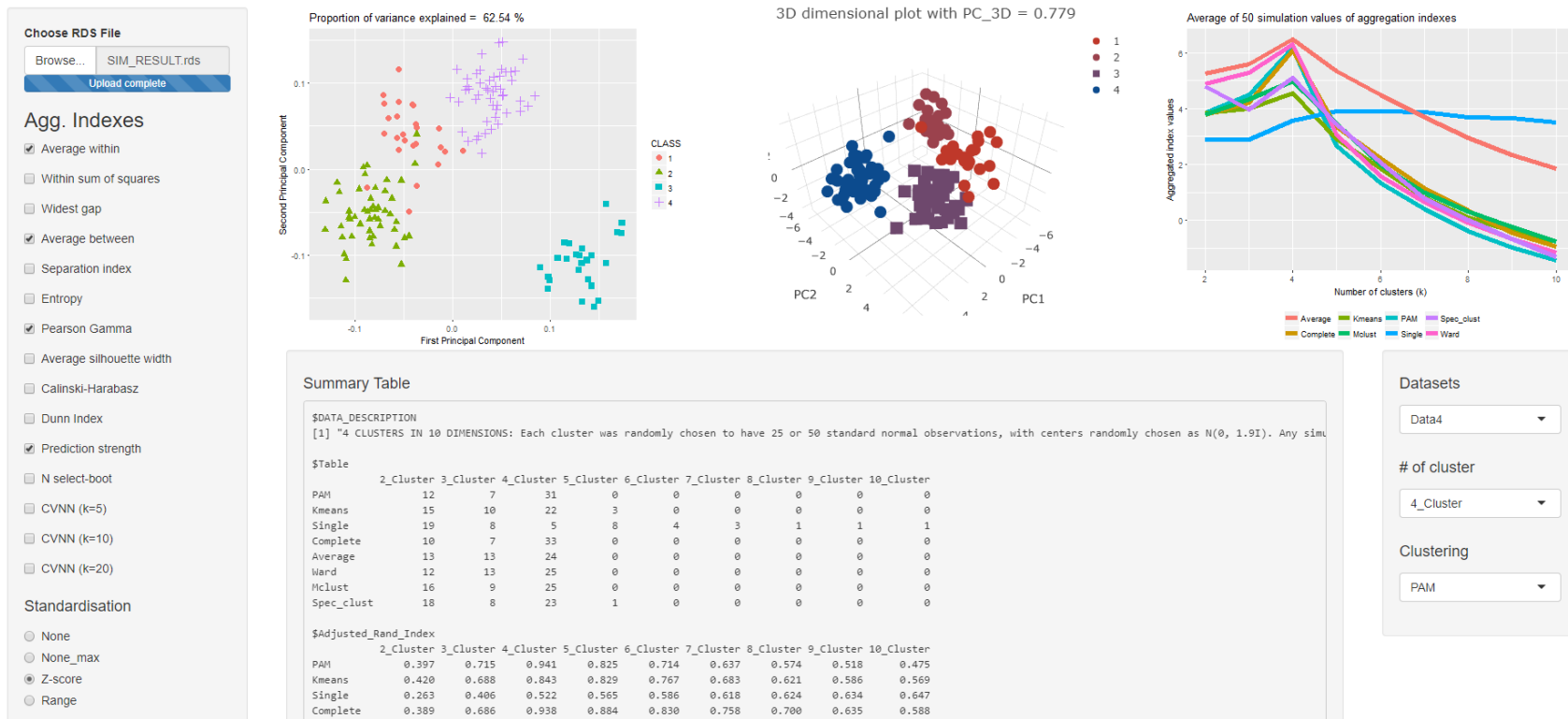
Figure B.1: R Shiny implementation for aggregation of clustering quality indexes on the simulated data set
