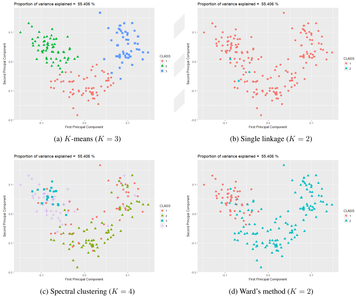
Figure 7.11: Two dimensional representation (PCA) of WINE data set for different clustering scenarios
