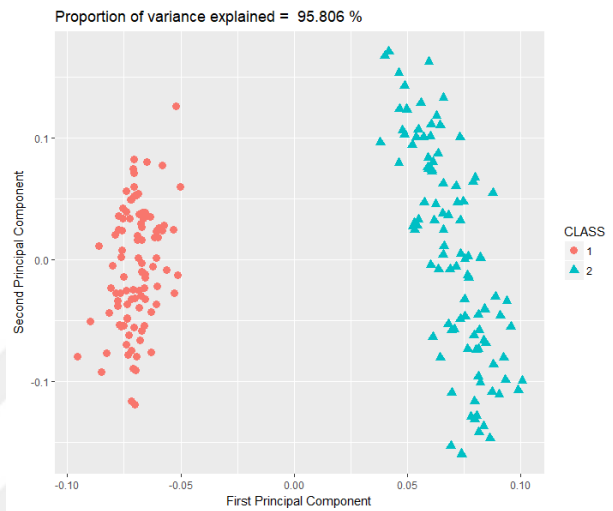
(b) Average linkage - Two dimensional representation
