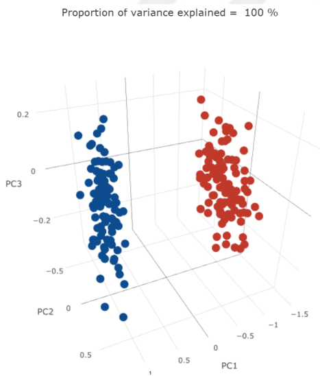
(c) Complete linkage - Two dimensional projections of three dimensions
