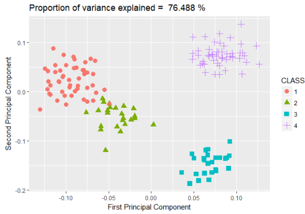
(a) PAM clustering - Two dimensional representation
