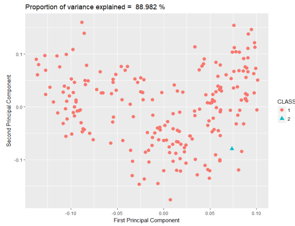
(c) Single linkage ( K = 2 )
