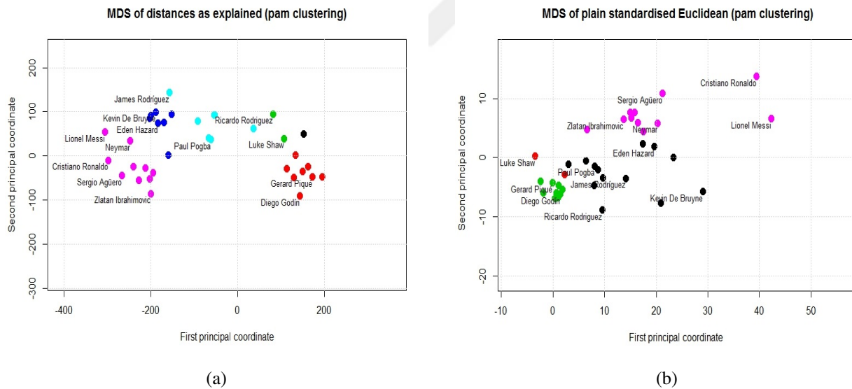
Figure 4.17: MDS and PAM clustering ( K = 6 ) for test subset of players based on all variables.
