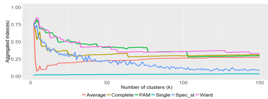
(i) CVNN ( \kappa = 10 ) Index K \sim [2 : 150]
