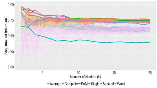
(b) Z - score: AW+(0.5)AB+Ent+PG+NSB K \sim [2 : 20]
