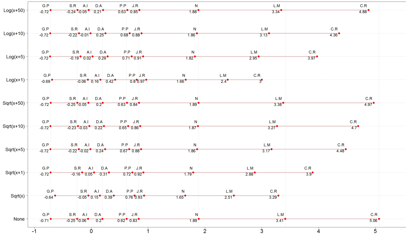
Figure 4.7: Comparison of transformations with different constants
