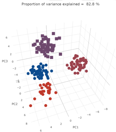
(c) PAM clustering - Two dimensional projections of three dimensions
