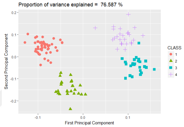
(b) Model based clustering - Two dimensional representation
