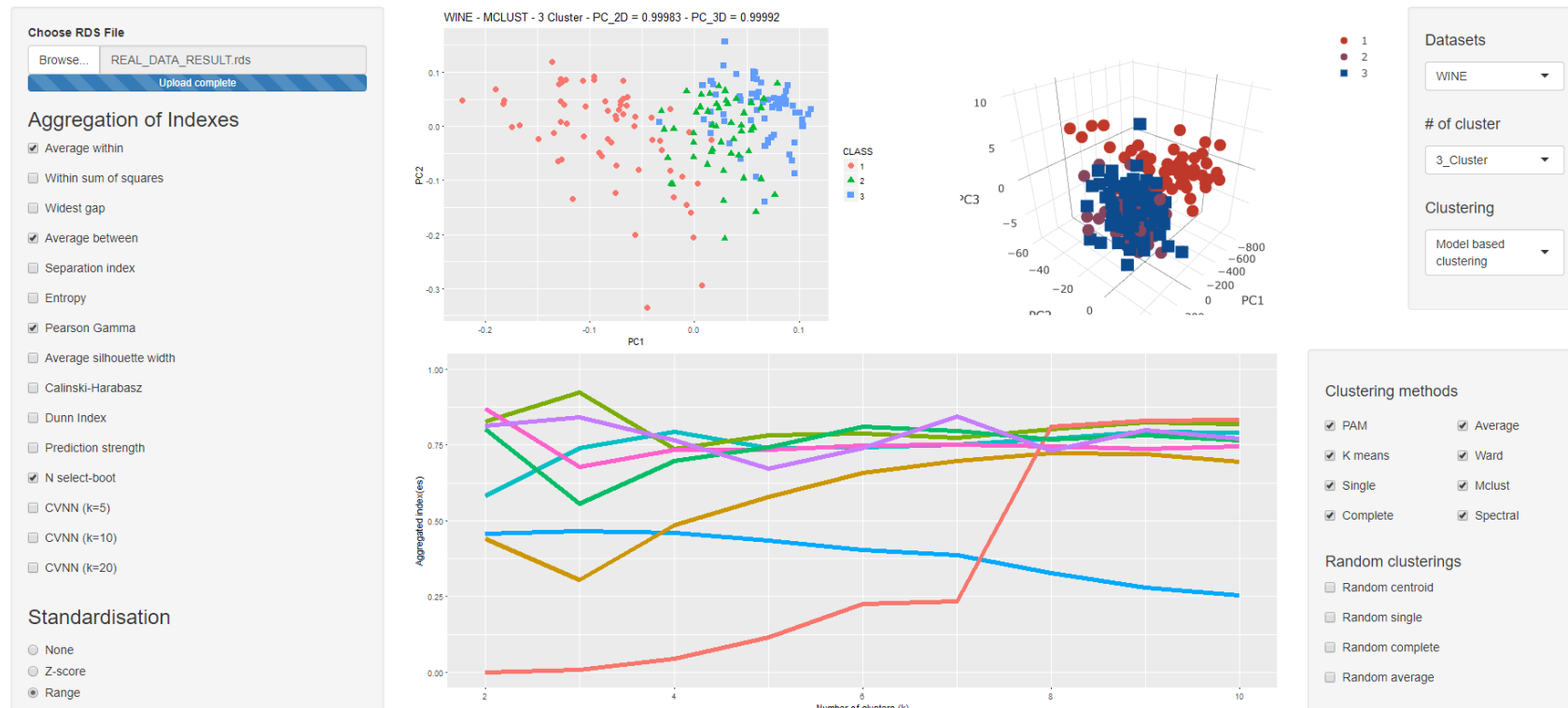
Figure B.2: R Shiny implementation for aggregation of clustering quality indexes on the real data sets
