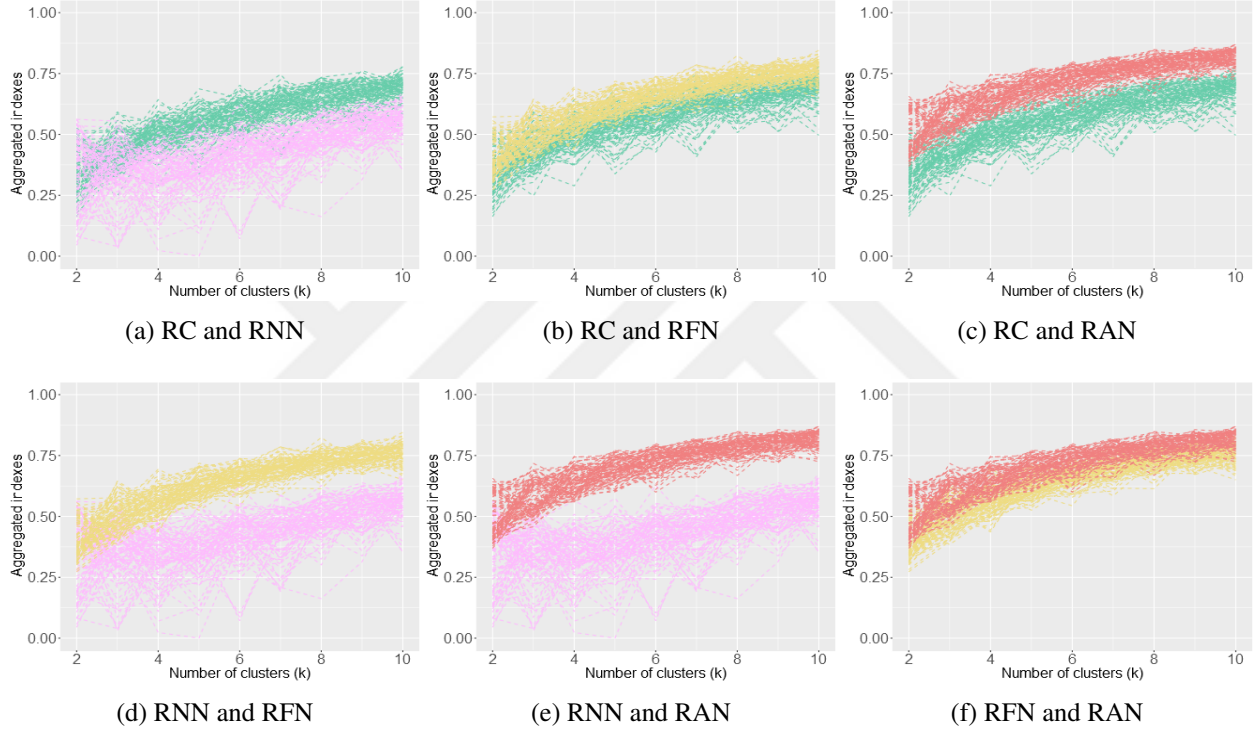
Figure 7.23: Clustering validation index results for different random clustering algorithms scenarios of MOVEMENT data set. The index results are based on the aggregated indexes of average within and between dissimilarities, Pearson Gamma Index and the bootstrap method
