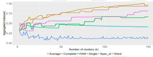
(e) Dunn Index K \sim [2 : 150]
