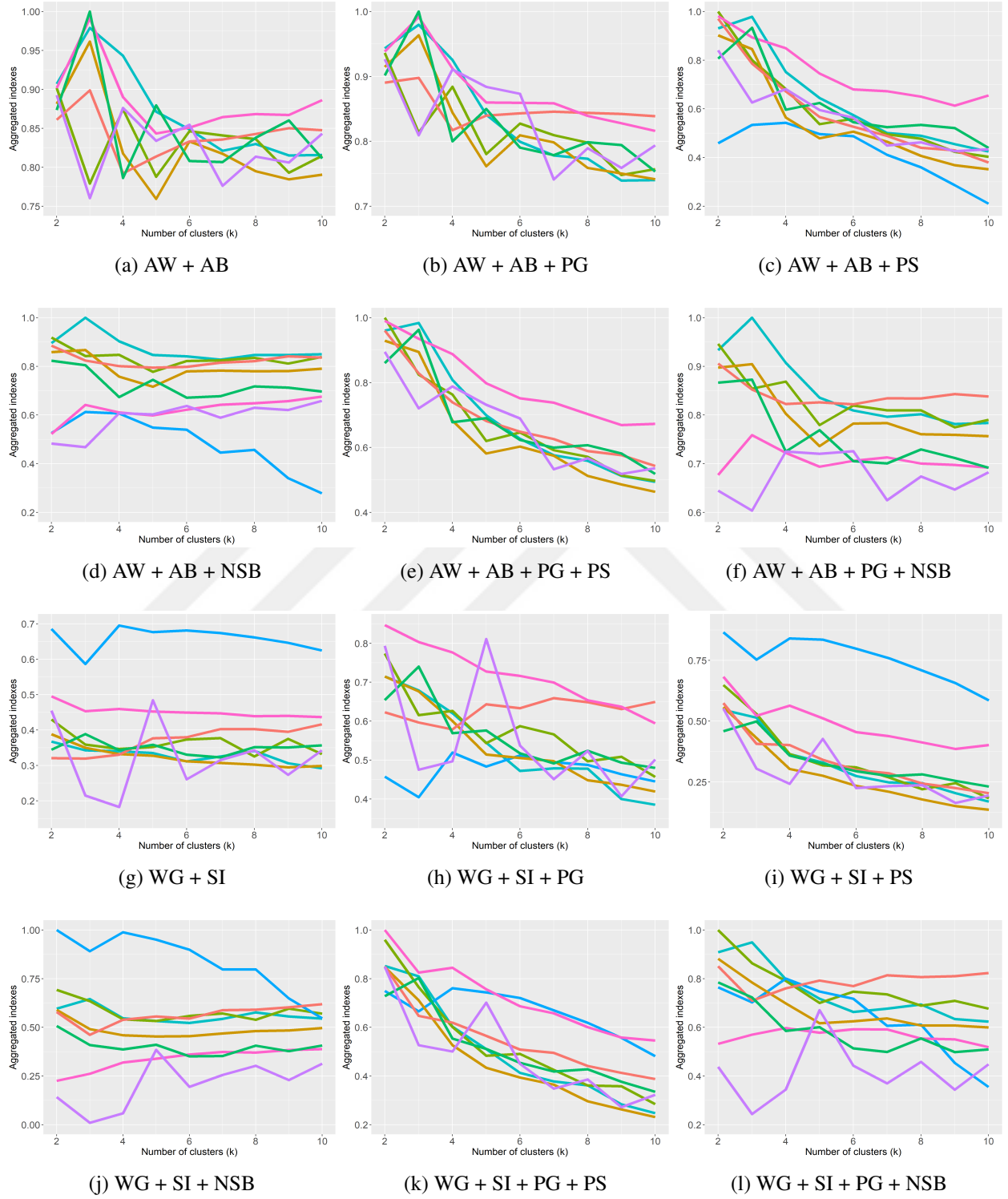
Figure 7.22: Different aggregated index considerations with Range standardisation for SEED data set.
