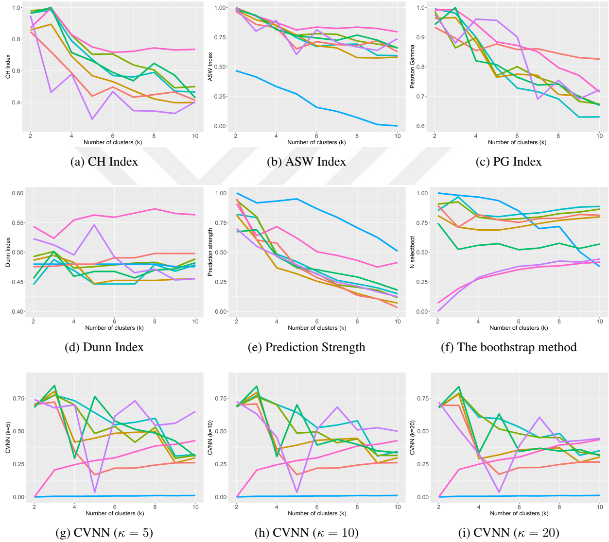
Figure 7.20: Various single criteria for SEED data set.
