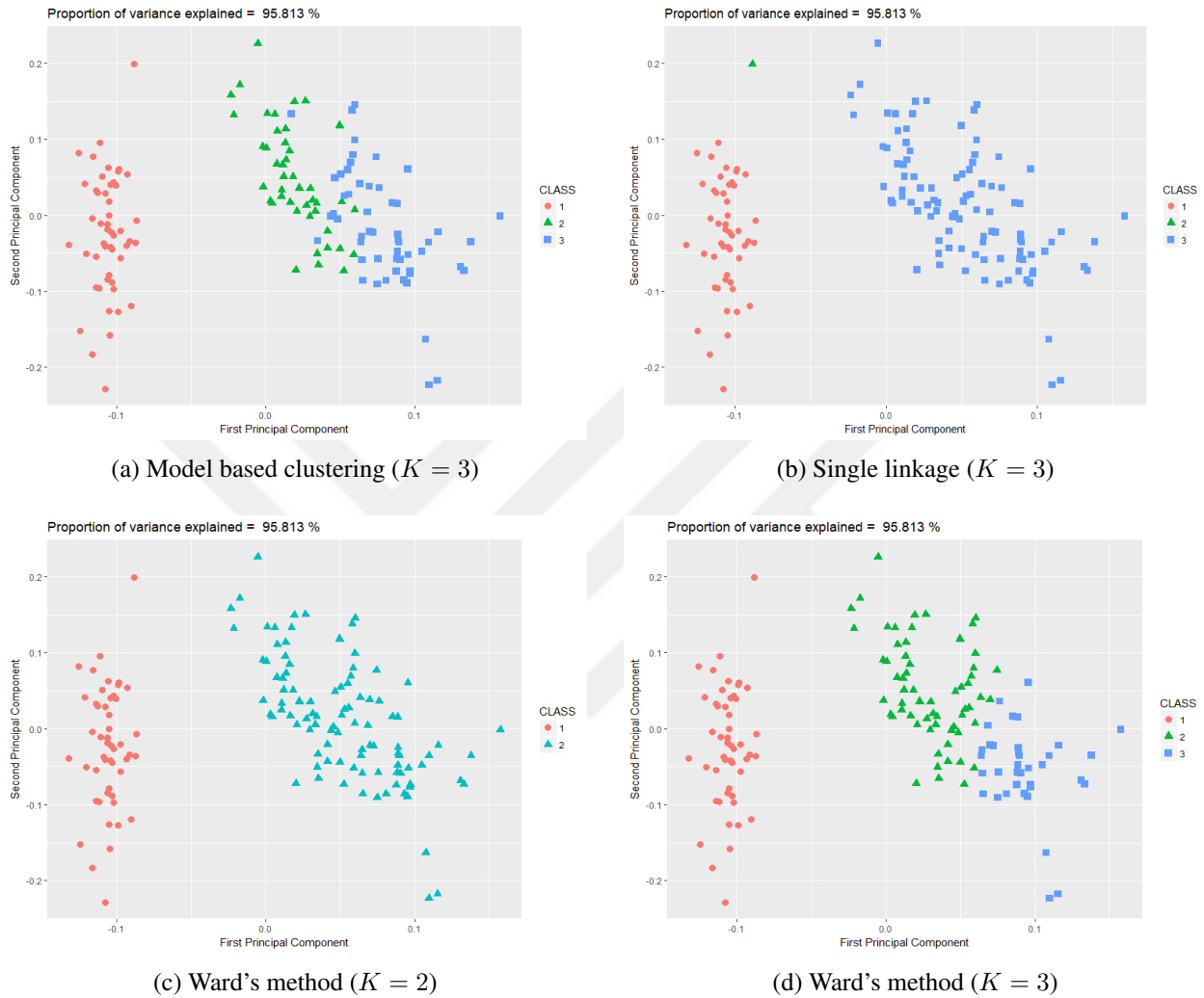
Figure 7.9: Two dimensional representation (PCA) of IRIS data set for different clustering scenarios
