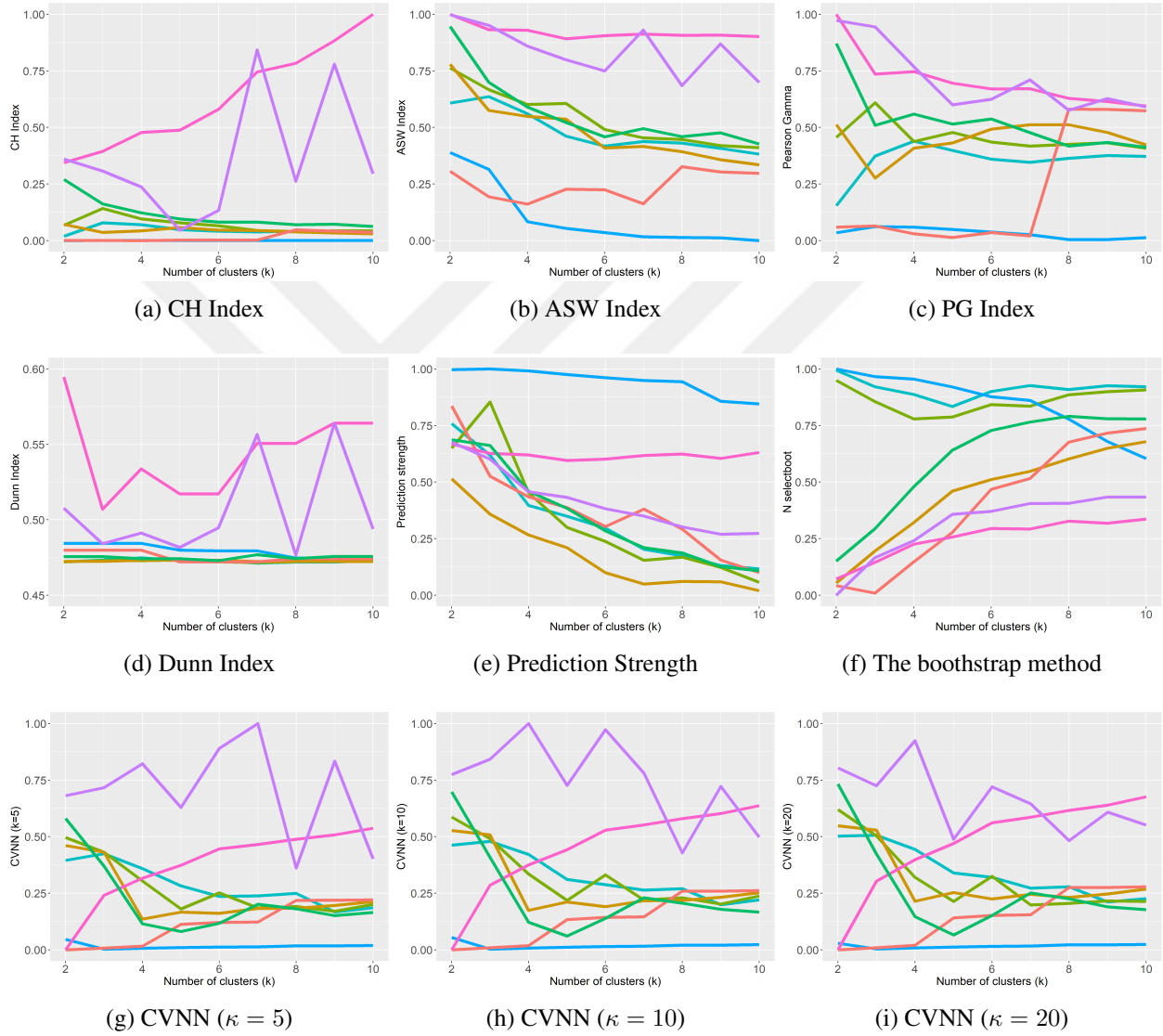
Figure 7.17: Various single criteria for WINE data set.
