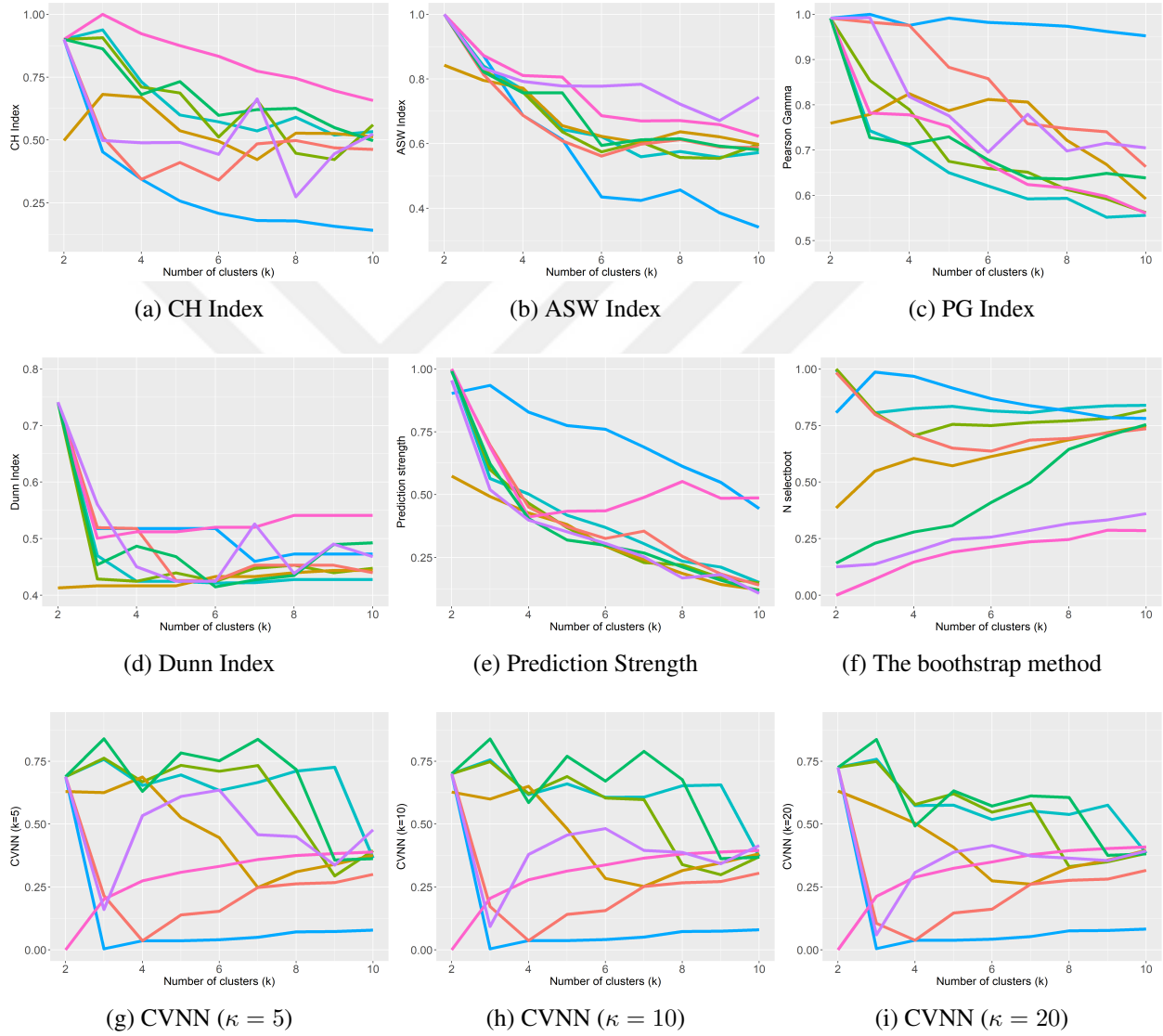
Figure 7.14: Various single criteria for IRIS data set.
