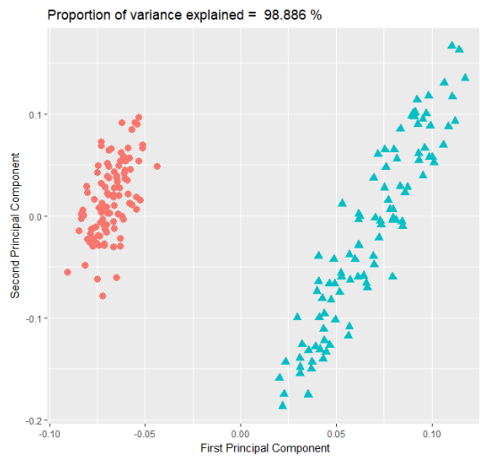
(a) Complete linkage - Two dimensional representation
