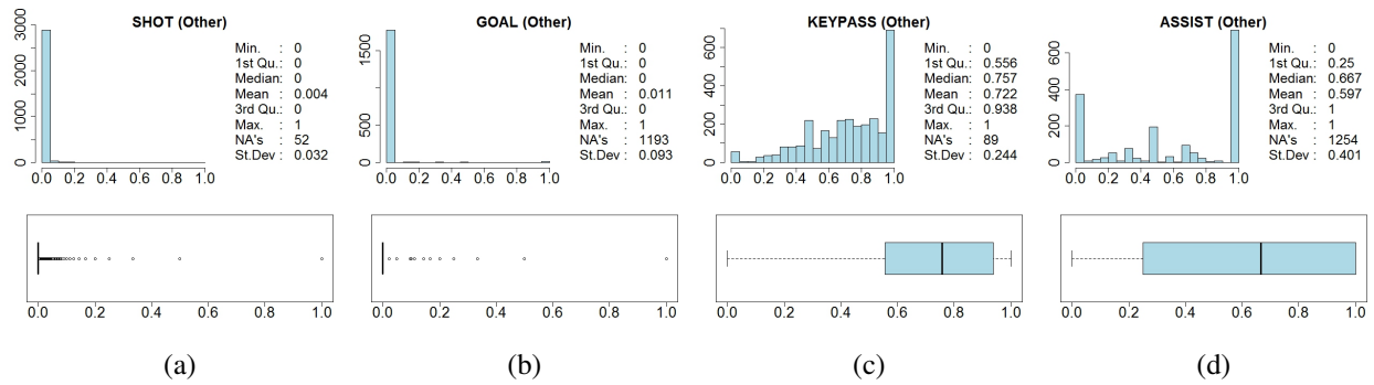
Figure 4.5: Summary of the 'Other' percentage variables
