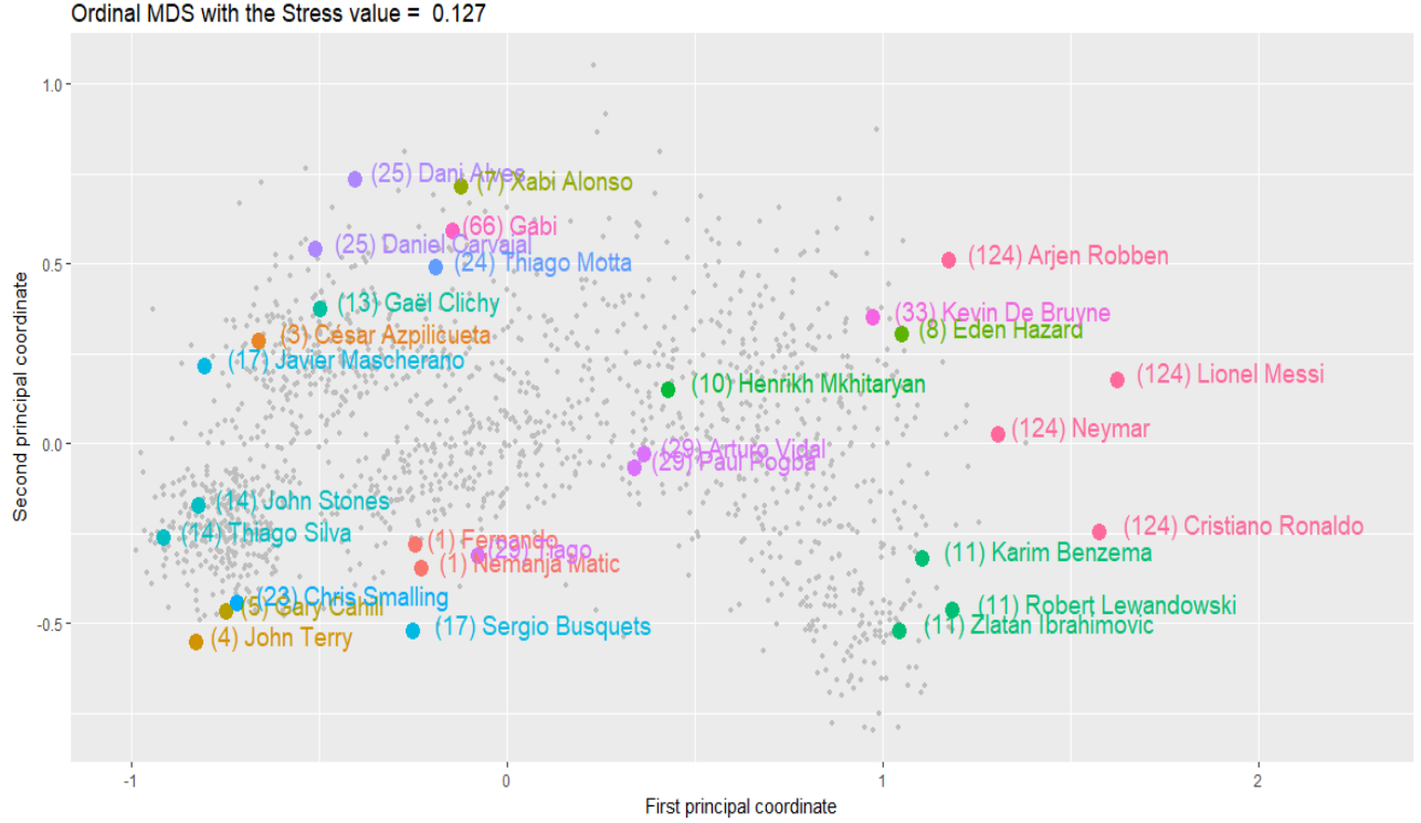
Figure 8.5: Two dimensional representation (MDS) of FOOTBALL data set with some famous players. Small gray points represent other players location on this MDS scatter plot. Although there are 146 cluster solutions, 18 cluster solutions are shown only for the famous players. The numbers in parenthesis with player's name represent the cluster number of that player to avoid confusion in case of the similarity between colors.
