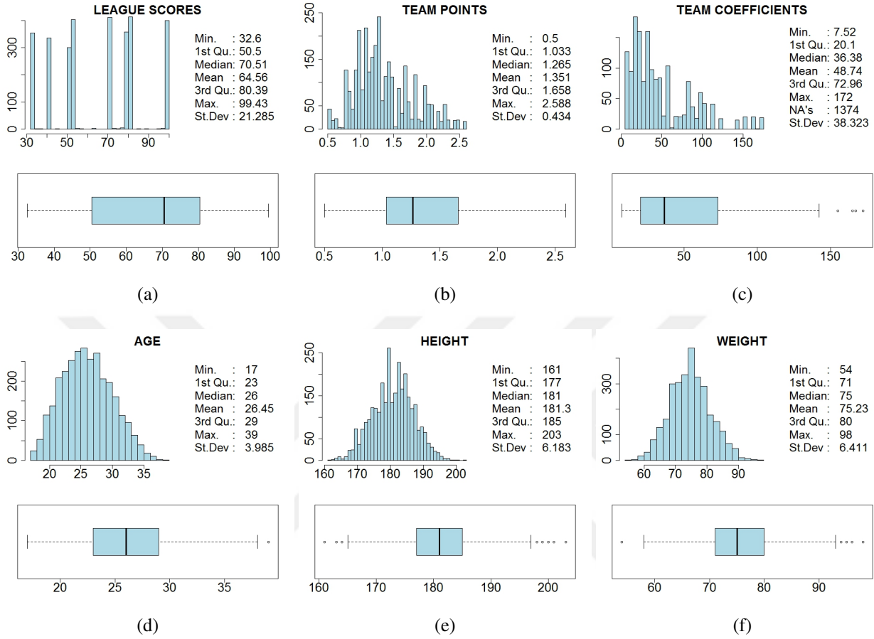
Figure 4.1: Summary of profile variables
