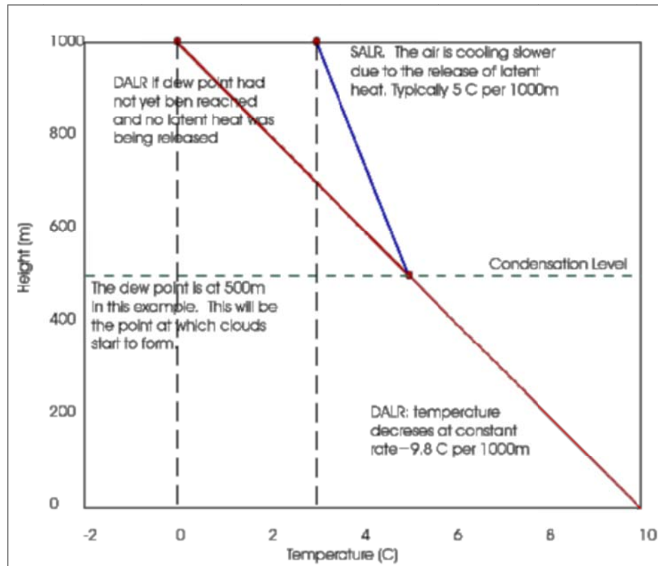
Figure 2.26. Temperature variations of DALR and SALR methods (assumed condensation level is 500m)
