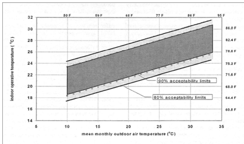
Figure 2.2. Required operative temperature ranges for naturally ventilated spaces (ASHRAE Standard 55, 2010)
