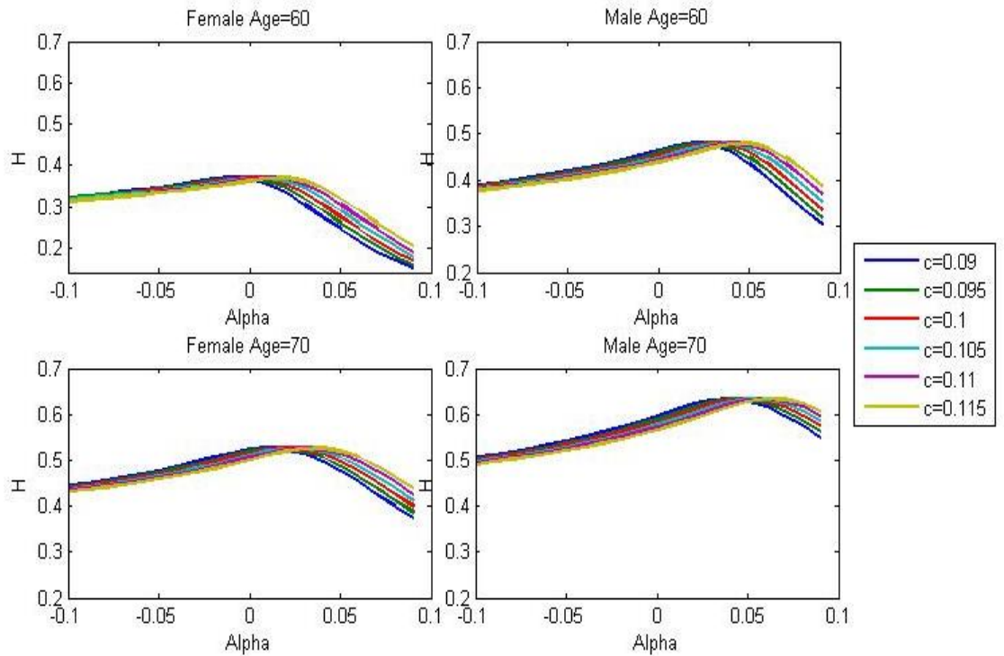
Fig. 4.6. H values for Females and Males at ages 60 and 70 in base year 2015 with different c values and \delta = 0\% .
