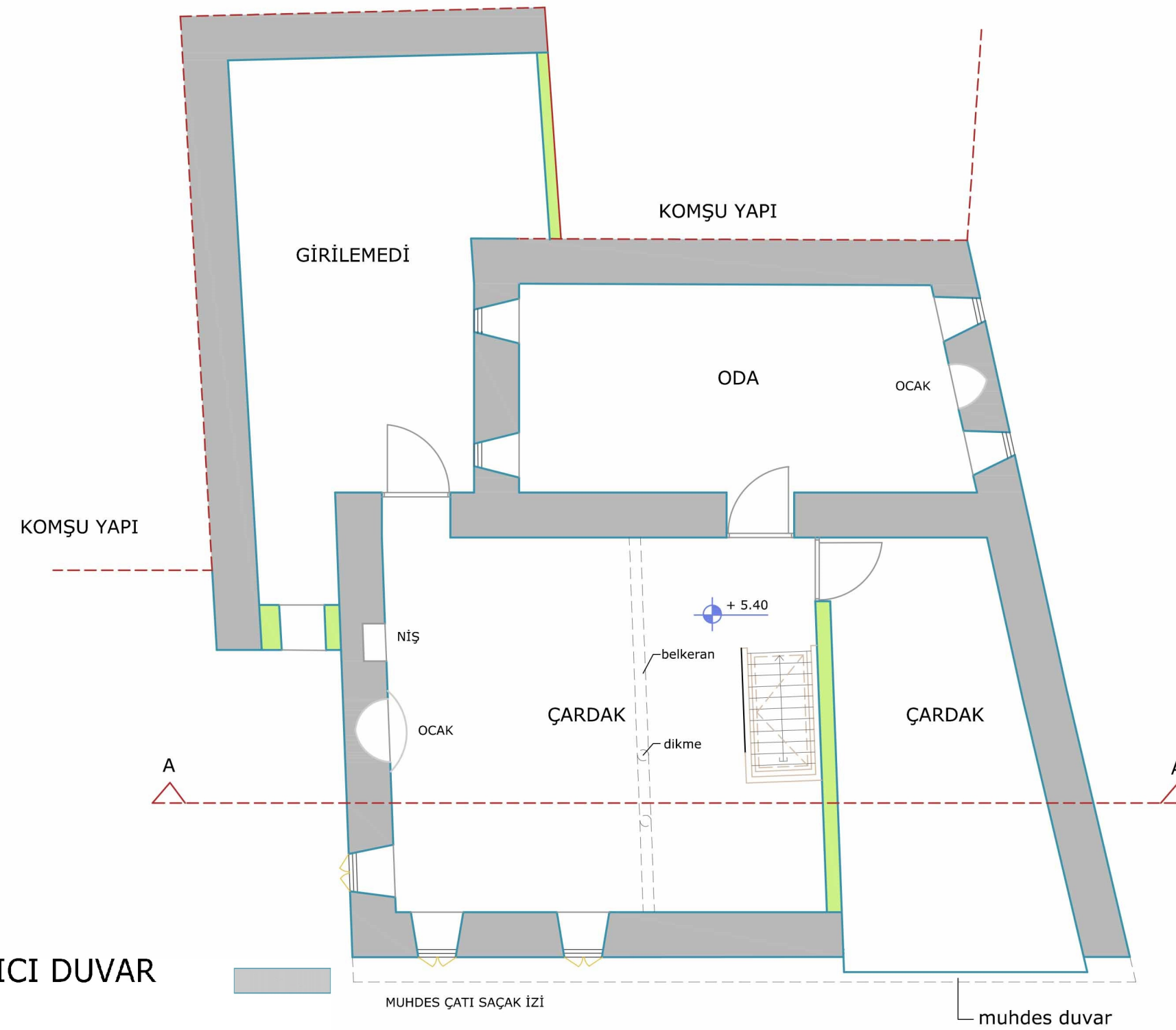
2. KAT PLANI
