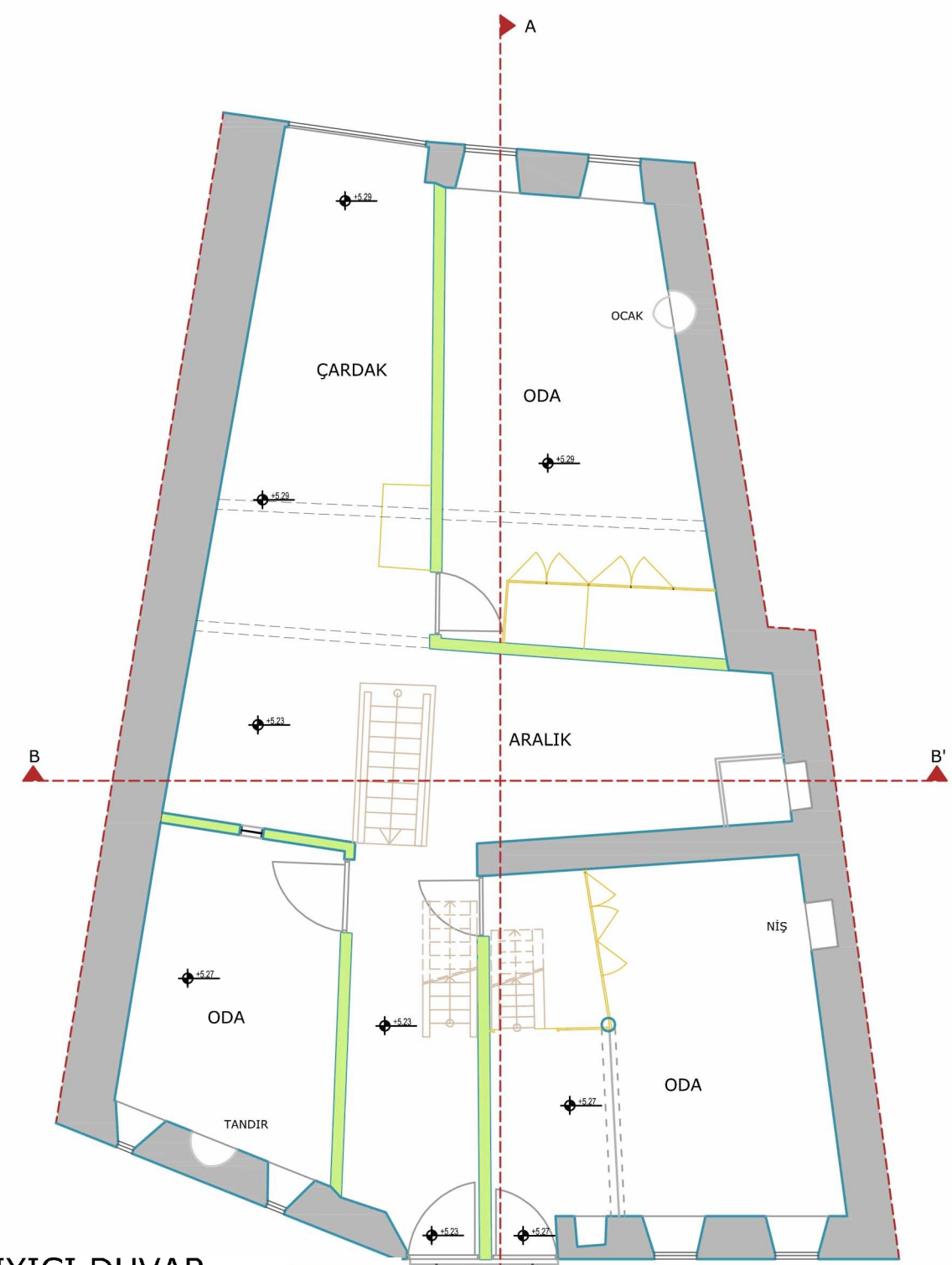
2. KAT PLANI
