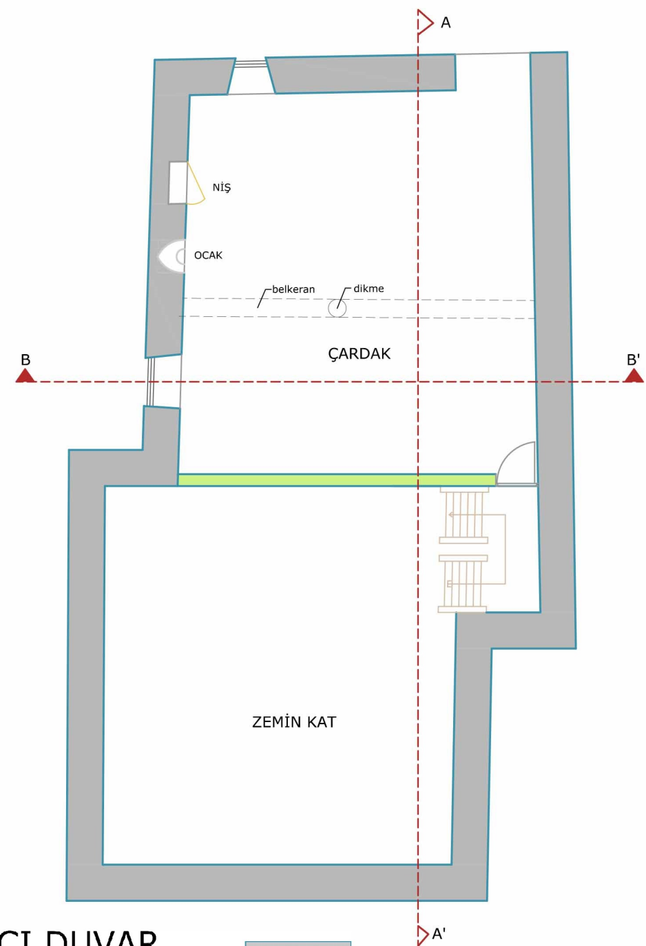
2. KAT PLANI
