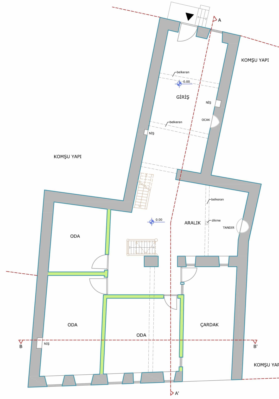
2. KAT PLANI
