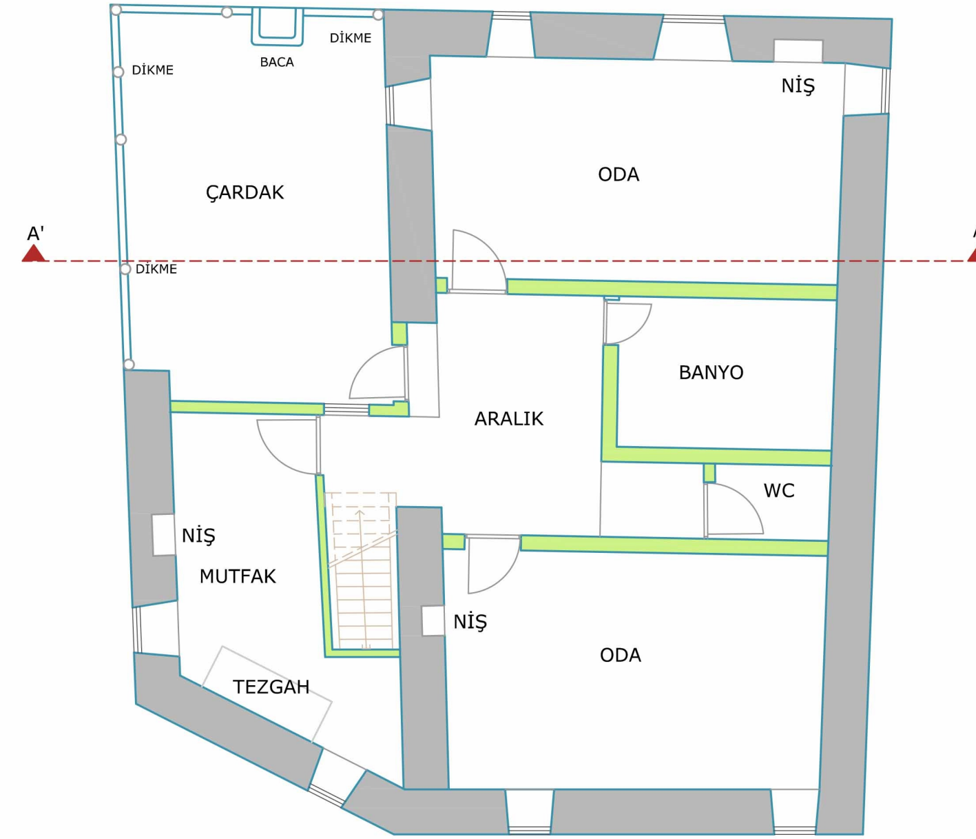
2. KAT PLANI
