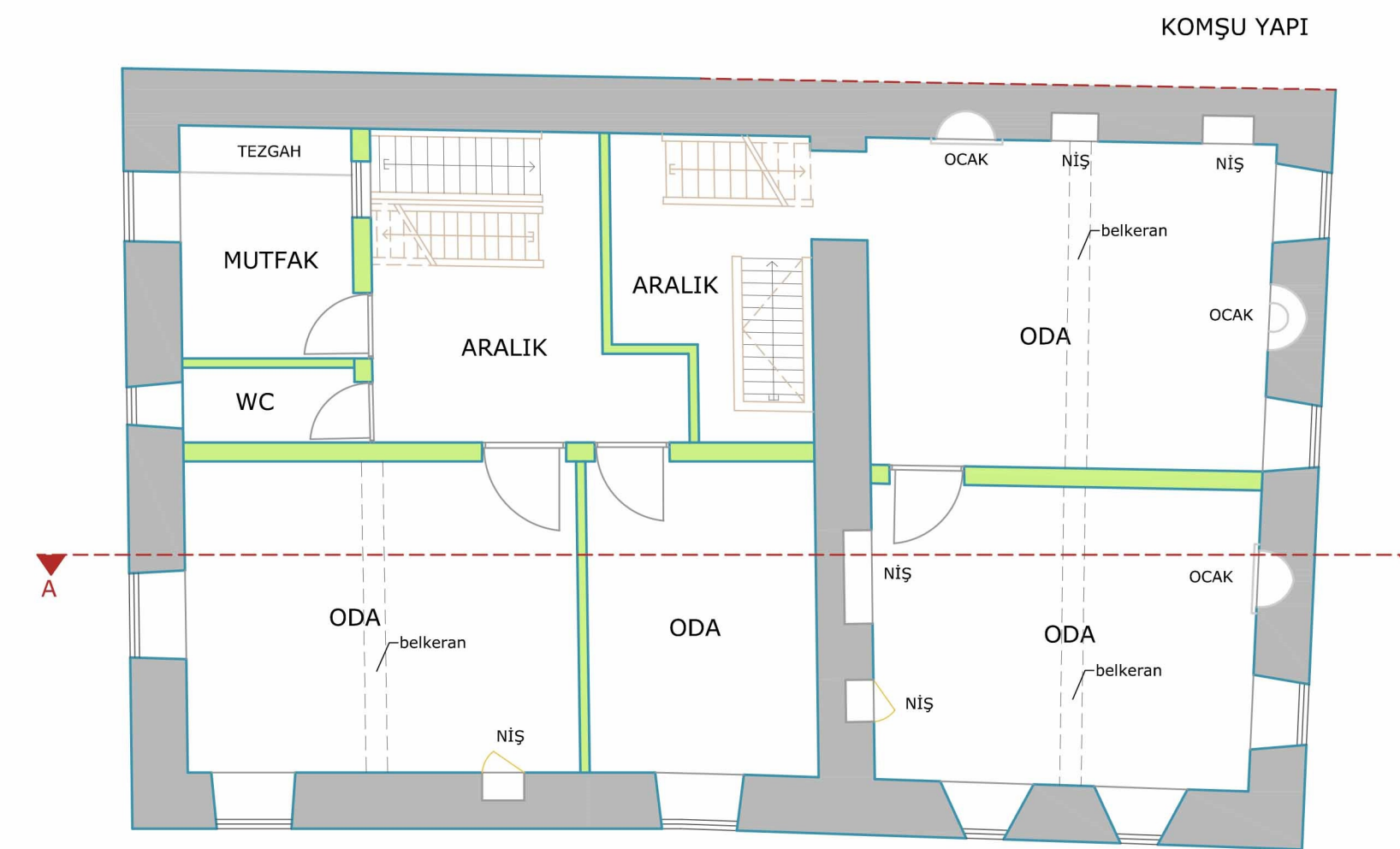
2. KAT PLANI
