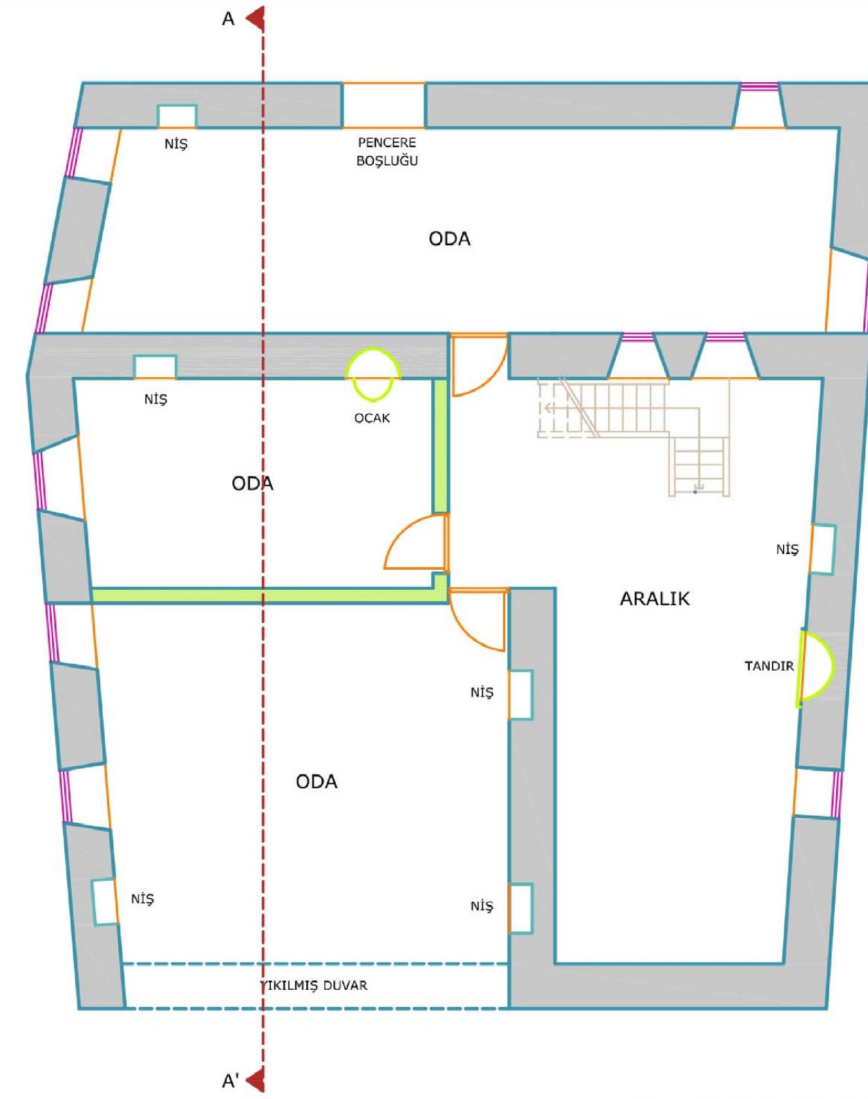
2. KAT PLANI
