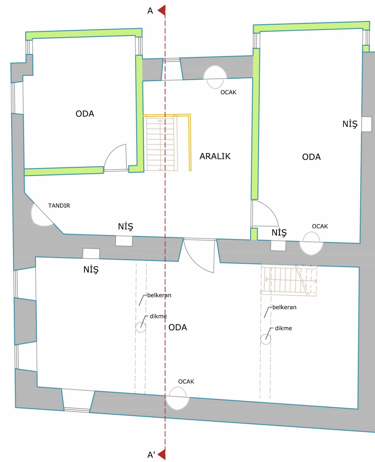
2. KAT PLANI
