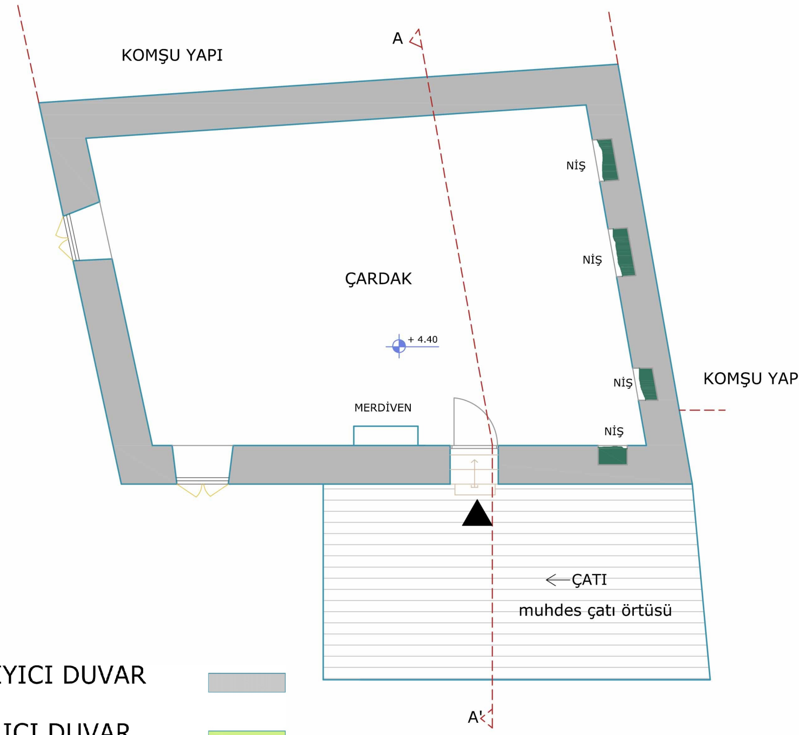
2. KAT PLANI
