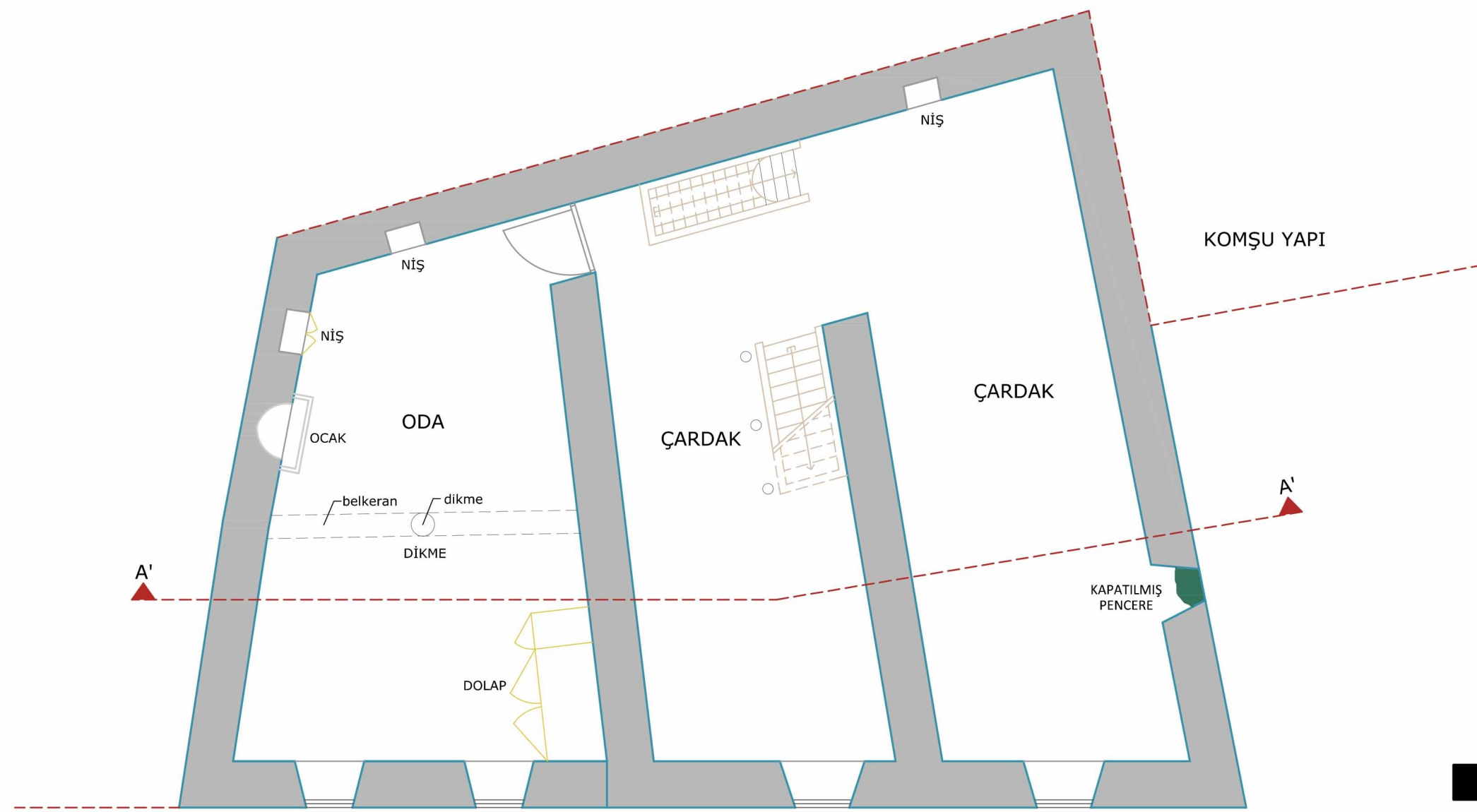
2. KAT PLANI
