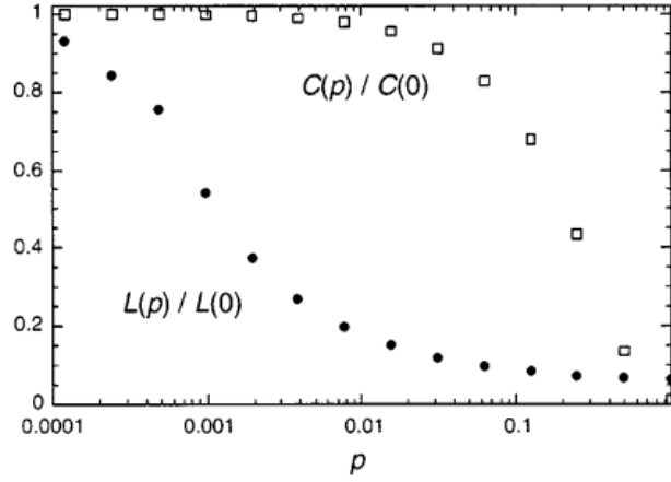
Figure 4 Watts-Strogatz Model
