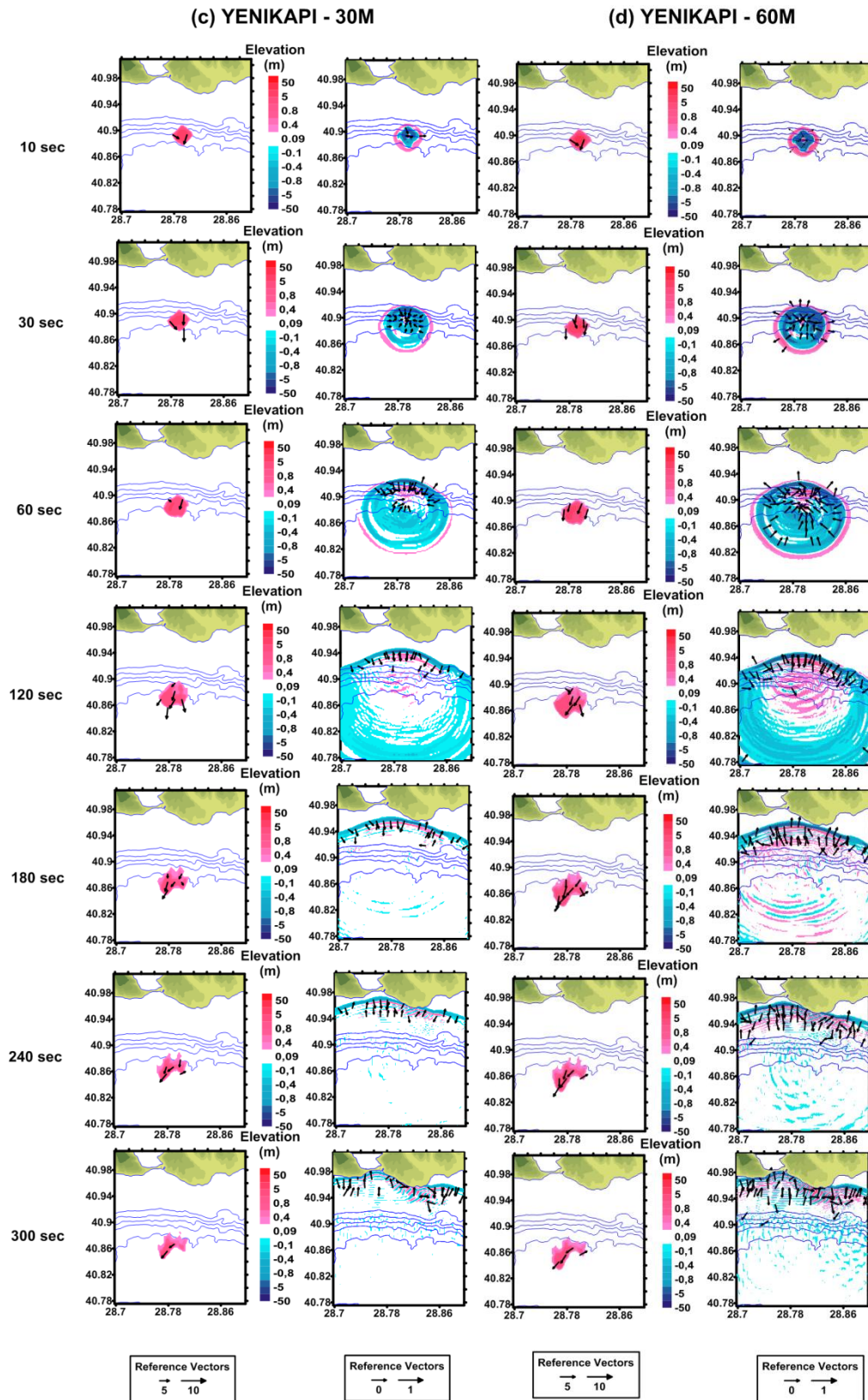
Figure 6.20. The view of the sea bottom material and corresponding water surface elevation at different time steps due to 30 m (c) and 60 m (d) sediment thicknesses of submarine landslide at Yenikapi.
