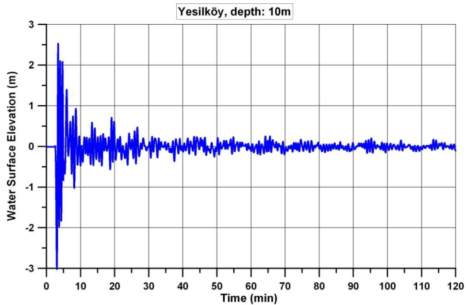
Figure 6.12. The time histories of water surface fluctuations computed at selected gauge point (Yeşilköy) for the simulation due to landslide of 60 m submarine sediment thickness at offshore of Yenikapı.
