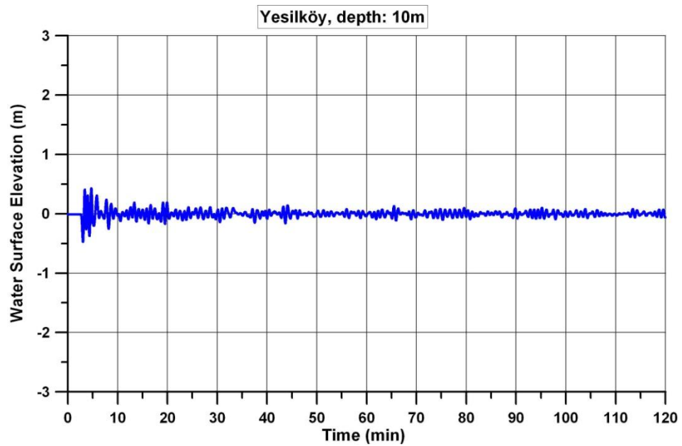
Figure 6.10. The time histories of water surface fluctuations computed at selected gauge point (Yeşilköy) for the simulation due to landslide of 10 m submarine sediment thickness at offshore of Yenikapı.
