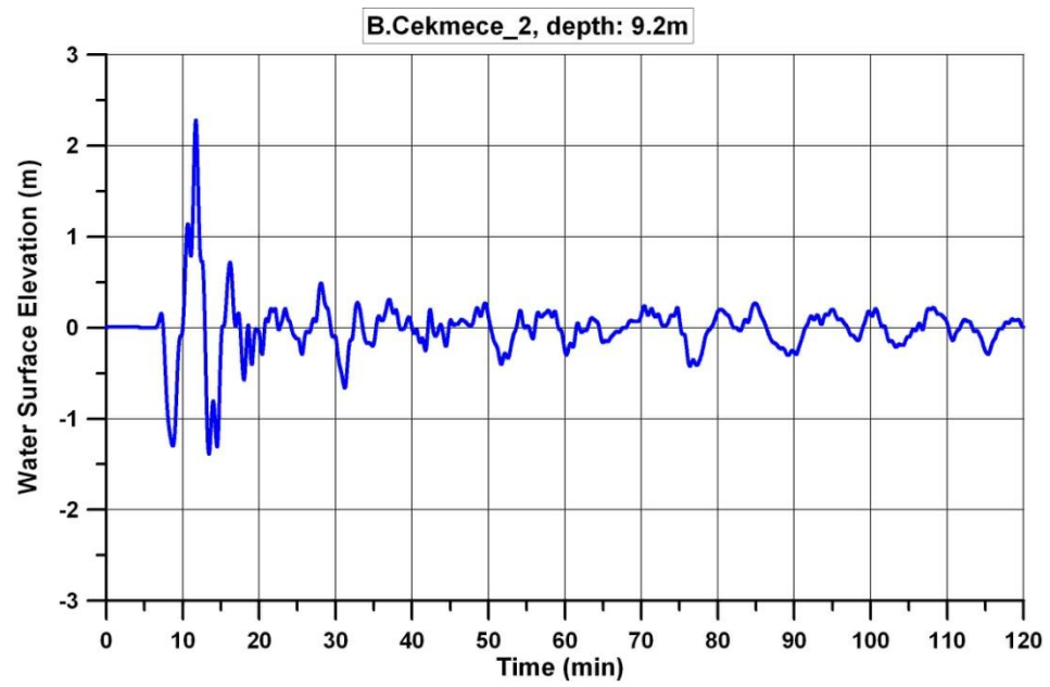
Figure 6.72. The time histories water surface fluctuations computed at selected gauge Point (B. Çekmece_2) for the simulation due to landslide of 50 m submarine sediment thickness at offshore of Küçükçekmece2.
