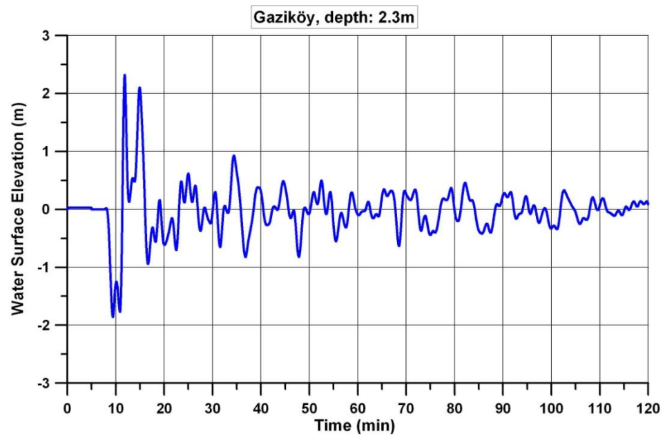
Figure 6.43. The time histories water surface fluctuations computed at selected gauge point (Gaziköy) for the simulation due to landslide of 50 m submarine sediment thickness at offshore of Ganos2.
