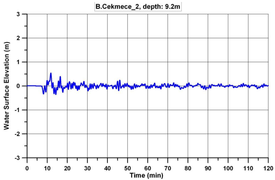
Figure 6.71. The time histories water surface fluctuations computed at selected gauge point (B. Çekmece_2) for the simulation due to landslide of 10 m submarine sediment thickness at offshore of Küçükçekmece2.
