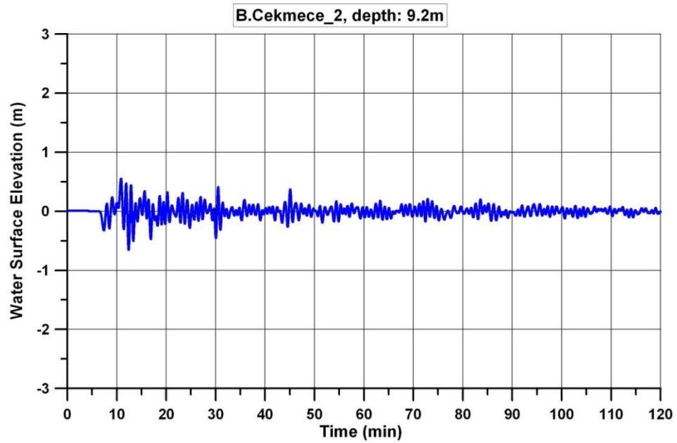
Figure 6.60. The time histories water surface fluctuations computed at selected gauge point (B. Çekmece_2) for the simulation due to landslide of 10 m submarine sediment thickness at offshore of Küçükçekmece1.
