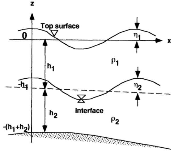
Figure 5.1. Definition sketch for Two-Layer Profile (Imamura and Imteaz, 1995).
