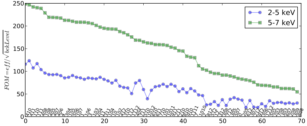
Figure C.6. The observable pairs vs. FOM for low and high energy events, for M9.
