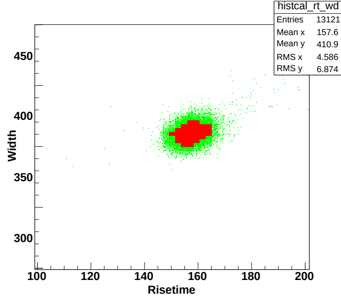
Figure 7.8. Risetime - width distribution during a single calibration run. All events are shown in green, while red region shows the selection region.
