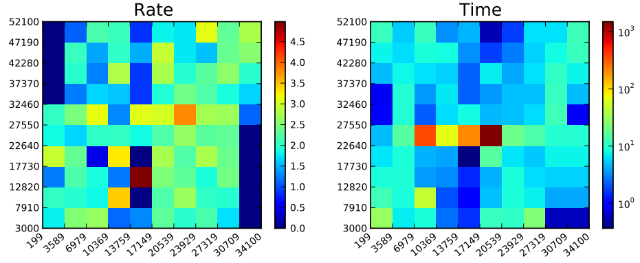
Figure C.19. Background rate in counts/hour at different magnet positions for M6.
