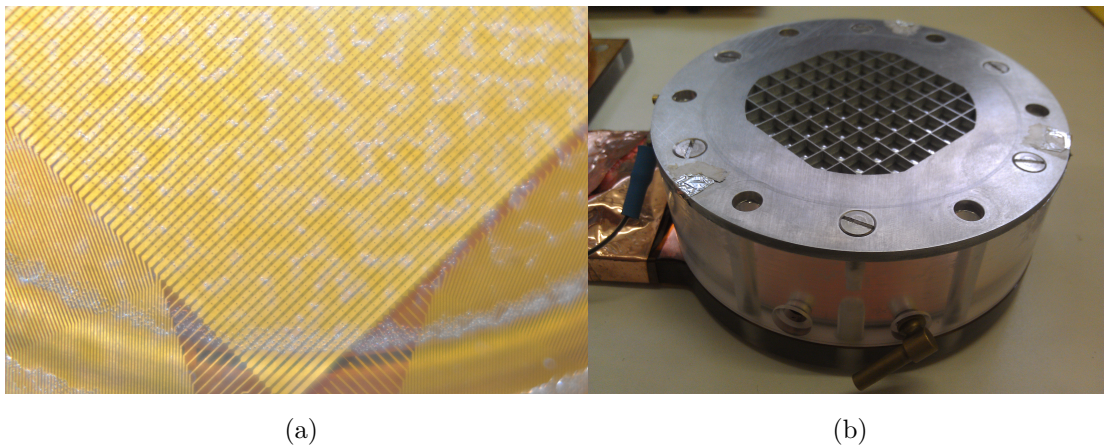
Figure 5.9. (a) Photo of the strip plane. (b) Plexiglas chamber and aluminized mylar drift window connected to micromegas detector.
