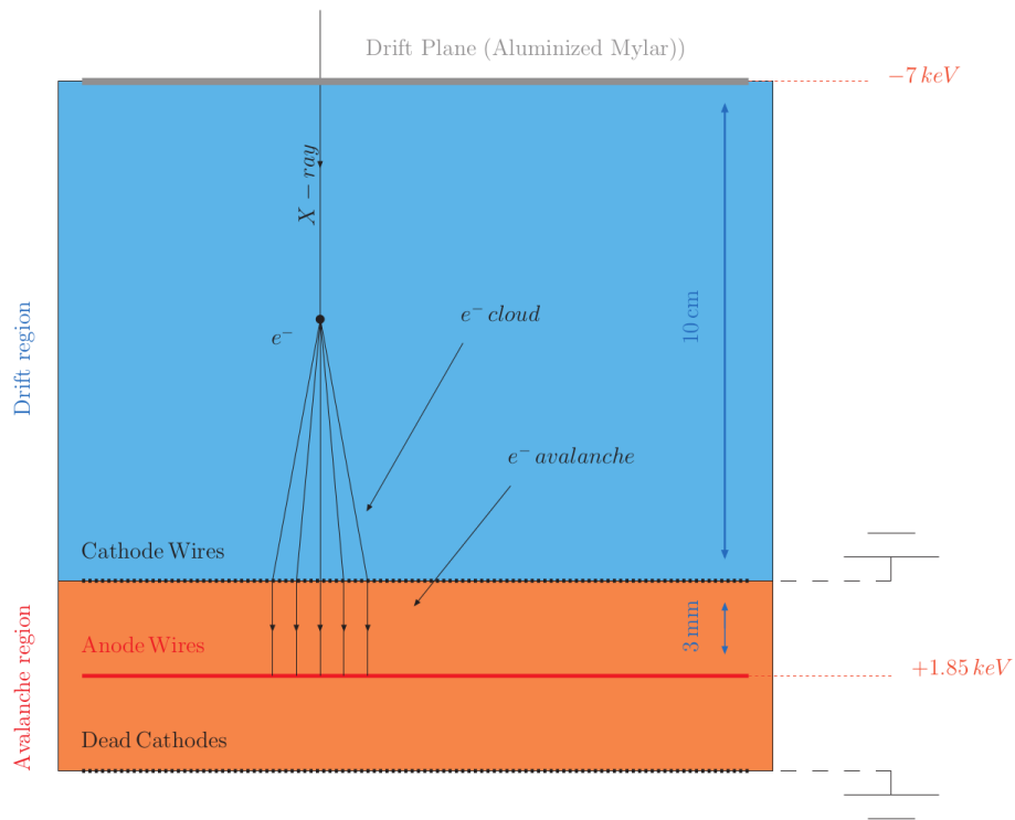
Figure 4.21. The schematics of the working principle of the CAST TPC [80].
