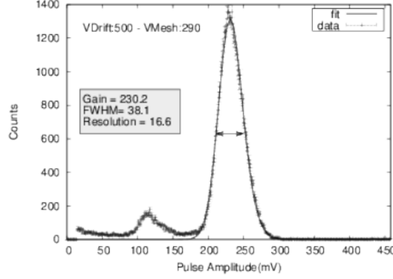
Figure 5.11. An example spectra from the characterization measurements. The ^{55}\text{Fe} peak is at channel 230, where the escape peak can be seen around channel 120.
