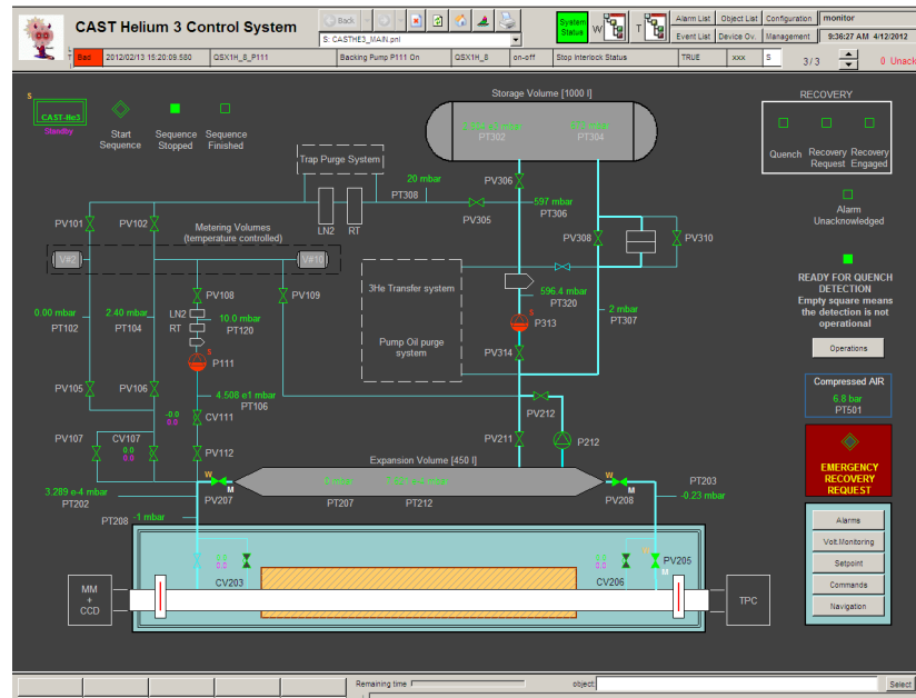
Figure 4.17. User interface of the CAST PLC System.
