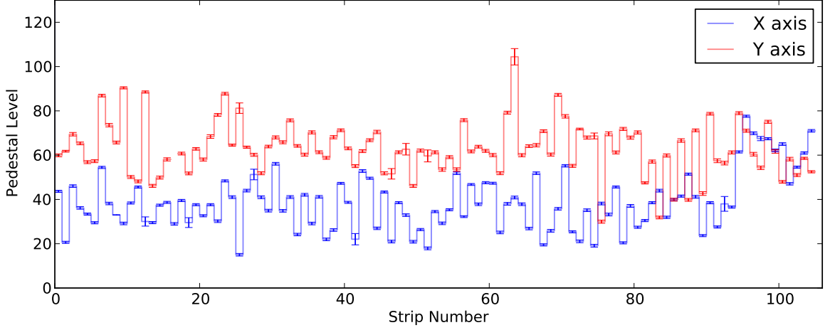
Figure 7.1. The mean and sigma of pedestals for x and y channels for M9 detector.
