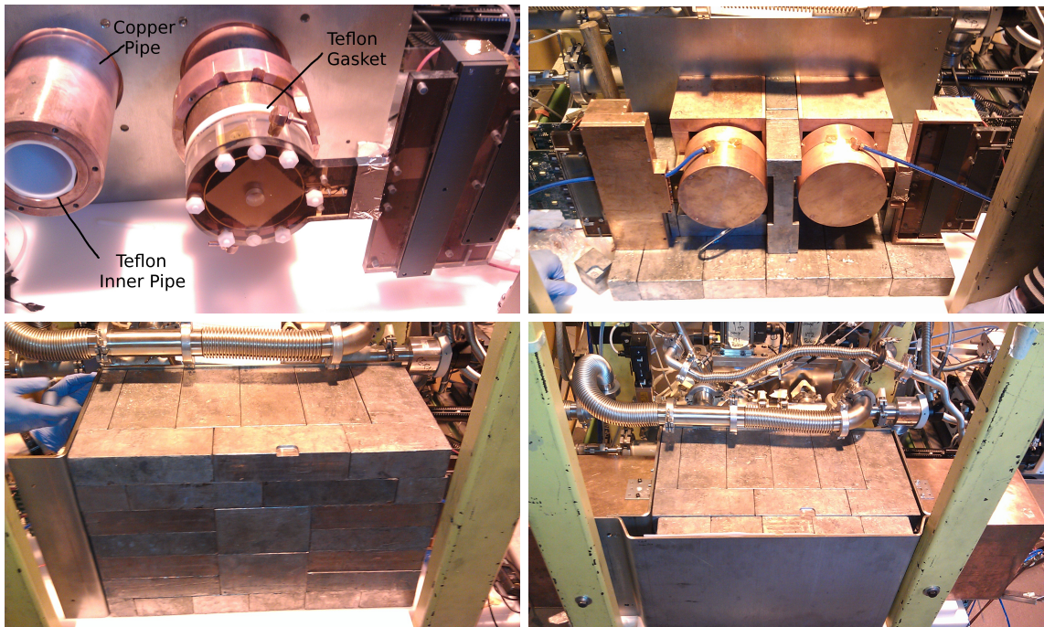
Figure 6.16. The different stages of installation of sunset micromegas.
