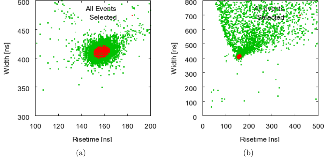
Figure 7.7. (a) Selection region of the risetime-width cut is indicated in red. (b) The effect of the same cut on the background data, where selected events account for 5% of the all events.
