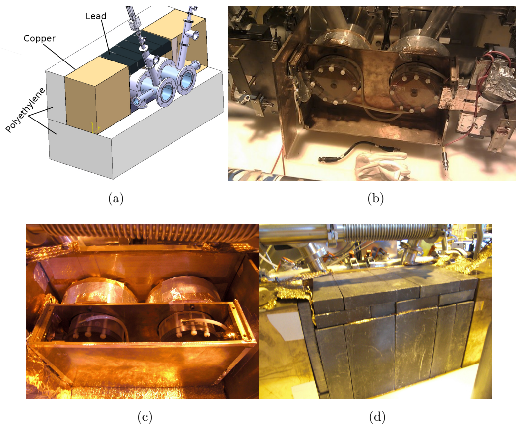
Figure 6.8. (a) Drawing of the shielding. (b) The inner view before the shielding is installed. (c) Inner Faraday cage. (d) Shielding with the lead bricks.
