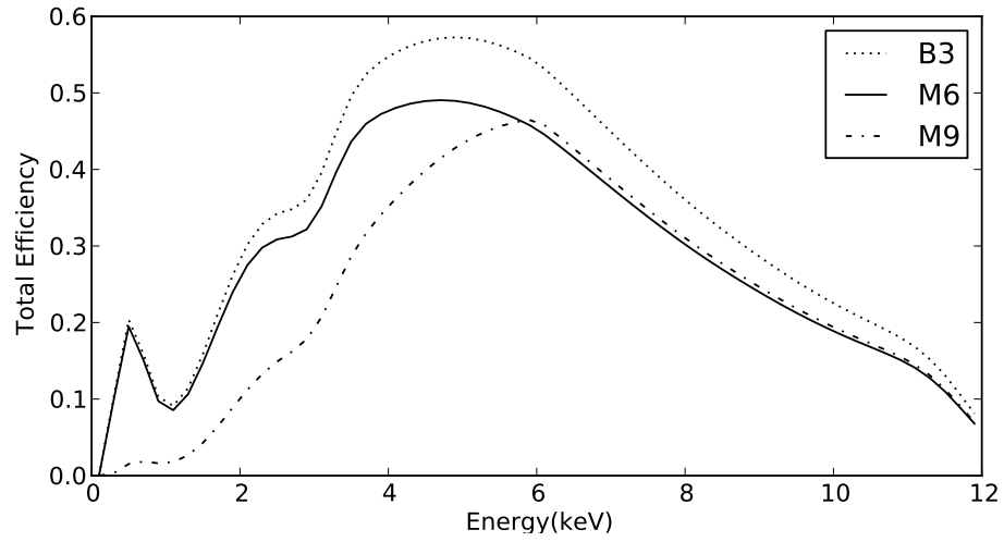
Figure 9.14. Total efficiency of all three detectors.
