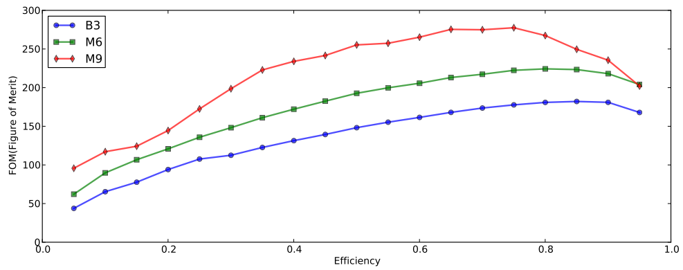
Figure 8.1. The efficiency vs. FOM curves for events in 5 – 7keV range.
