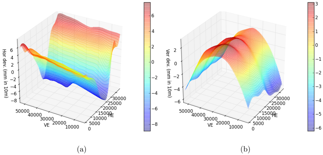
Figure 4.8. Non linearity of the encoder-angle relation. In each plot, a linear fit was done for encoders vs. angles, and this fit were subtracted from the angles. (a) Deviation of horizontal angle. (b) Deviation of vertical angle.
