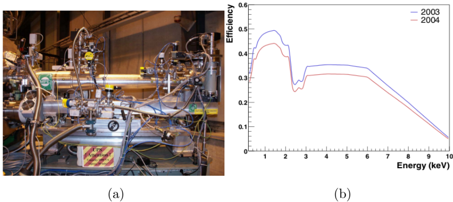
Figure 4.18. (a) The photo of the X-ray telescope and pn-CCD detector. (b) The combined efficiency of the telescope system and the pn-CCD for 1 – 10keV range.
