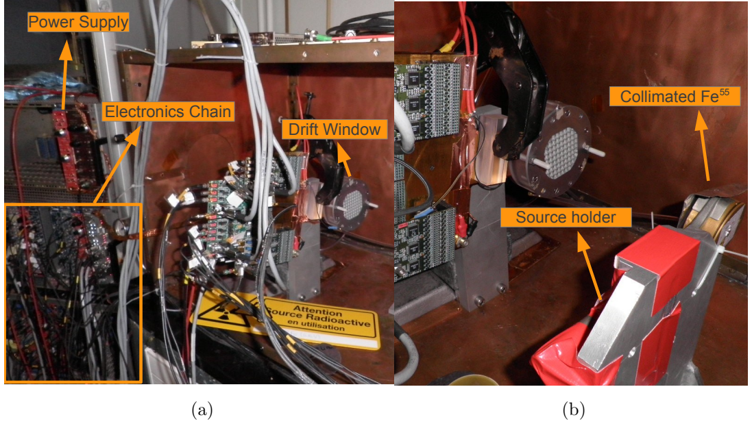
Figure 5.10. (a) The experimental setup of the characterization tests. (b) The positioning of the ^{55}\text{Fe} source.
