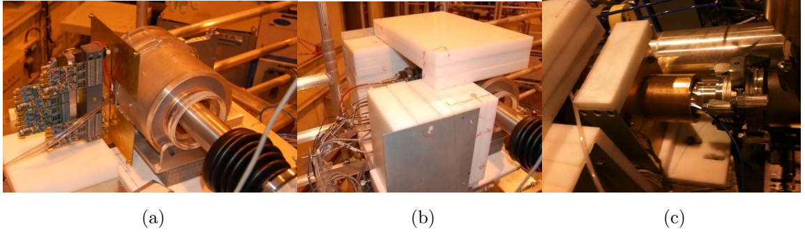
Figure 4.22. Different shielding setups of the sunrise micromegas. (a) The detector with the compact shielding. (b) The detector with the additional layers of polyethylene shielding. (c) Latest addition to the shielding.
