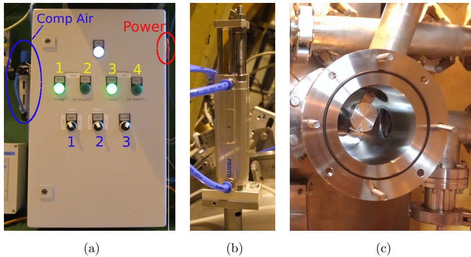
Figure 6.18. (a) The control box of the calibrators. (b) The source manipulator. (c) View of the source inside the vacuum pipe.
