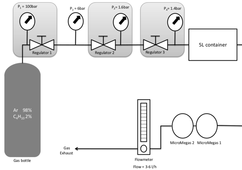
Figure 6.3. Schematics of the sunset micromegas gas system.
