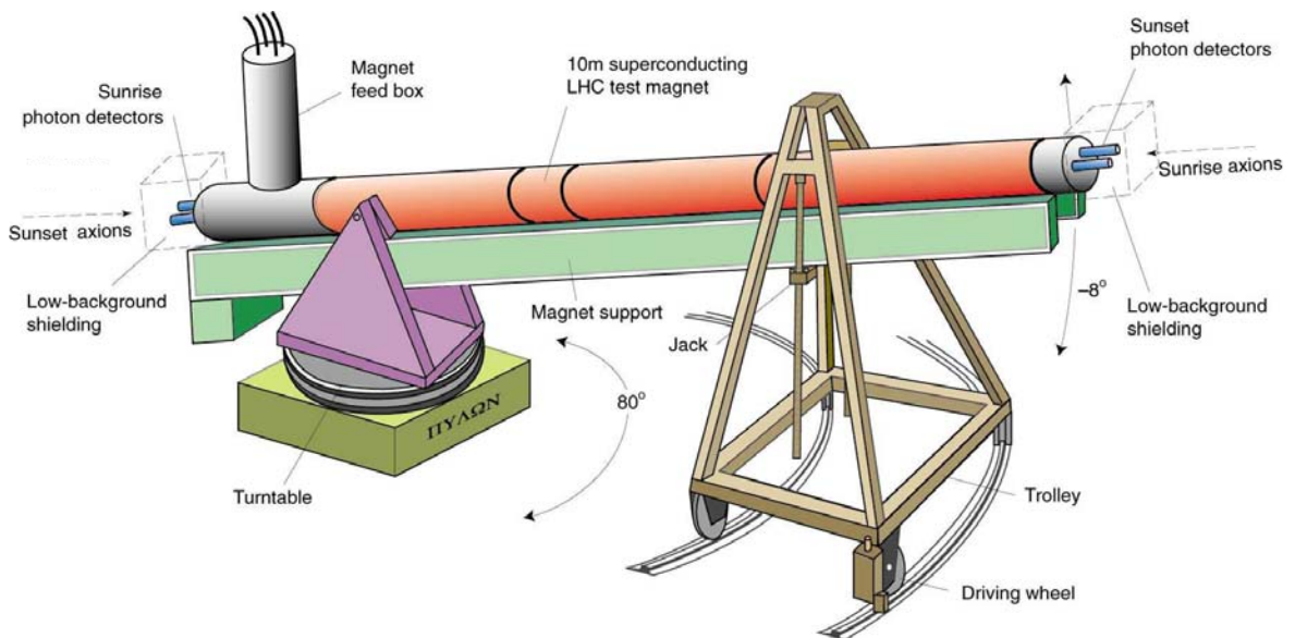
Figure 4.5. Drawing of the CAST Magnet and movement system.
