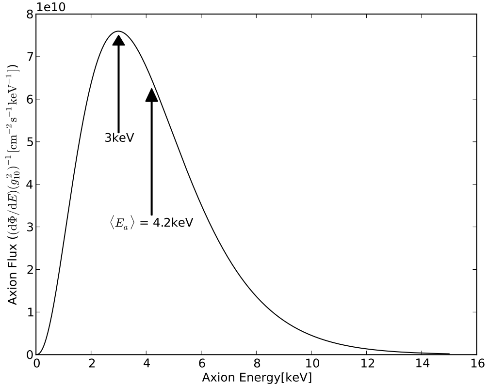
Figure 3.2. Differential solar axion flux at Earth. Note that the real flux depends on the value of coupling constant.
