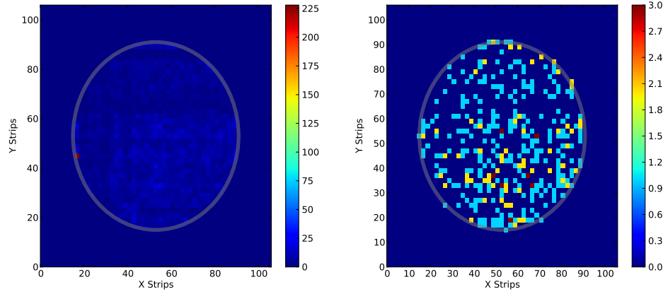
Figure 9.7. Cumulative hitmap of background events in M6 after background selection. Tracking and background counts are shown in separate plots. The noisy area in the background can be seen in the left bottom part of the coldbore circle.
