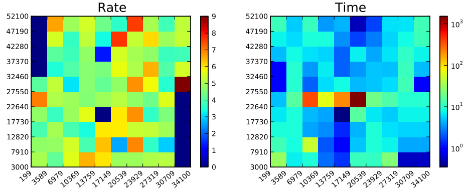
Figure C.18. Background rate in counts/hour at different magnet positions for B3.
