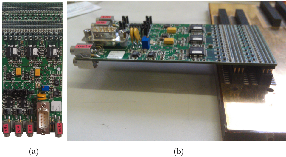
Figure 6.9. (a) Gassiplex card: On the bottom, lemo connectors of clear, clock, track and hold, and output signal can be seen. (b) A gassiplex card connected to the micromegas detector.
