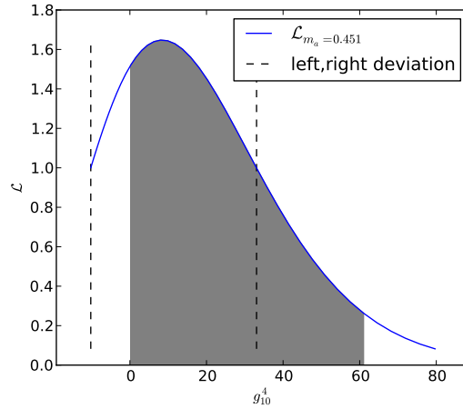
Figure 10.4. Likelihood function for m_a = 0.451\text{eV} , plotted as a function of g_{10}^4 .
