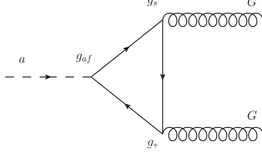
Figure 2.1. Axion-gluon interaction with a triangle fermion loop. g_{af} is the axion-fermion Yukawa coupling, while g_s is the strong coupling constant.
