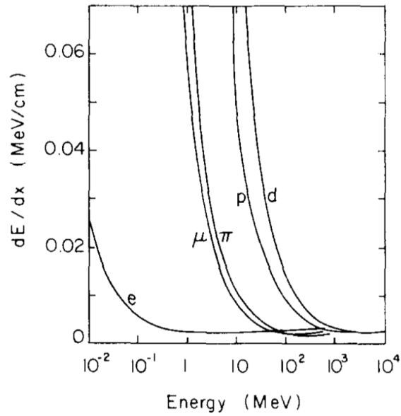
Figure 5.1. dE/dx in air for different particles. Plot taken from [83]. At high energies, differential energy loss becomes almost same for all particles, independent of their mass, until radiative effects become considerable.
