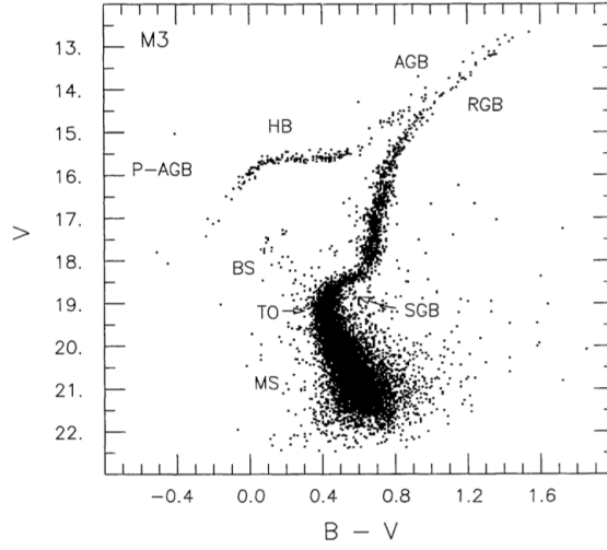
Figure 2.4. The Hertzsprung-Russell diagram for 10637 stars in M3 [27]. The surface brightness is plotted in y axis and increases towards the top while the surface temperature is plotted in x axis and increases towards left.
