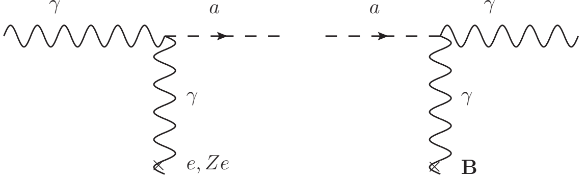
Figure 3.1. Primakoff Effect.
