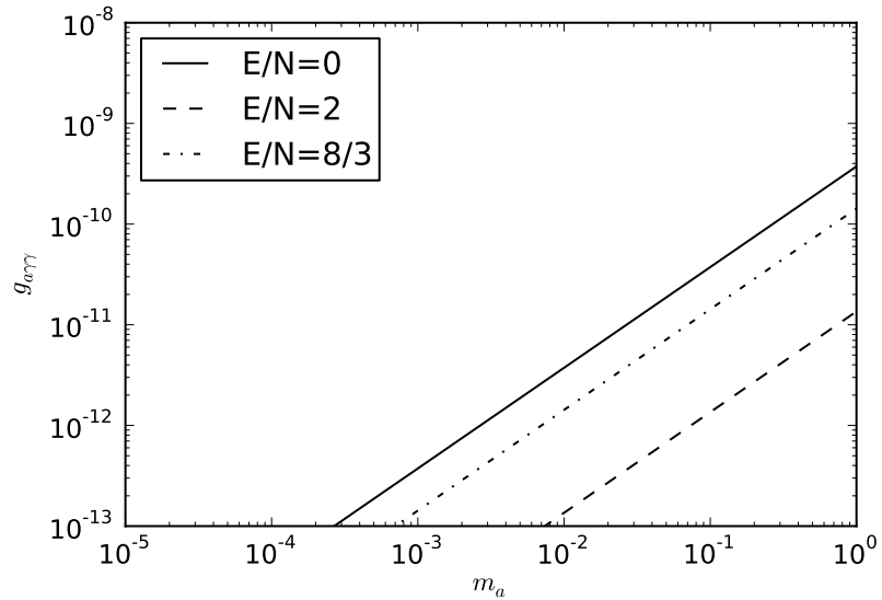
Figure 2.3. Axion mass versus the coupling constant, depending on the E/N ratio for most widely accepted axion models.
