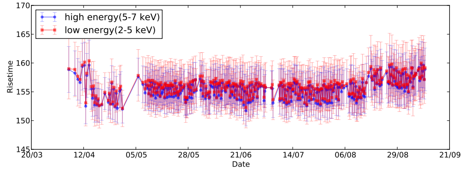
Figure C.12. Evolution of pulse risetime for M6.
