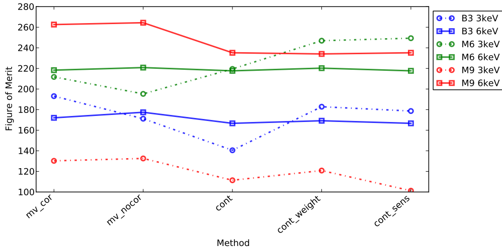
Figure 8.5. Comparison of FOM for different methods. FOM is directly related with the sensitivity of CAST experiment, thus is the most essential parameter in choosing of the discrimination method.
