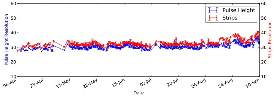
Figure C.10. Evolution of the energy resolution for M6, given in FWHM percentage at 5.96keV.
