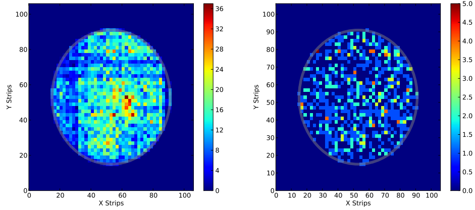
Figure 9.5. Cumulative hitmap of background events in B3 after background selection. Tracking and background counts are shown in different colors.
