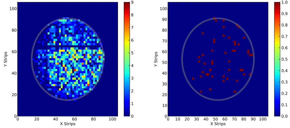
Figure 9.11. Cumulative hitmap of background events in M9 after background selection. Tracking and background counts are shown in separate plots.
