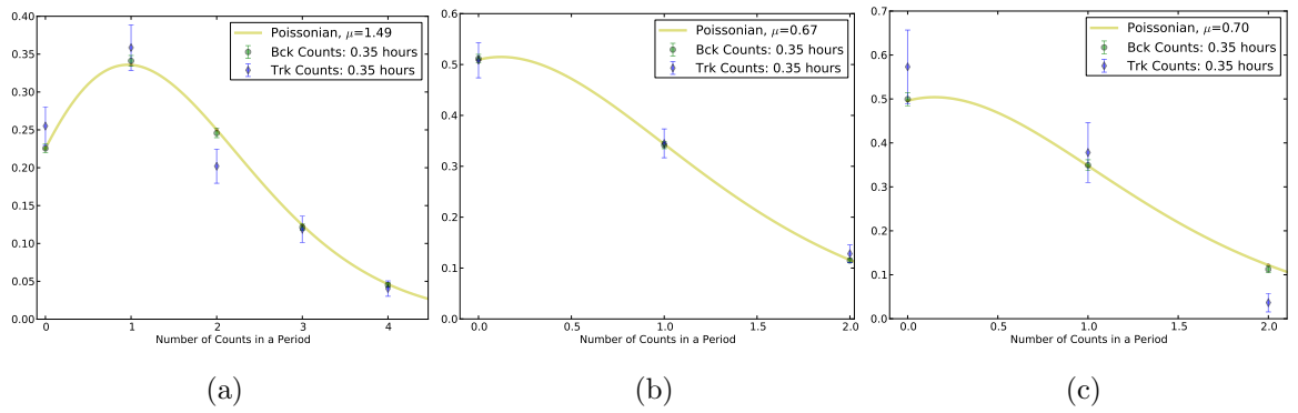
Figure 9.19. Compatibility of background and tracking count rates with Poissonian statistics considering a time bin of 0.35 hours. (a) B3, (b) M6, (c) M9.
