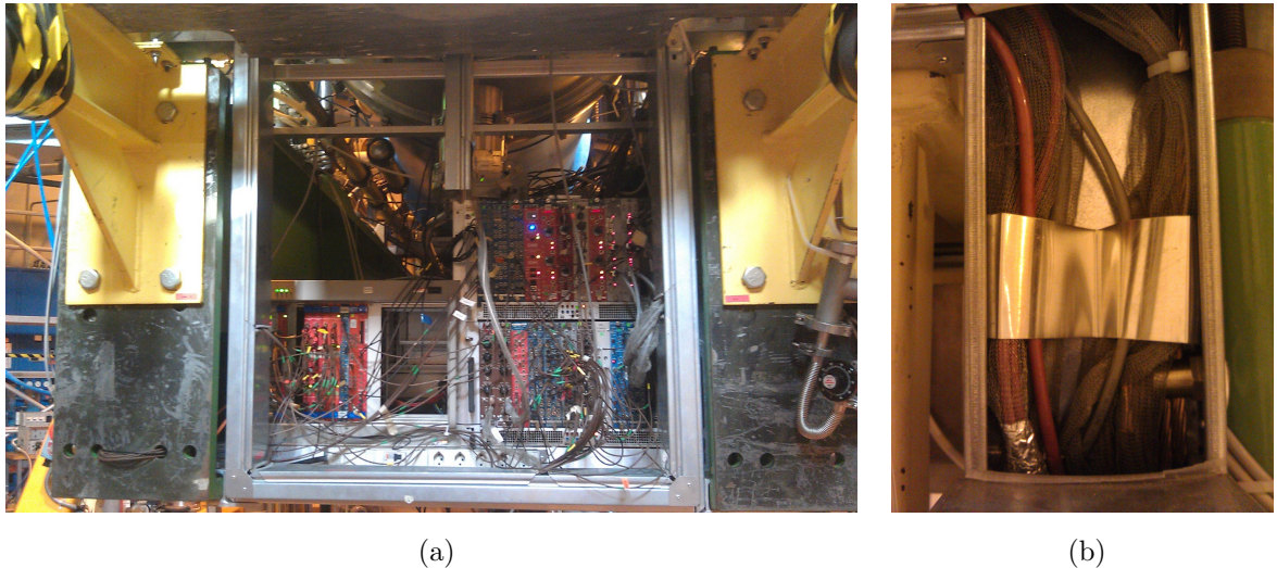
Figure 6.14. (a) General view of the cable trays and the electronics. (b) View of the cables inside the cable tray.
