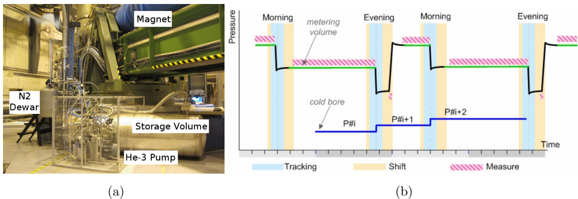
Figure 4.15. (a) Photo of the gas system. (b) Filling scheme used during 2008.
