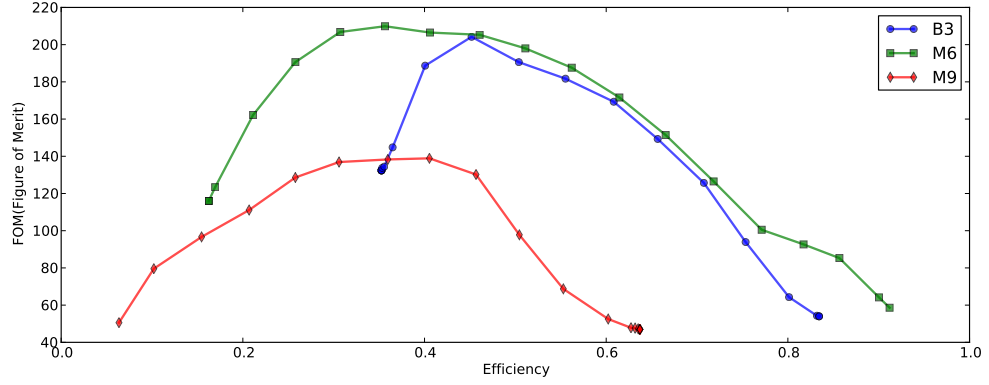
Figure 8.2. The efficiency vs. FOM curves for events in 2 – 5keV range. The efficiency of the low energy events are fine tuned by varying the energy correction factor.
