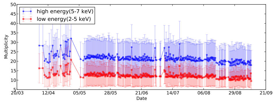
Figure C.14. Evolution of strip multiplicity for M6.
