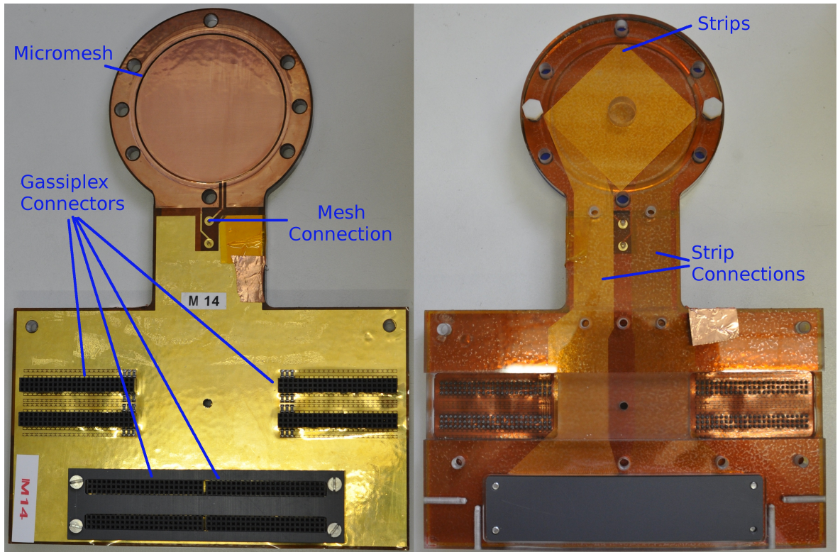
Figure 5.8. Photo of two sides of a microbulk micromegas detector without the readout cards and plexiglas chamber.
