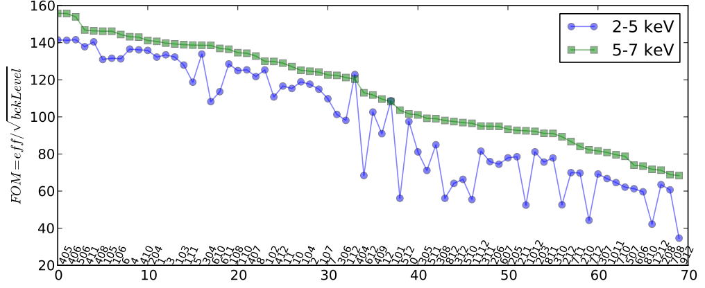
Figure C.4. The observable pairs vs. FOM for low and high energy events, for B3.
