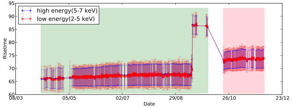
Figure C.11. Evolution of pulse risetime for B3 and M9. Different detectors are indicated by different background colors.
