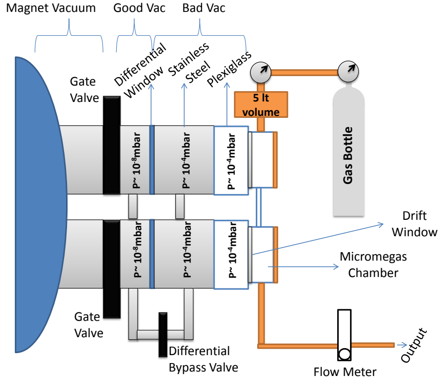
Figure 6.2. Simplified schematics of sunset micromegas vacuum and gas systems.
