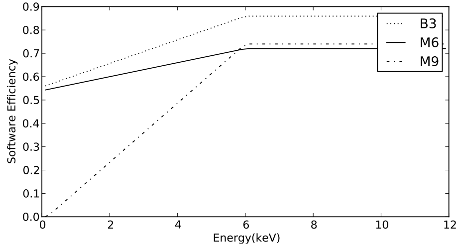
Figure 9.13. Software efficiency curves for all three detectors.
