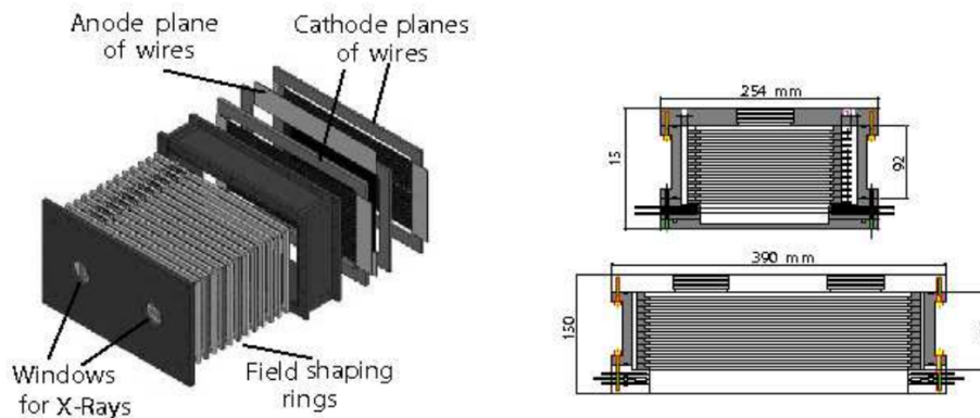
Figure 4.20. The exploded view of the CAST TPC.
