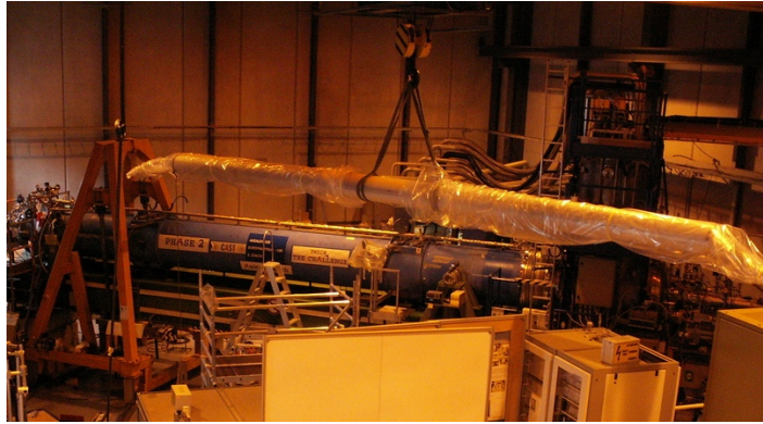
Figure 4.16. A photo from the installation of the expansion volume.
