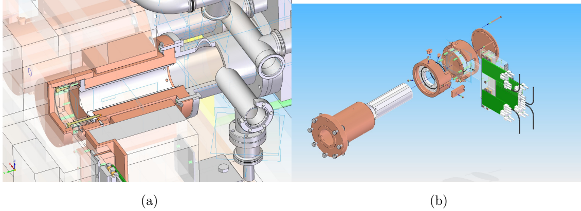
Figure 6.15. (a) Drawing of sunset micromegas shielding, (b) Exploded view of the inner part of the shielding.
