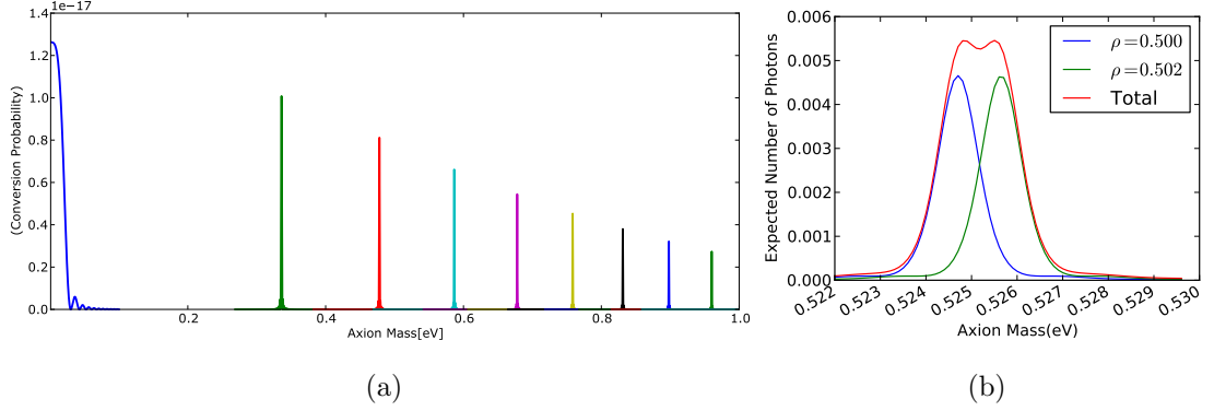
Figure 3.5. (a) Conversion probability for axions with energy 3keV, for pressures between 0-100 mbar, with step of 10mbar. (b) Total expected number of photons per unit area for 2 different densities.
