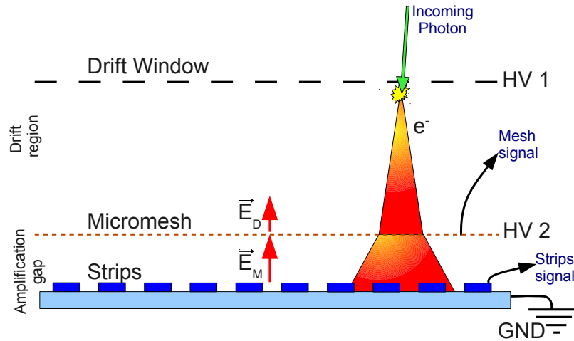
Figure 5.4. The working principle of the micromegas detector.
