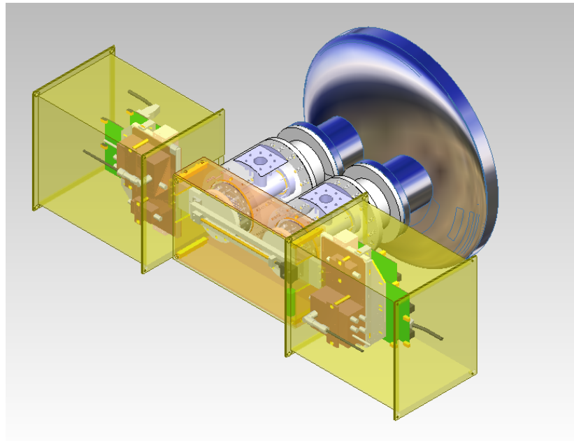
Figure 6.1. Drawing of the sunset micromegas.
