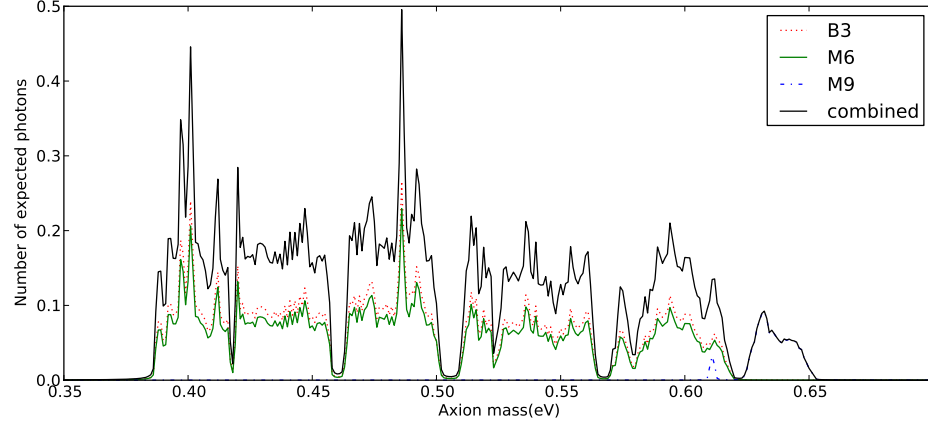
Figure 10.3. (b) Expected number of photons during 2008 data for all sunset micromegas, depending on the axion mass, assuming coupling constant g_{a\gamma} = 10^{-10} .
