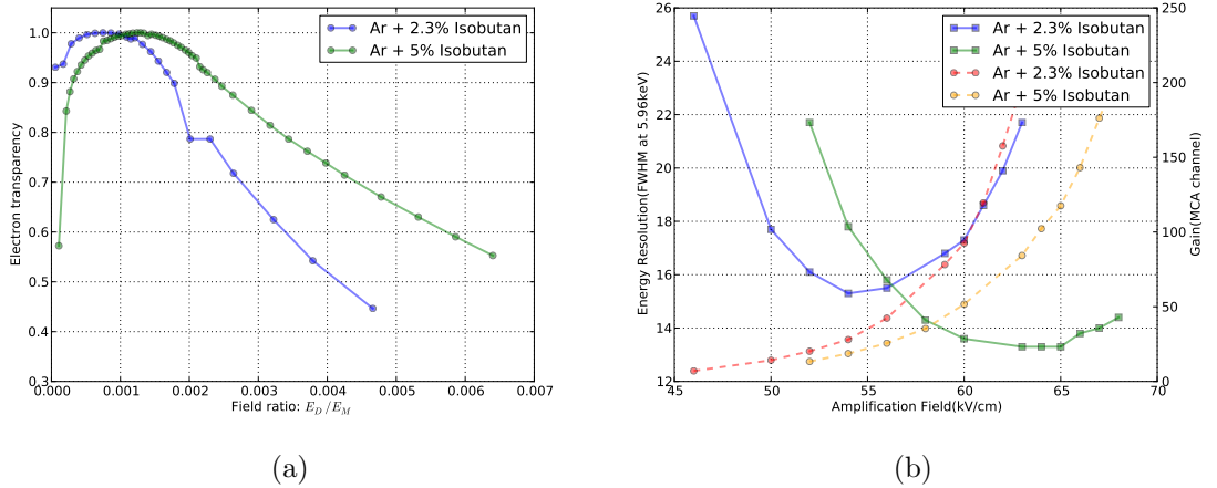
Figure 5.12. (a) Electric field ratio vs. electron transparency. The transparency of the highest gain is normalized to 1. (b) Amplification field vs. energy resolution(continuous lines) and gain(dashed lines).
