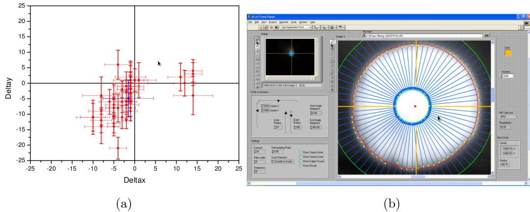
Figure 4.11. 2008 Sun Filming. (a) The deviation from the center of the Sun in pixels. (b) Analysis software that calculates the position of the center of the Sun.
