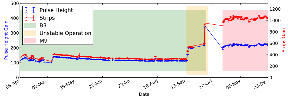
Figure C.7. The gain of pulse amplitude and strip charge in fADC units during the calibrations for B3 and M9. The period when each detector is used and an unstable period of operation is shown in different background colors.
