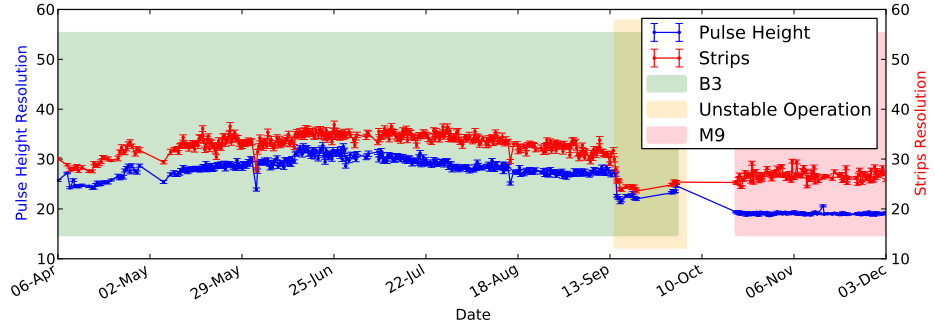
Figure C.9. Evolution of the energy resolution for B3 and M9, given in FWHM percentage at 5.96keV.
