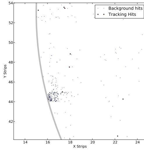
Figure 9.8. Closeup look at the noisy area in the detector M6.
