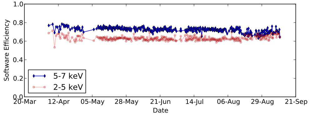
Figure C.16. Evolution of the software efficiency for M6.
