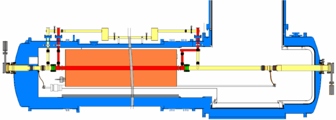
Figure 4.13. The schematics of the gas pipes inside of the cryostat. Green parts denote the cold windows and horizontal red pipes are the cold bores of the magnet. Yellow pipes denote the various vacuum parts of the system.
