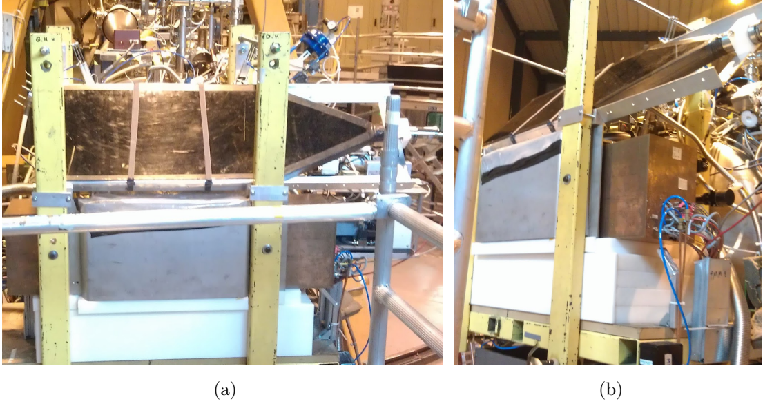
Figure 6.17. The muon veto counter.
