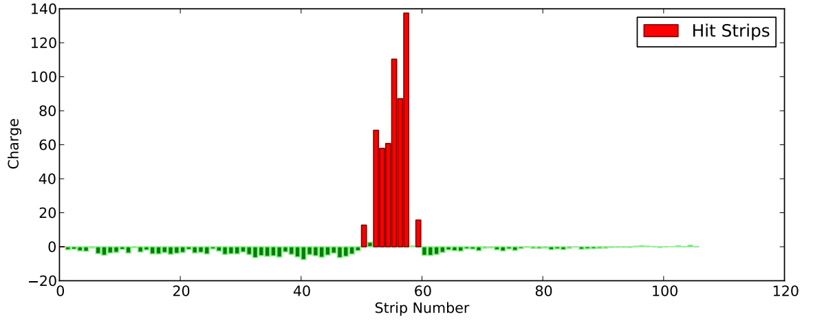
Figure 7.2. A single cluster event that has multiplicity eight, with two non-hit strips inside.
