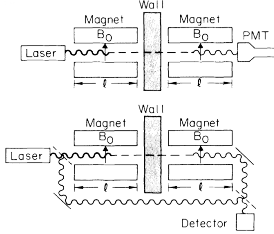
Figure 2.7. Schematics and different possible setups of photon regeneration experiments.
