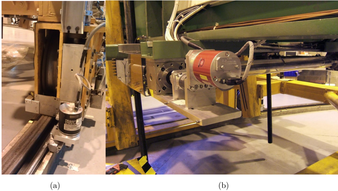
Figure 4.6. Vertical and horizontal driving mechanisms. (a) Driving wheel and horizontal motor encoder. (b) Vertical movement jacks and vertical motor encoder.
