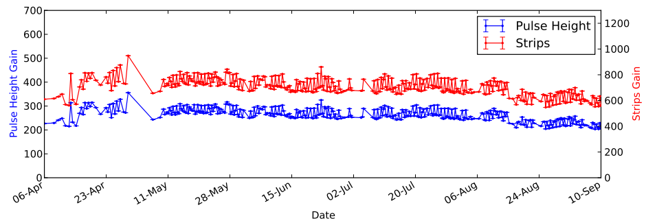
Figure C.8. The gain of pulse amplitude and strip charge in fADC units during the calibrations for M6.
