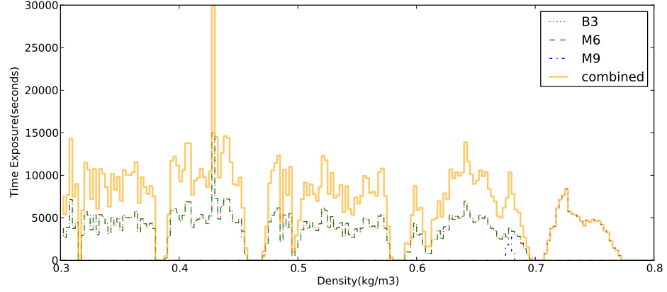
Figure 10.2. Density exposure of all three detectors(dashed lines) and combined exposure(solid line).
