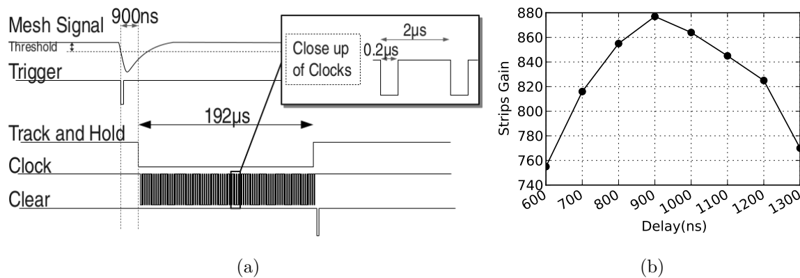
Figure 6.10. (a) Sketch of the important signals in the micromegas DAQ chain. (b) The strips gain of different runs with different delay values. The highest gain was obtained when the delay was set to 900ns.
