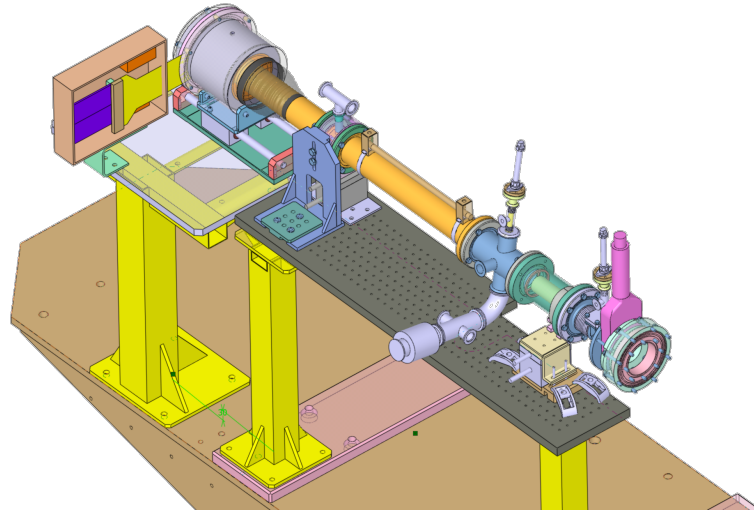
Figure 4.23. Drawing of the sunrise micromegas.
