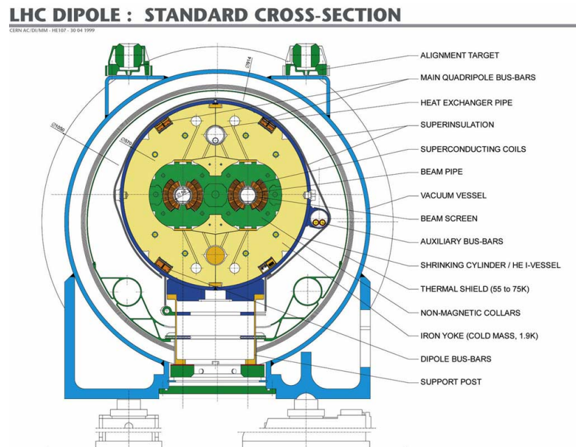
Figure 4.3. Cross section of LHC dipole magnets.
