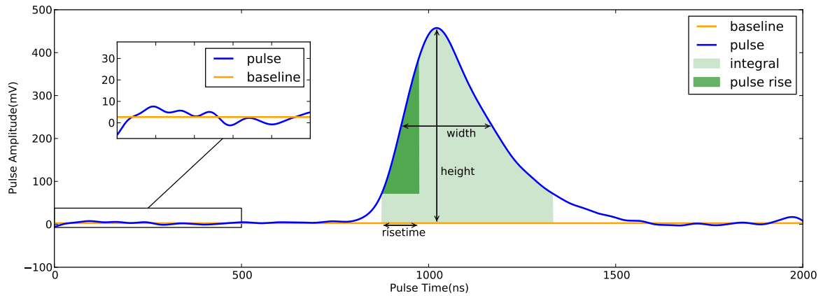
Figure 7.3. A sample mesh pulse from ^{55}\text{Fe} calibration with explanation of mesh observables.
