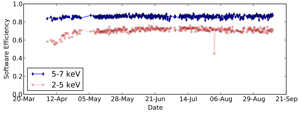
Figure C.15. Evolution of the software efficiency for B3.
