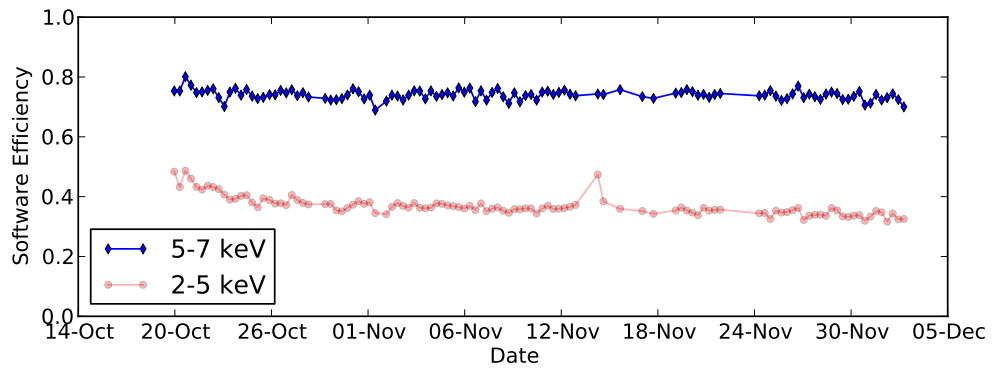
Figure C.17. Evolution of the software efficiency for M9.
