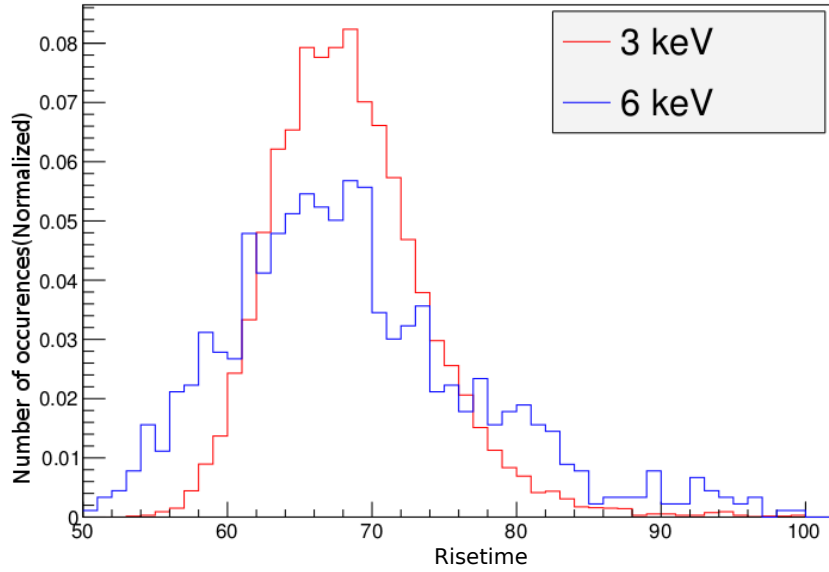
Figure 7.5. Risetime distribution for 6 and 3keV events. The energy from the escape peak has the same mean, but higher standard deviation.
