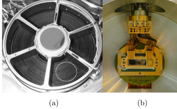
Figure 4.19. (a) The comparison of the aperture of the cold bore and the X-ray telescope. (b) The pn-CCD chip.
