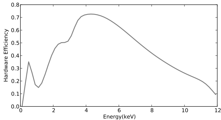
Figure 6.6. The hardware efficiency curve of sunset micromegas.
