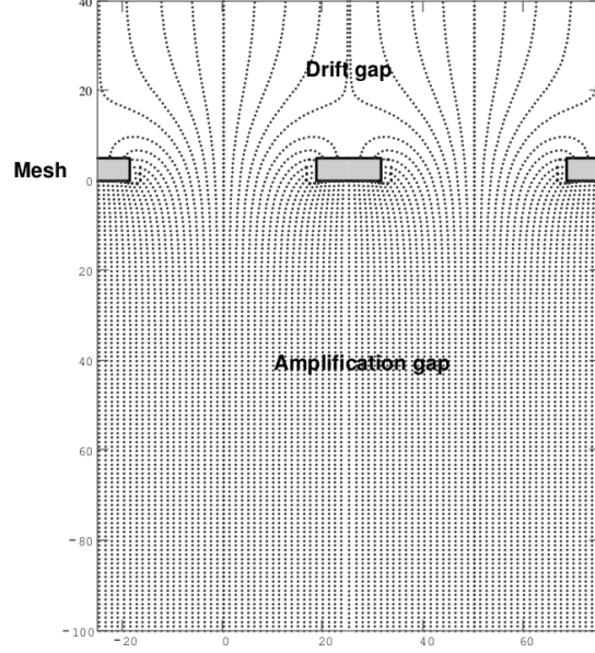
Figure 5.5. The funnel like shape of the electric field lines around the micromesh.
