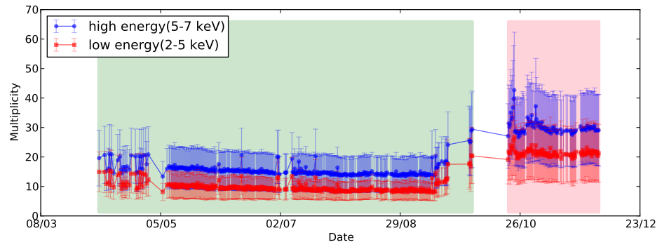
Figure C.13. Evolution of strip multiplicity for B3 and M9. Different detectors are indicated by different background colors.
