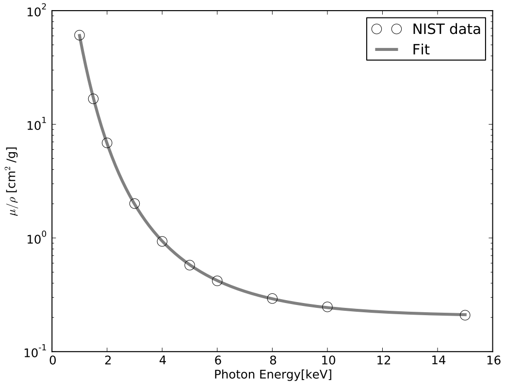
Figure 3.3. He 3 mass attenuation coefficient: Circles show the values taken from NIST database, continuous line show the fit function.
