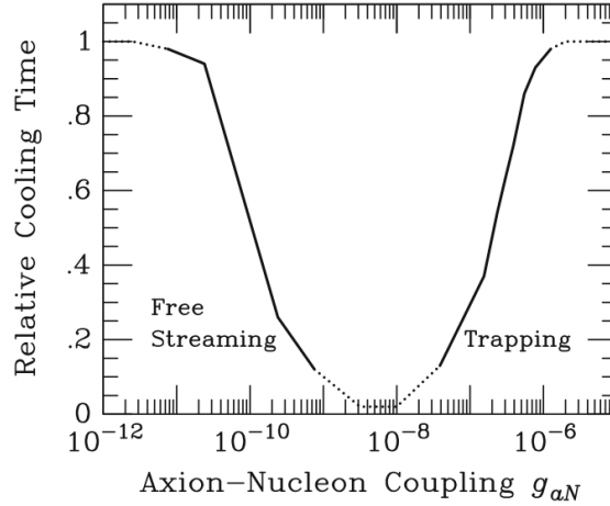
Figure 2.5. Cooling time vs. axion-nucleon coupling constant. In case of small or large couplings the cooling time would be affected minimally, while in between, axion-nucleon interaction would decrease the time significantly. Image taken from [9].
