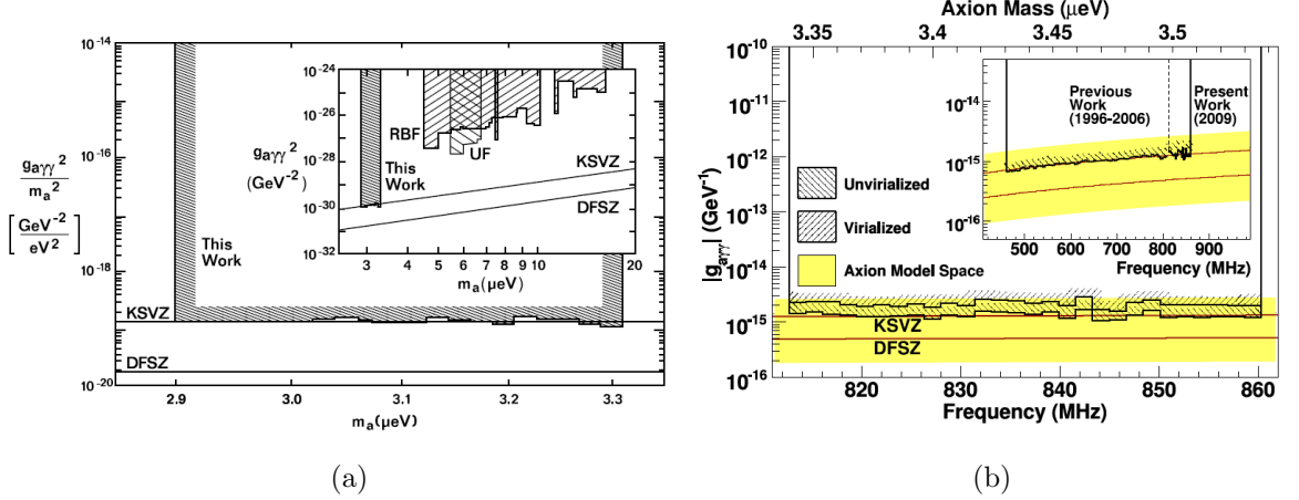
Figure 2.8. (a) Results of first generation haloscopes and ADMX [44]. (b) Recent results from ADMX [47].
