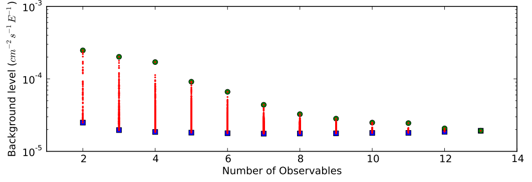
Figure C.1. The number of observables vs. the background levels, for B3.
