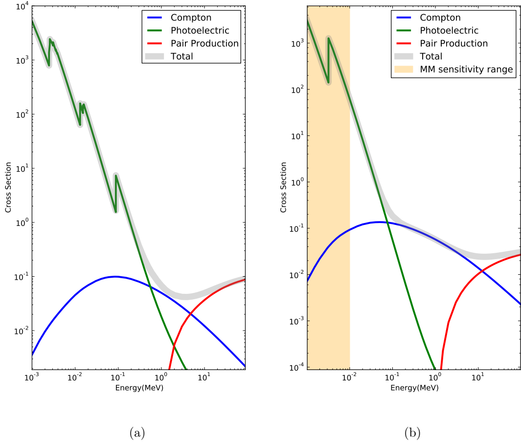
Figure 5.3. Cross section of different photon interactions in (a) Lead, (b) Argon. X axis shows the energy of the beam, while y axis shows the cross section, which is proportional to the interaction probability.
