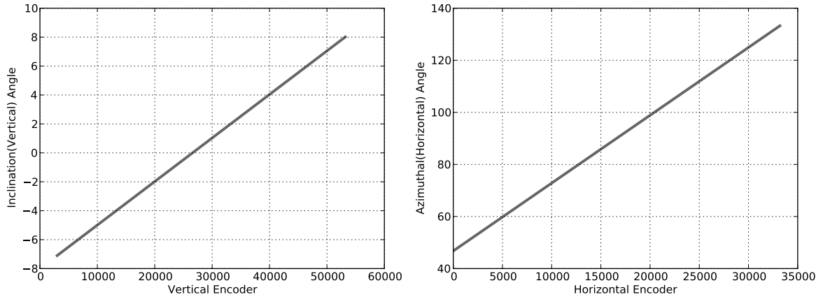
Figure 4.7. Motor encoders vs. angles.
