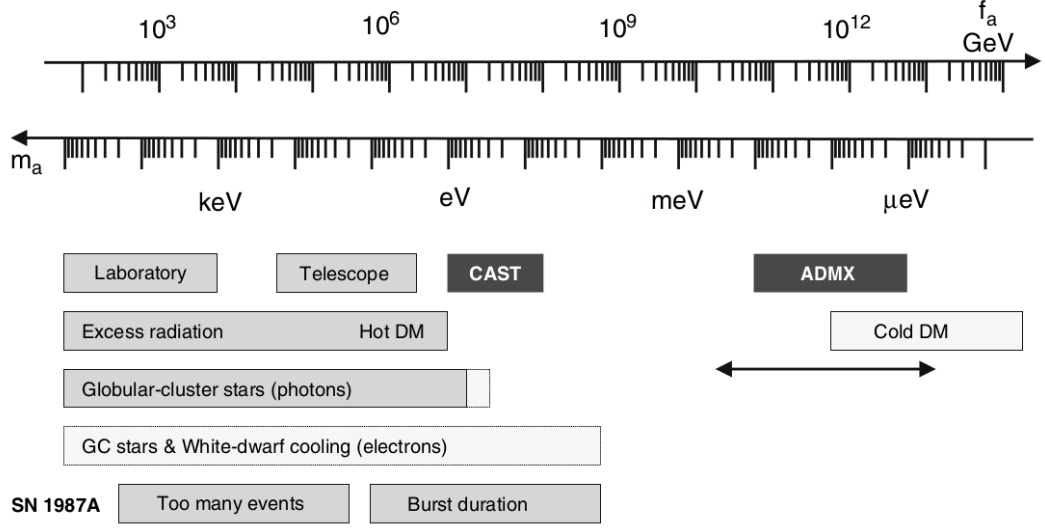
Figure 2.6. Summary of excluded mass and PQ scale ranges due to different constraints. Image taken from [9].
