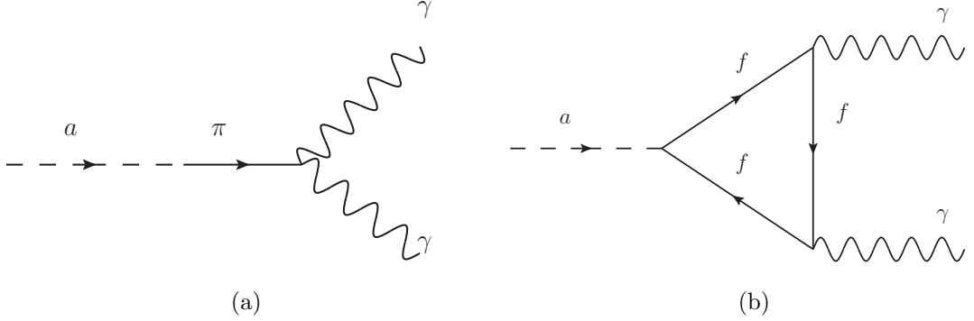
Figure 2.2. (a) The axion-photon interaction due to pion mixing. (b) The axion-photon interaction due to Primakoff effect.
