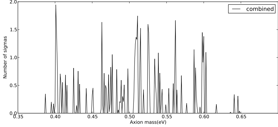
Figure 10.5. Deviation of maximum likelihood from the null hypothesis for the axion masses CAST was sensitive in 2008. The deviation is in terms of left sigma of the distribution.
