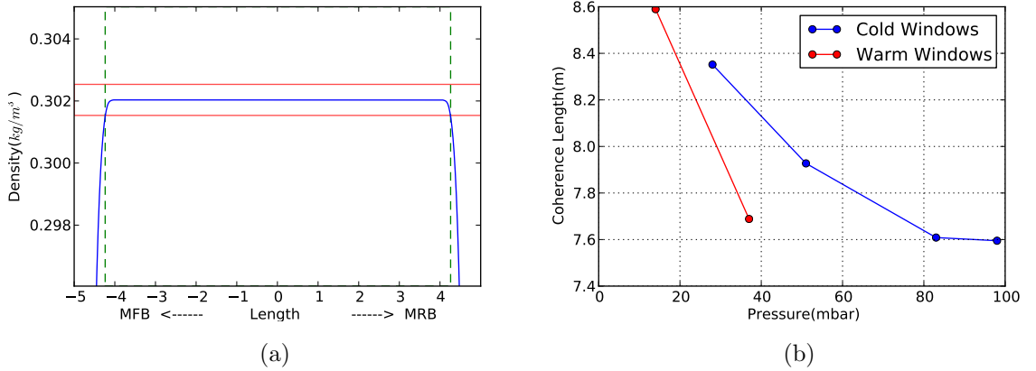
Figure 10.1. (a) Density profile in the magnet for pressure 14mbar. The red lines show the DST while the dashed vertical lines show the length of the gas volume within the DST. (b) Parametrization of effective length for warm(red) and cold(blue) windows.
