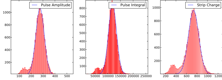
Figure 7.4. The spectra and Gaussian fits to three gain observables.
