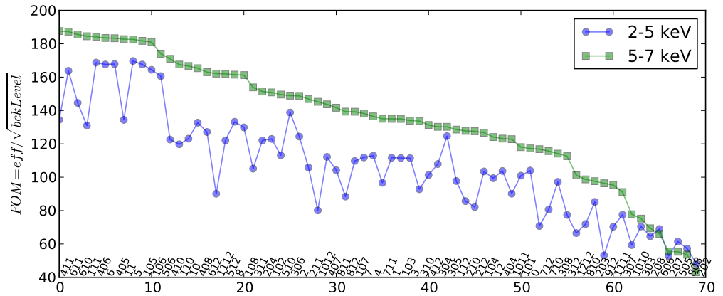
Figure C.5. The observable pairs vs. FOM for low and high energy events, for M6.
