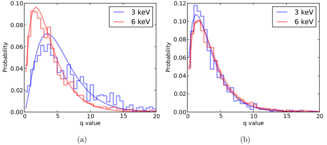
Figure 7.6. The distribution of the q value for main and escape peaks during the calibration. (a) Non-corrected q value. (b) Corrected q value, with a = 1.1 .
