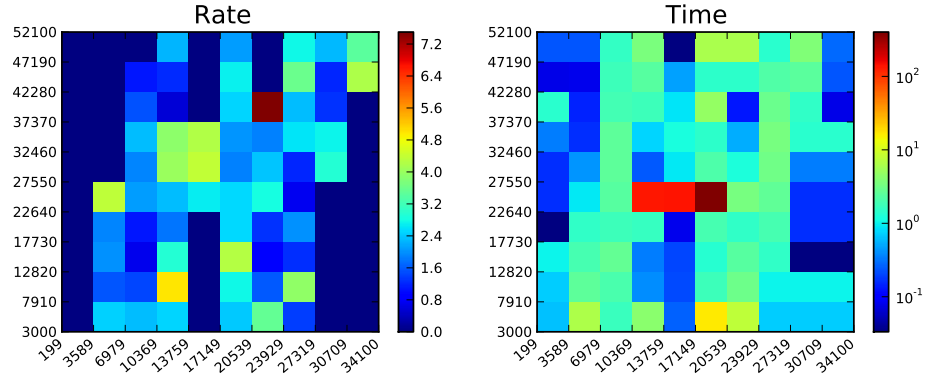
Figure C.20. Background rate in counts/hour at different magnet positions for M9.
