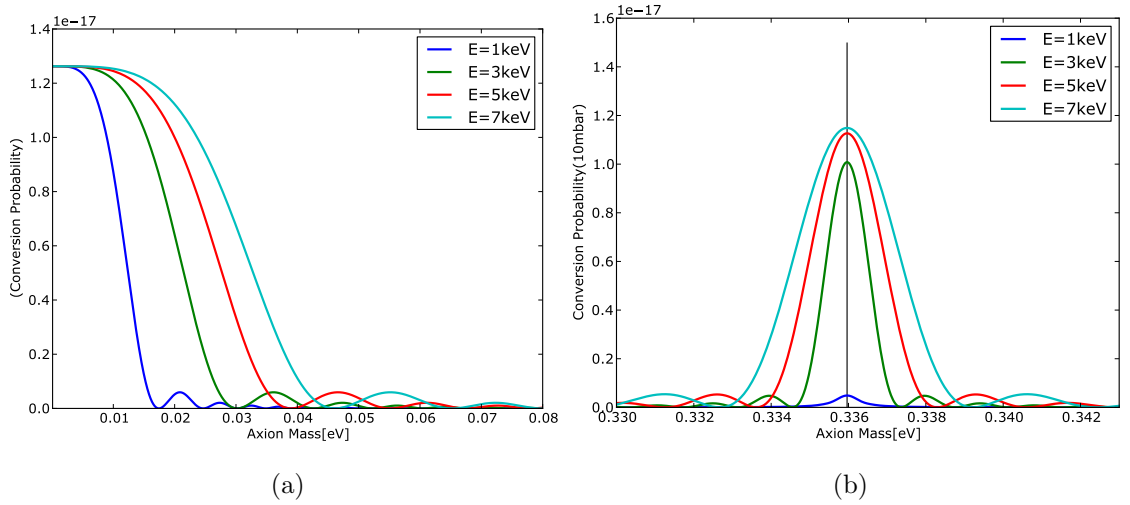
Figure 3.4. (a) Conversion probability in vacuum for different energies. (b) Conversion probability with 10mbar of pressure for different energies, the vertical line shows effective photon mass for 10mbar, m_\gamma = 0.33596 .
