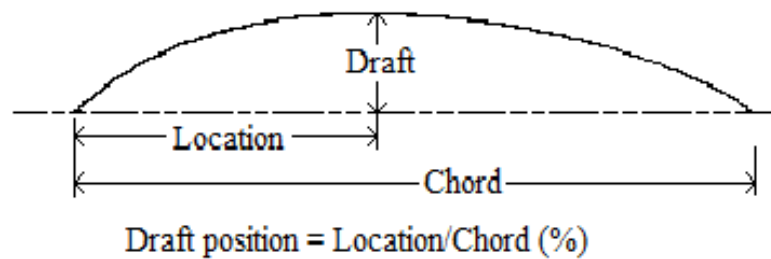
Figure 2.3 : Sail camber [3].
