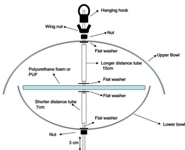
Figure 2.5. Detailed PUF disc as a passive sampler (United Nations Environment Programme, 2017)
