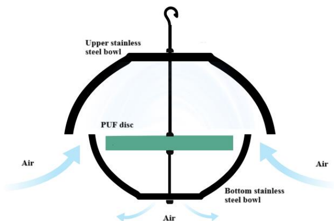
Figure 2.6. Air circulation in stainless steel bowls using PUF disc
