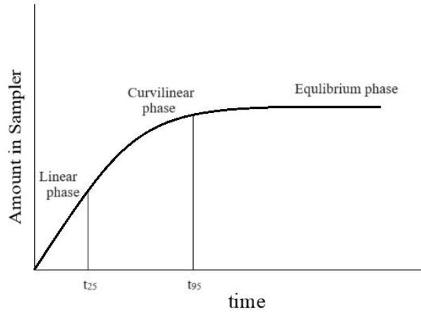
Figure 3.6. The uptake phases of chemicals in a passive sampler (Shoieb and Harner (2002))
