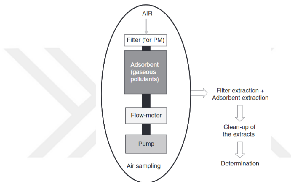
Figure 2.4. The active air sampling device and the analytical steps (Garcia-Jares et al., 2012)
