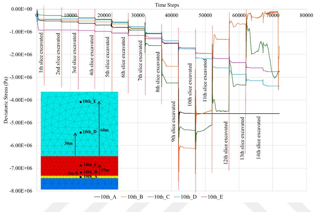
Figure 5.15. Deviatoric stress (Pa) analysis of points with different depths (Discontinuum model with orientation of 60^\circ and k=1 )
