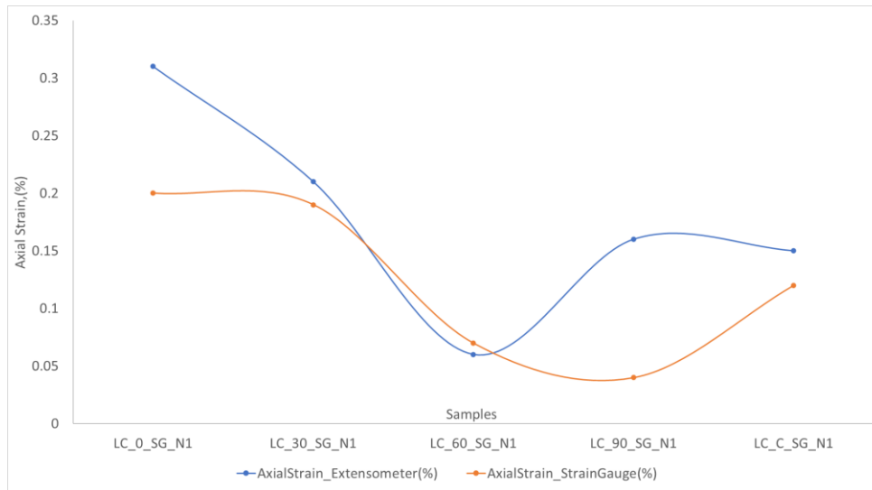
Figure 3.15. Axial strain (%) of LC samples at failure (Extensometer versus Strain Gauge)
