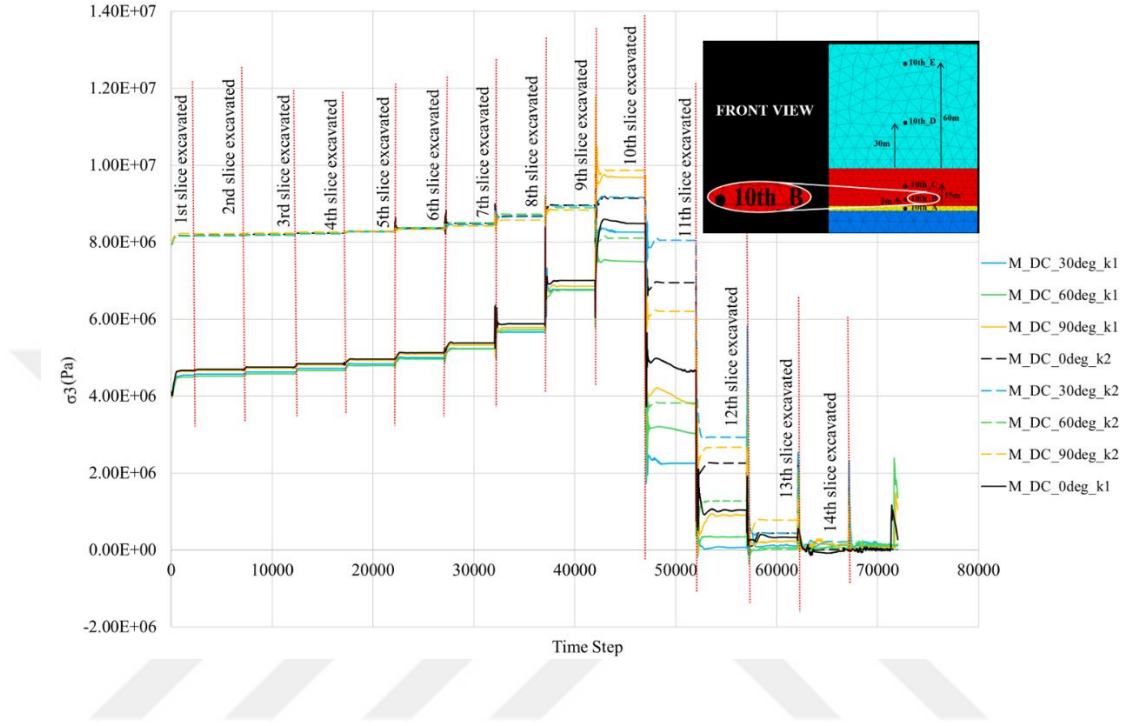
Figure 5.8. Comparison of \sigma_3 values (Pa) from the history point located above the 10 th coal slice - 3 meters high on the immediate roof (10th_B) in different discontinuous cases
