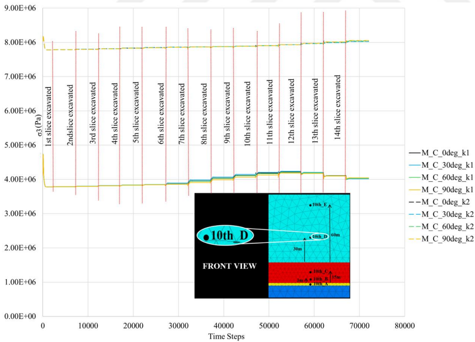
Figure A.4 Comparison of \sigma_3 values (Pa) from the history point located above the 10 th coal slice - 30 m high on the overburden (10th_D) in different continuous cases
