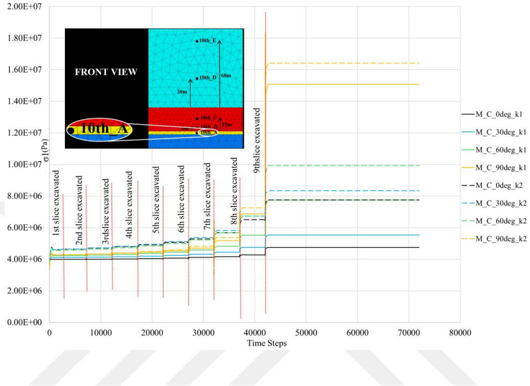
Figure 5.5. Comparison of \sigma_1 values (Pa) from the history point located inside the 10 th coal slice (10th_A) in different continuous cases
