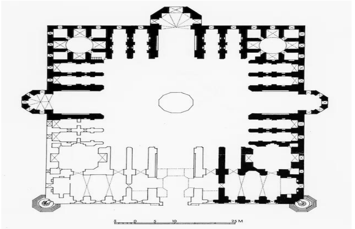
Plan 6. Mahmûd Gâvân Medresesi Planı ( https://www.archnet.org/sites/3988 )
