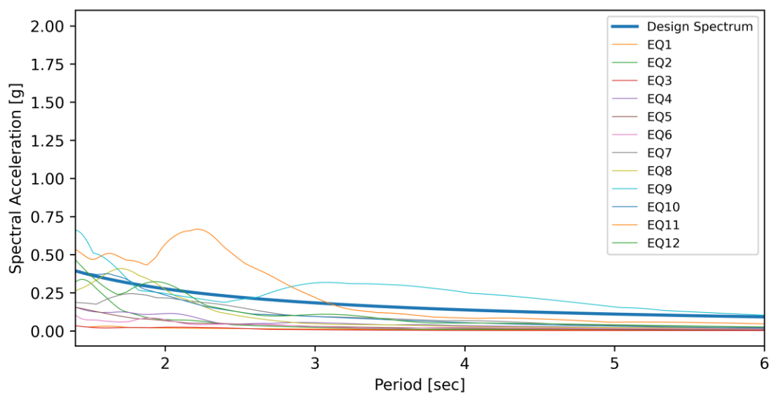
Figure 2.5 Close look unmatched Spectral Acceleration for all Earthquake
