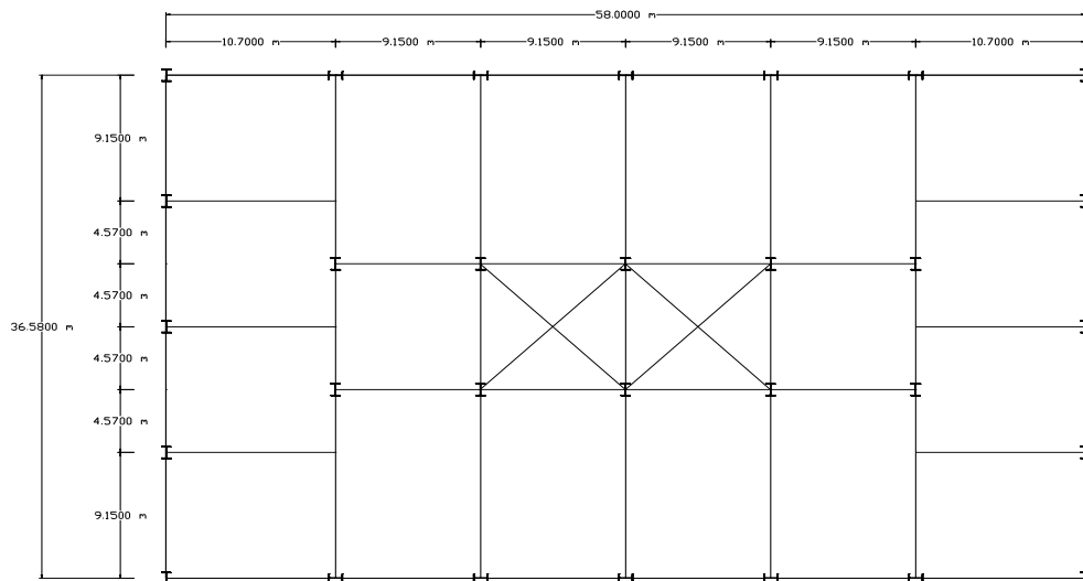
Figure 2.1 Plan view of the structure
