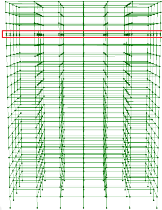
Figure 4.5 Controlled building when isolator at 17th floor
