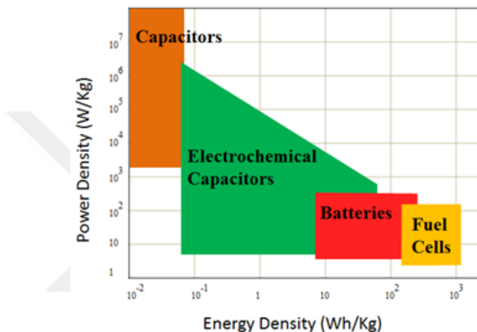
Figure 1. Ragone plot for different electrochemical systems.
