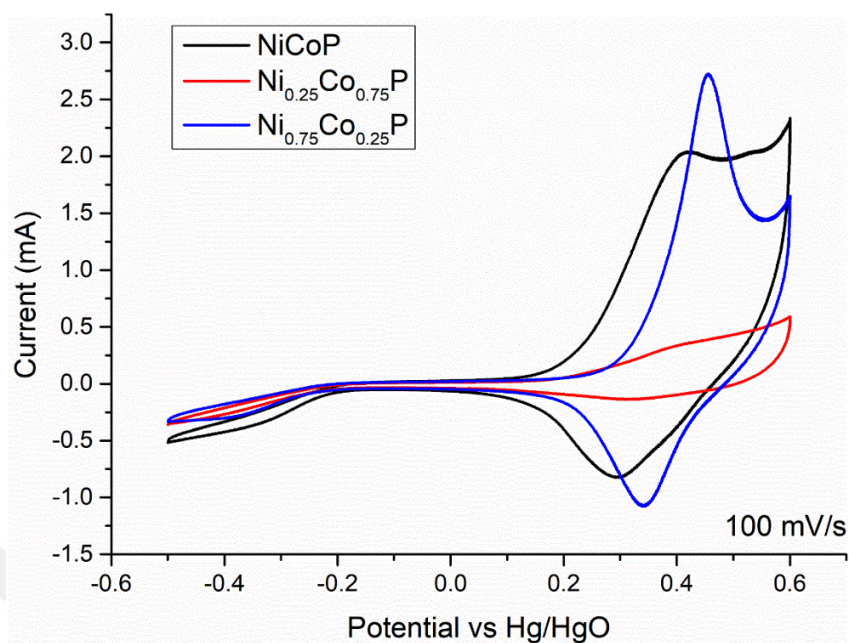
Figure 29. Cyclic voltammograms of \text{Ni}_x\text{Co}_{1-x}\text{P} samples at 1600 rpm in RDE.
