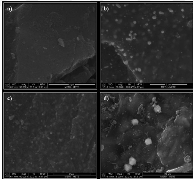
Figure 7. SEM micrographs of a) 4IR-1Ni, b) 4IR-5Ni, c) and d) 4IR-10Ni.
