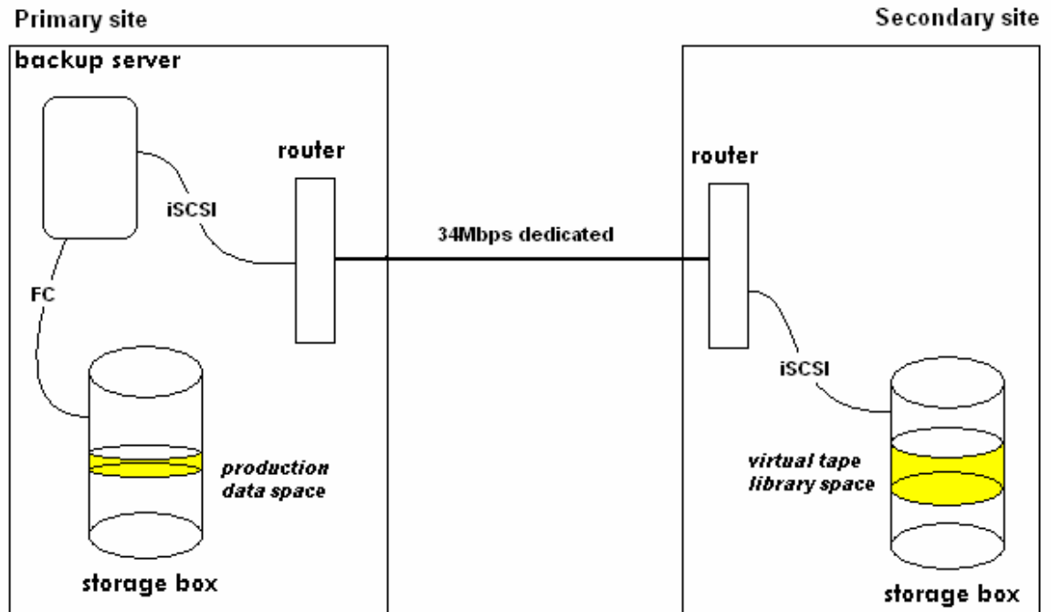
Figure 6.1: iSCSI-based remote data backup
