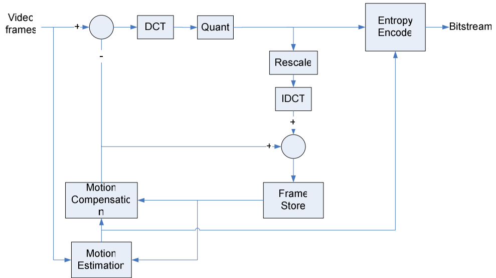
Figure 4-1: Block Diagram of H.263 encoder.
