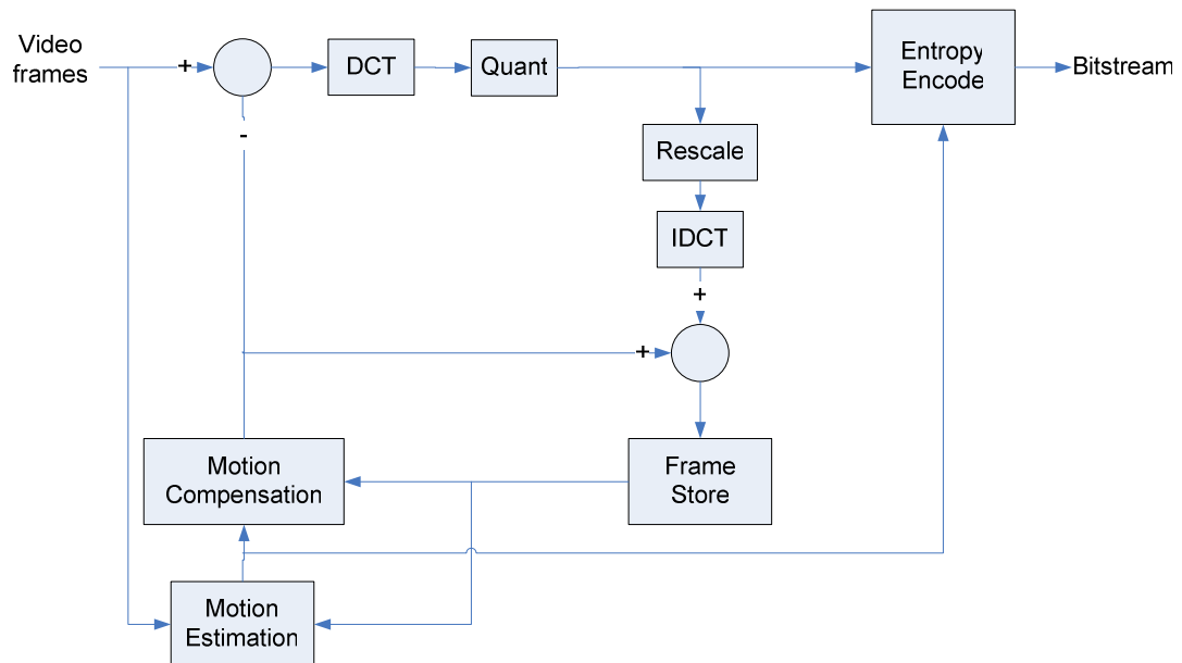
Figure 2-7: Block diagram of H.263 Encoder
