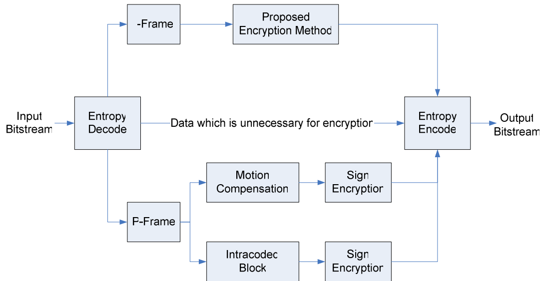
Figure 4-3: General Block Diagram of H.263 Bitstream Encryption
