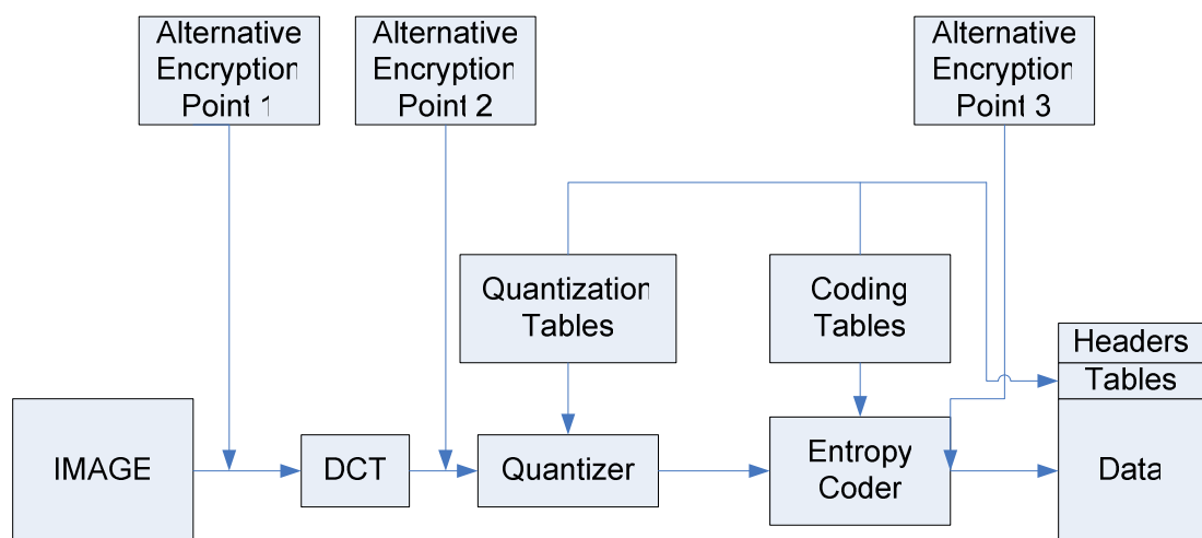
Figure 3-1: Encryption attempts to JPEG encoder
