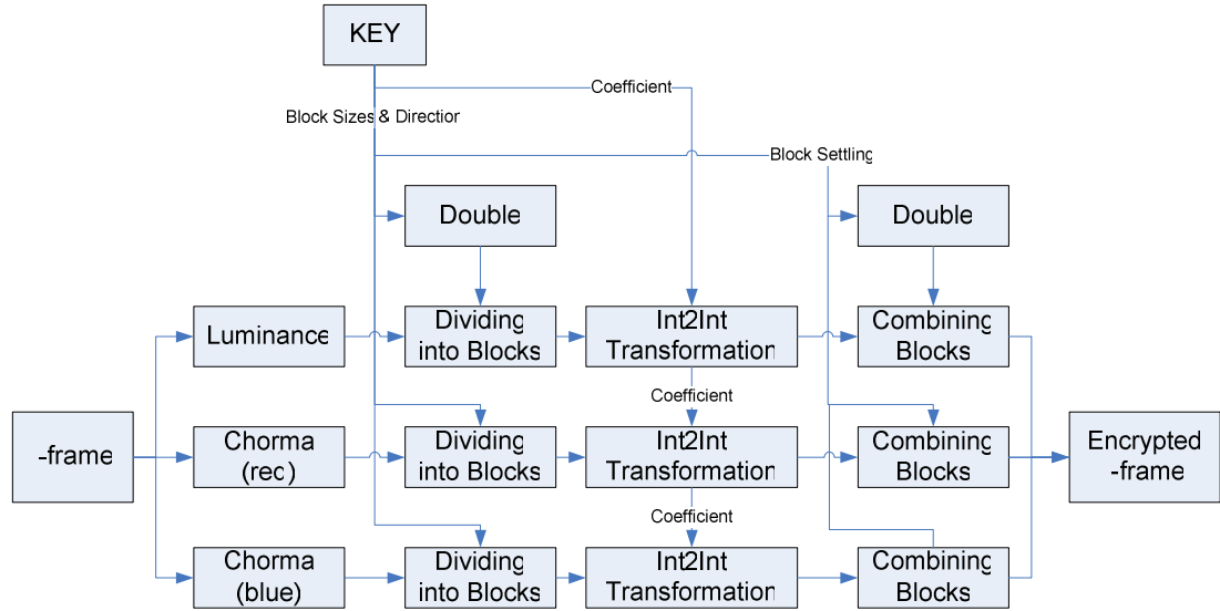
Figure 4-2: Usage of proposed method on I-frames
