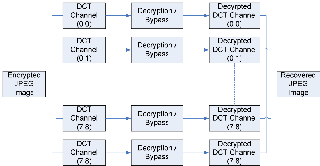
Figure 3-12: Block Diagram of proposed Method (Decryption)
