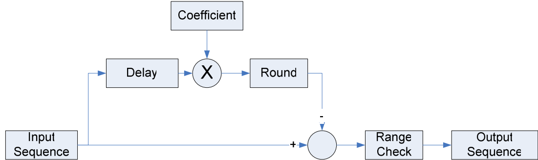
Figure 3-7: Block diagram of integer to integer transformation
