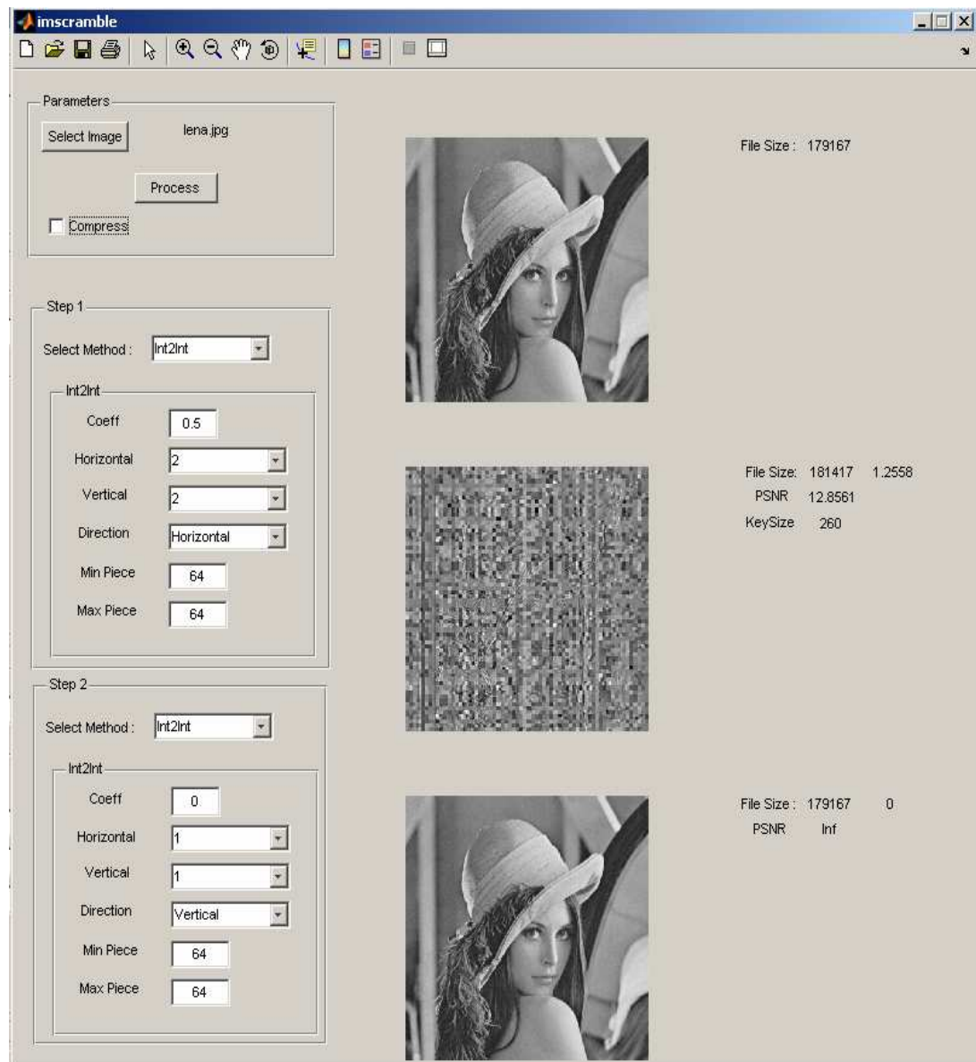
Figure 5-1: MATLAB GUI
