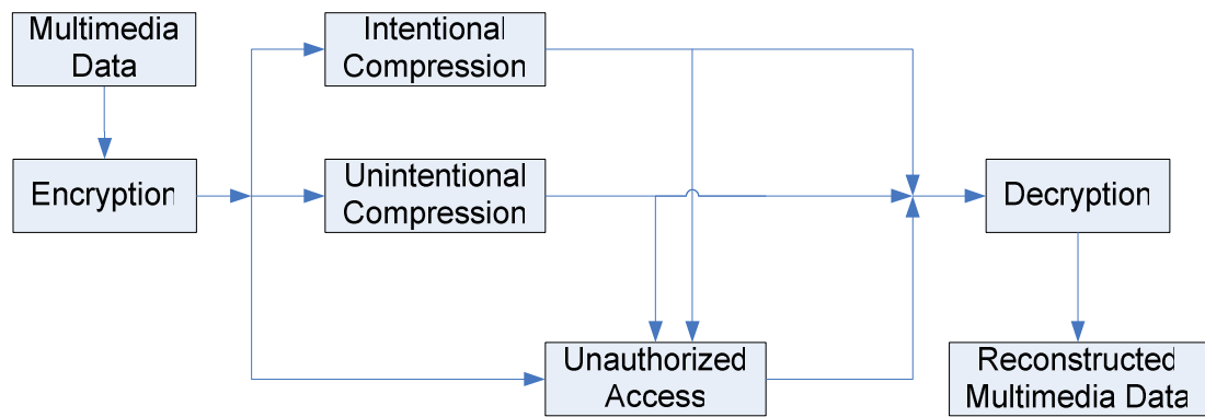
Figure 1-1: Insecure Transmission
