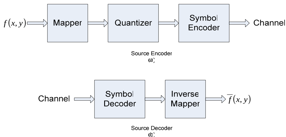
Figure 2-2: (a) Source Encoder Model (b) Source Decoder Model
