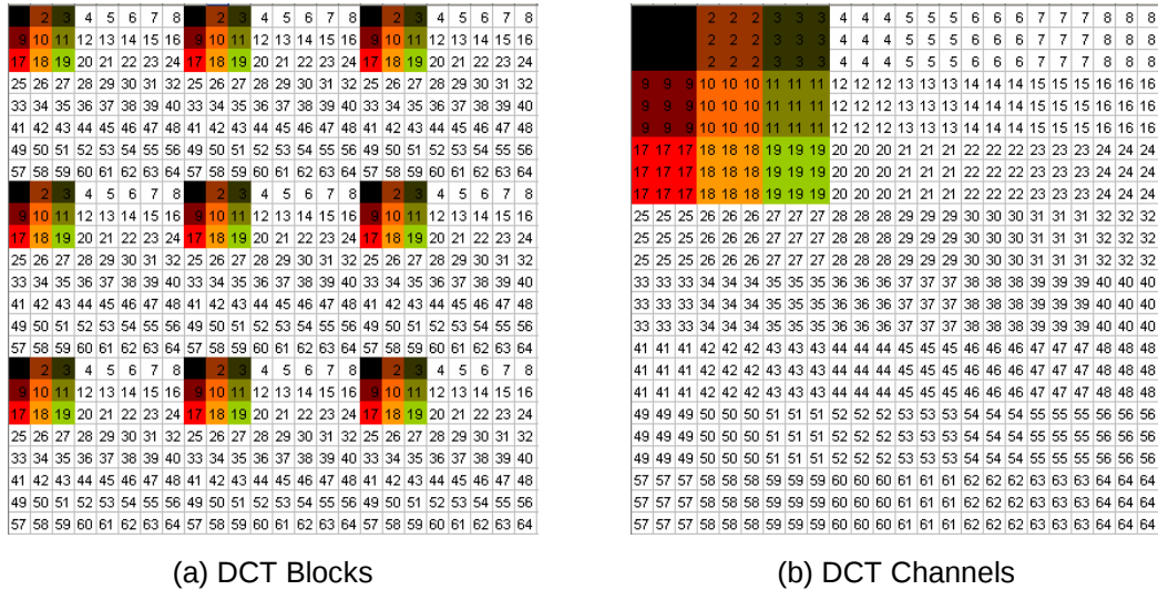
Figure 3-2: Relation between DCT Blocks and DCT Channels
