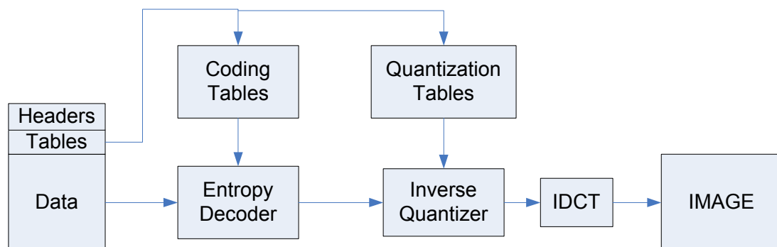
Figure 2-6: Block diagram of DCT-based JPEG decoder
