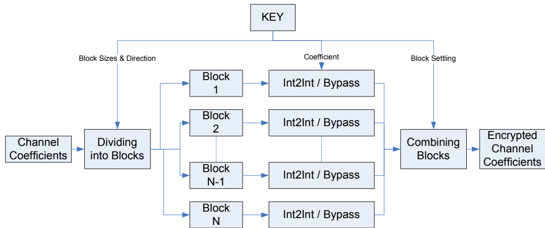
Figure 3-11: Encryption Block
