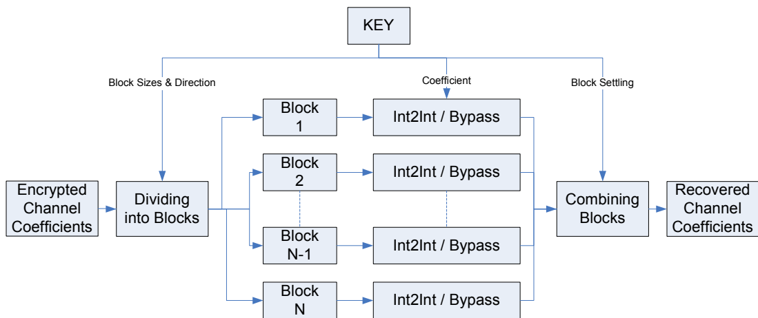
Figure 3-13: Decryption Block
