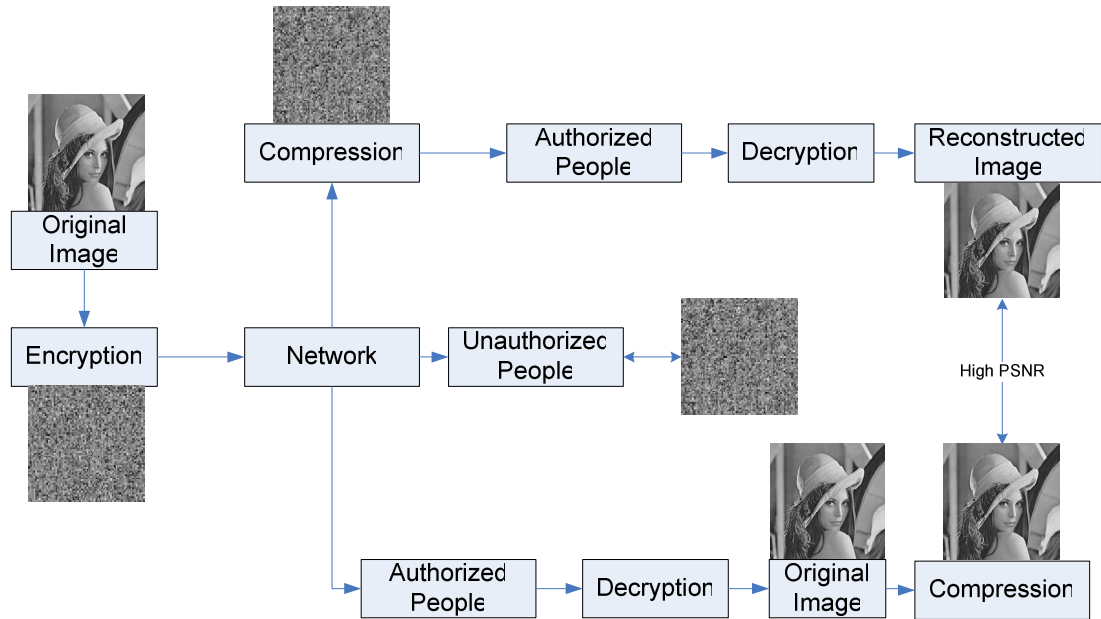
Figure 6-1: Secure Transmission
