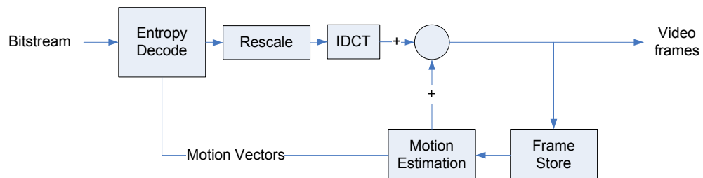
Figure 2-8: Block diagram of H.263 Decoder
