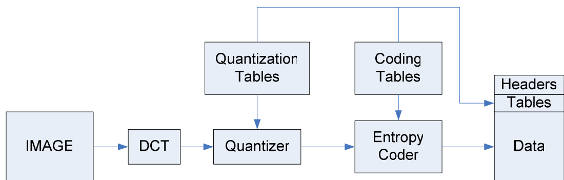
Figure 2-4: Block diagram of DCT-based JPEG encoder
