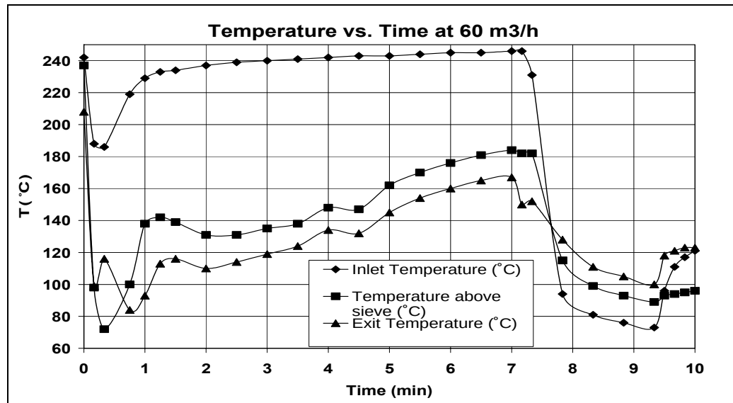
Figure 4.9 Temperature vs. time graph at 60 m³/h – 243°C for 6.5 minute (C7) operation period (330 g wheat germ)
