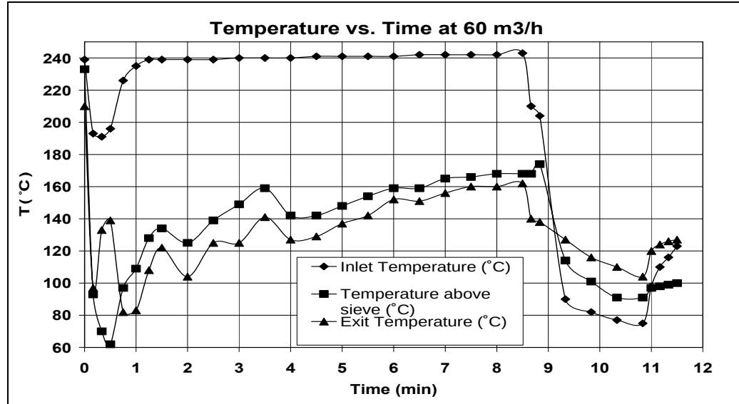
Figure 4.11 Temperature vs. time graph at 60 m³/h – 241°C for 8 minute (C9) operation period (440 g wheat germ)
