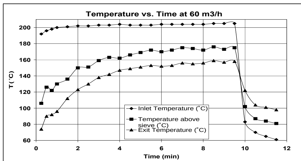
Figure A.5 Temperature vs. time graph at 203°C - 60 m 3 /h for 9.5 minute operation period (330 g wheat germ)
