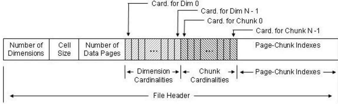
Figure 4.8. File header
