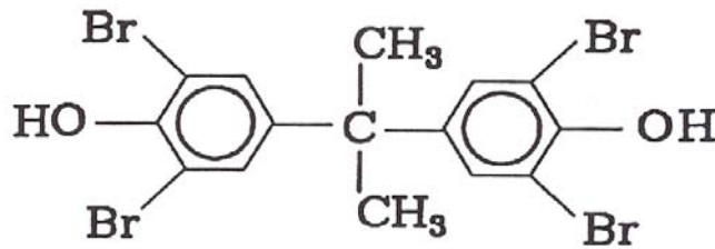
Tetrabromobisfenol A
