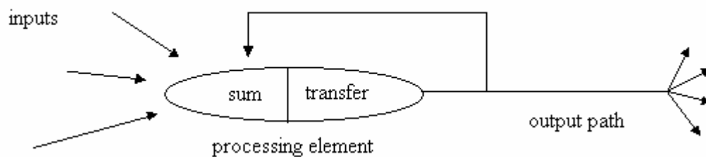
Figure 3.2. An artificial neuron and its structure.
