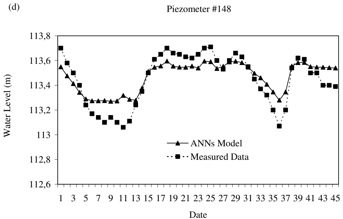
Figure 5.4. Calculated and Measured Water Levels at Piezometers (a) P37, (b) P38, (c) P39, (d) P148 for the Period 28.08.2000-20.05.2002. VALIDATION RUN.
