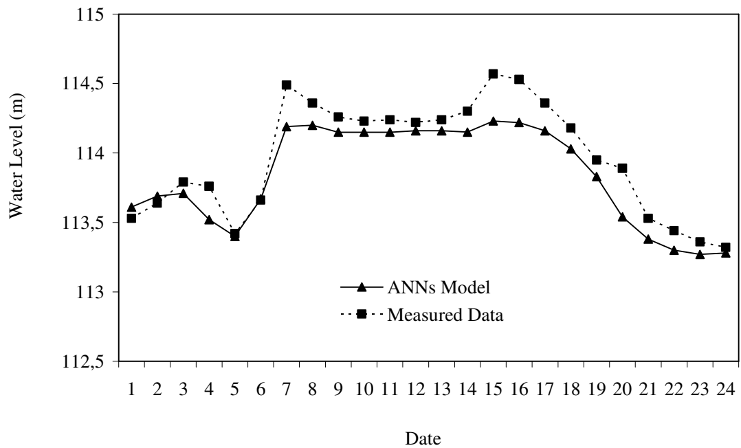
Piezometer #39
