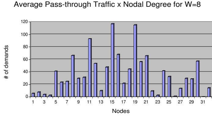
Figure 5.5: The average transit traffic times the degree of the node for each node for W=8
