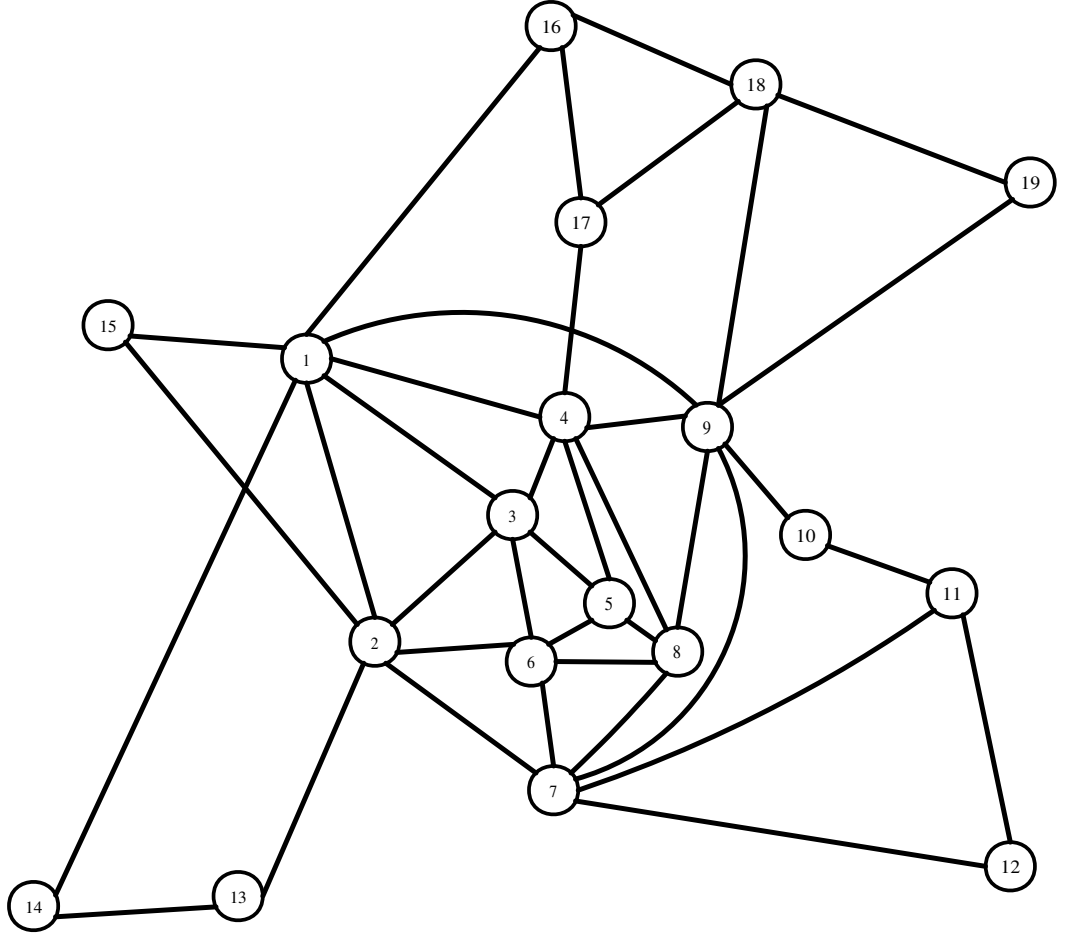
Figure 5.10: 19-node EON
