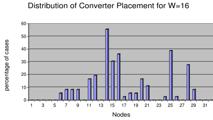
Figure 5.6: The percentage of the cases that a converter is placed at the node for each node for W=16
