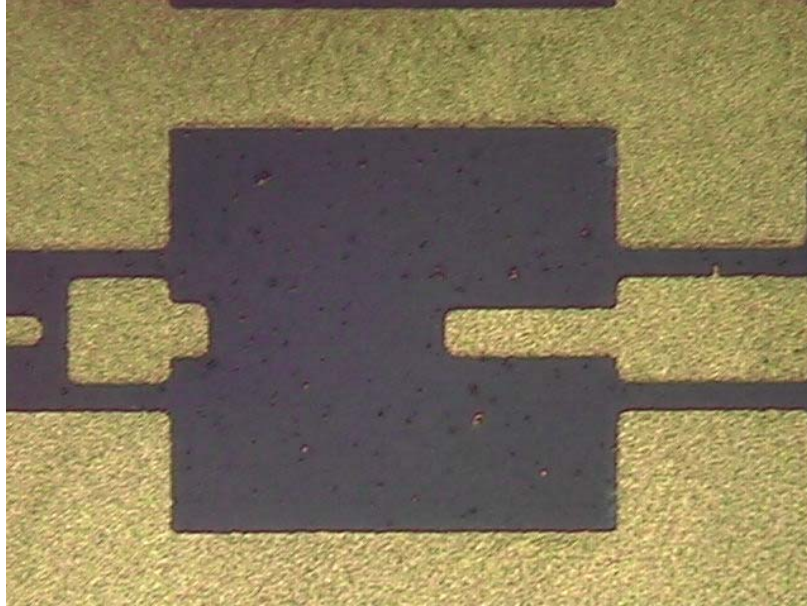
Figure 4-7: Bottom contacts (Al) of the fabricated inductor
