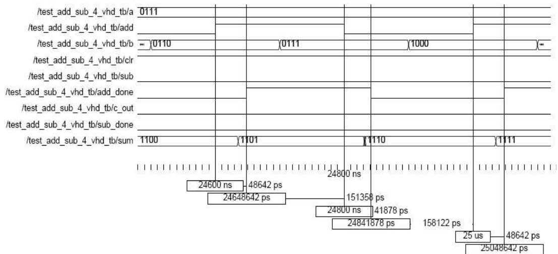
Figure A.15. Simulation Waveform for ADD/SUB (addition) (81 slices)
