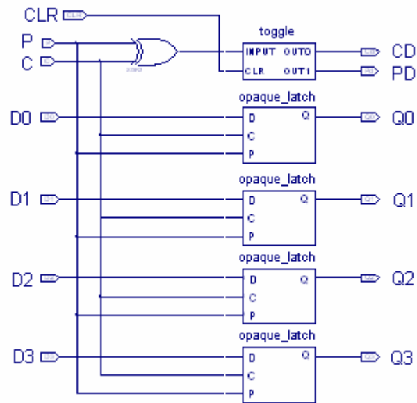
Figure 3.20 Circuit diagram of four-bit register
