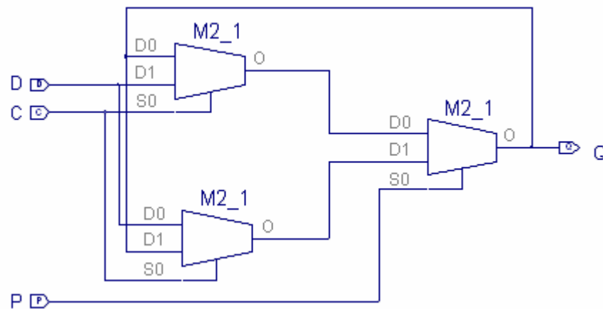
Figure 3.16 OPAQUE LATCH module and its truth function
