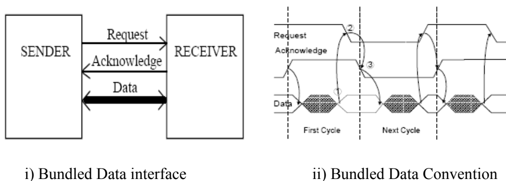
Figure 2.2 Bundled Data Interface and Convention
