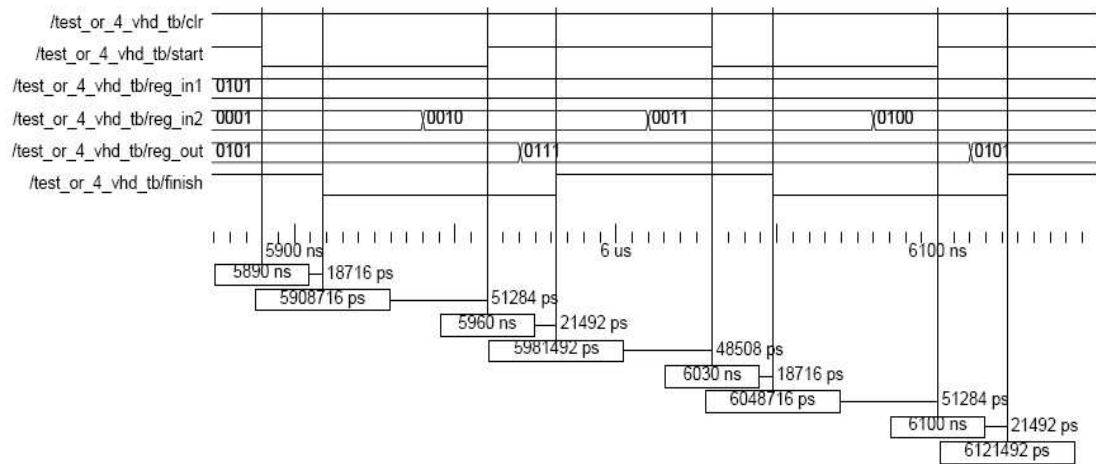
Figure A.9. Simulation Waveform for FOUR-BIT OR (13 slices)
