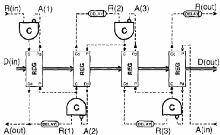
Figure 2.5 Micropipeline without Processing
