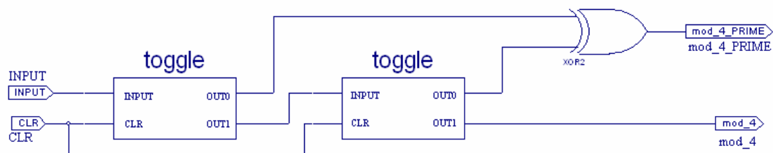
Figure 3.40 Circuit diagram of special modulo-4 counter
