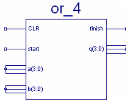
Figure 3.25 Black Box Representation of four-bit OR
