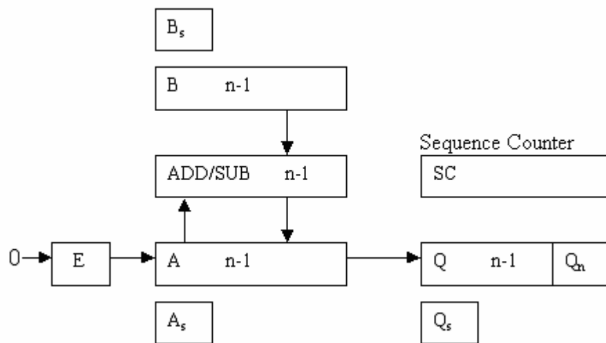
Figure 3.38 Required Hardware for Signed-Magnitude Multiplication
