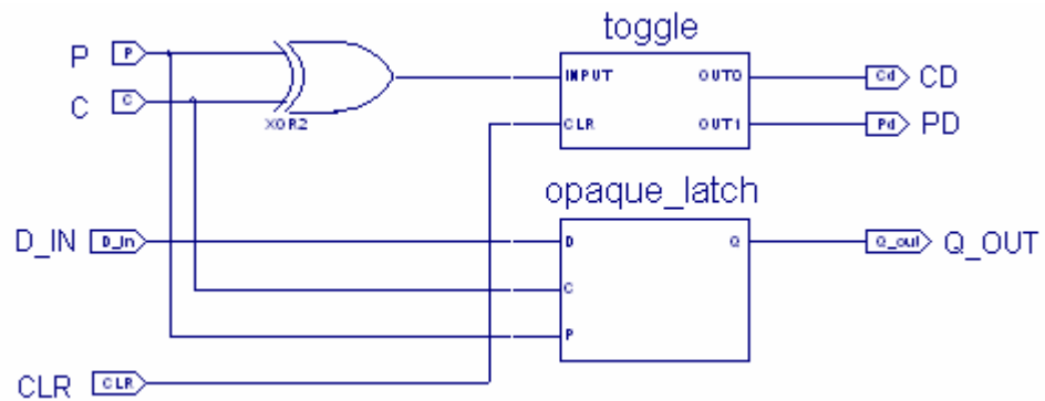
Figure 3.18 Circuit diagram of one-bit register
