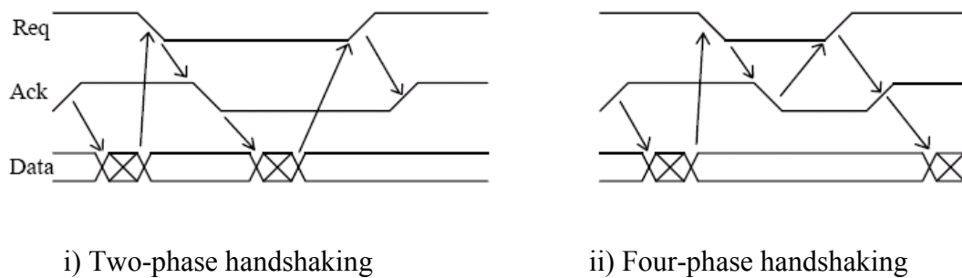
Figure 2.1 Two-phase and four-phase handshakings
