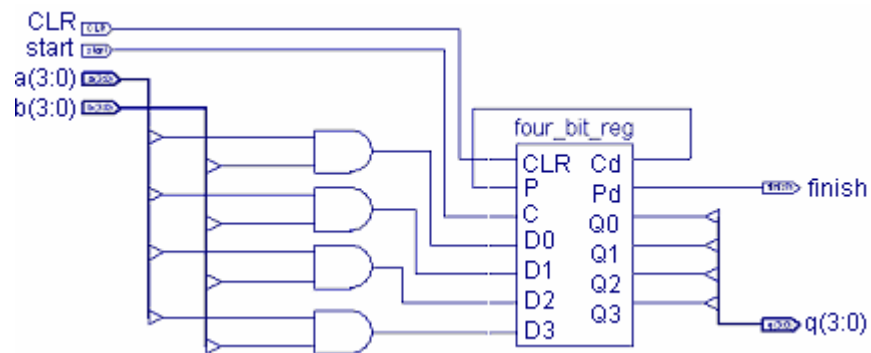
Figure 3.22 Circuit Diagram of four-bit AND
