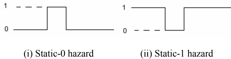
Figure 3.1 Static hazards
