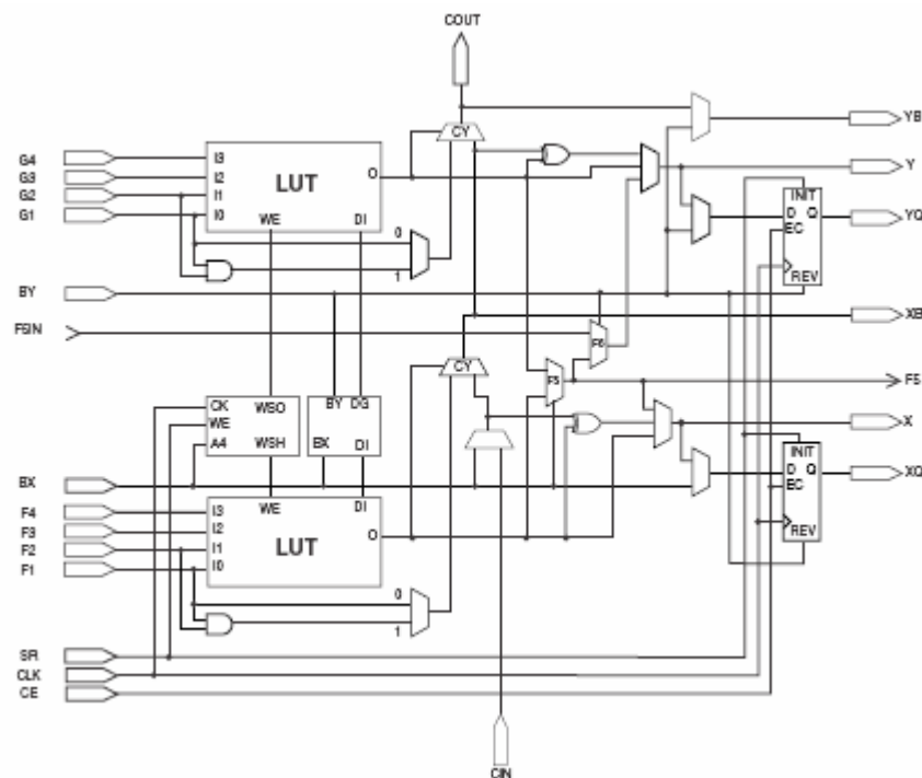
Figure 3.6 Detailed view of Virtex slice
