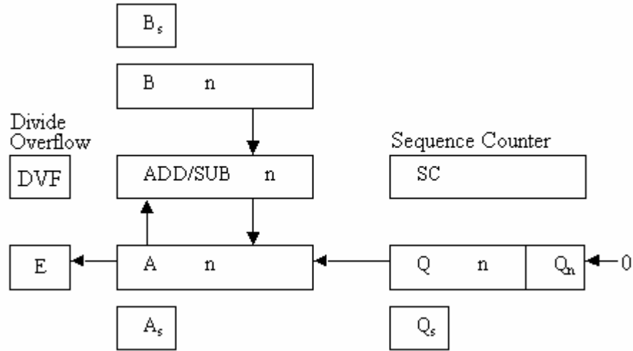
Figure 3.43 Required Hardware for Signed-Magnitude Division
