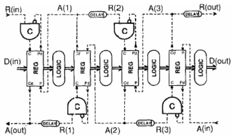
Figure 2.6 Micropipeline with Processing
