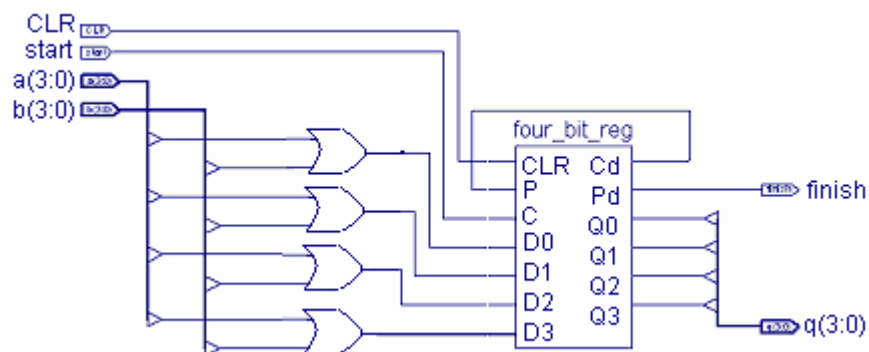
Figure 3.24 Circuit diagram of four-bit OR
