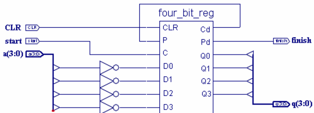
Figure 3.26 Circuit Diagram of four-bit COMPLEMENT
