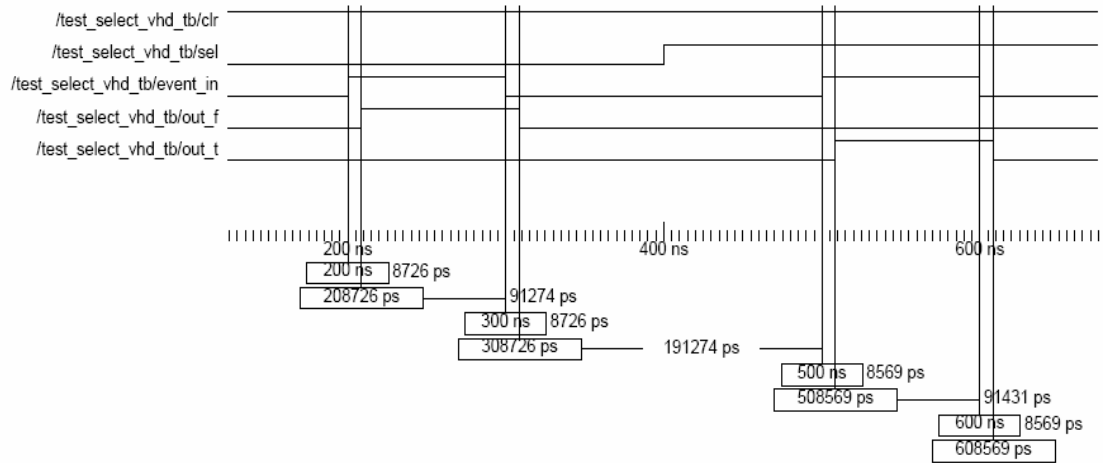
Figure A.3. Simulation Waveform for SELECT (2 slices)
