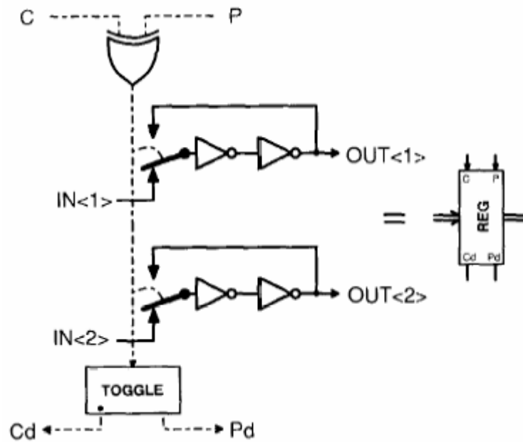
Figure 2.3 Latches Used as an Event Controlled Storage Register
