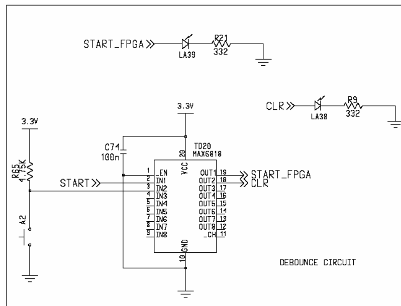
Figure B.5 Debounce Circiut
