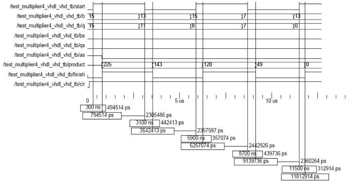
Figure A.17. Simulation Waveform for MULTIPLIER (232 slices)
