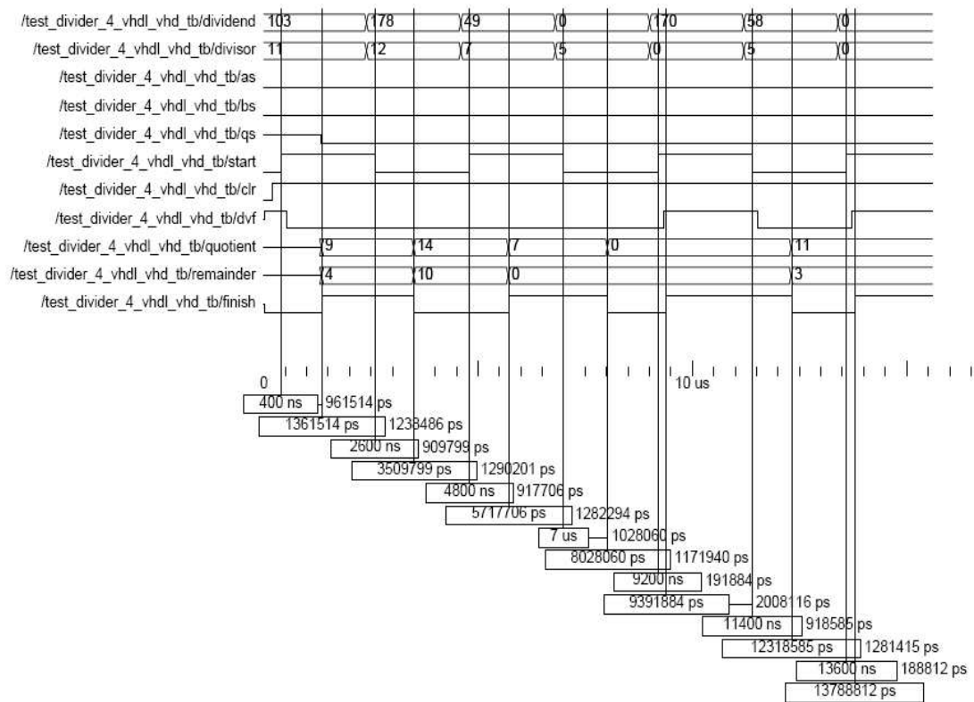
Figure A.18. Simulation Waveform for DIVIDER (328 slices)
