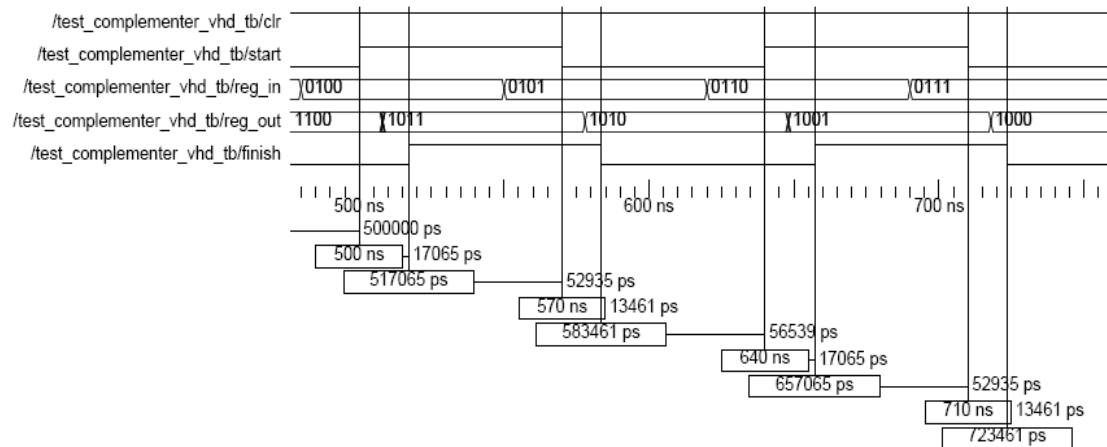
Figure A.10. Simulation Waveform for FOUR-BIT COMPLEMENT (13 slices)
