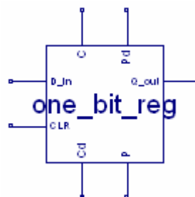
Figure 3.19 Black Box Representation of one-bit register
