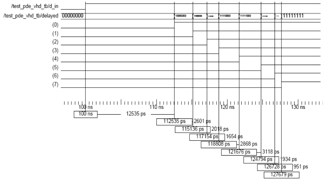
Figure A.11. Simulation Waveform for PDE (16 slices)
