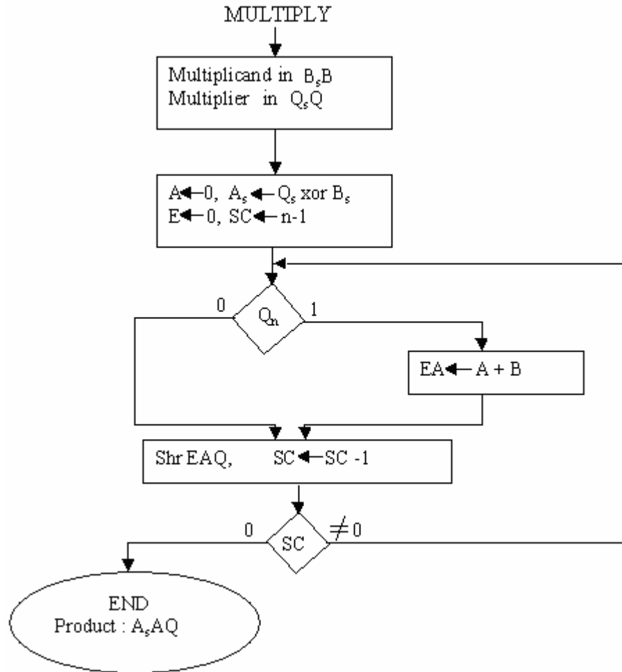
Figure 3.39 Hardware Flow Chart for Multiplication
