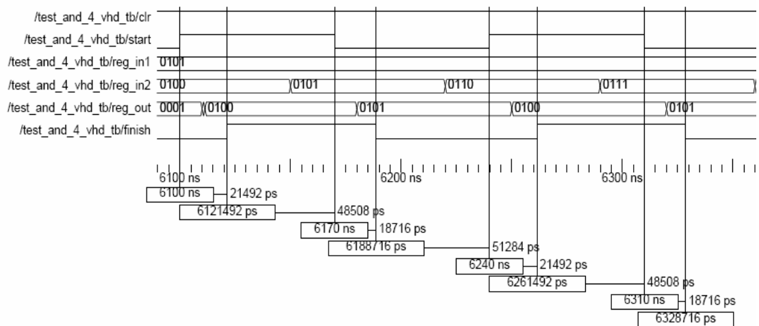
Figure A.8. Simulation Waveform for FOUR-BIT AND (13 slices)
