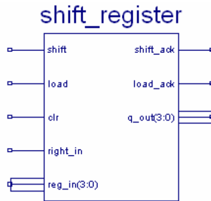
Figure 3.33 Black Box Representation of loadable shift register (type 2)
