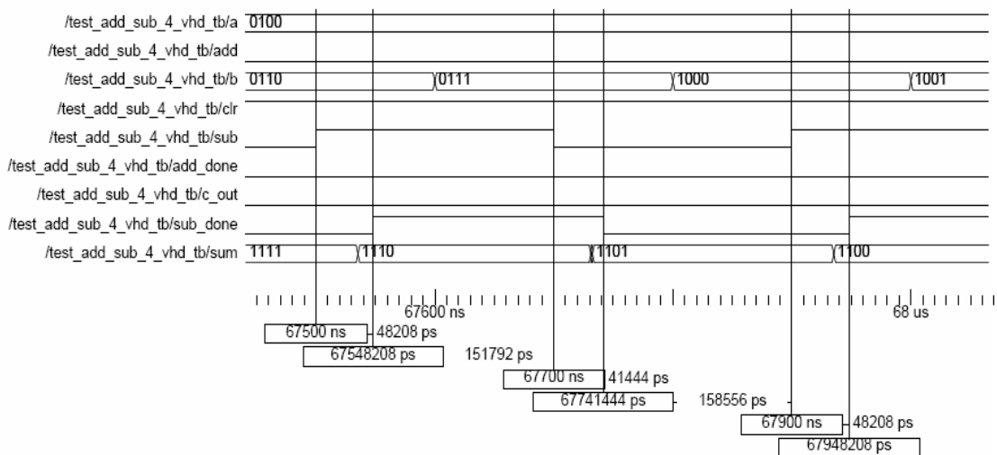
Figure A.16. Simulation Waveform for ADD/SUB (subtraction) (81 slices)
