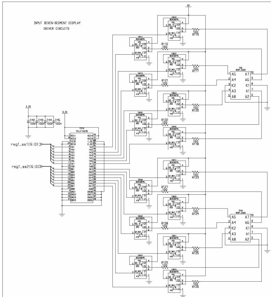
Figure B.14 Input Seven-Segment Displays and Driver Circuits
