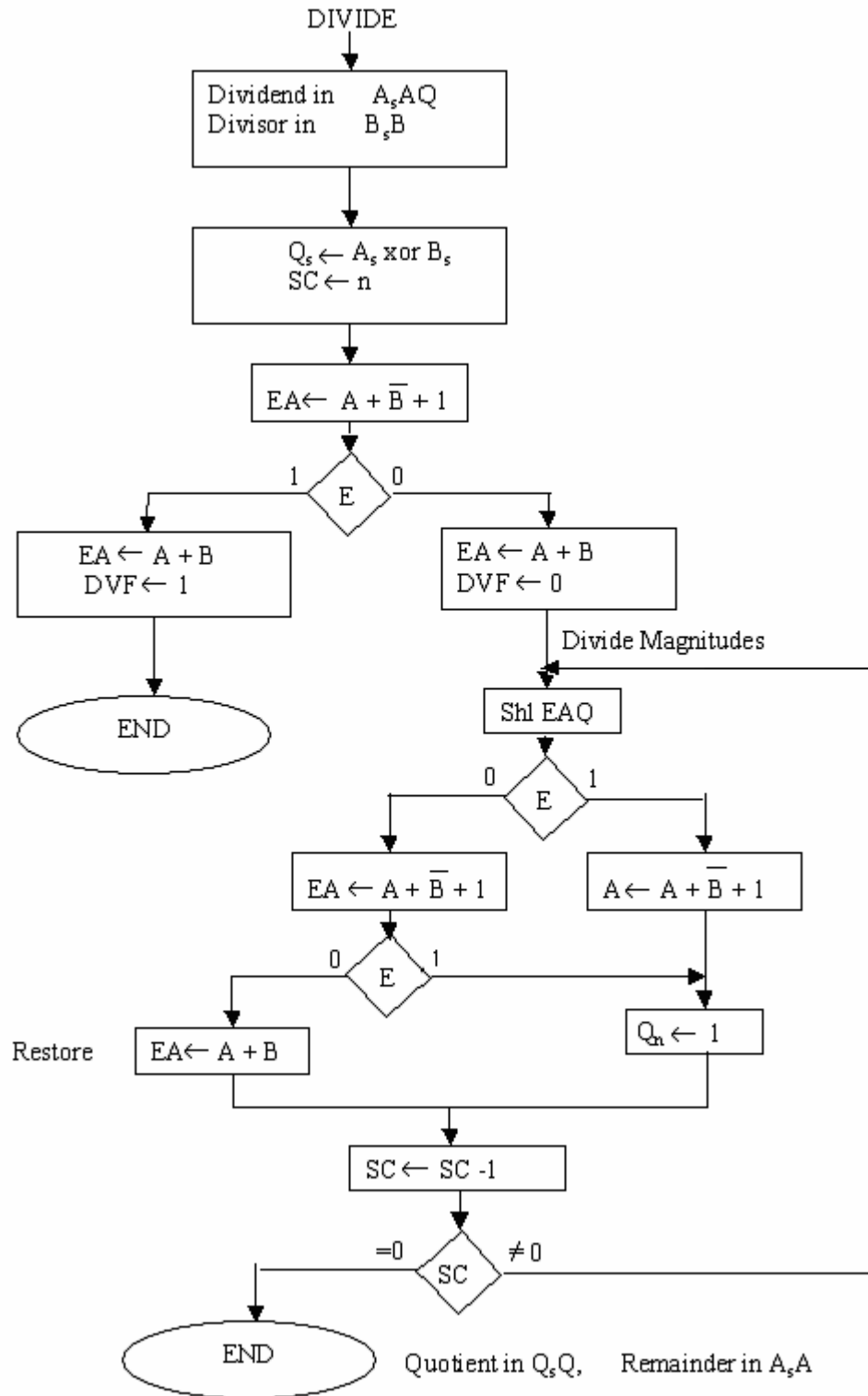
Figure 3.44 Hardware Flow Chart for Signed-Magnitude Division
