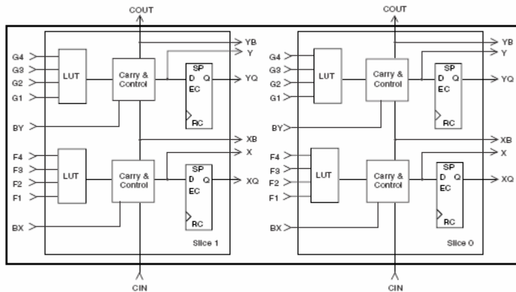
Figure 3.5 2-Slice Virtex CLB
