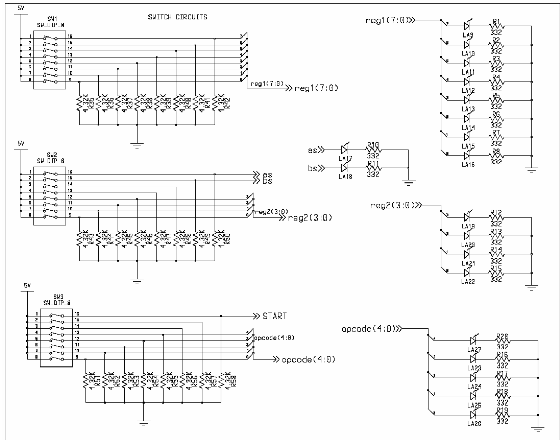
Figure B.4 Input Switches and LEDs
