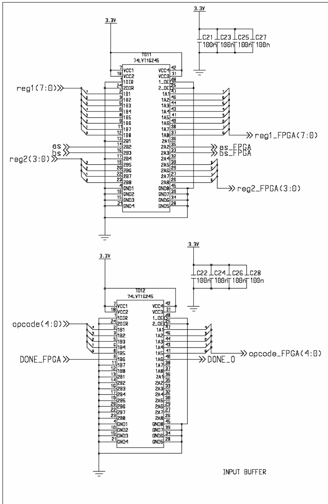
Figure B.6 Input Buffers
