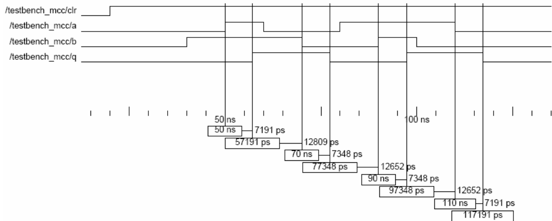
Figure A.1. Simulation Waveform for Muller-C (1 slice)
