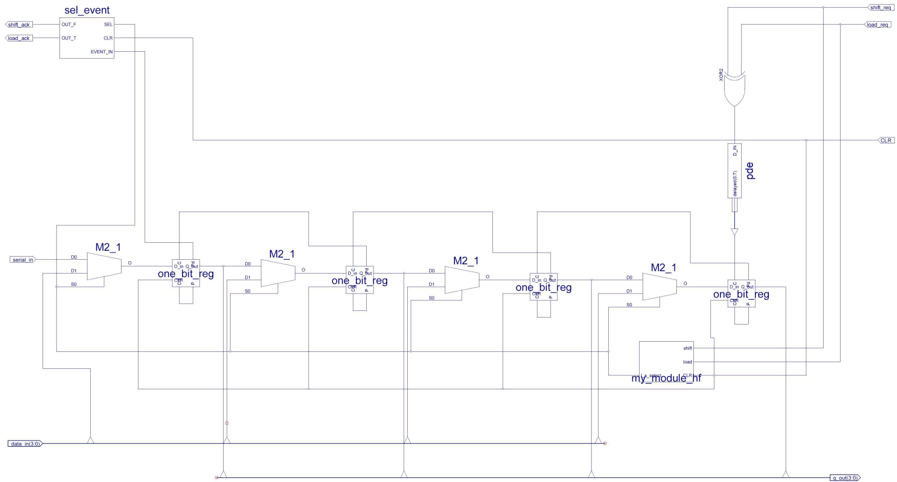
Figure 3.30 Circuit diagram of loadable shift register (type 1)
