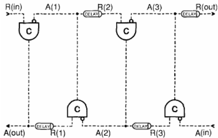
Figure 2.4 Control Circuit for a Micropipeline
