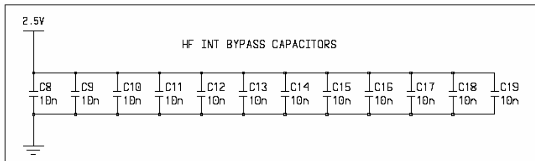
Figure B.8 High Frequency Integrated Circuit Bypass Capacitors
