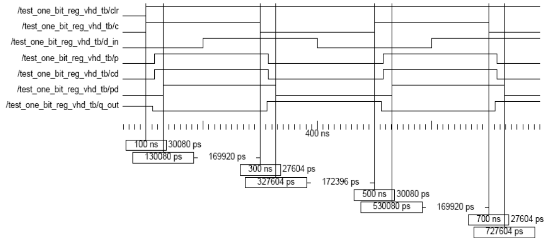
Figure A.6. Simulation Waveform for ONE-BIT REGISTER (6 slices)
