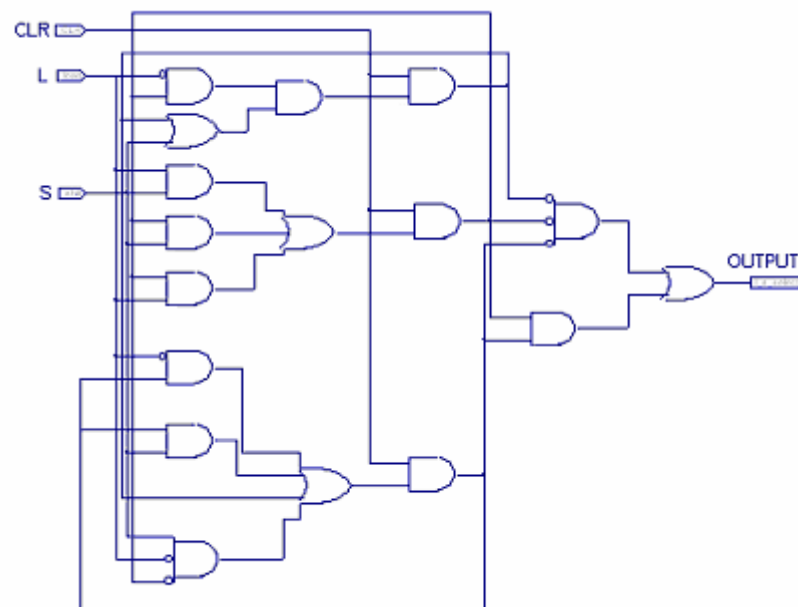
Figure 3.34 Circuit diagram of my_module_hf
