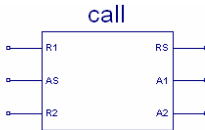
Figure 3.15 Black Box Representation of CALL element
