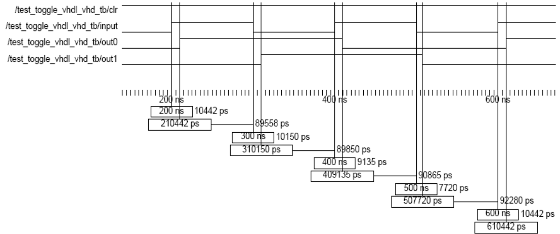
Figure A.2. Simulation Waveform for TOGGLE (4 slices)
