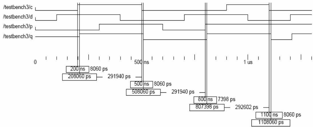
Figure A.5. Simulation Waveform for OPAQUE LATCH (1 slice)
