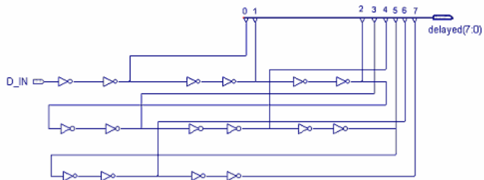
Figure 3.28 Circuit diagram of PDE
