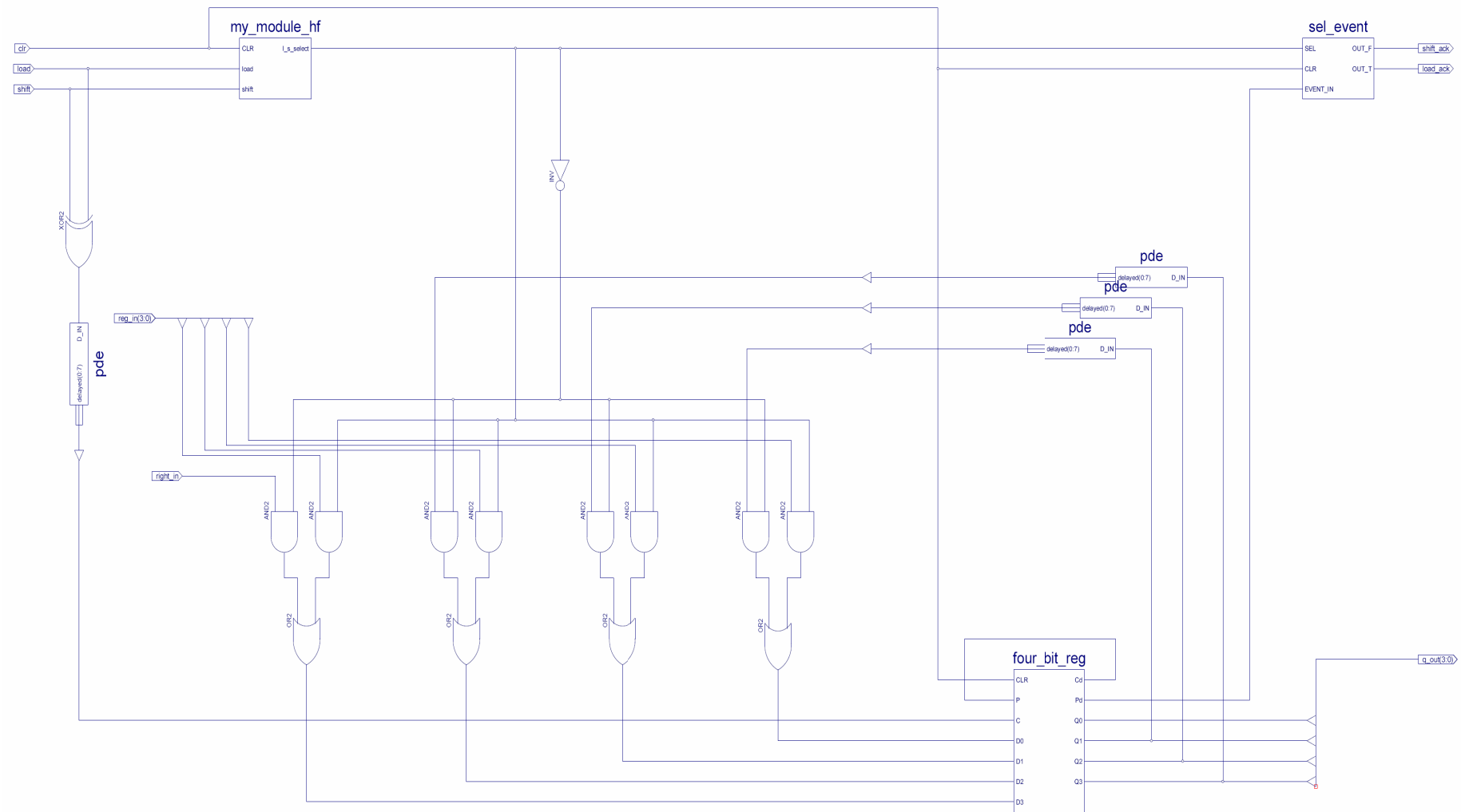
Figure 3.32 Circuit diagram of loadable shift register (type 2)
