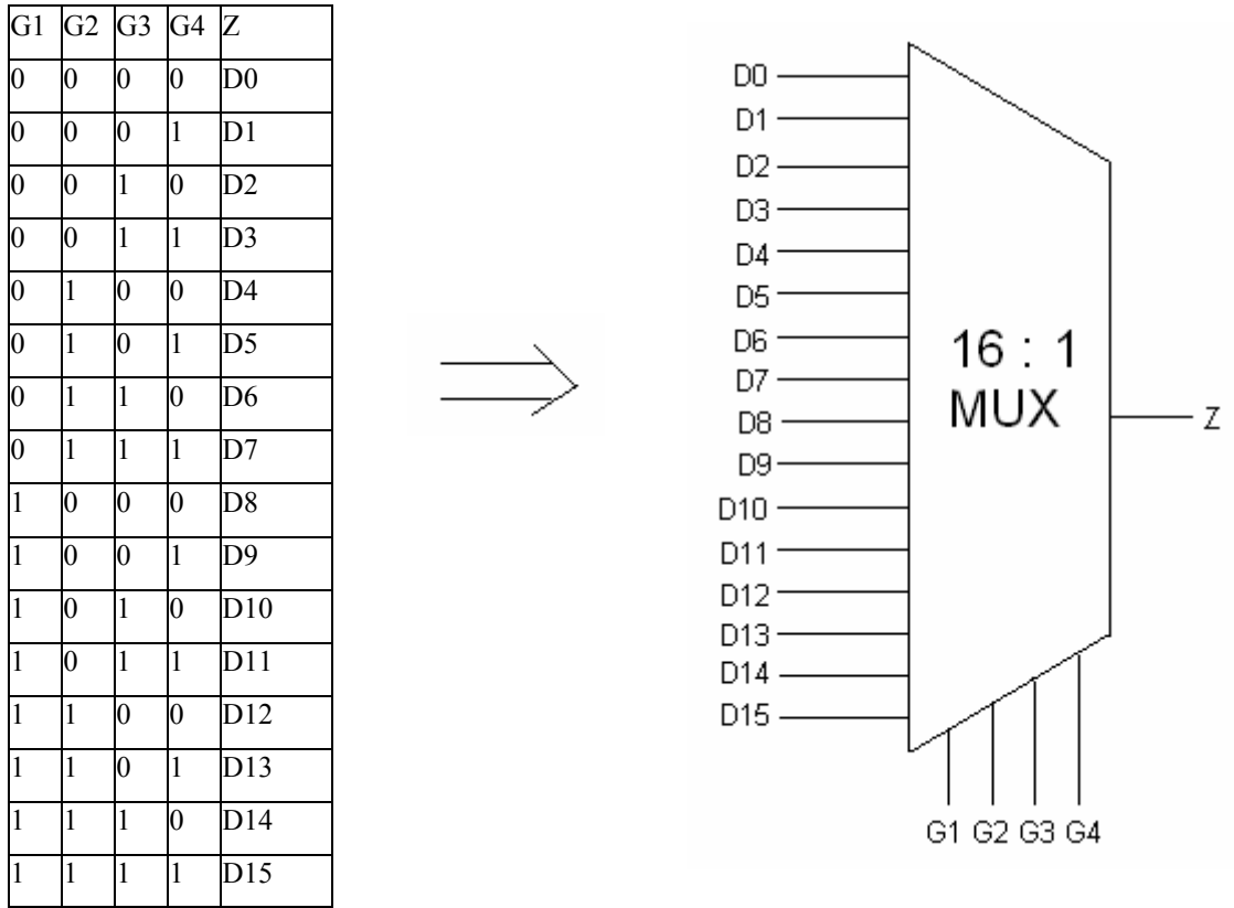
Figure 3.7 LUT-Based Implementation
