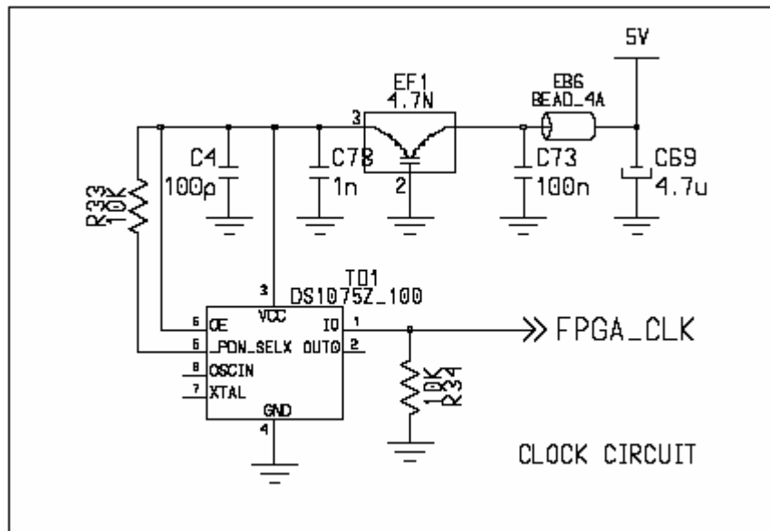
Figure B.12 Clock Circuit for Synchronous Operation Option
