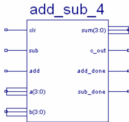
Figure 3.37 Black Box Representation of ADD/SUB module
