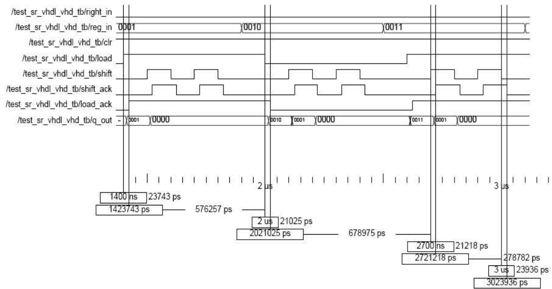
Figure A.13. Simulation Waveform for LOADABLE SHIFT REGISTER (Type 2) (34 slices)
