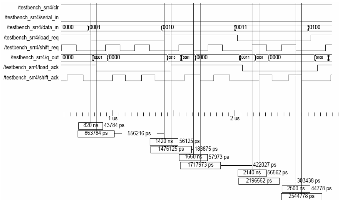
Figure A.12. Simulation Waveform for LOADABLE SHIFT REGISTER (Type 1) (44 slices)
