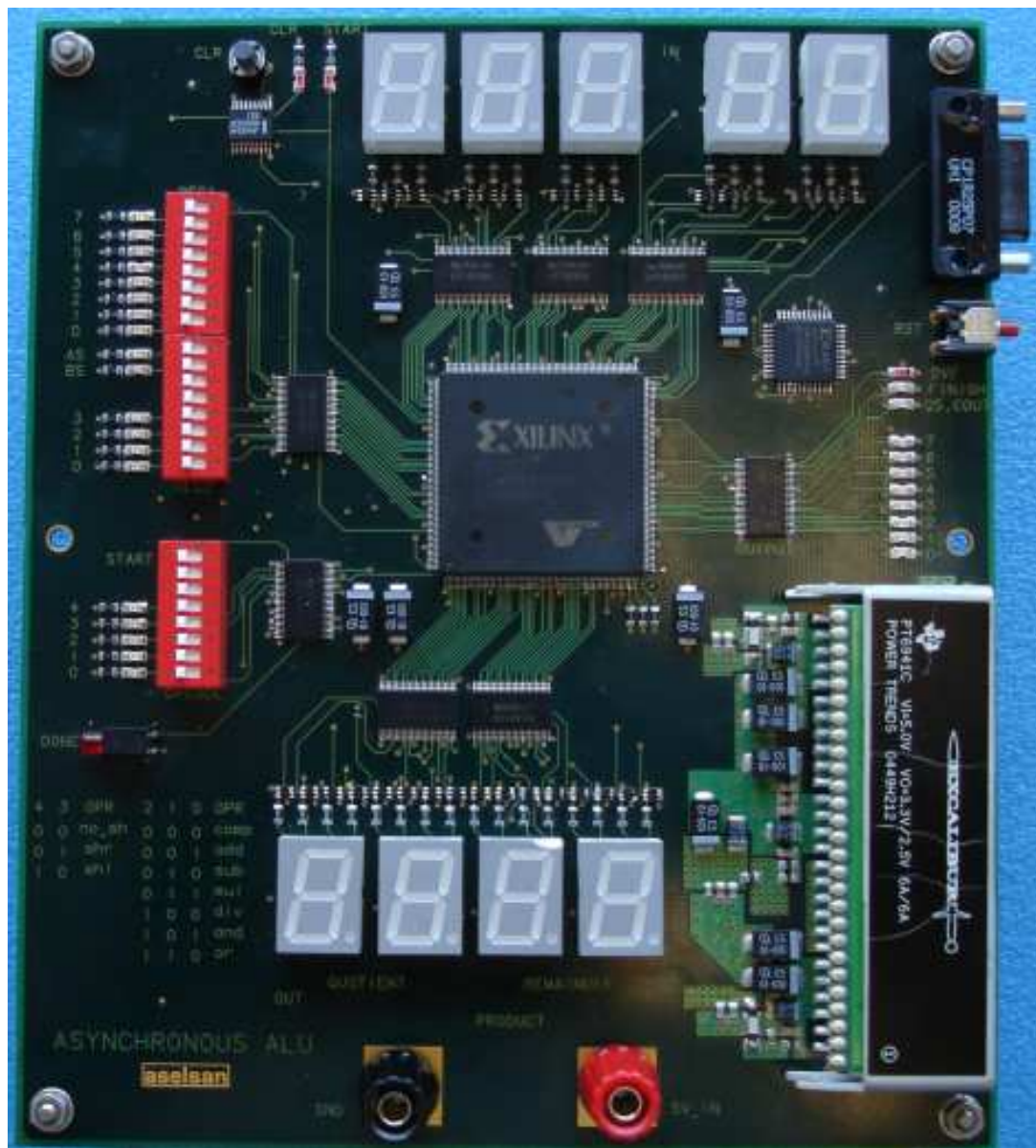
Figure 5.2 Top view of the board
