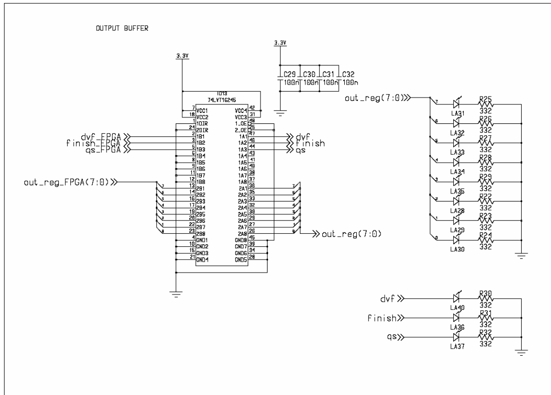
Figure B.7 Output Buffer and LEDS
