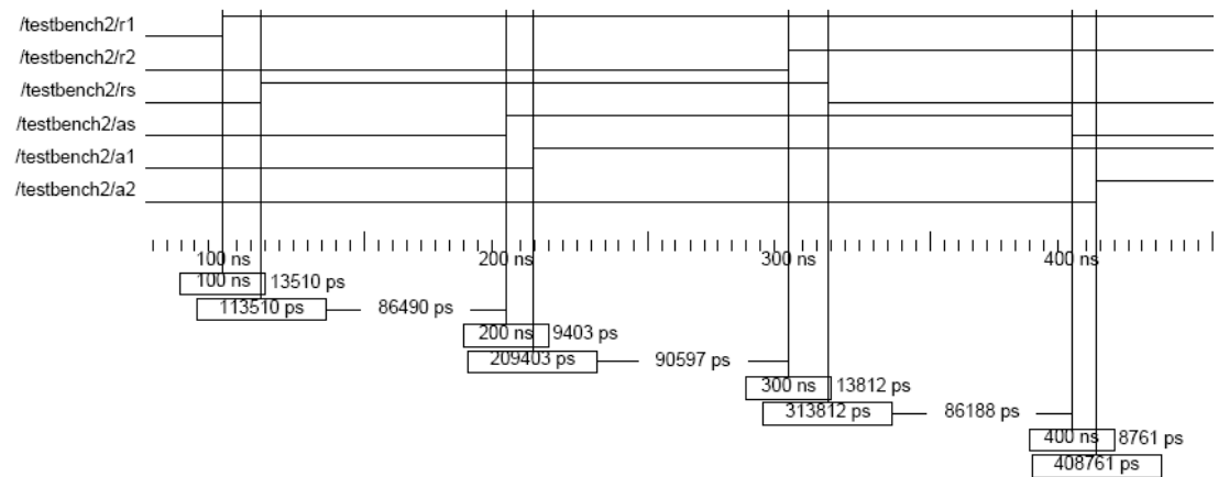
Figure A.4. Simulation Waveform for CALL (2 slices)
