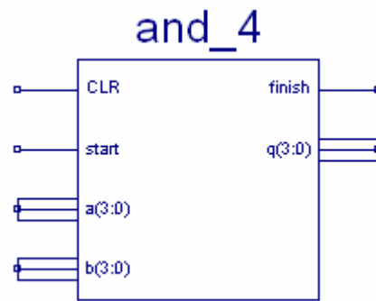
Figure 3.23 Black Box Representation of four-bit AND
