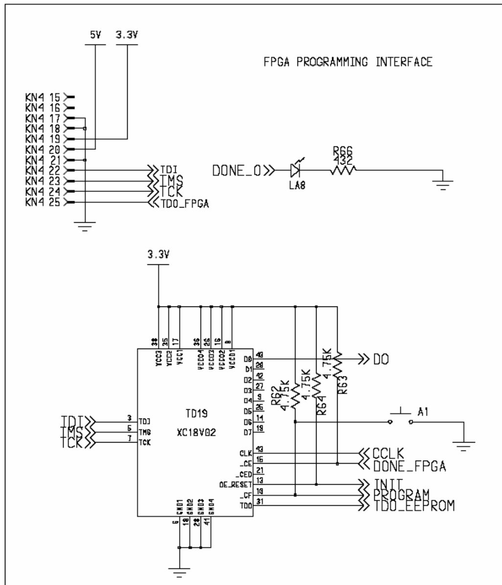
Figure B.11 FPGA Programming Interface
