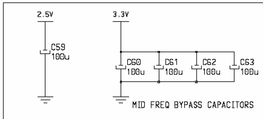
Figure B.10 Mid-frequency Bypass Capacitors
