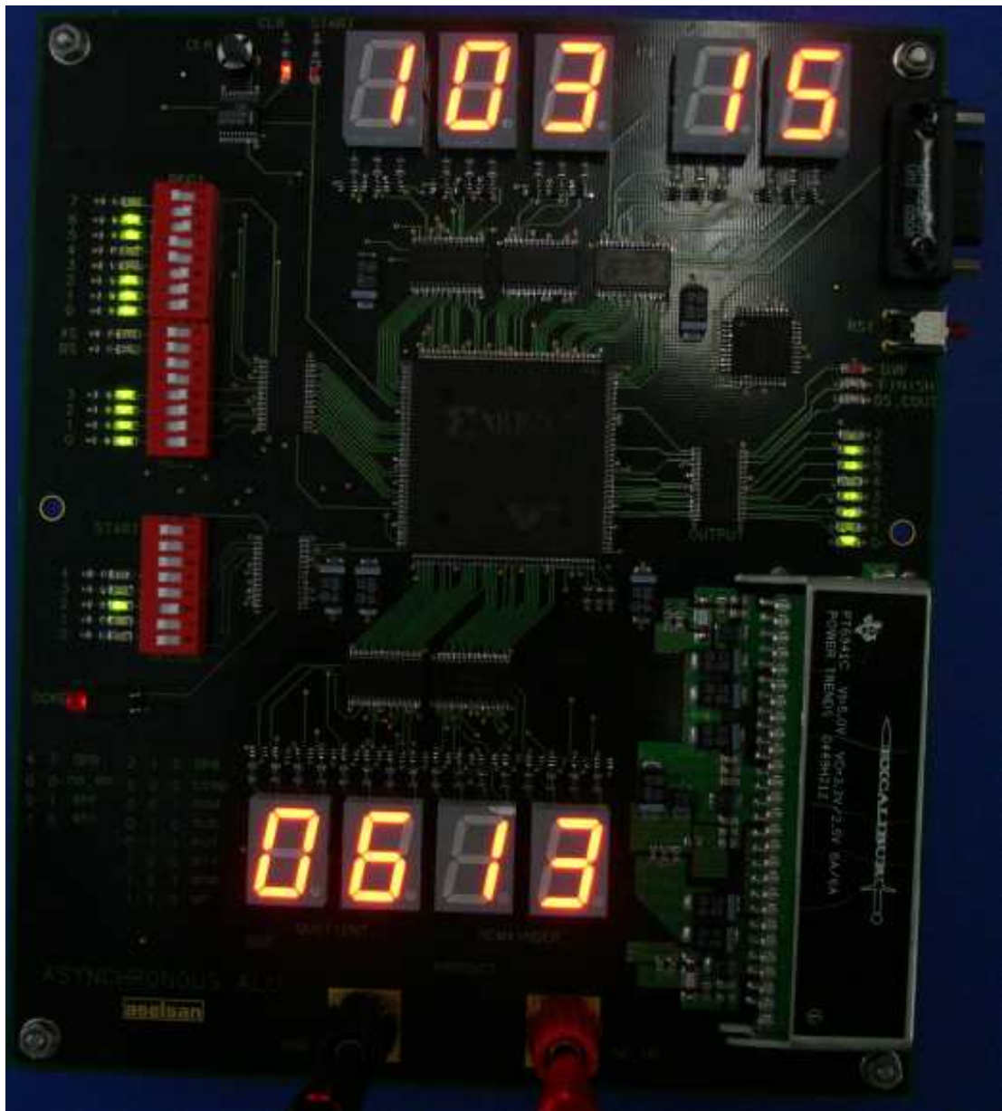
Figure 5.3 A sample operation (103/15, quotient: 6, remainder:13)
