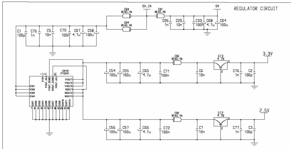
Figure B.1 Regulator Circuit
