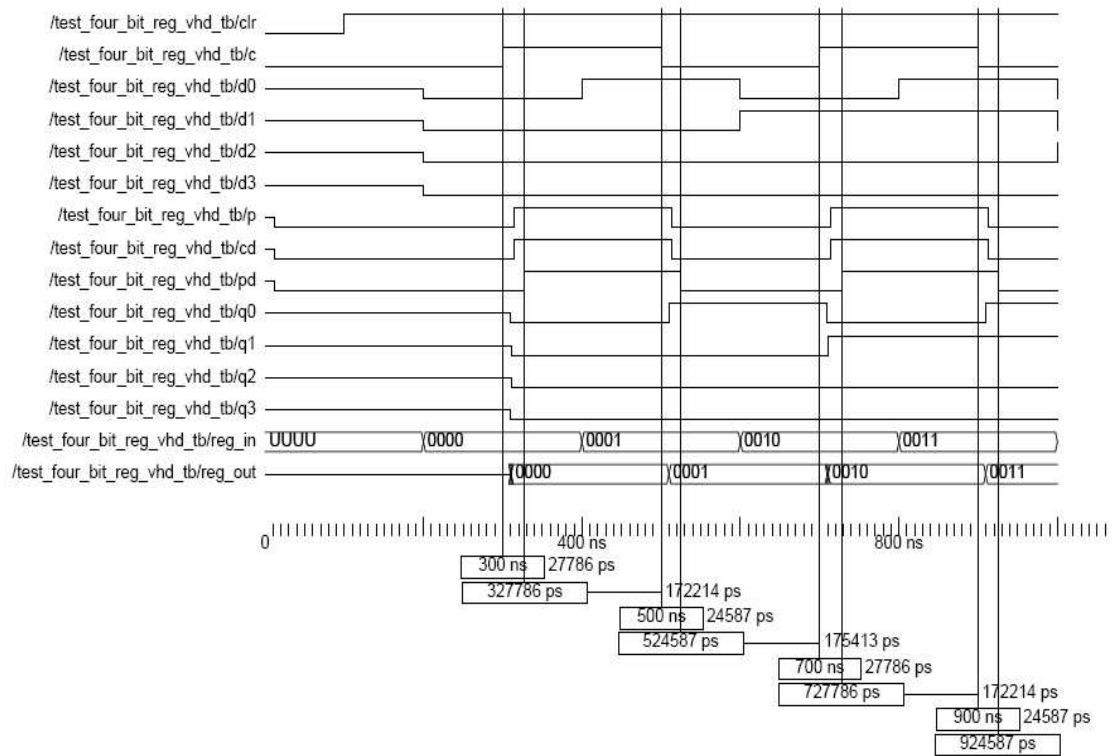
Figure A.7. Simulation Waveform for FOUR-BIT REGISTER (9 slices)
