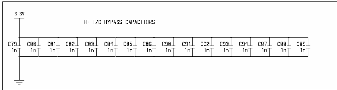
Figure B.9 High Frequency I/O Bypass Capacitors
