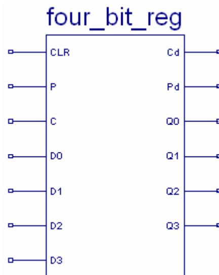
Figure 3.21 Black Box Representation of four-bit register
