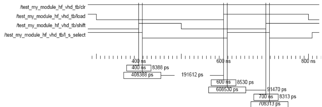
Figure A.14. Simulation Waveform for MY_MODULE_HF (2 slices)
