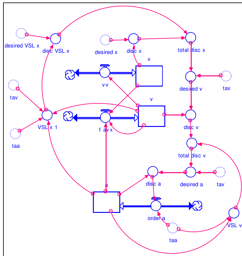
Figure 3.15. Stock-flow diagram of a third order indirect stock control structure
