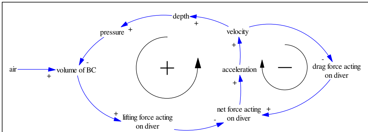
Figure 3.3. Causal loop diagram of ScubaSim when friction is present
