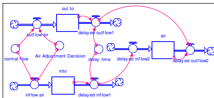
Figure 4.5. Material delay structure used in ScubaSim
