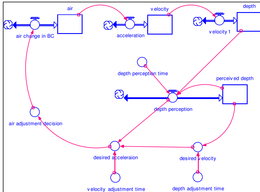
Figure 3.28. Model structure with depth information delay
