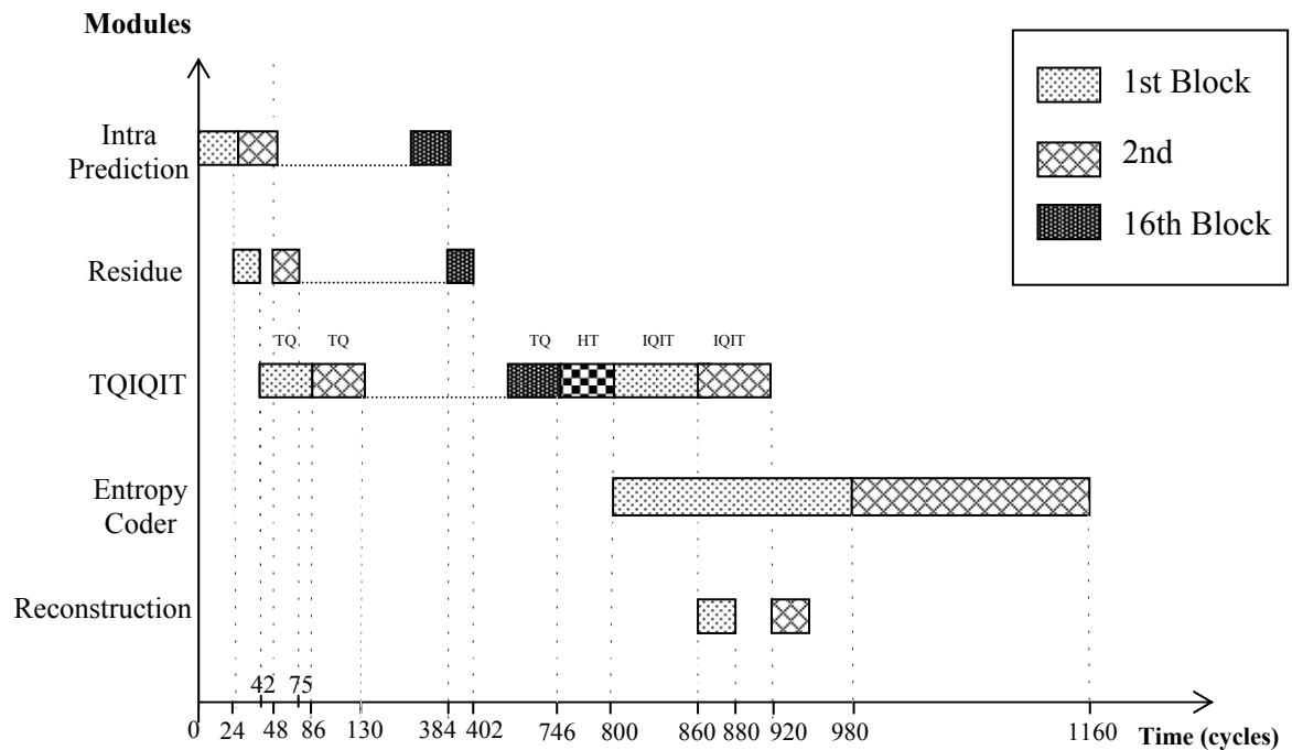
Figure 4.9 Coder Hardware Scheduling for 16x16 Intra Modes
