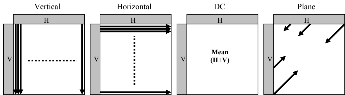
Figure 2.5 16x16 Luma Prediction Modes
