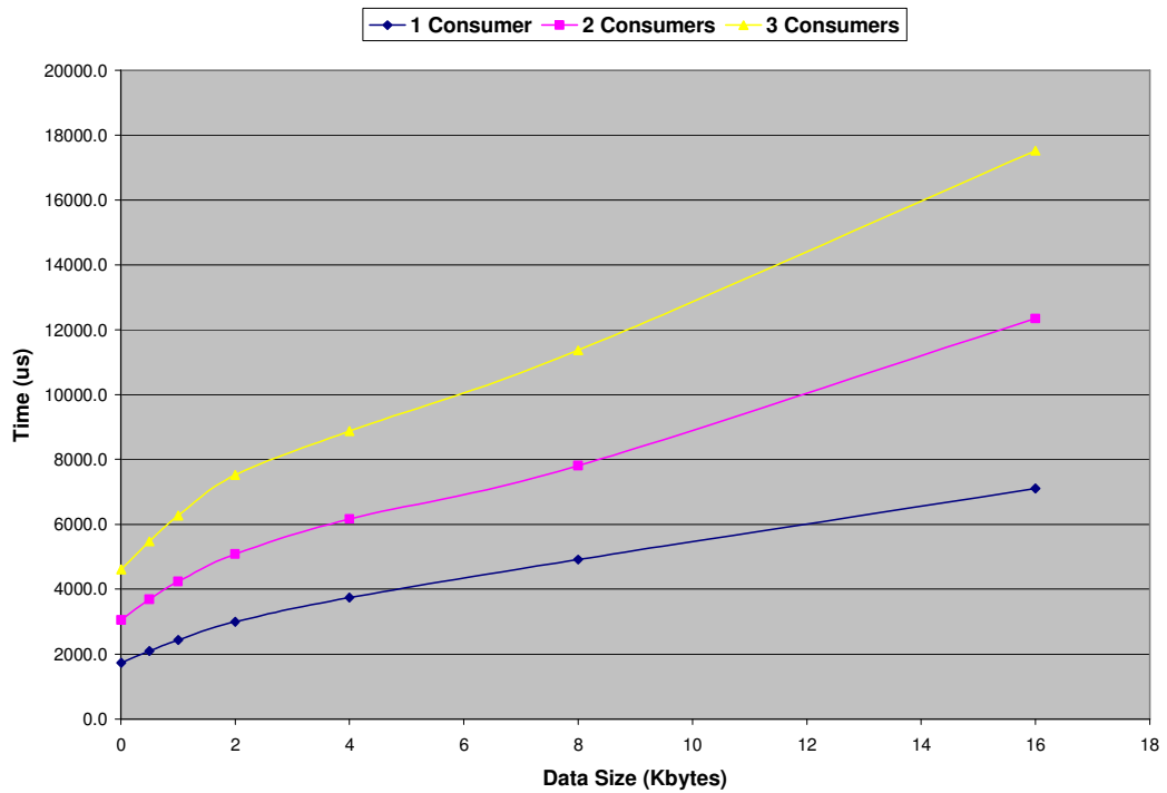
Figure 26 Performance of CDDS for different number of consumers
