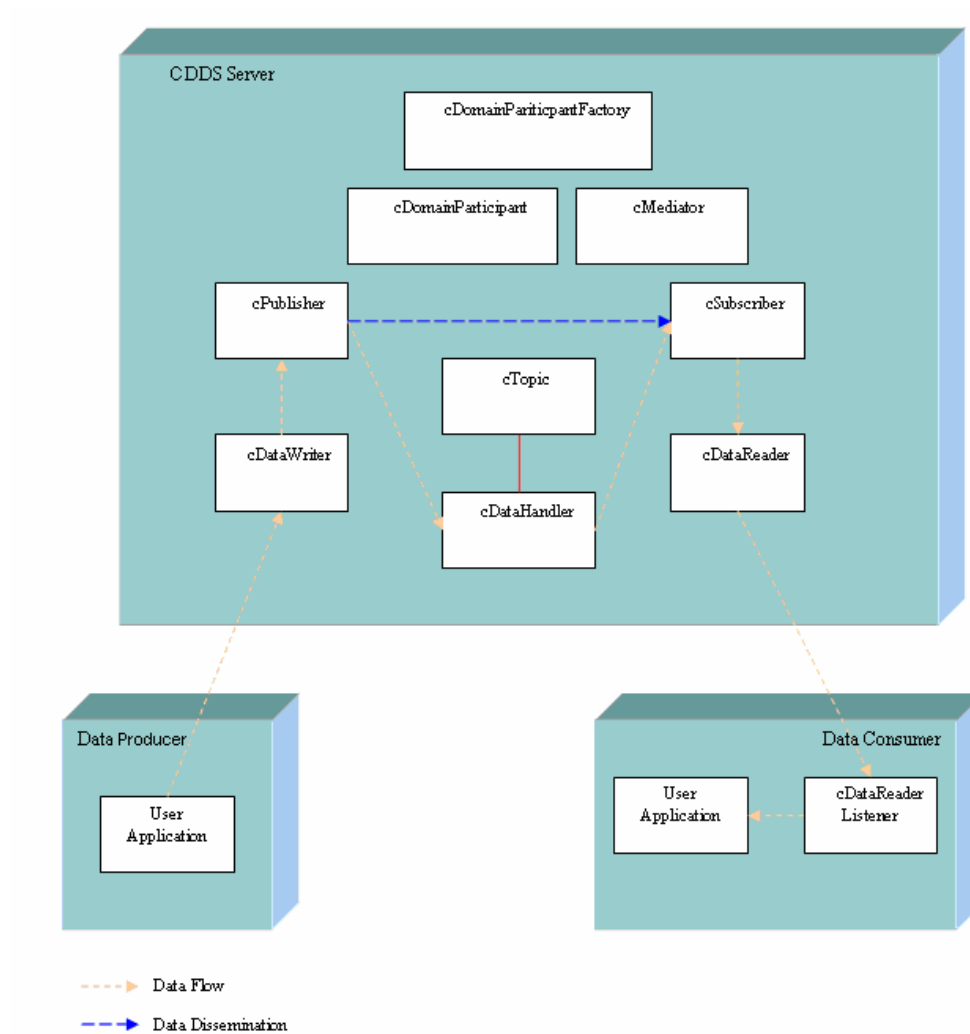
Figure 11 CDDS Participants Deployment Diagram
