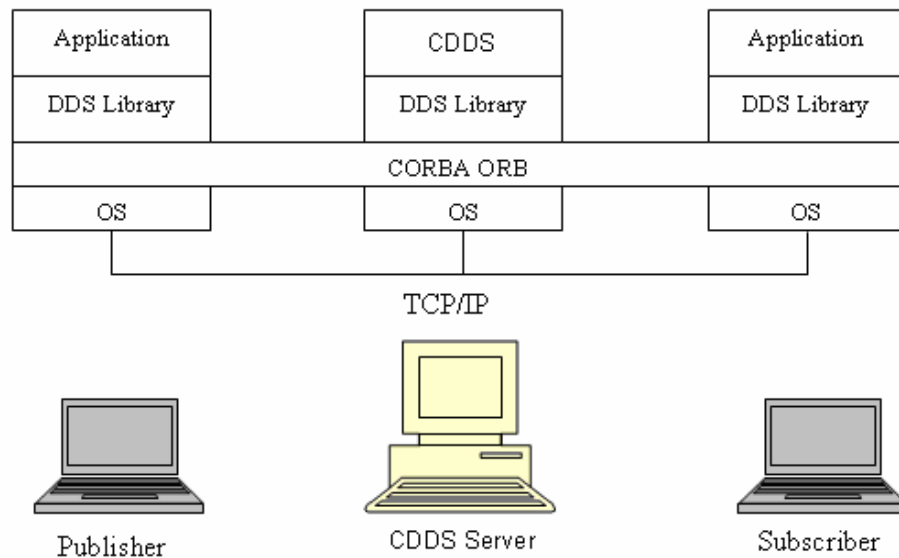
Figure 19 Testbed Configuration
