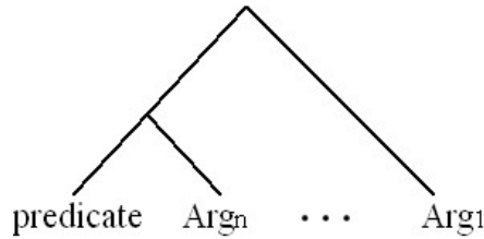
Figure 5.1: Predicate-argument structure
