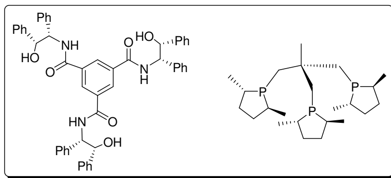
Figure 8. Examples to C_3 symmetric chiral ligands
