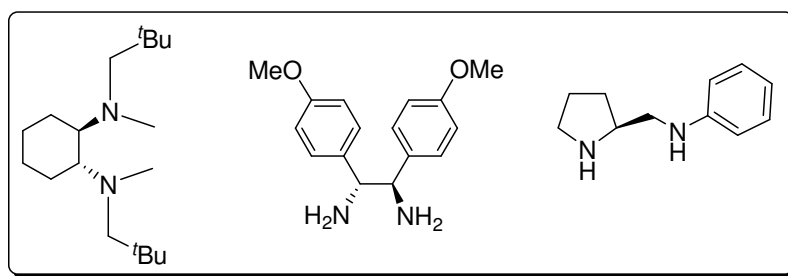
Figure 9. Examples to chiral 1,2-diamine ligands
