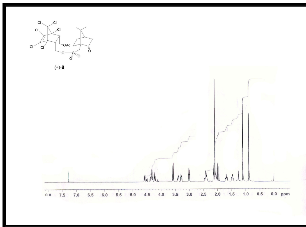
Figure A17. ^1\text{H} -NMR spectrum of the suphonate ester (+)- 8 .
