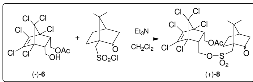
Scheme 13. The synthesis of the sulphonate ester (+)-8
