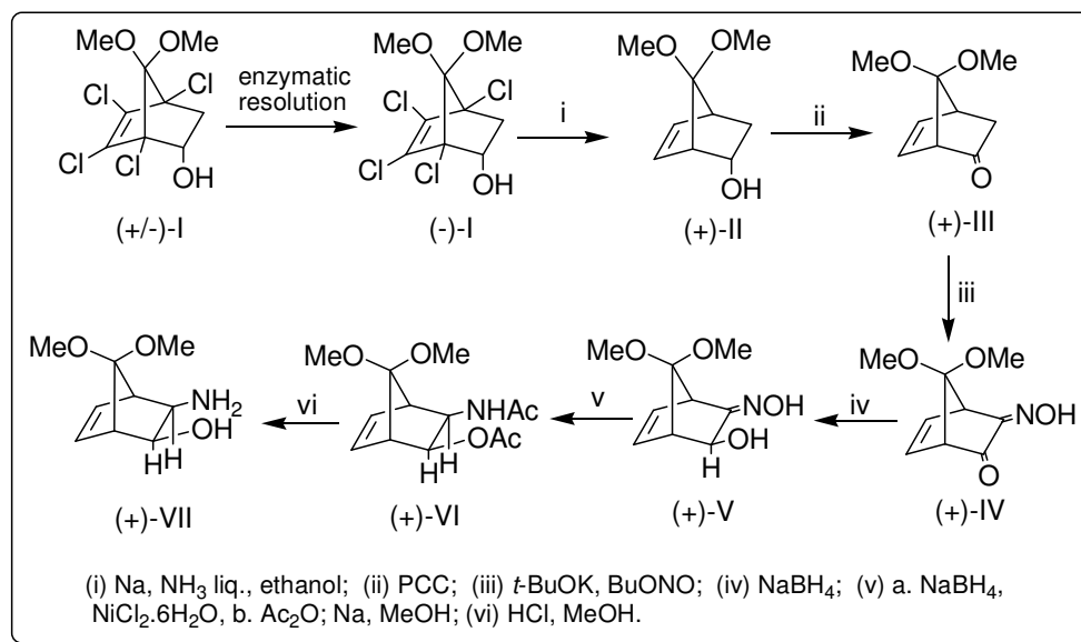
Scheme 4. The synthesis of a chiral ligand starting from a tetrachloro-dimethoxy norbornene derivative
