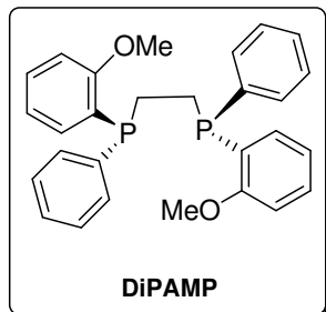
Figure 6. The structure of the chiral ligand DiPAMP
