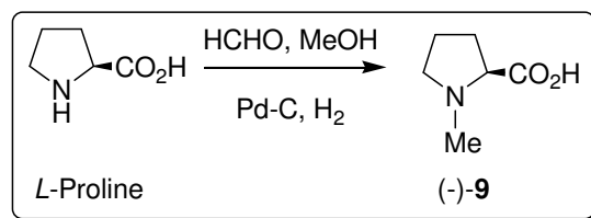
Scheme 14. The synthesis of N -methyl L-proline from L-proline
