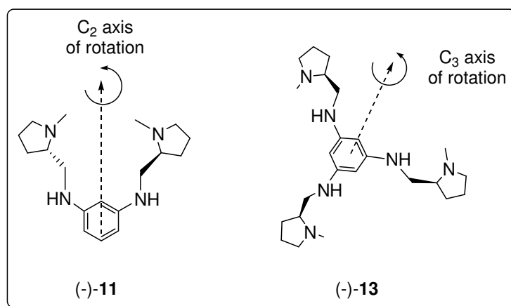
Figure 10. The structures of the target C_2 and C_3 ligands (-)- 11 and (-)- 13
