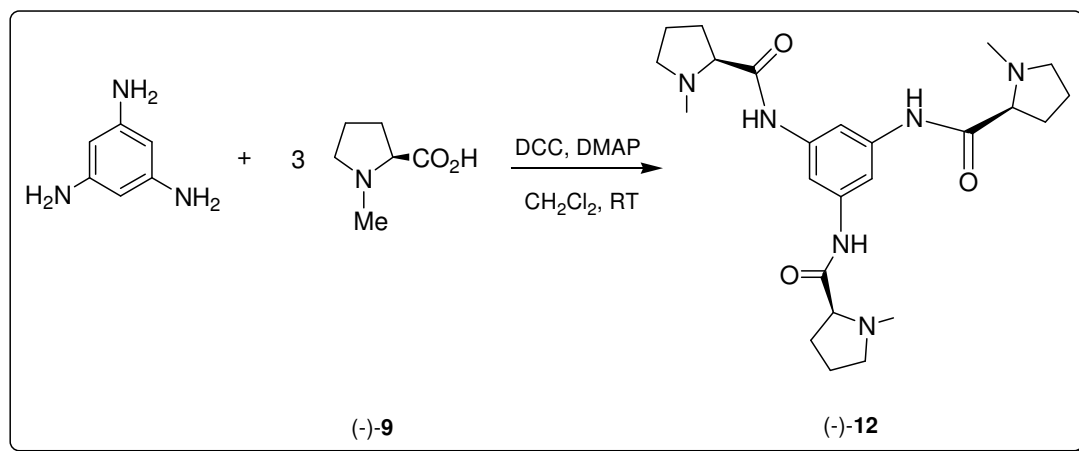
Scheme 16. The synthesis of the \text{C}_3 symmetric triamide (-)- 12
