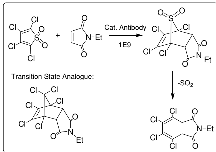
Scheme 3. Use of the catalytic antibody 1E9 in the model Diels-Alder reaction
