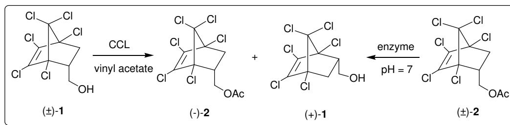
Scheme 8. General strategy for the enzymatic resolution of ( \pm )- 1 and ( \pm )- 2
