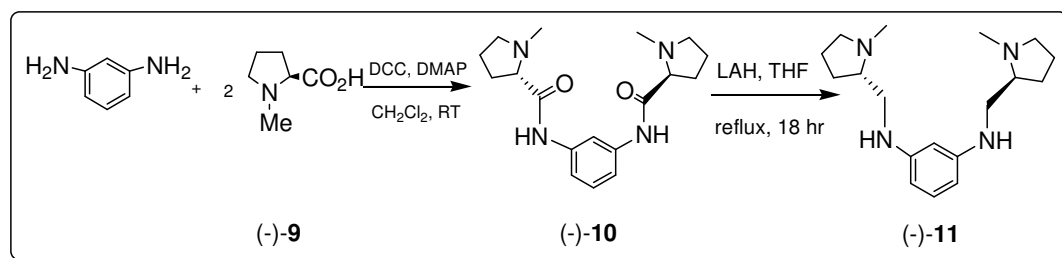
Scheme 15. The synthesis of the chiral diamine ligand (-)- 11
