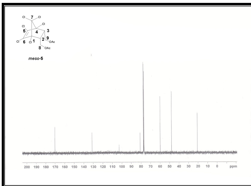
Figure A10. ^{13}\text{C} -NMR spectrum of meso -2,3- endo -bis(acetoxymethyl)-1,4,5,6,7,7-hexachlorobicyclo[2.2.1] hept-5-ene meso -5
