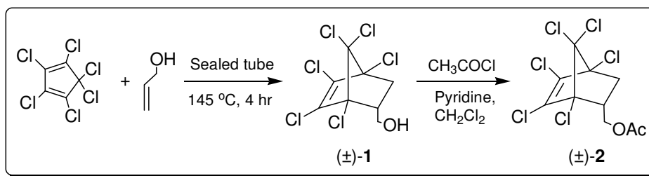
Scheme 5. The synthesis of (±)- 1 and (±)- 2
