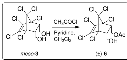
Scheme 7. The synthesis of (±)-6
