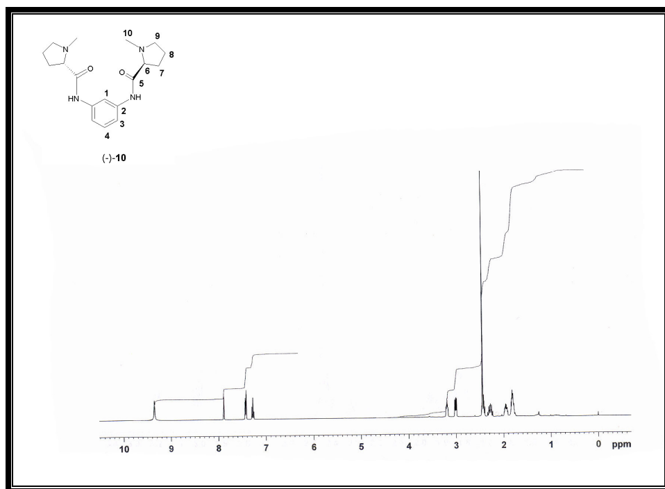
Figure A19. 1 H-NMR spectrum of the diamide derivative (-)-10
