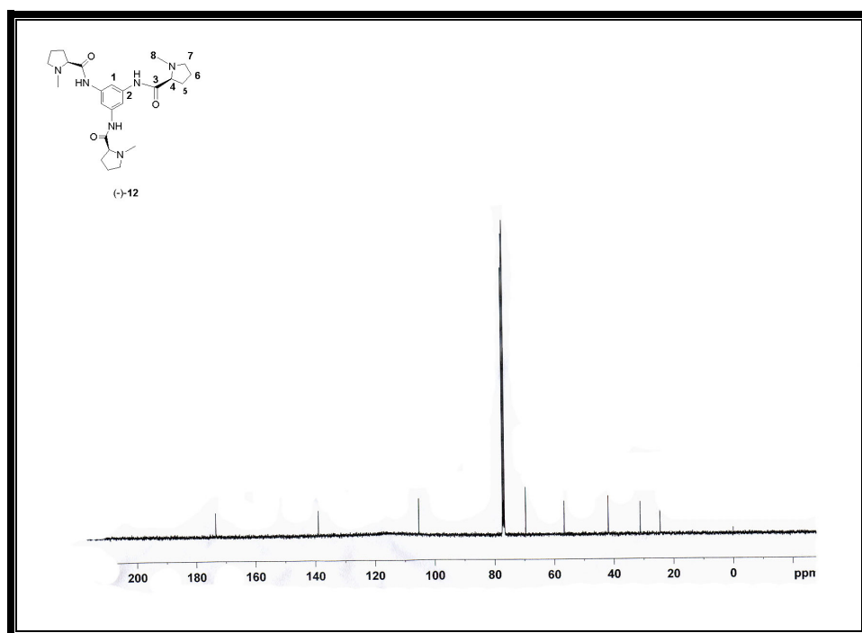
Figure A24. ^{13}\text{C} -NMR spectrum of the triamide derivative (-)-12
