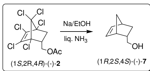
Scheme 9. Reductive dechlorination of (-)- 2
