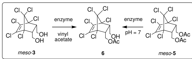
Scheme 10. General strategy for the enzymatic desymmetrization of meso -3 and meso -5
