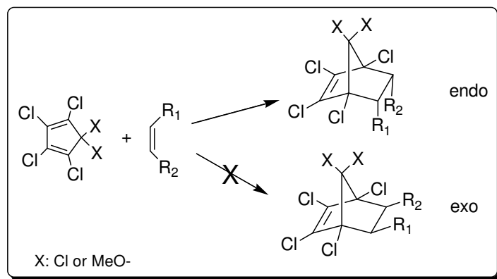
Scheme 1. Endo selective synthesis of polychlorinated norbornene derivatives
