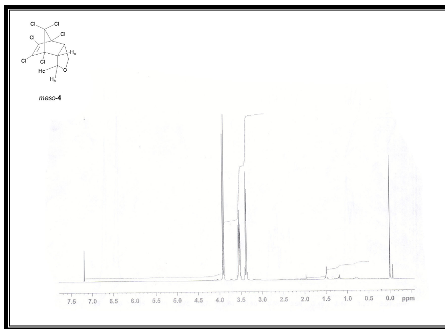
Figure A7. ^1\text{H} -NMR spectrum of meso -4-oxa-1,4,5,6,7,7-hexachlorotricyclo[5.2.1.0]dec-8-ene, meso -4
