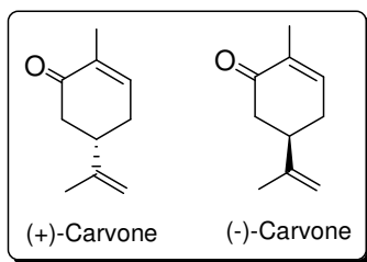
Figure 2. The structures of (+) and (-) Carvone
