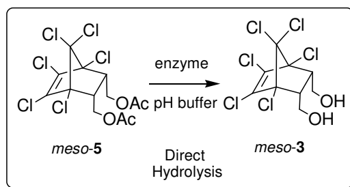
Scheme 11. Enzymatic hydrolysis of meso -5
