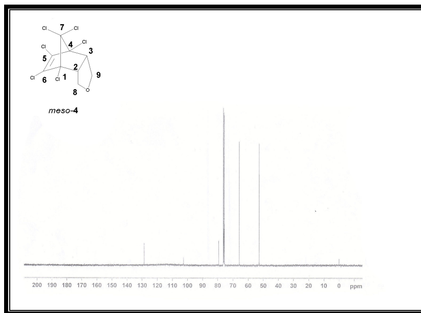
Figure A8. ^{13}\text{C} -NMR spectrum of meso -4-oxa-1,4,5,6,7,7-hexachlorotricyclo[5.2.1.0]dec-8-ene, meso -4
