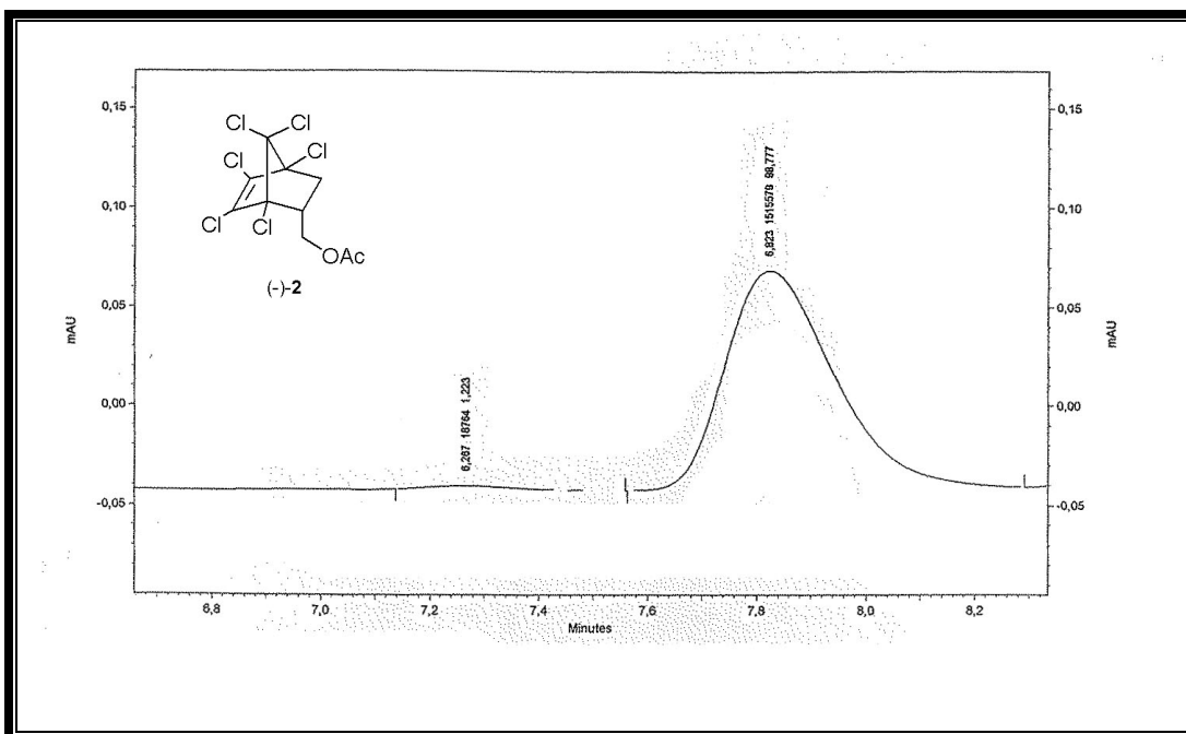
Figure A14. HPLC chromatogram of enantio-enriched acetoxymethyl derivative (-)-2
