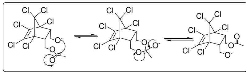
Scheme 12. Mechanism of the racemization of (-)- 6 in basic medium
