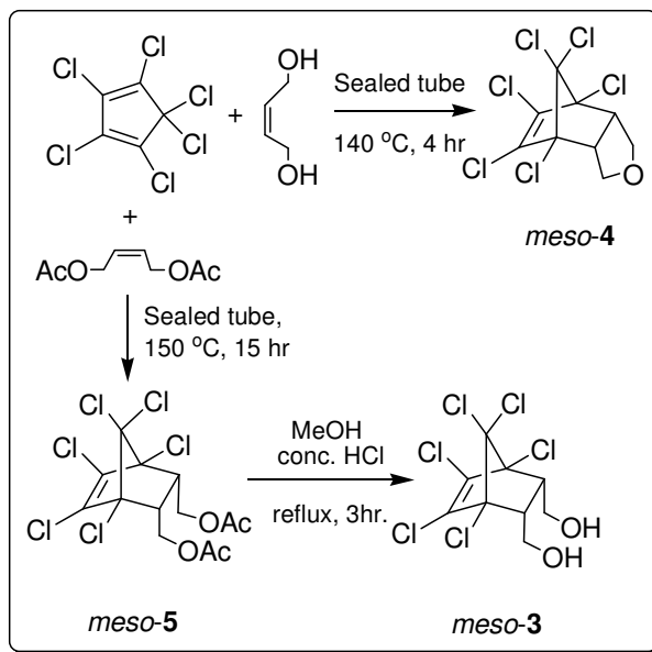
Scheme 6. The synthesis of meso-3 , meso-4 and meso-5
