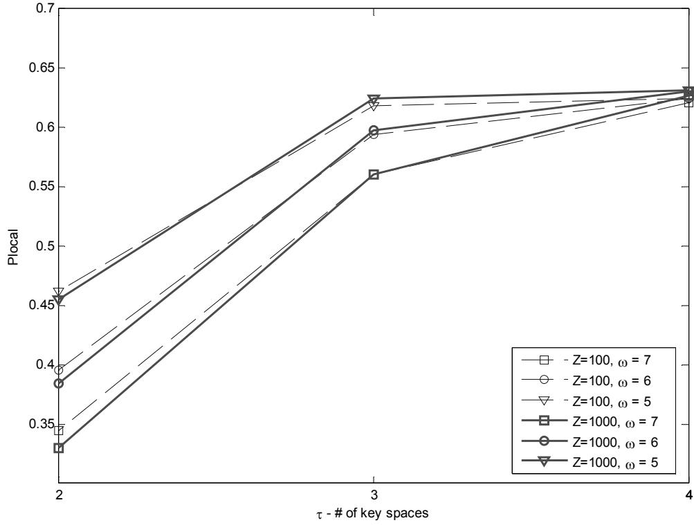
Figure 4-19 Local connectivity for our scheme when Z=100 and Z=1000
