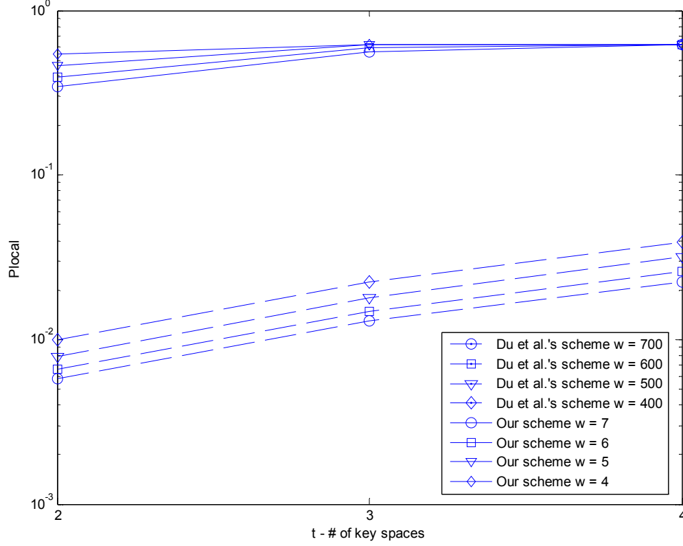
Figure 4-1 Local connectivity, P_{local} , vs. \tau , # of key spaces installed in a node
