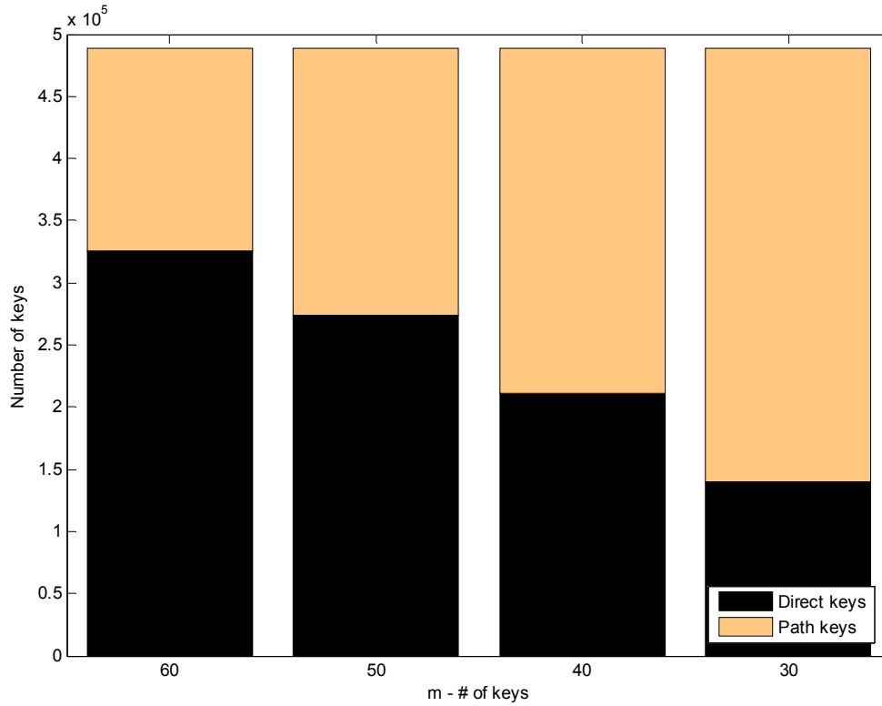
Figure 4-15 Number of keys established in Du et al's scheme 2. Path keys use flooding.
