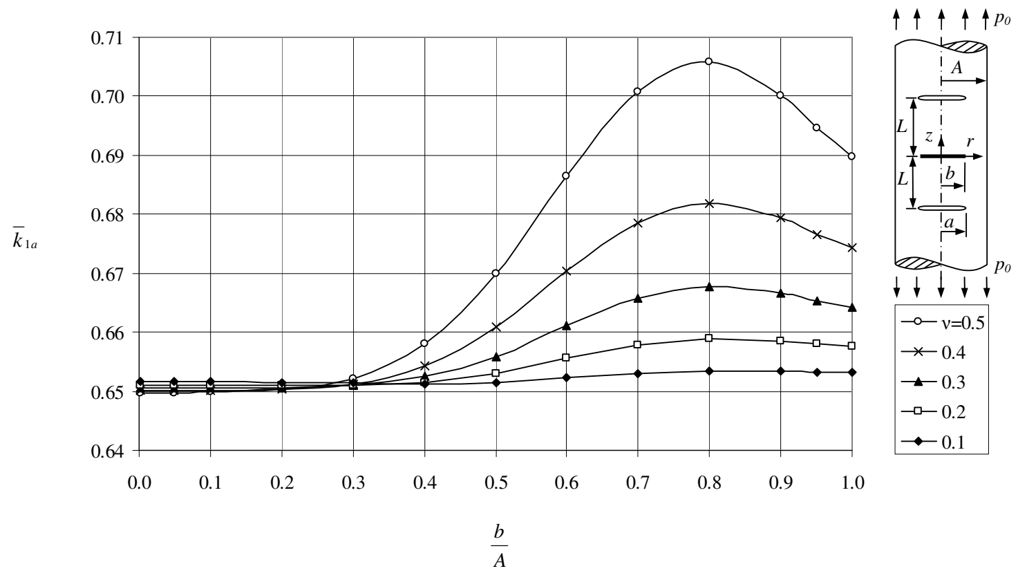
Figure 6.25 Normalized Mode I stress intensity factor \bar{k}_{Ia} when a = L = 0.5A .
