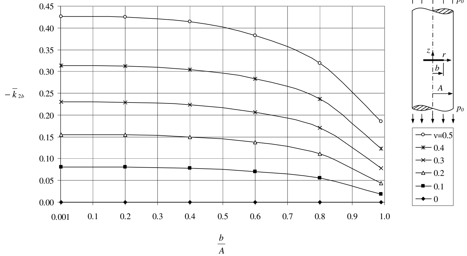
Figure 6.2 Normalized Mode II stress intensity factor \bar{k}_{2b} at the inclusion edge.
