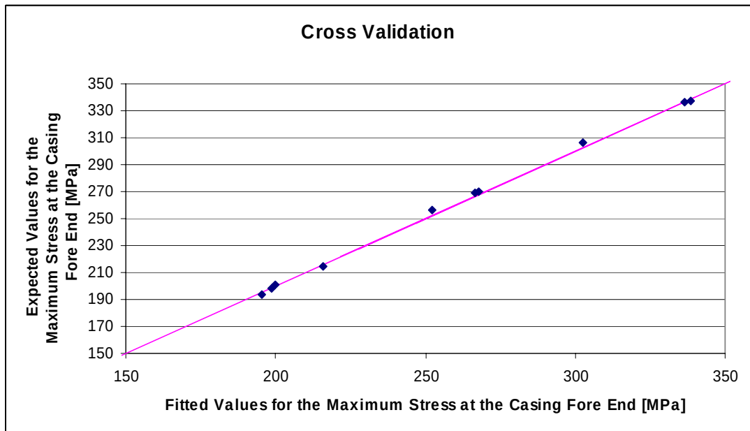
Figure 6.22. Cross validation of the response function for maximum stress at the casing fore end
