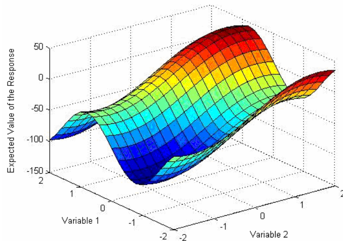
Figure 4.7. Response surface example for two variables
