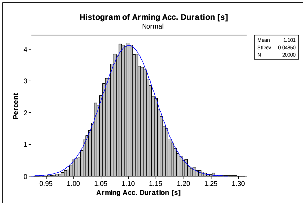
Figure 6.15. Distribution of arming acceleration duration at +60°C
