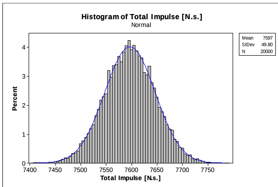
Figure D.7. Distribution of the total impulse at -35°C
