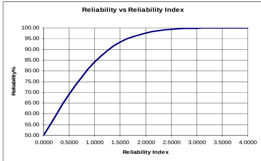
Figure 4.2. Reliability vs. Reliability Index
