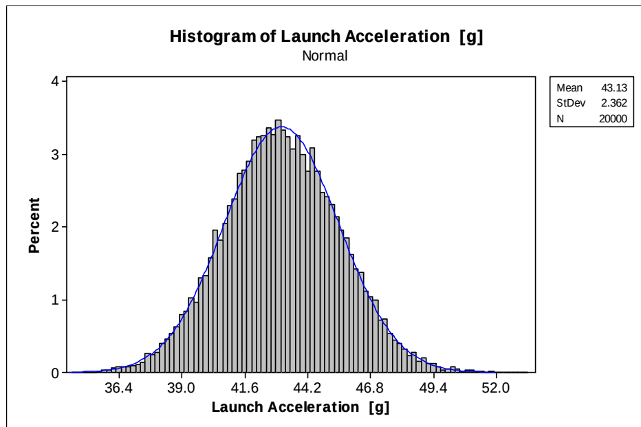
Figure D.10. Distribution of launch acceleration at -35°C
