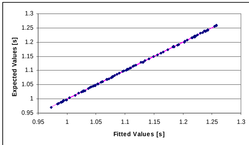
Figure 6.11. Expected vs. Fitted values for arming acceleration duration (Max. absolute error = 0.0023)
