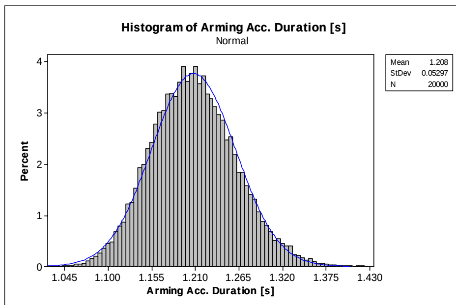
Figure D.3. Distribution of arming acceleration duration at 20°C
