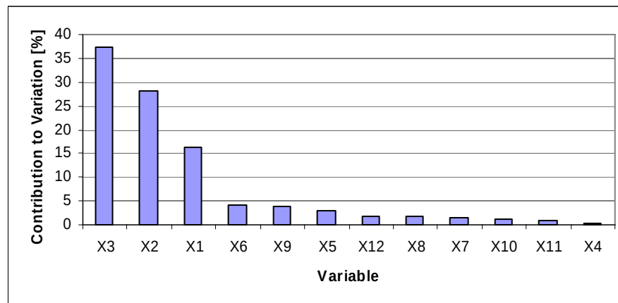
Figure 6.33. Sensitivity of variation in total impulse
