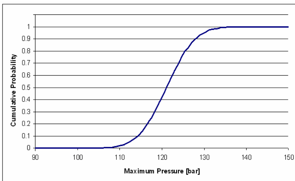
Figure 6.27. CDF of maximum pressure at 60°C
