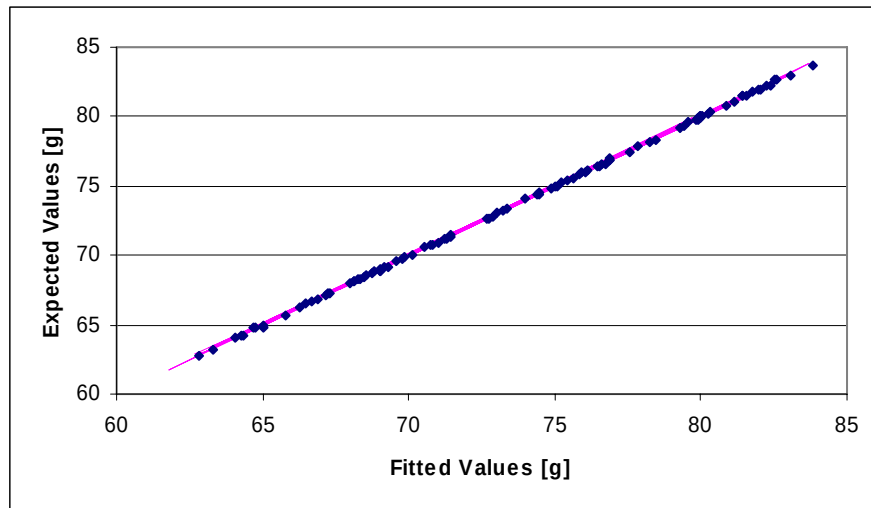
Figure B.6. Expected vs. Fitted values for the response function of maximum acceleration [g] at -35 °C (Maximum Absolute Error = 0.187)
