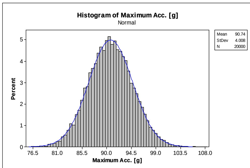
Figure 6.14. Distribution of maximum acceleration at +60°C
