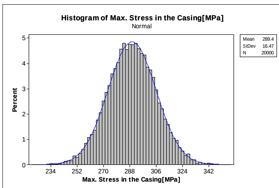
Figure D.5. Distribution of maximum stress at 20°C
