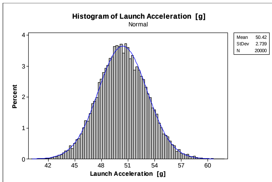
Figure D.4. Distribution of launch acceleration at 20°C
