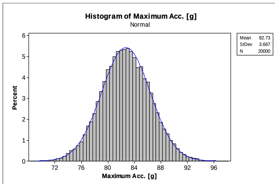
Figure C.2. Distribution of maximum acceleration at 20°C
