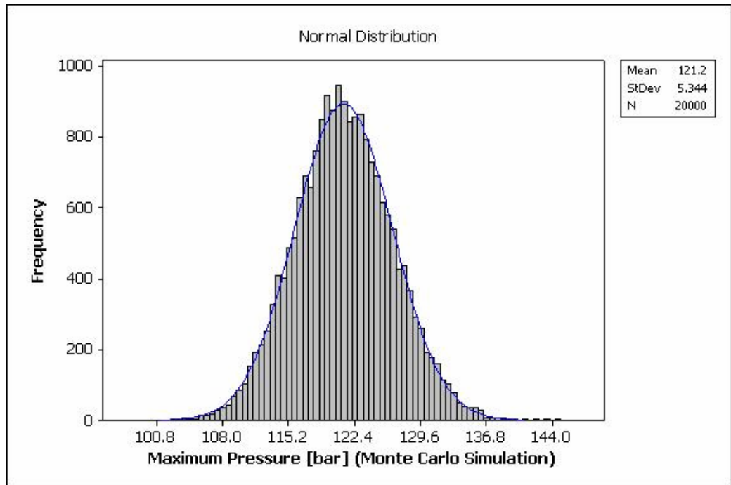
Figure 6.1. Maximum pressure distribution with Normal Distribution Curve
