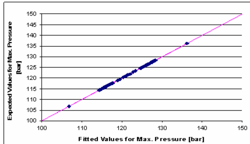
Figure 6.7. Expected vs. Fitted values for CCC Design with 1/32 fraction at response surface Design Points
