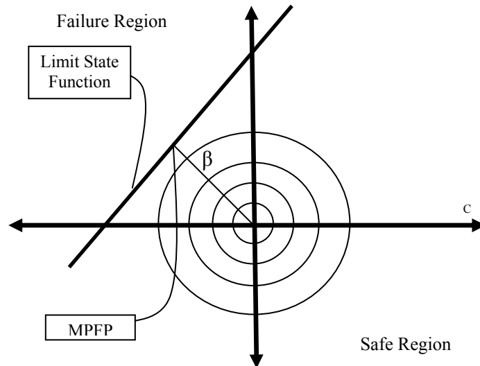
Figure 4.4. Variable space after transformation
