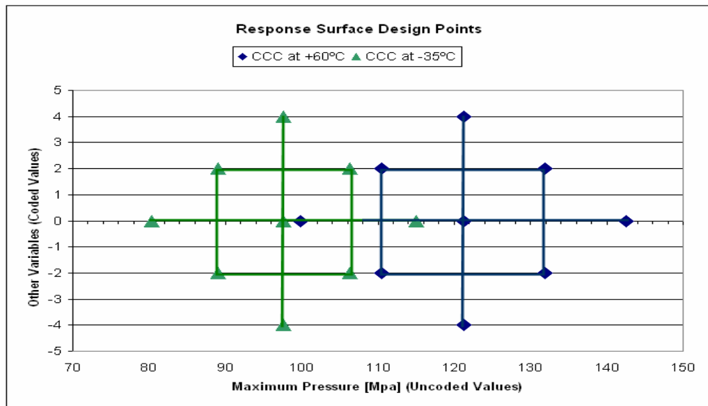
Figure 6.18. Response surface data points for the maximum stress estimation
