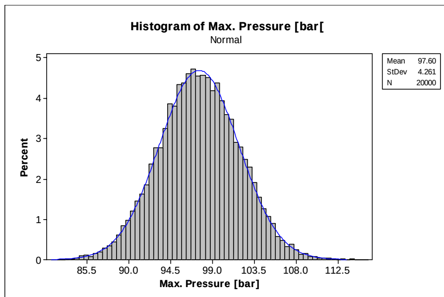
Figure D.12. Distribution of maximum pressure at -35°C
