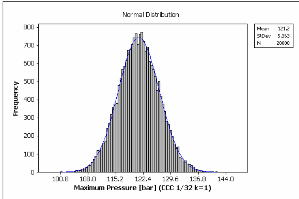
Figure 6.6. Distribution of maximum pressure (simulation with CCC 1/32 Fraction k=1 )
