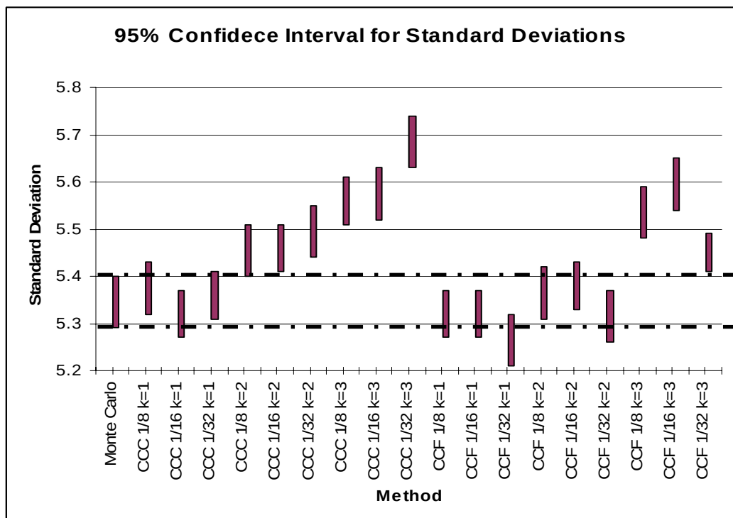
Figure 6.5. 95% Confidence intervals for estimated standard deviations with different RS methods
