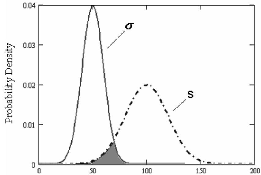
Figure 3.3. Unreliability region for normal distributed stress and strength (\sigma=N(50,10), S=N(100,20))
