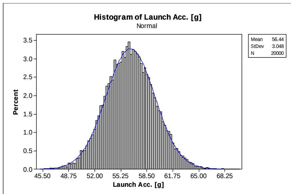
Figure 6.16. Distribution of launch acceleration at +60°C
