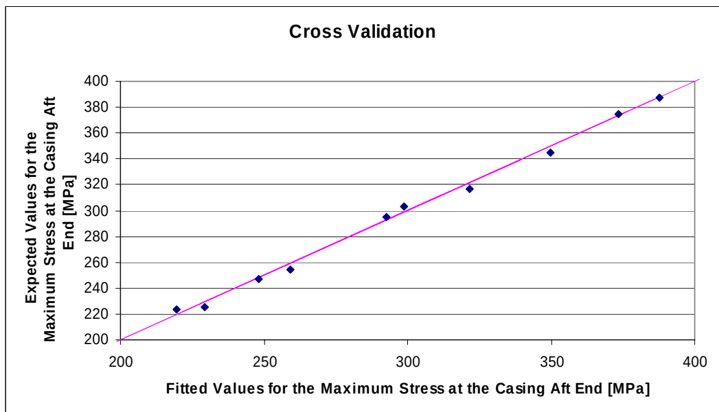
Figure 6.23. Cross validation of the response function for maximum stress at the casing aft end
