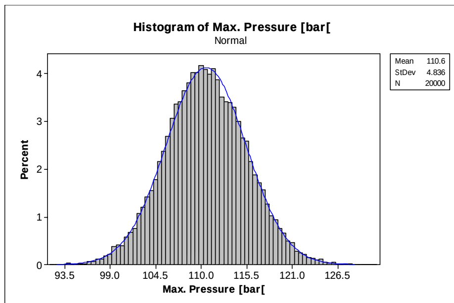
Figure D.6. Distribution of maximum pressure at 20°C
