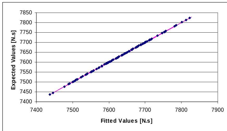
Figure B.1. Expected vs. Fitted values for the response function of total impulse [N.s] at 20°C (Maximum Absolute Error = 1.014)
