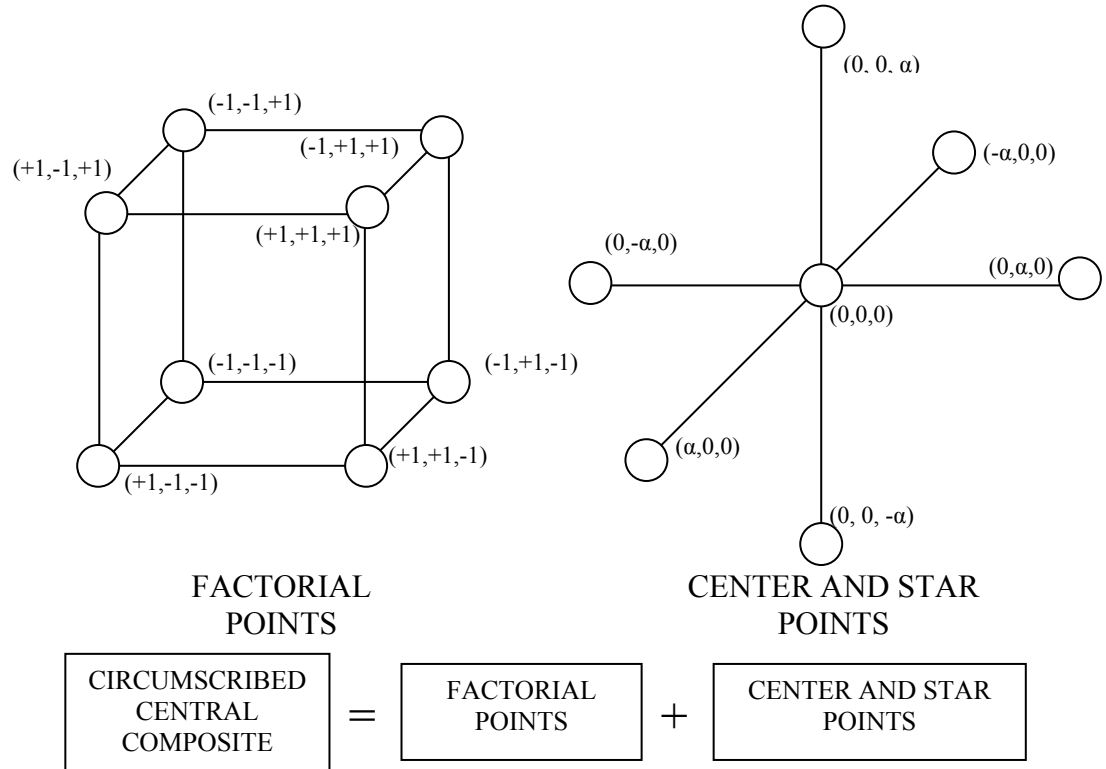
Figure 4.10. Central Composite Circumscribed (CCC) Design
