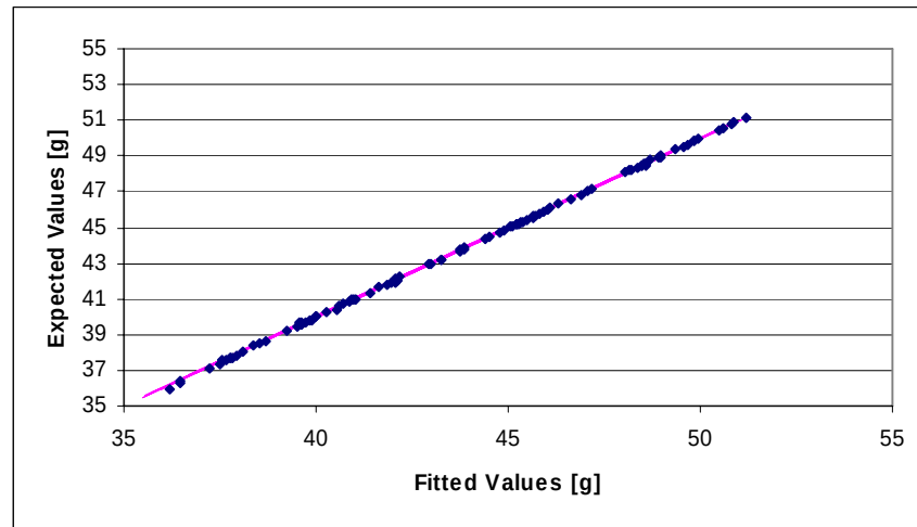
Figure B.8. Expected vs. Fitted values for response function of launch acceleration at -35 °C (Maximum Absolute Error = 0.222)
