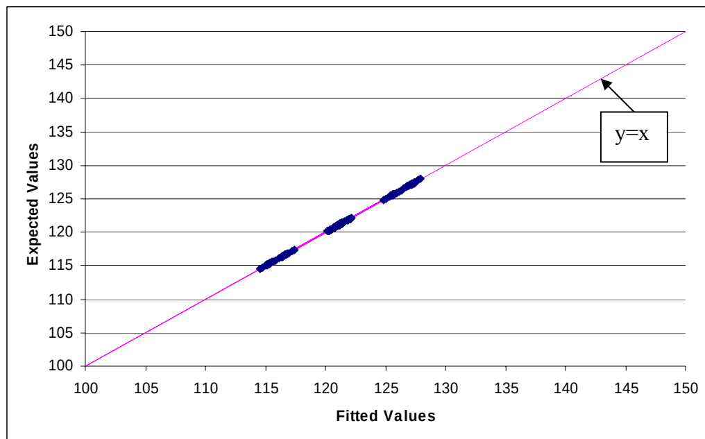
Figure 6.2. Expected vs. Fitted values for Box-Behnken design at response surface design points
