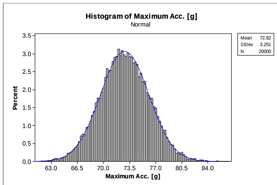
Figure D.8. Distribution of maximum acceleration at -35°C
