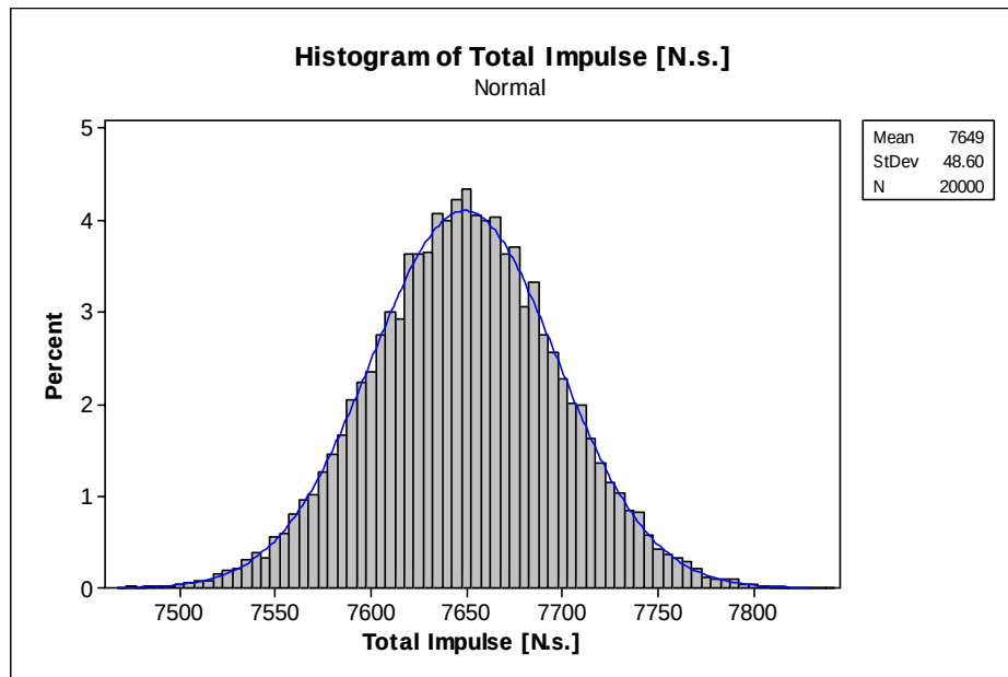
Figure D.1. Distribution of the total impulse at 20°C
