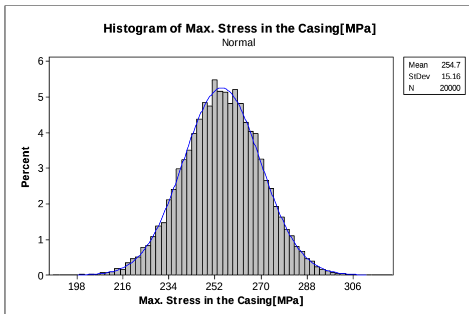
Figure D.11. Distribution of maximum stress at -35°C
