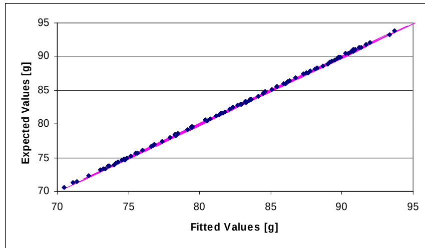
Figure B.2. Expected vs. Fitted values for the response function of maximum acceleration [g] at 20°C (Maximum Absolute Error = 0.268)
