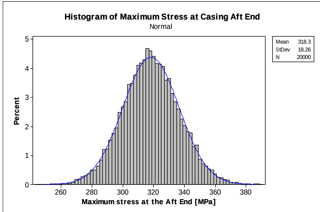
Figure 6.24. Distribution of maximum stress at the aft end (+60°C)
