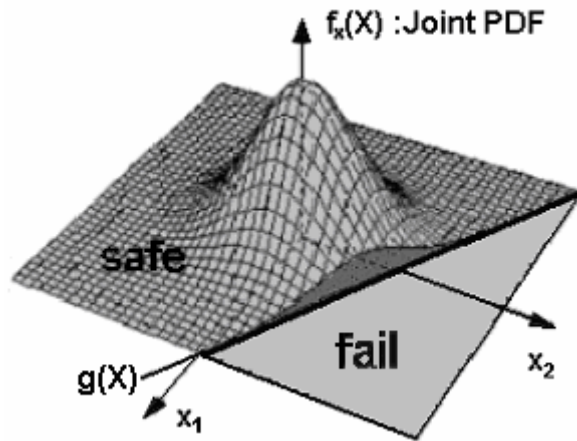
Figure 4.1. An example for Joint Probability Distribution and g(X)
