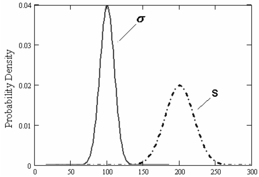
Figure 3.4. Unreliability region for normal distributed stress and strength (\sigma=N(100,10), S=N(200,20))
