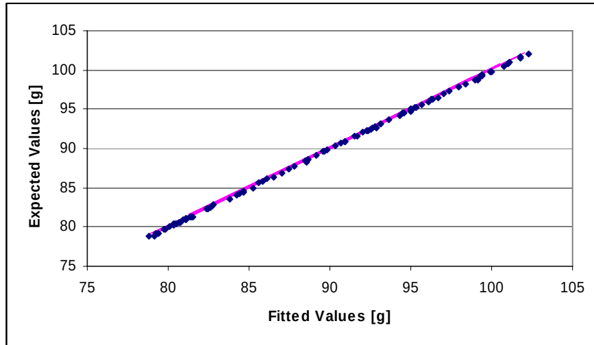
Figure 6.10. Expected vs. Fitted values for maximum acceleration (Max. absolute error = 0.358)
