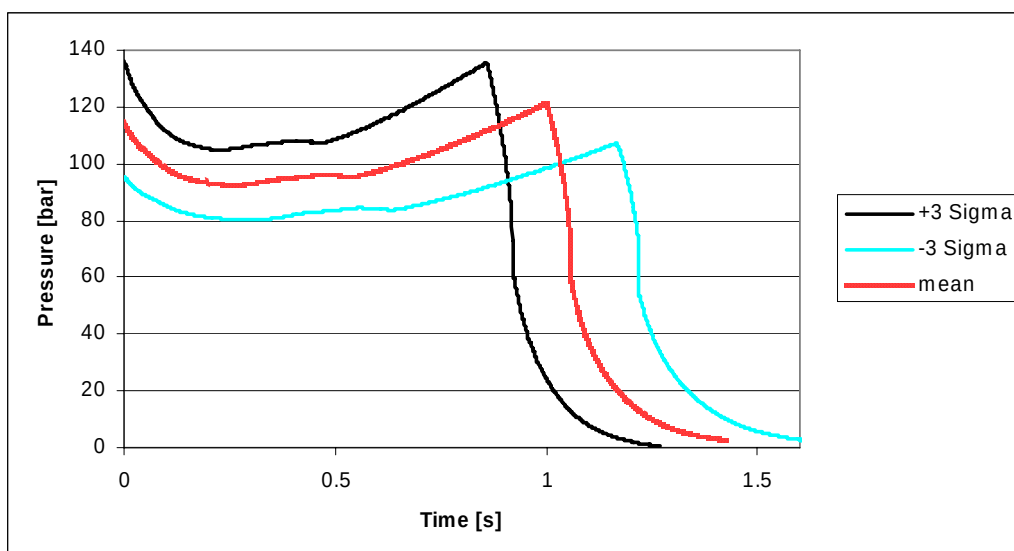
Figure 6.26. \pm 3\sigma limits for estimated pressure profile at 60°C
