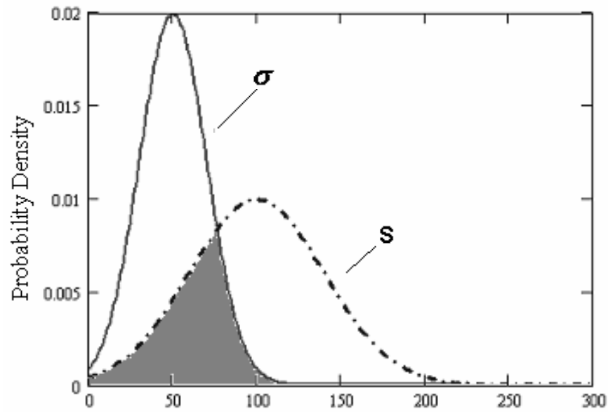
Figure 3.5. Unreliability region for normal distributed stress and strength (\sigma=N(50,20), S=N(100,40))
