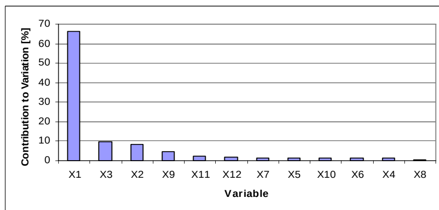
Figure 6.36. Sensitivity of variation in launch acceleration
