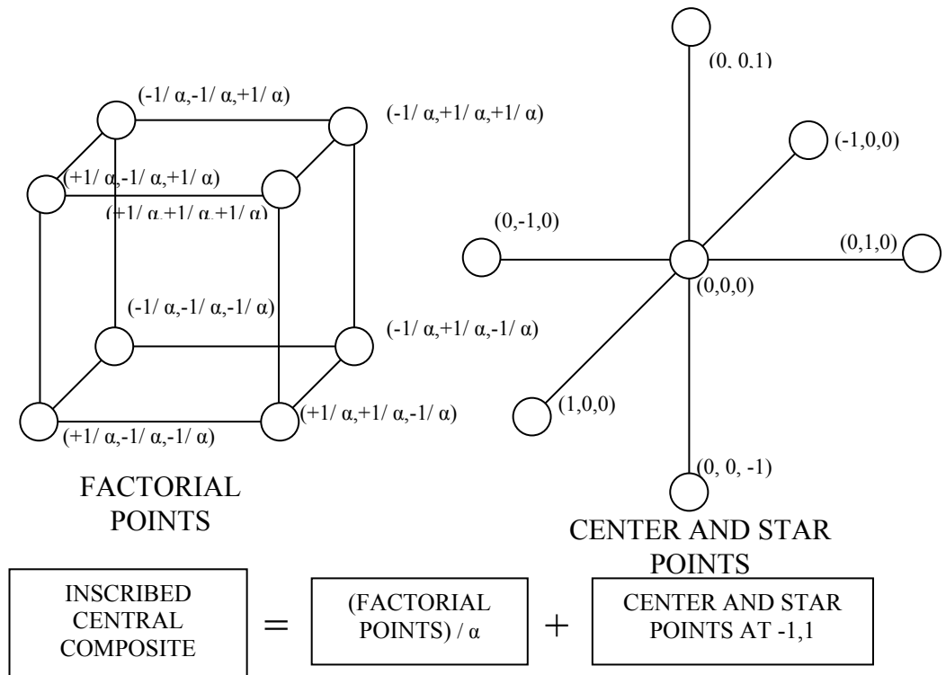
Figure 4.11. Central Composite Inscribe (CCI) Design
