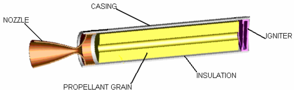
Figure 2.1. Solid rocket motor
