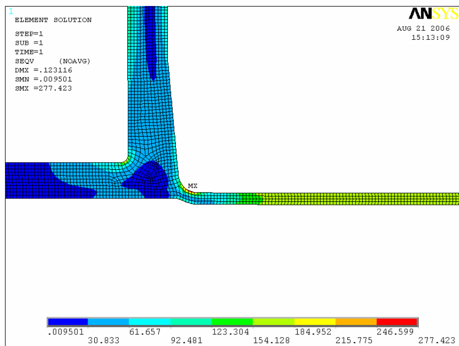
Figure 6.19. von Mises stresses for a sample run (fore end)
