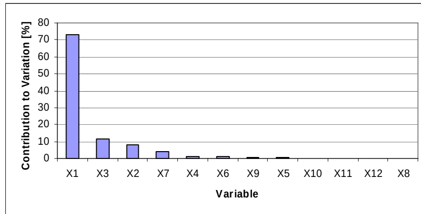
Figure 6.37. Sensitivity of variation in maximum pressure
