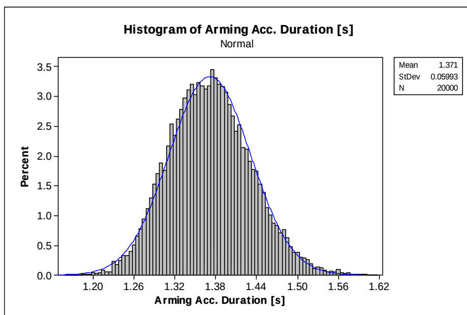
Figure D.9. Distribution of arming acceleration duration at -35°C
