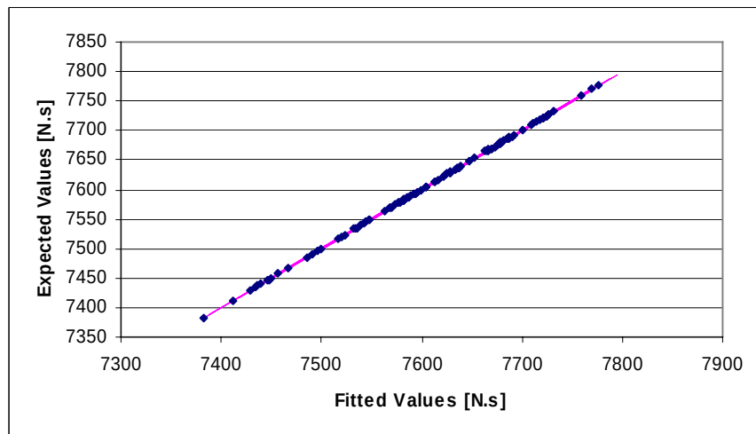
Figure B.5. Expected vs. Fitted values for the response function of the total impulse [N.s] at -35 °C (Maximum Absolute Error = 1.771)
