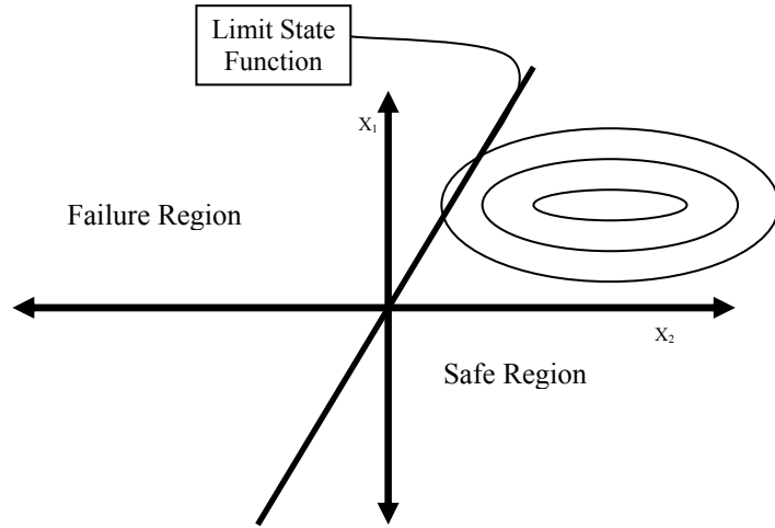
Figure 4.3. Variable space before transformation
