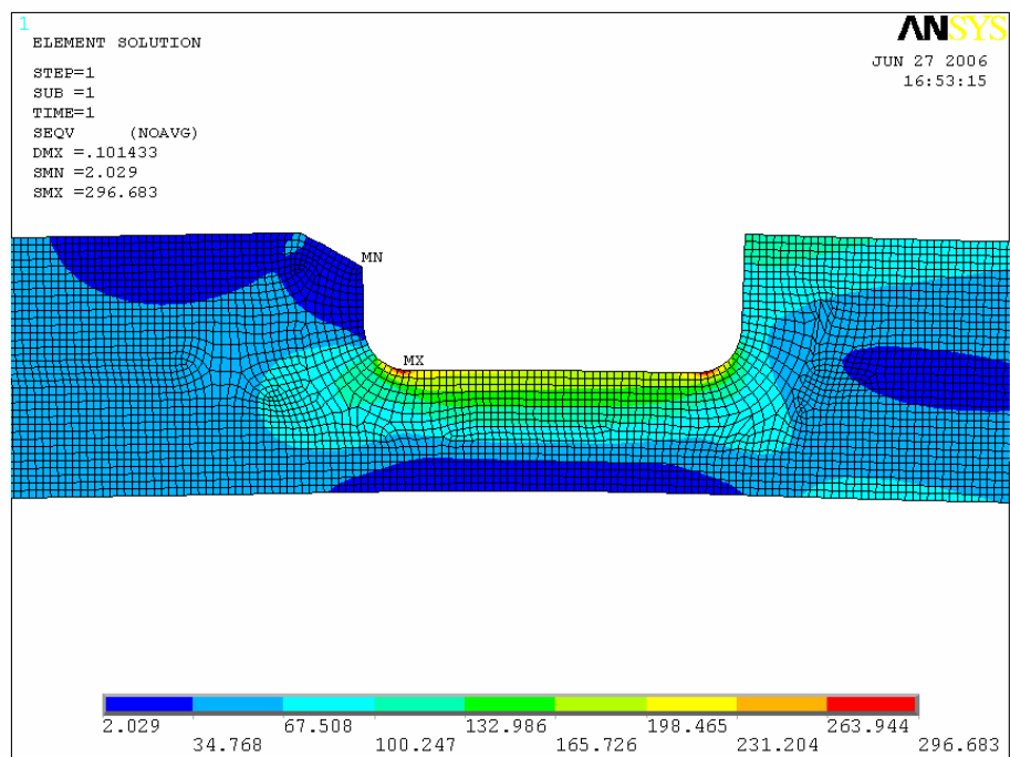
Figure 6.21. von Mises stresses for sample run (aft end)
