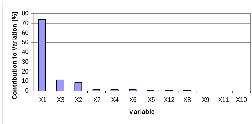
Figure 6.34. Sensitivity of variation in maximum acceleration
