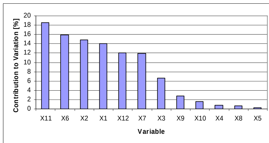
Figure 6.31. Sensitivity of launch acceleration
