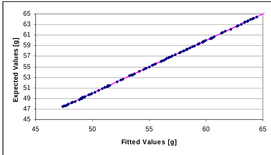
Figure 6.12. Expected vs. Fitted values for launch acceleration (Max. absolute error = 0.113)
