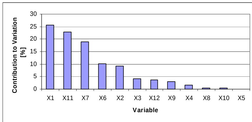
Figure 6.30. Sensitivity of arming acceleration duration
