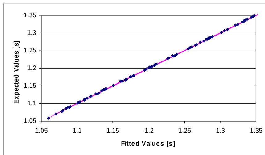
Figure B.3. Expected vs. Fitted values for the response function of arming acceleration duration [s] at 20°C (Maximum Absolute Error = 0.0038)
