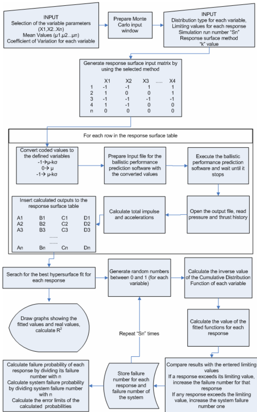
Figure 5.3. Flowchart for Monte Carlo simulation with response surface fitting
