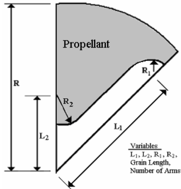
Figure 2.4. Parameters describing the star grain geometry
