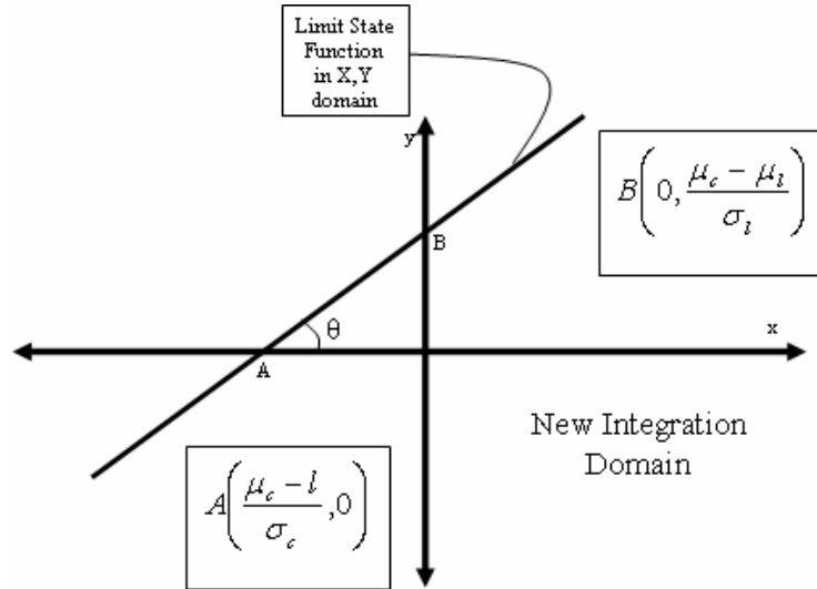
Figure A.2. New failure and safe region after converting C and L to standard normal distribution
