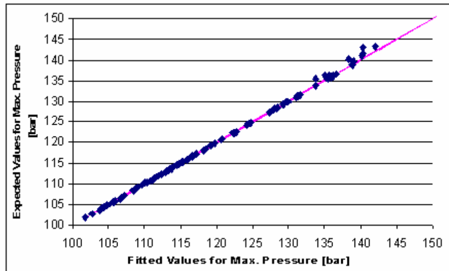
Figure 6.8. Expected vs. Fitted values for CCC Design with 1/32 fraction at random points (Cross Validation)
