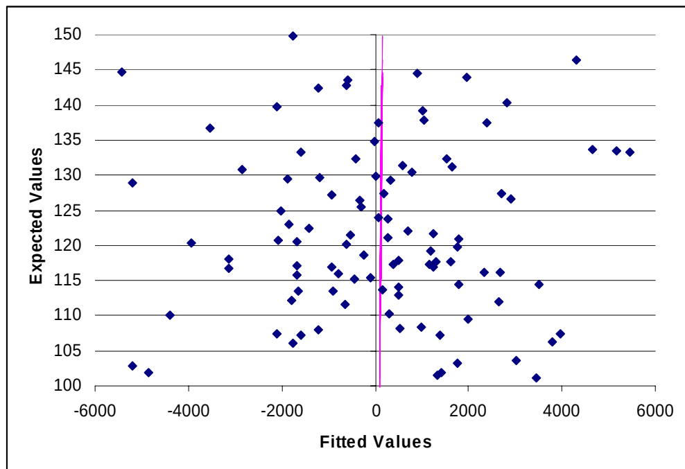
Figure 6.3. Expected vs. Fitted values for Box-Behnken design at random points
