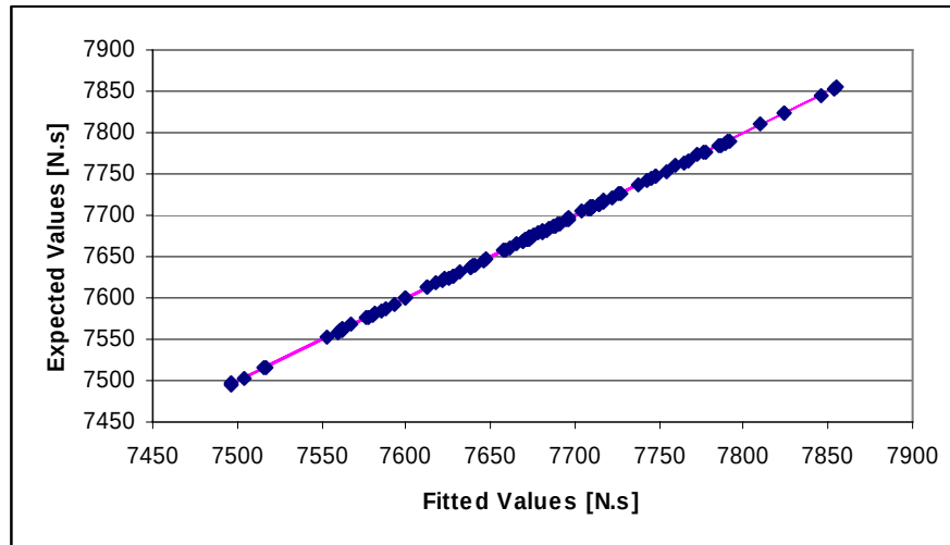
Figure 6.9. Expected vs. Fitted values for total impulse (Max. absolute error = 1.36)
