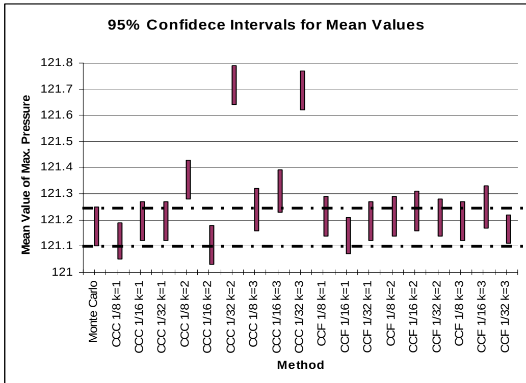
Figure 6.4. 95% Confidence intervals for estimated means with different RS methods
