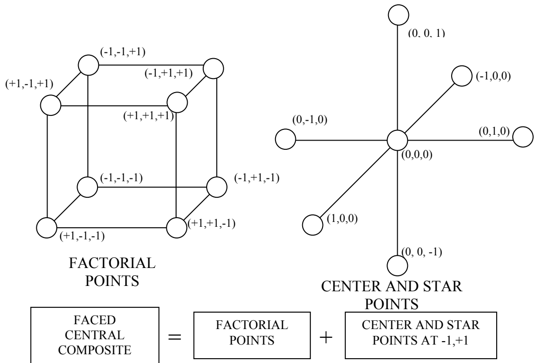
Figure 4.12. Central Composite Faced (CCF) Design
