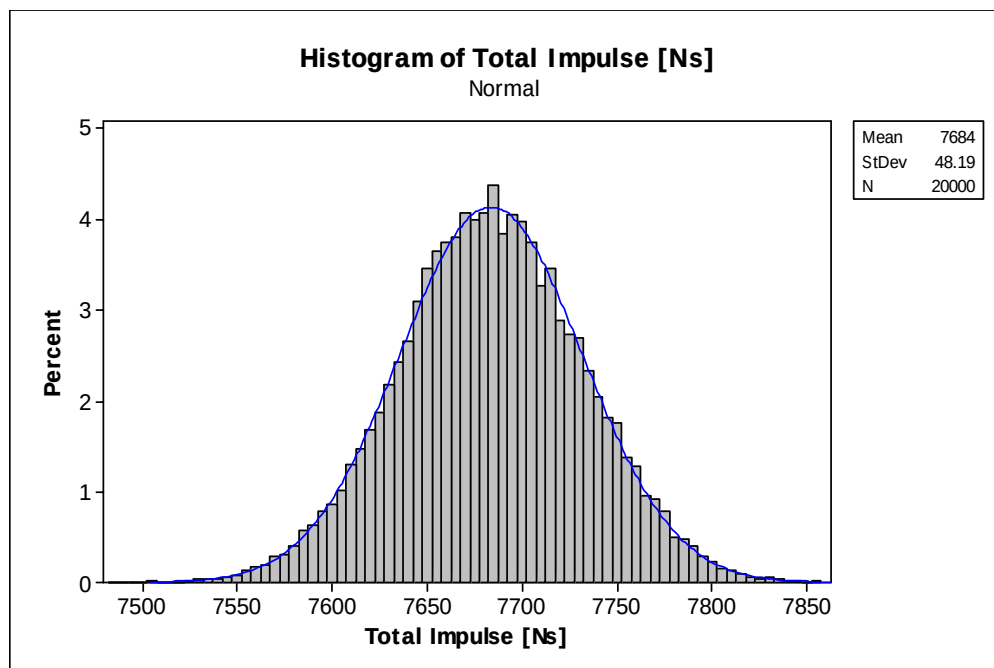
Figure 6.13. Distribution of total impulse at +60°C
