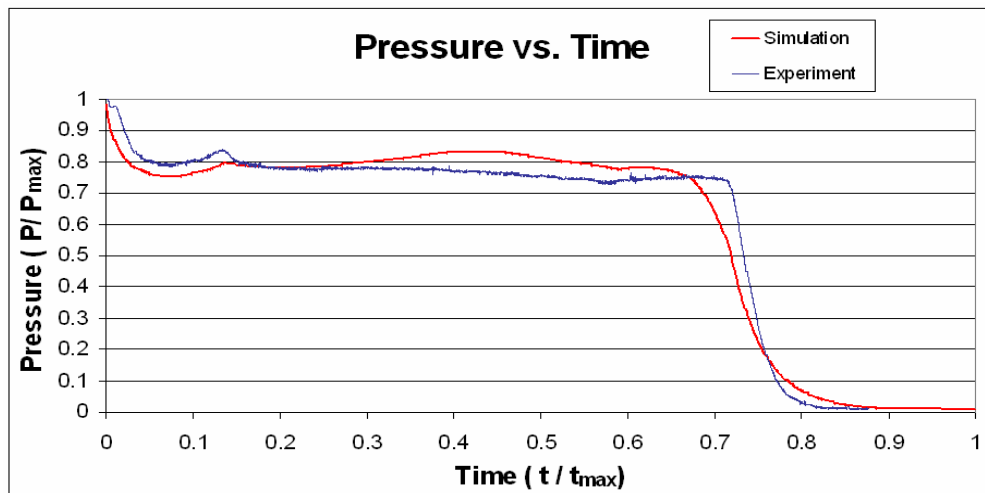
Figure 5.4. Comparison of Pressure vs. Time curve obtained from the experiment and simulation for a solid rocket motor
