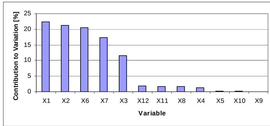
Figure 6.29. Sensitivity of maximum acceleration
