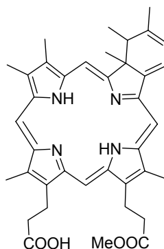
Figure 21: Structure of Benzoporphyrin derivate
