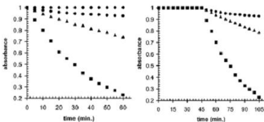
Figure 26: (A) (left) The change in the absorbance (at 415 nm) of 1,3 diphenylisobenzofuran (50 \mu\text{M} ) in 2-propanol under red-light illumination in the
