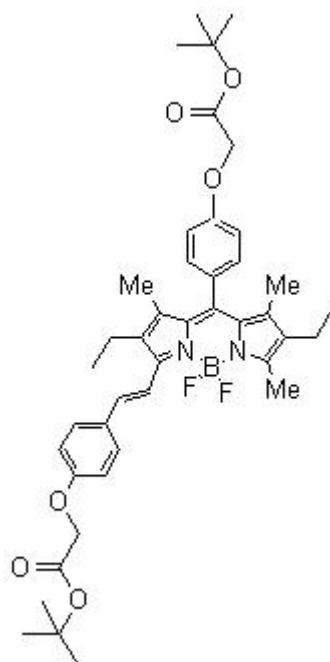
Figure 45: Structure of monostyryl BODIPY dyes ( 14 )
