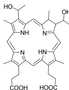
Figure 8: Structure of Haematoporphyrin
