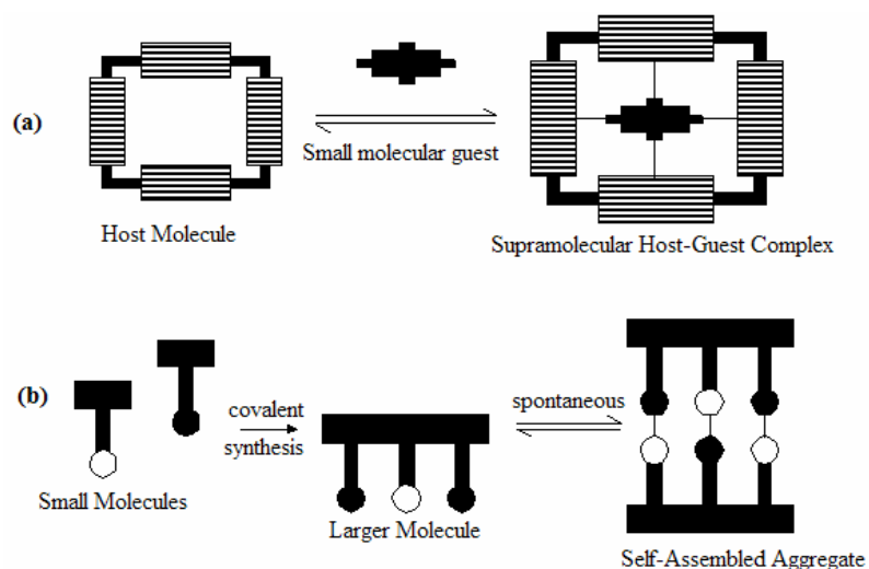
Figure 2: The development of a supramolecular system from molecular building blocks. (a) Host-guest complexation and (b) Assembly between complementary species (circles represent binding sites).
