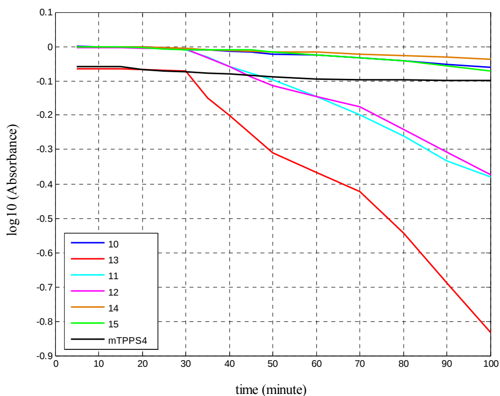
Figure 50: Comparative singlet oxygen generation of compounds 10-15 in \text{CHCl}_3 at 7.5 \mu\text{M} concentration.
