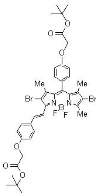
Figure 41: Structure of monostyryl BODIPY dyes ( 12 )
