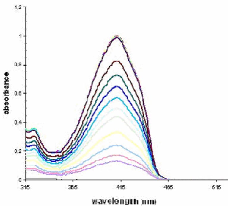
Figure 44: the change in the absorbance spectrum of 1,3-diphenyl- iso -benzofuran and compound ( 13 ) mixture on irradiation with light (625 nm)
