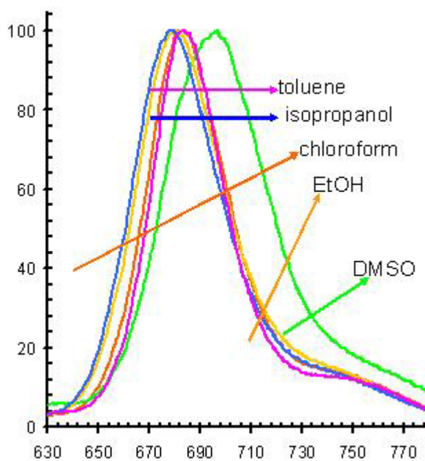
Figure 53: Normalized emission spectra of distyryl-BODIPY dye 13 in solvents of varying polarities. Excitation was at 610 nm, with 5 nm slit widths.
